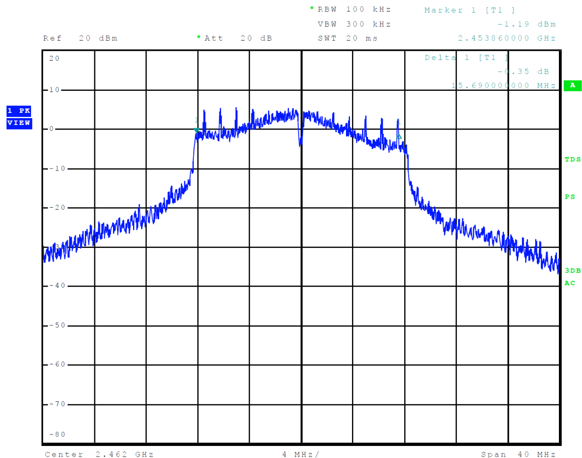
Figure 29 Plot of 6-dB Occupied Bandwidth Mode 6, 802.11g
