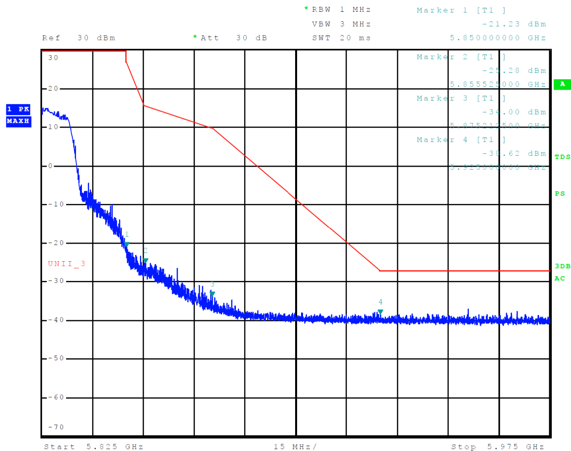
Figure 24 Plot of Upper Band Edge Across 5725-5850 MHz Mode 13 U-NII-3 (802.11n)
