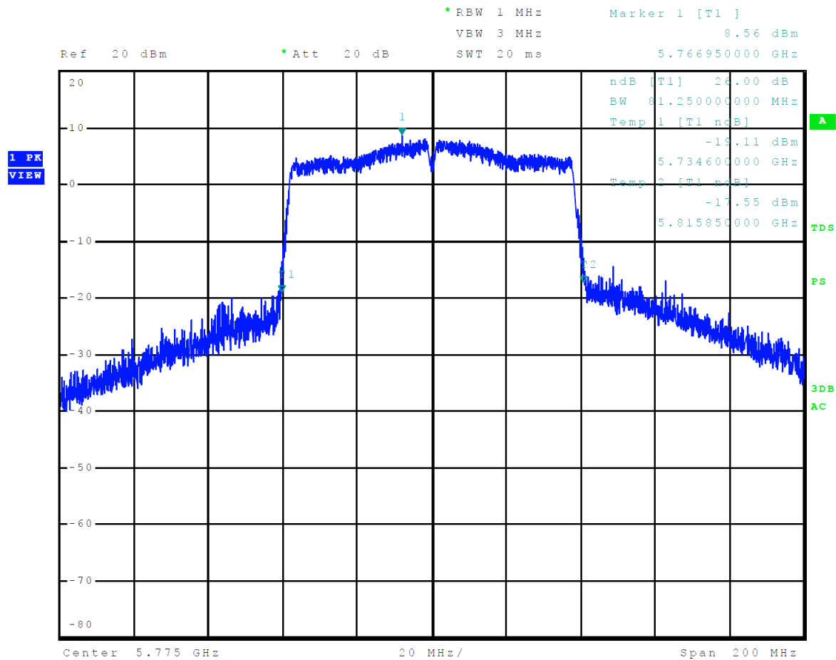
Figure 34 Plot of 26-dB Occupied Bandwidth 5725-5850 MHz Mode 15 U-NII-3 (802.11ac80)
