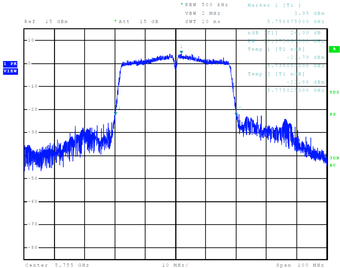
Figure 33 Plot of 26-dB Occupied Bandwidth 5725-5850 MHz Mode 14 U-NII-3 (802.11n40)
