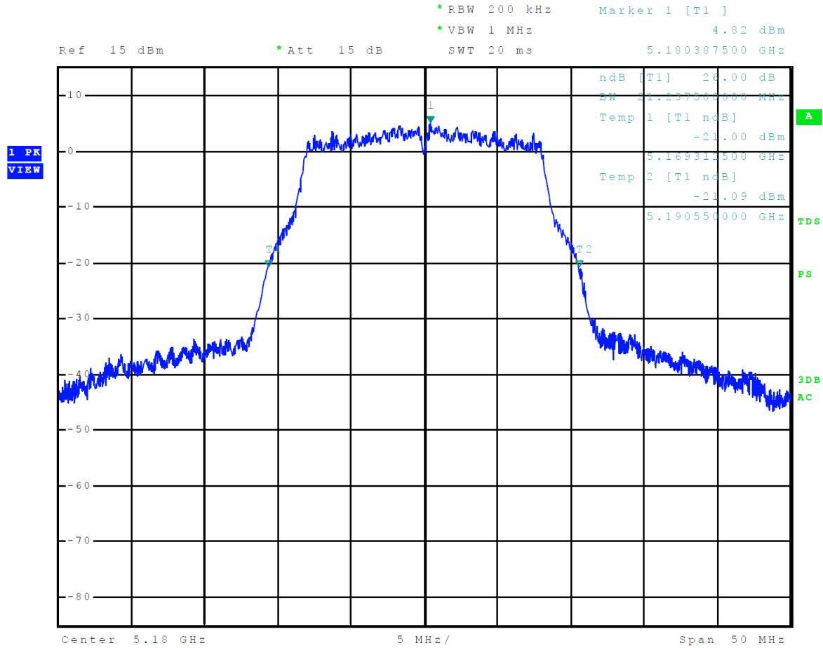
Figure 27 Plot of 26-dB Occupied Bandwidth 5150-5250 MHz Mode 8 U-NII-1 (802.11a)
