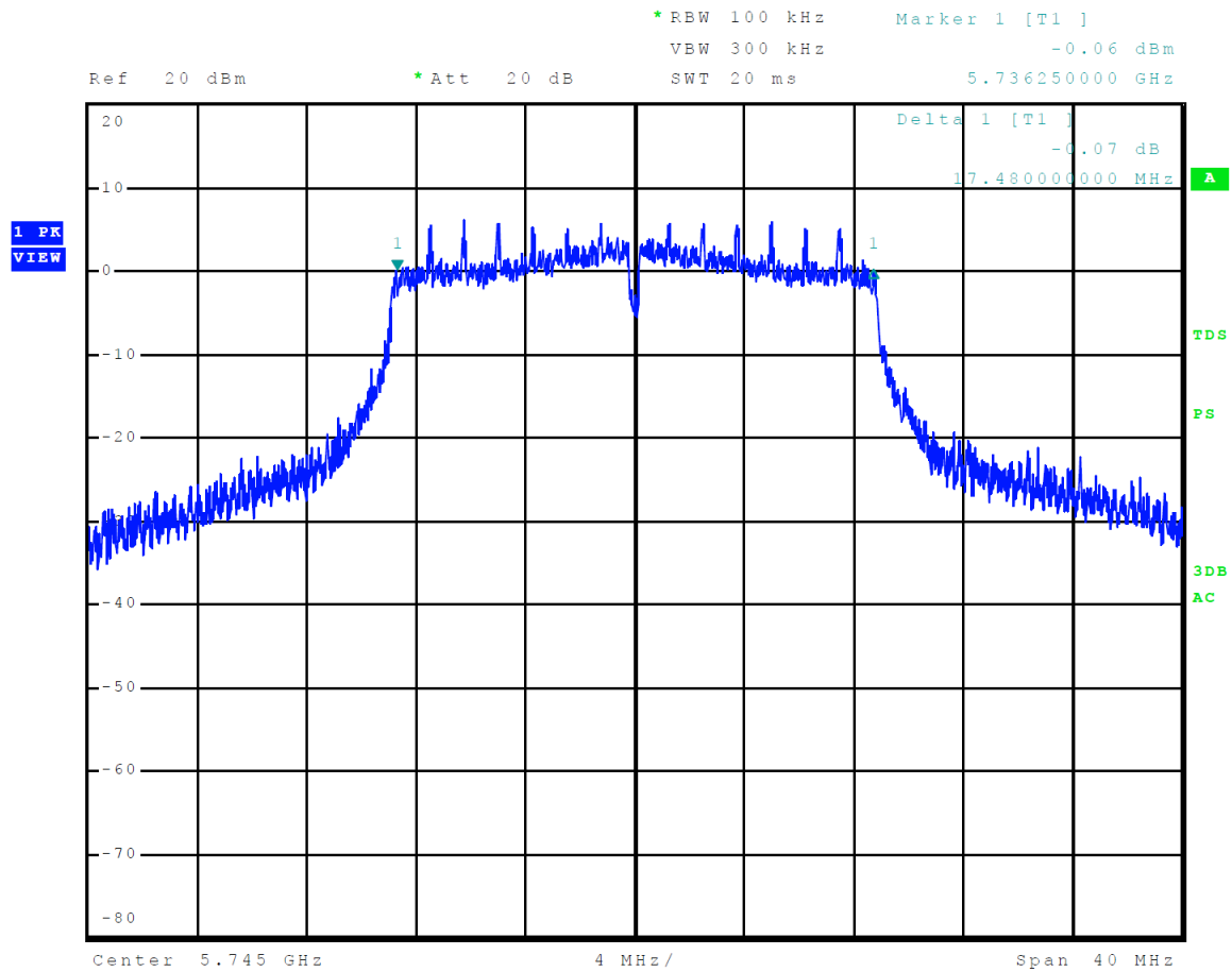
Figure 44 Plot of 6-dB Occupied Bandwidth 5725-5850 MHz Mode 13 U-NII-3 (802.11n)
