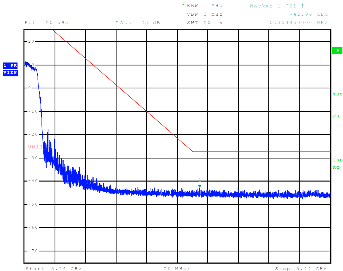
Figure 20 Plot of Upper Band Edge Across 5150-5250 MHz Mode 9 U-NII-1 (802.11n)
