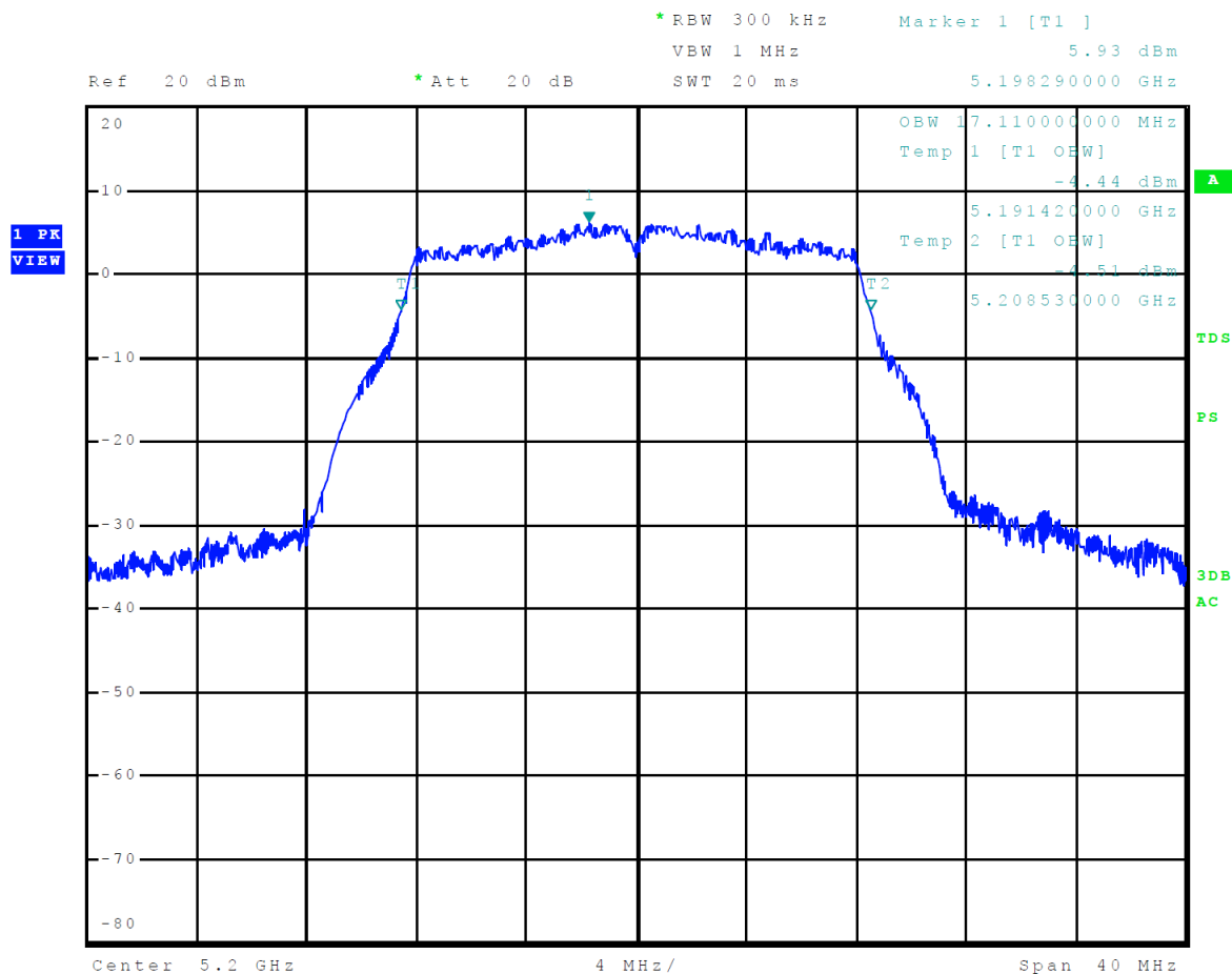
Figure 35 Plot of 99% Occupied Bandwidth 5150-5250 MHz Mode 8 U-NII-1 (802.11a)
