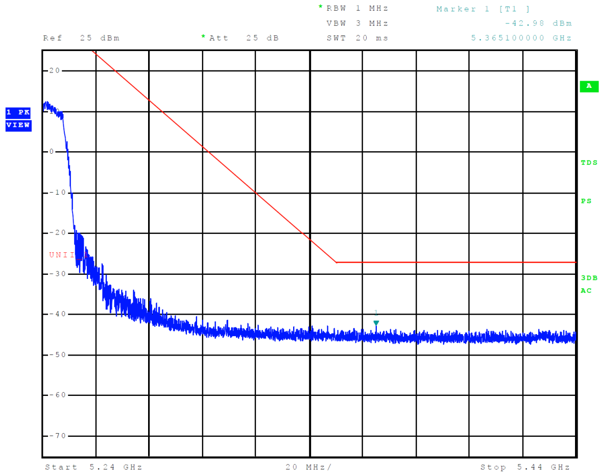
Figure 19 Plot of Upper Band Edge Across 5150-5250 MHz Mode 8 U-NII-1 (802.11a)
