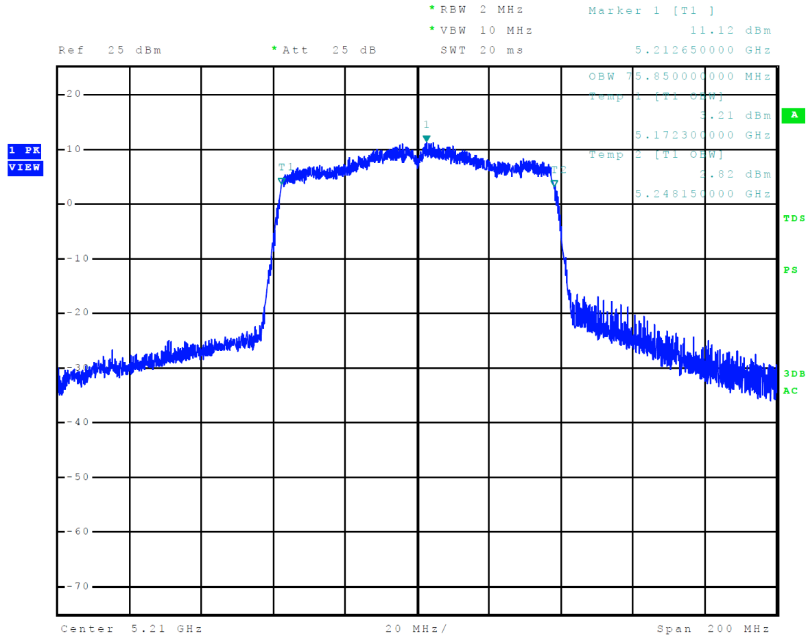
Figure 38 Plot of 99% Occupied Bandwidth 5150-5250 MHz Mode 11 U-NII-1 (802.11ac80)
