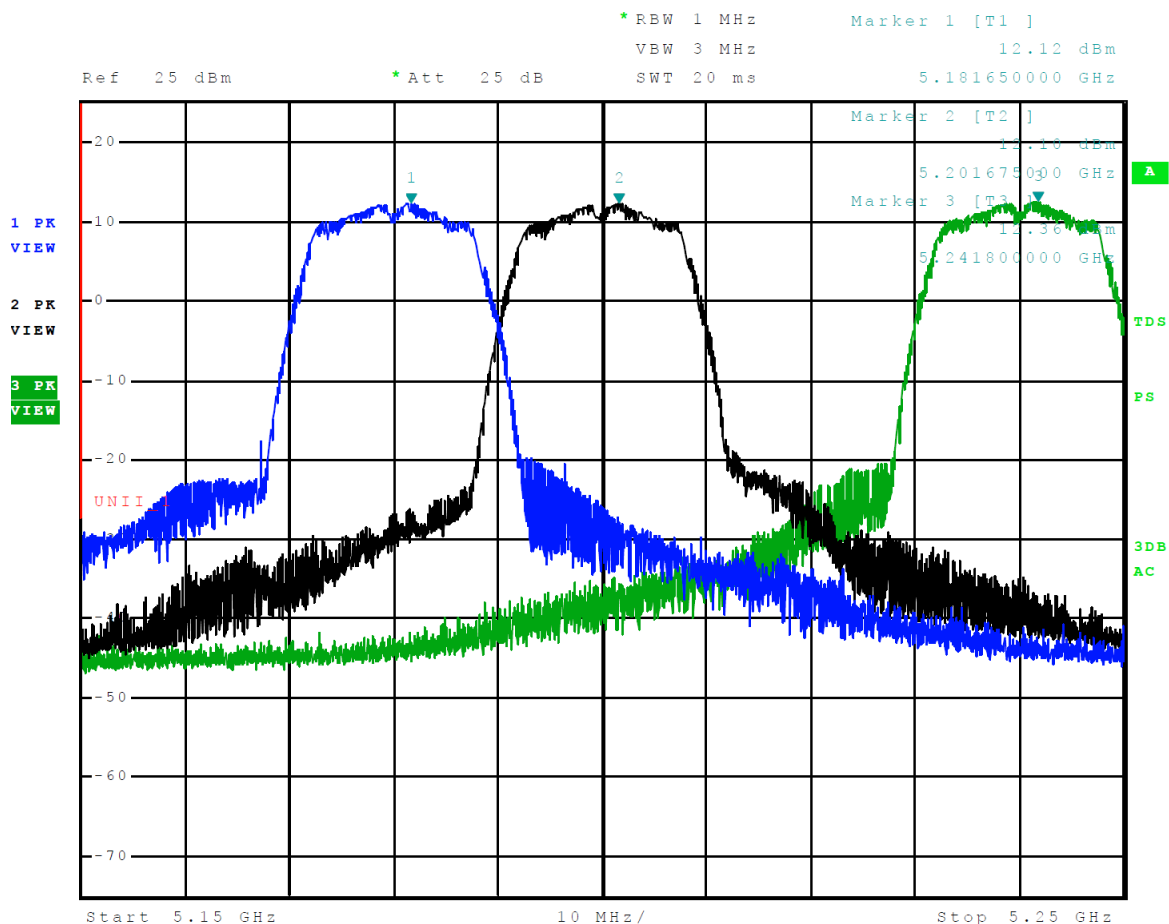
Figure 3 Plot of Transmitter Emissions Across 5150-5250 MHz Mode 8 U-NII-1 (802.11a)
