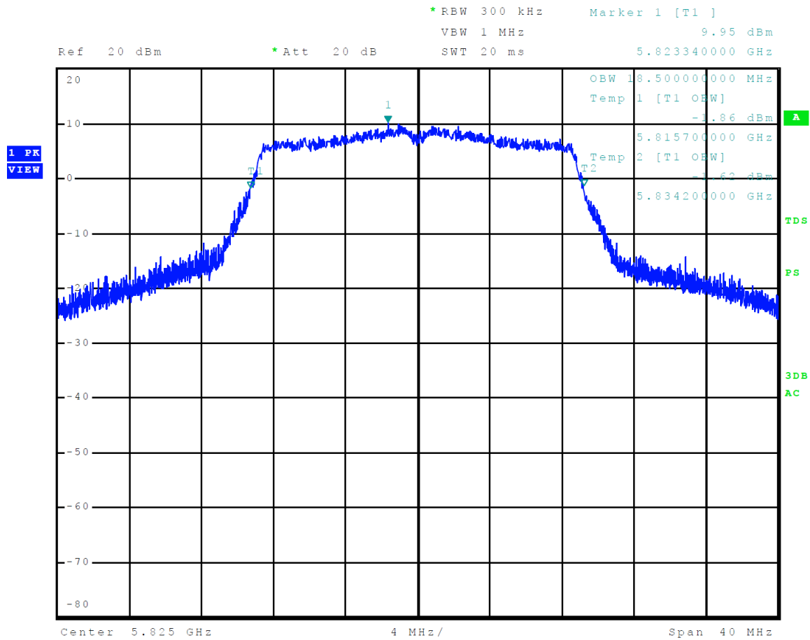
Figure 40 Plot of 99% Occupied Bandwidth 5725-5850 MHz Mode 13 U-NII-3 (802.11n)
