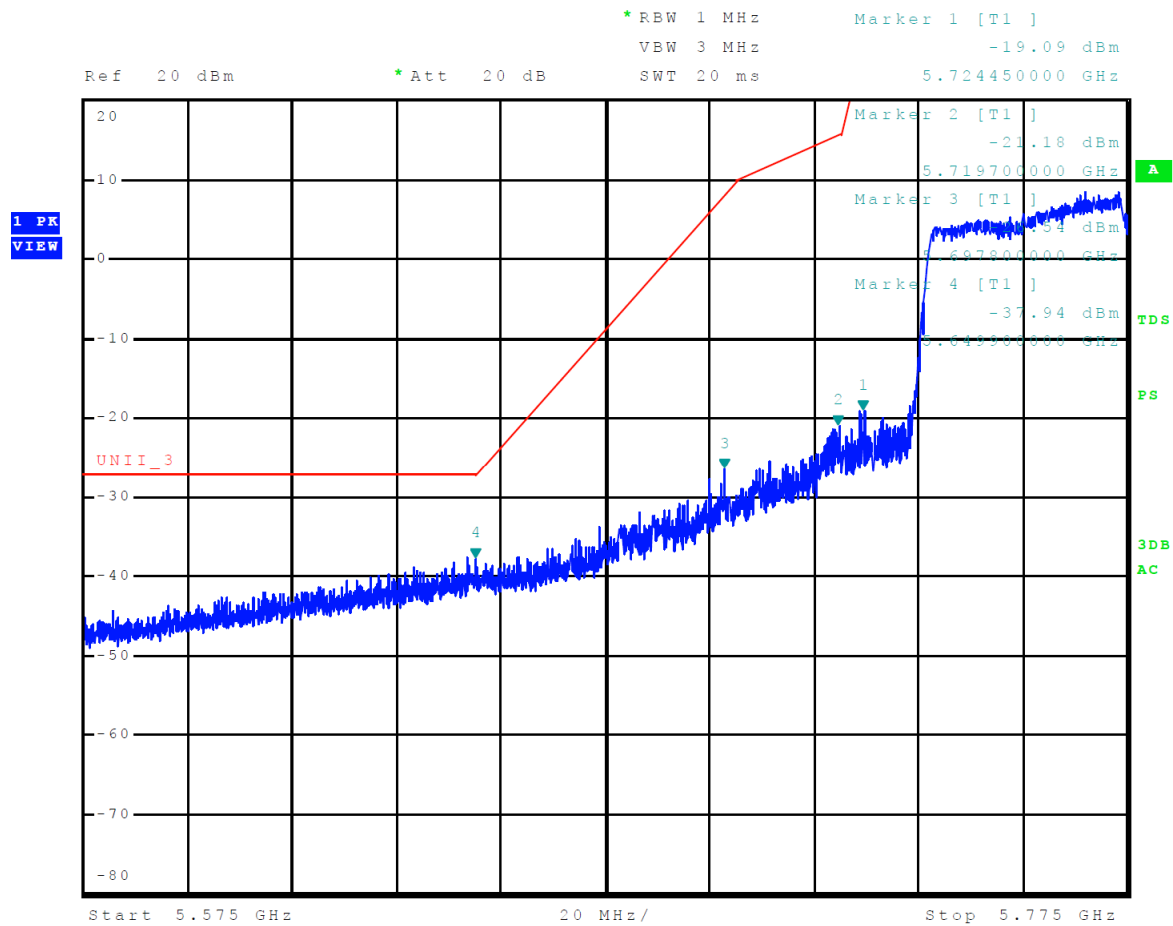
Figure 18 Plot of Lower Band Edge Across 5725-5850 MHz Mode 15 U-NII-3 (802.11ac80)
