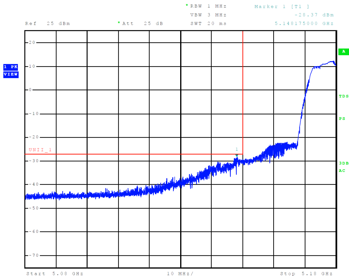
Figure 11 Plot of Lower Band Edge Across 5150-5250 MHz Mode 8 U-NII-1 (802.11a)
