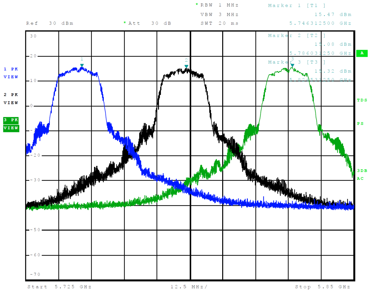
Figure 7 Plot of Transmitter Emissions Across 5725-5850 MHz Mode 9 U-NII-3 (802.11a)
