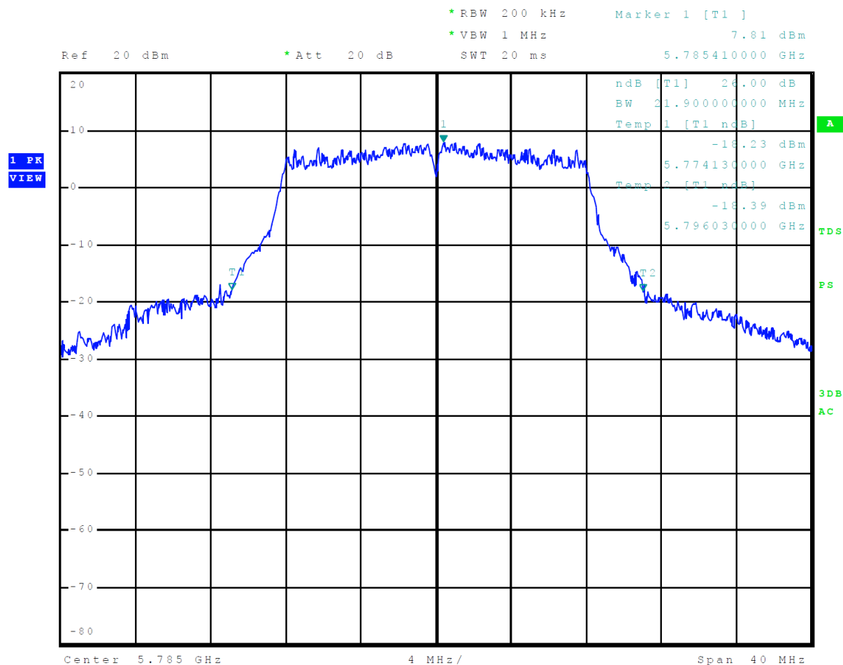
Figure 31 Plot of 26-dB Occupied Bandwidth 5725-5850 MHz Mode 12 U-NII-3 (802.11a)
