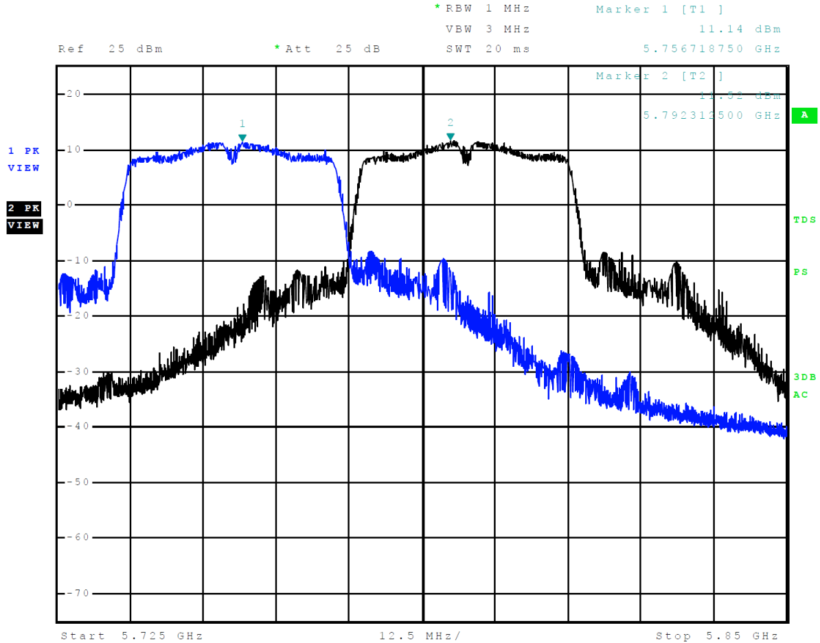
Figure 9 Plot of Transmitter Emissions Across 5725-5850 MHz Mode 11 U-NII-3 (802.11n40)
