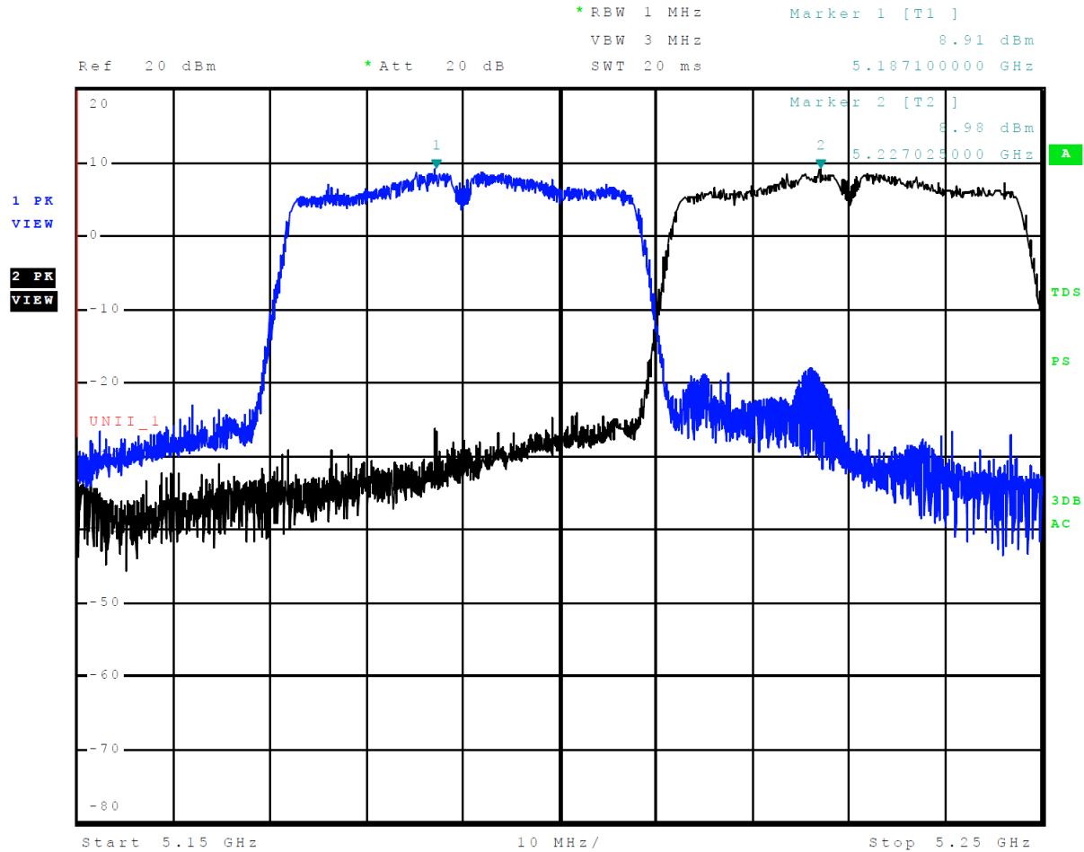
Figure 5 Plot of Transmitter Emissions Across 5150-5250 MHz Mode 10 U-NII-1 (802.11n40)
