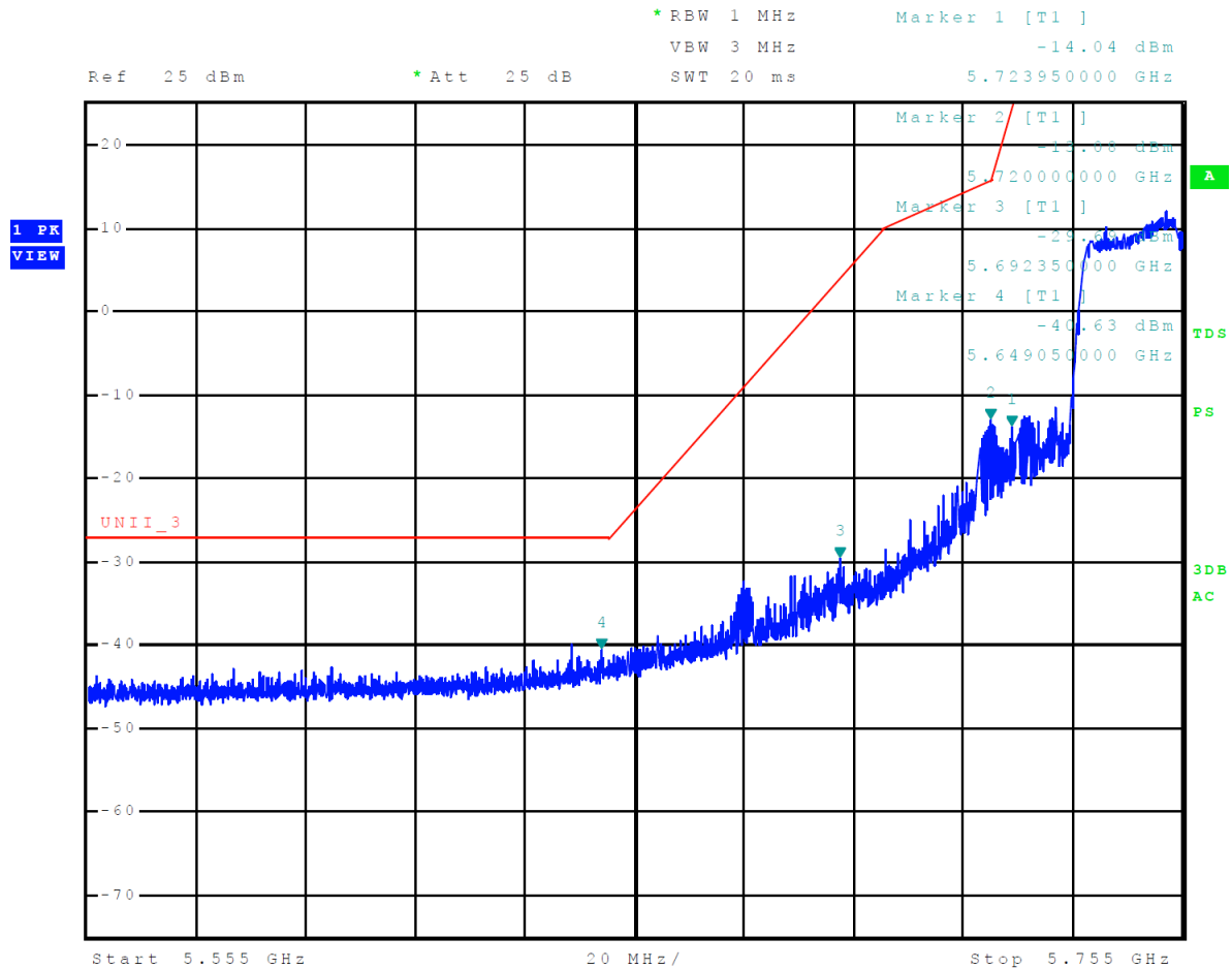
Figure 17 Plot of Lower Band Edge Across 5725-5850 MHz Mode 14 U-NII-3 (802.11n40)
