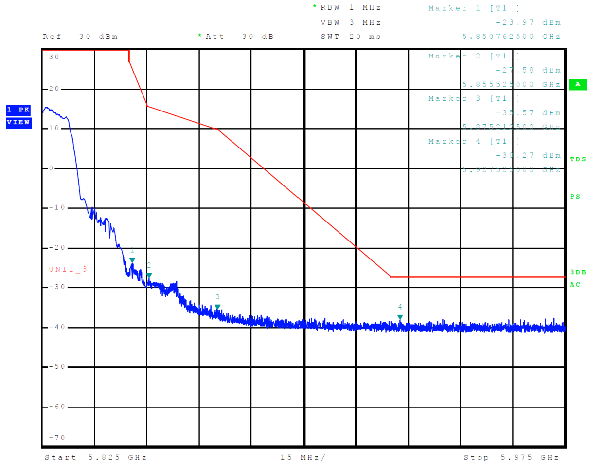
Figure 23 Plot of Upper Band Edge Across 5725-5850 MHz Mode 12 U-NII-3 (802.11a)
