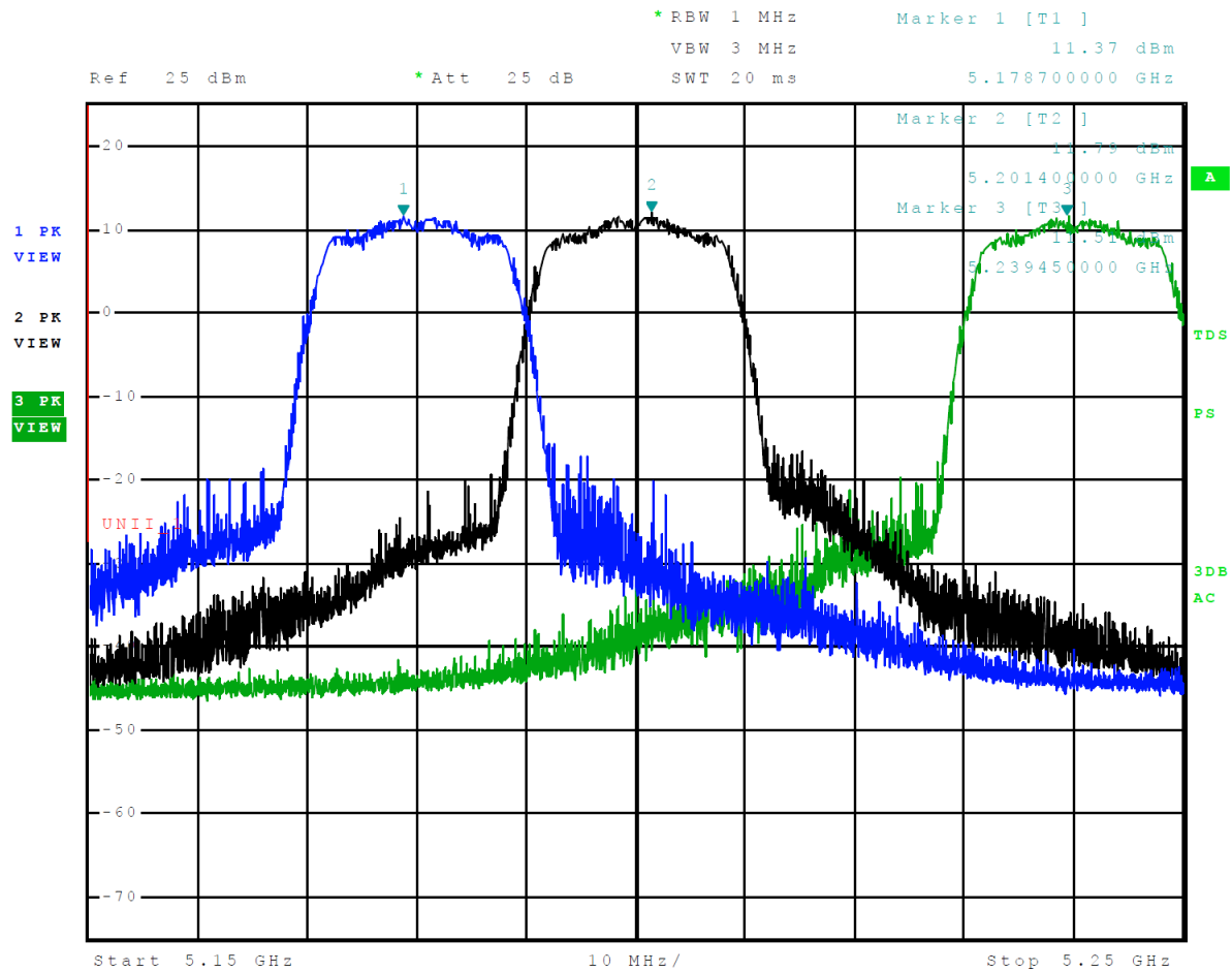
Figure 4 Plot of Transmitter Emissions Across 5150-5250 MHz Mode 9 U-NII-1 (802.11n)
