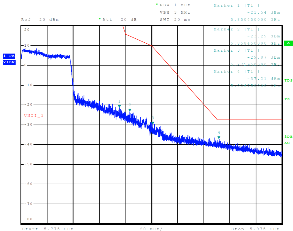
Figure 26 Plot of Upper Band Edge Across 5725-5850 MHz Mode 15 U-NII-3 (802.11ac80)
