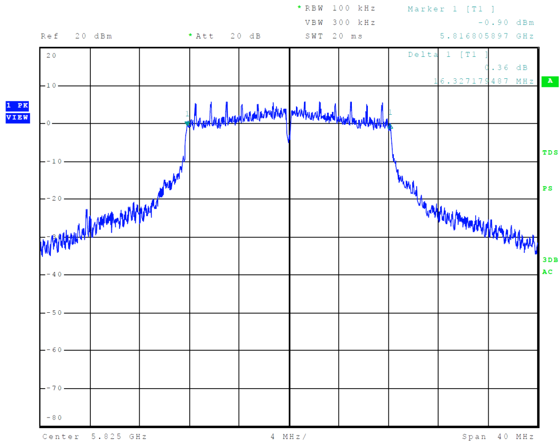
Figure 43 Plot of 6-dB Occupied Bandwidth 5725-5850 MHz Mode 12 U-NII-3 (802.11a)
