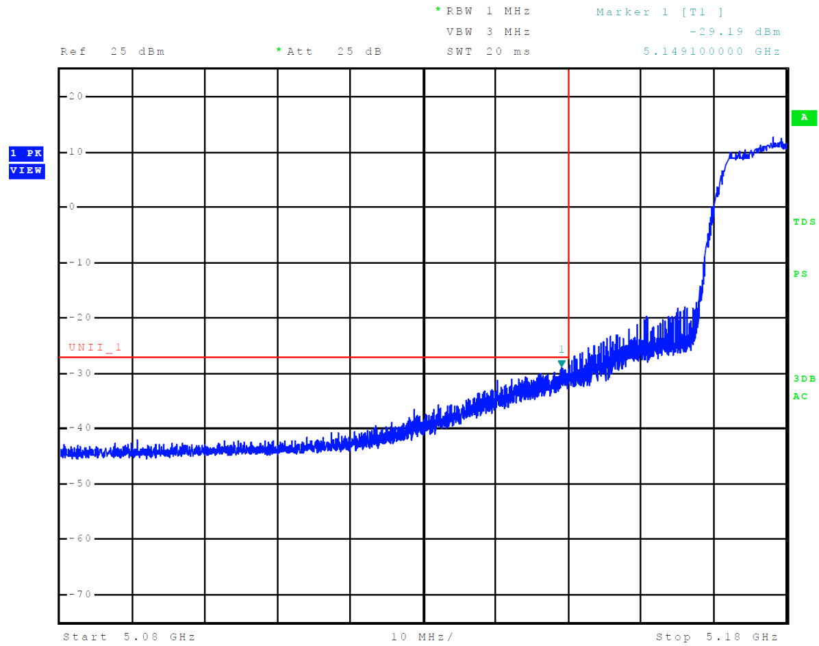
Figure 12 Plot of Lower Band Edge Across 5150-5250 MHz Mode 9 U-NII-1 (802.11n)
