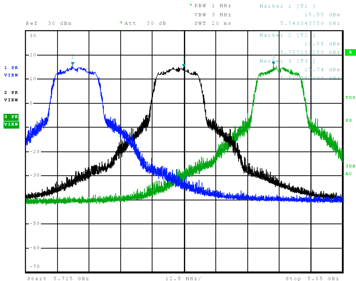
Figure 8 Plot of Transmitter Emissions Across 5725-5850 MHz Mode 10 U-NII-3 (802.11n)
