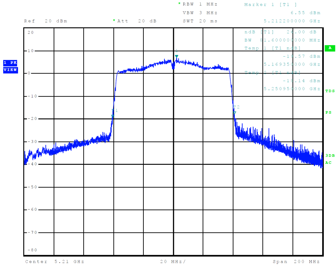
Figure 30 Plot of 26-dB Occupied Bandwidth 5150-5250 MHz Mode 11 U-NII-1 (802.11ac80)
