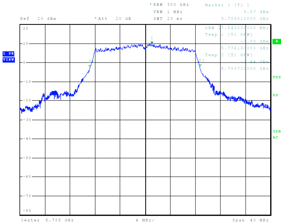
Figure 39 Plot of 99% Occupied Bandwidth 5725-5850 MHz Mode 12 U-NII-3 (802.11a)
