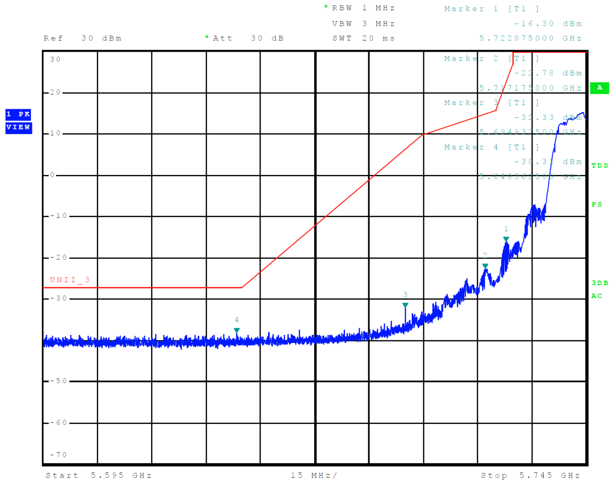
Figure 15 Plot of Lower Band Edge Across 5725-5850 MHz Mode 12 U-NII-3 (802.11a)
