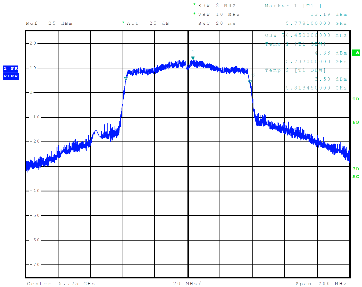
Figure 42 Plot of 99% Occupied Bandwidth 5725-5850 MHz Mode 15 U-NII-3 (802.11ac80)
