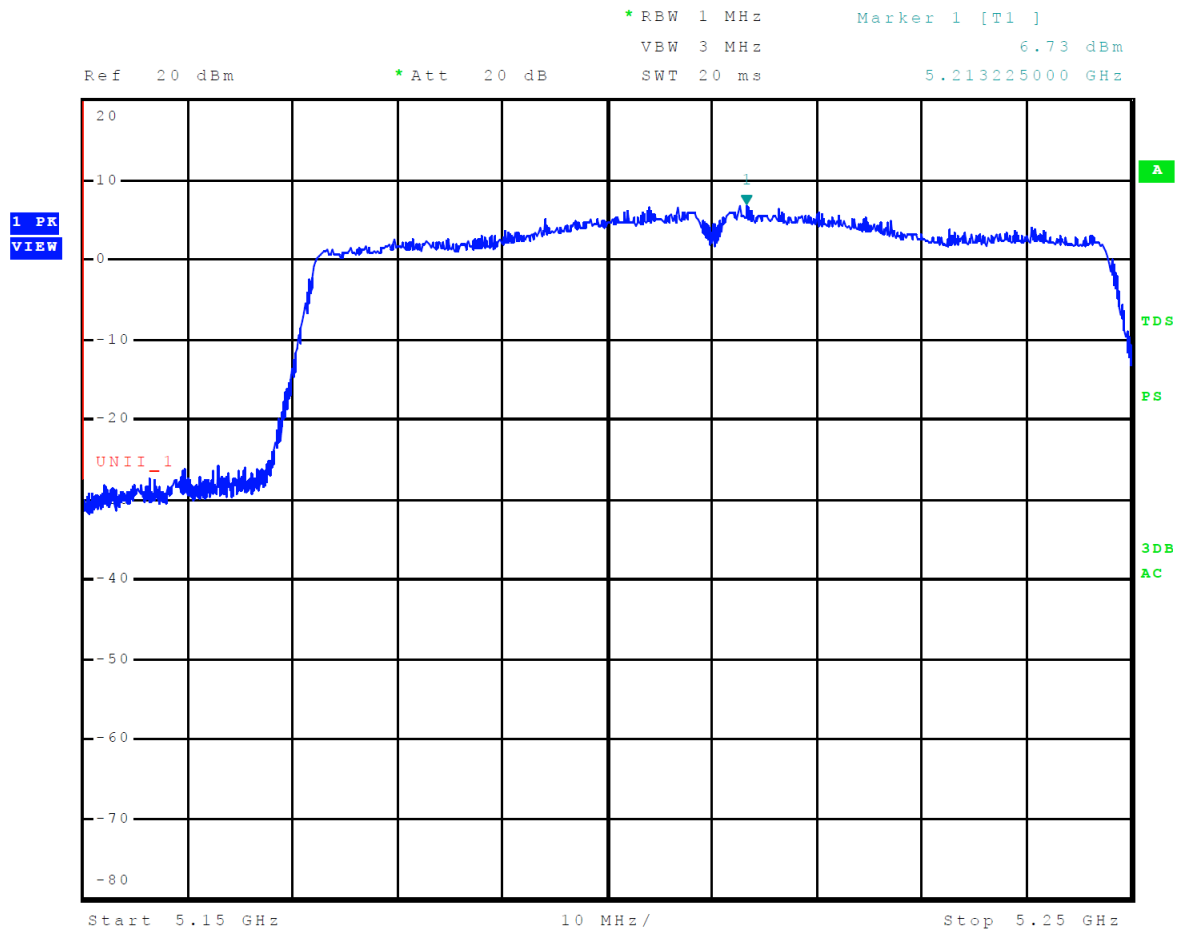
Figure 6 Plot of Transmitter Emissions Across 5150-5250 MHz Mode 11 U-NII-1 (802.11ac80)
