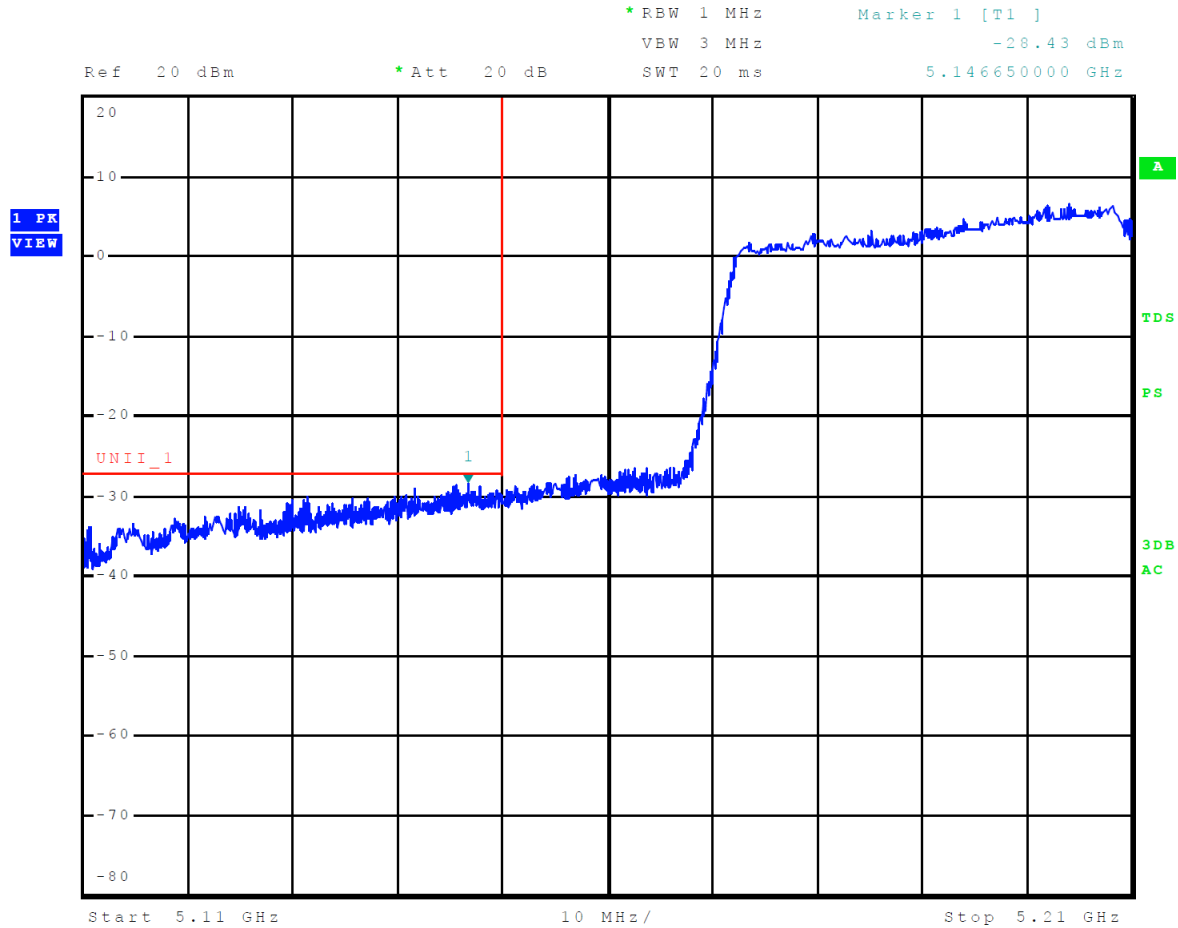
Figure 14 Plot of Lower Band Edge Across 5150-5250 MHz Mode 11 U-NII-1 (802.11ac80)
