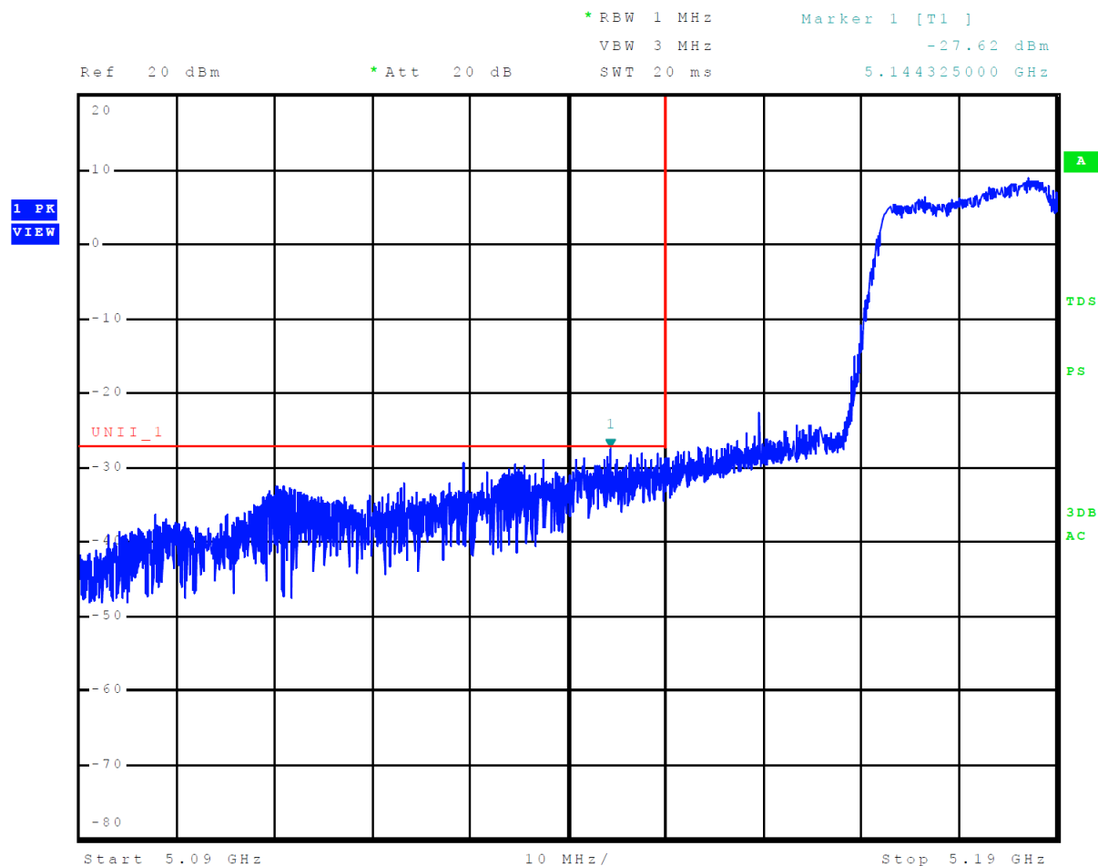
Figure 13 Plot of Lower Band Edge Across 5150-5250 MHz Mode 10 U-NII-1 (802.11n40)
