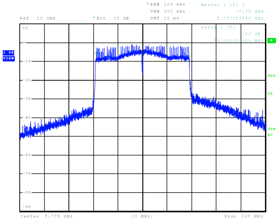
Figure 46 Plot of 6-dB Occupied Bandwidth 5725-5850 MHz Mode 15 U-NII-3 (802.11ac80)
