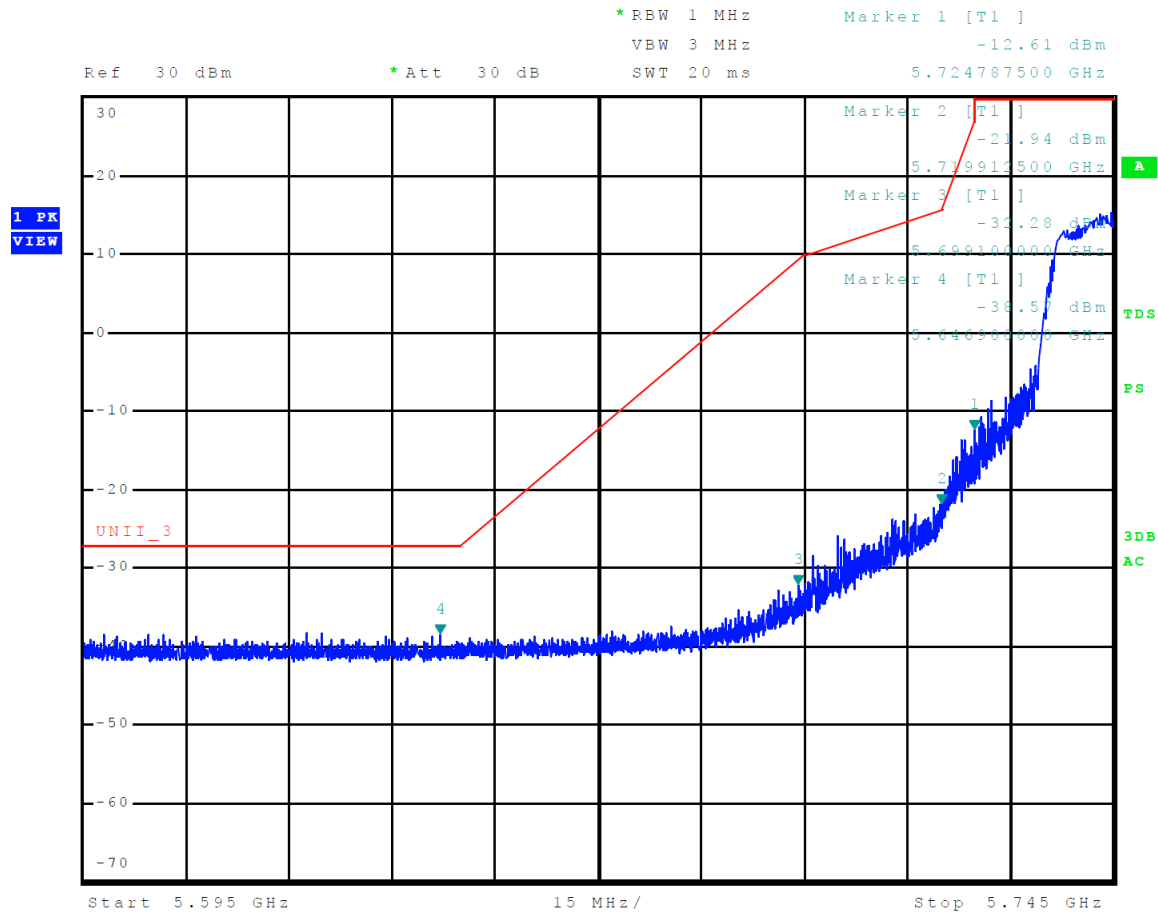
Figure 16 Plot of Lower Band Edge Across 5725-5850 MHz Mode 13 U-NII-3 (802.11n)
