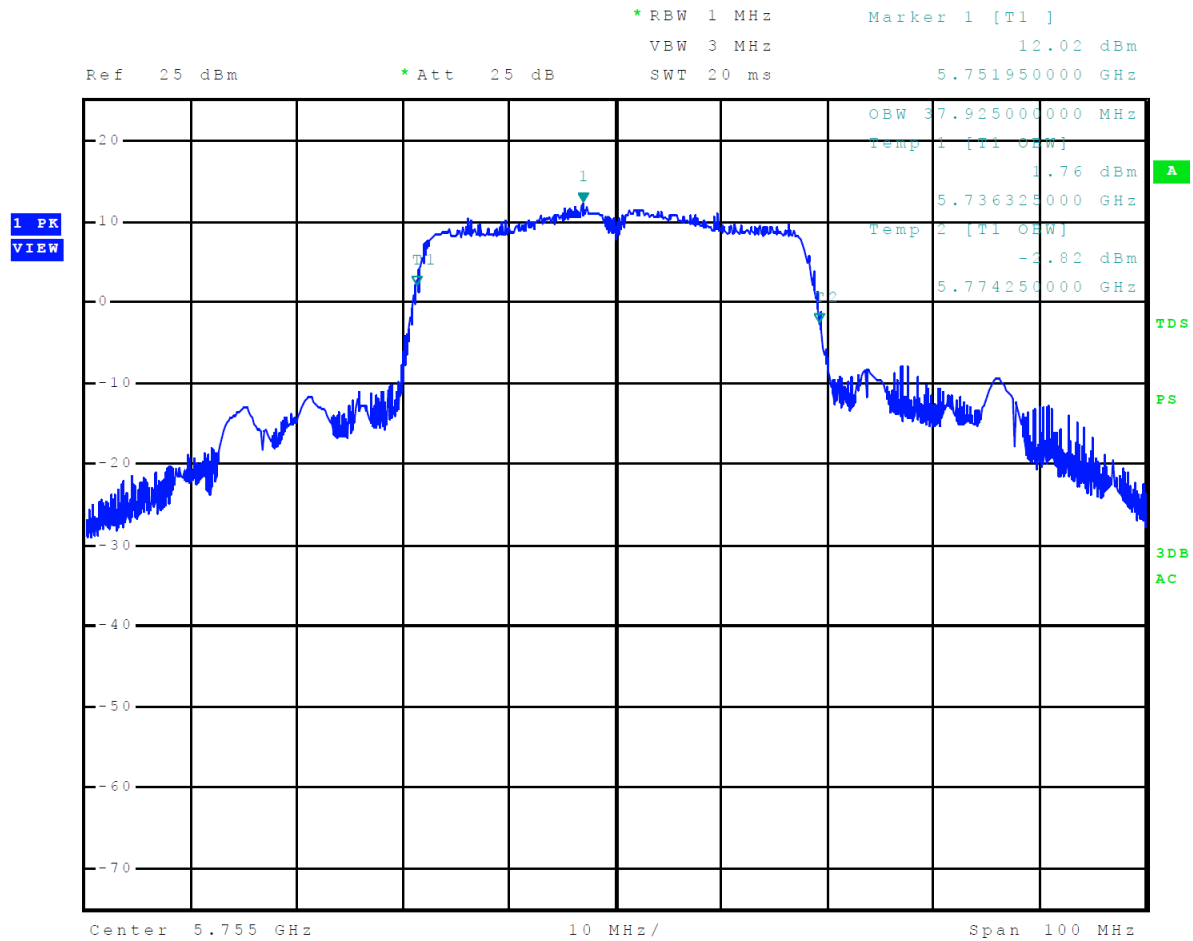
Figure 41 Plot of 99% Occupied Bandwidth 5725-5850 MHz Mode 14 U-NII-3 (802.11n40)
