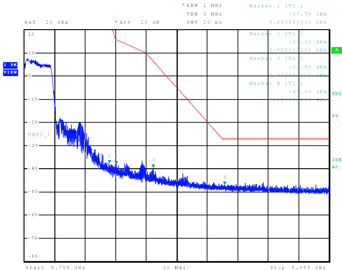
Figure 25 Plot of Upper Band Edge Across 5725-5850 MHz Mode 14 U-NII-3 (802.11n40)
