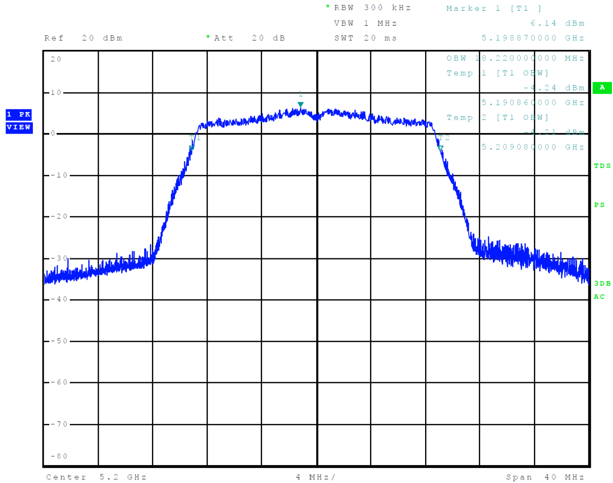
Figure 36 Plot of 99% Occupied Bandwidth 5150-5250 MHz Mode 9 U-NII-1 (802.11n)
