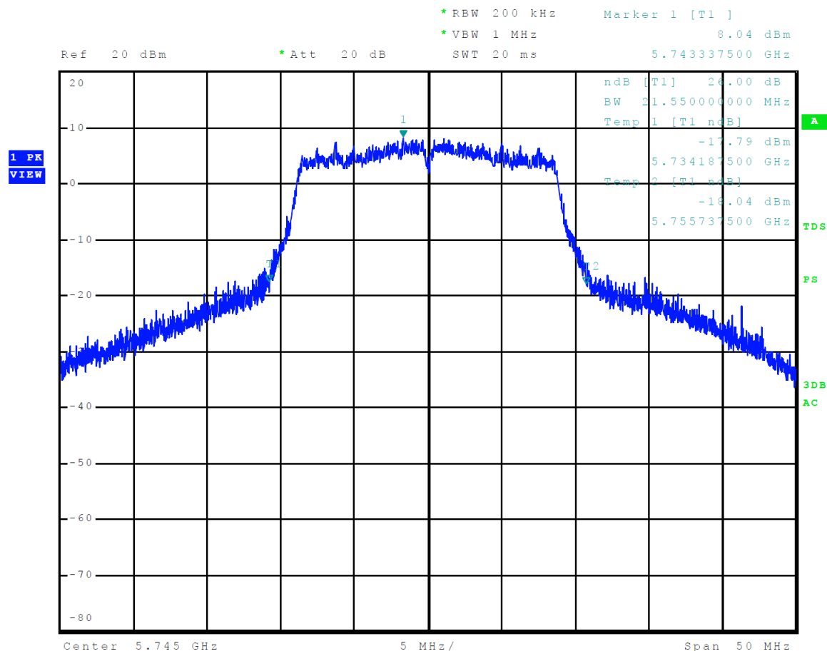
Figure 32 Plot of 26-dB Occupied Bandwidth 5725-5850 MHz Mode 13 U-NII-3 (802.11n)
