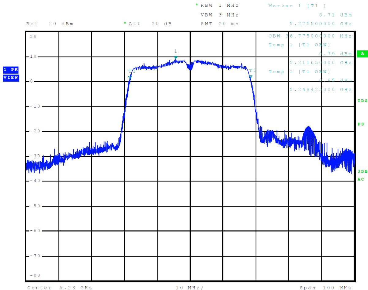
Figure 37 Plot of 99% Occupied Bandwidth 5150-5250 MHz Mode 10 U-NII-1 (802.11n40)
