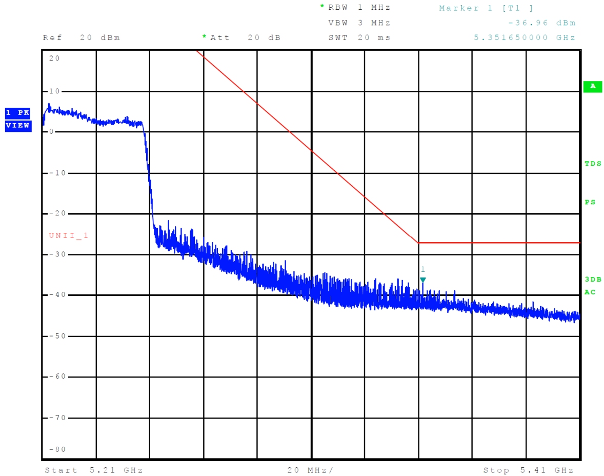
Figure 22 Plot of Upper Band Edge Across 5150-5250 MHz Mode 11 U-NII-1 (802.11ac80)
