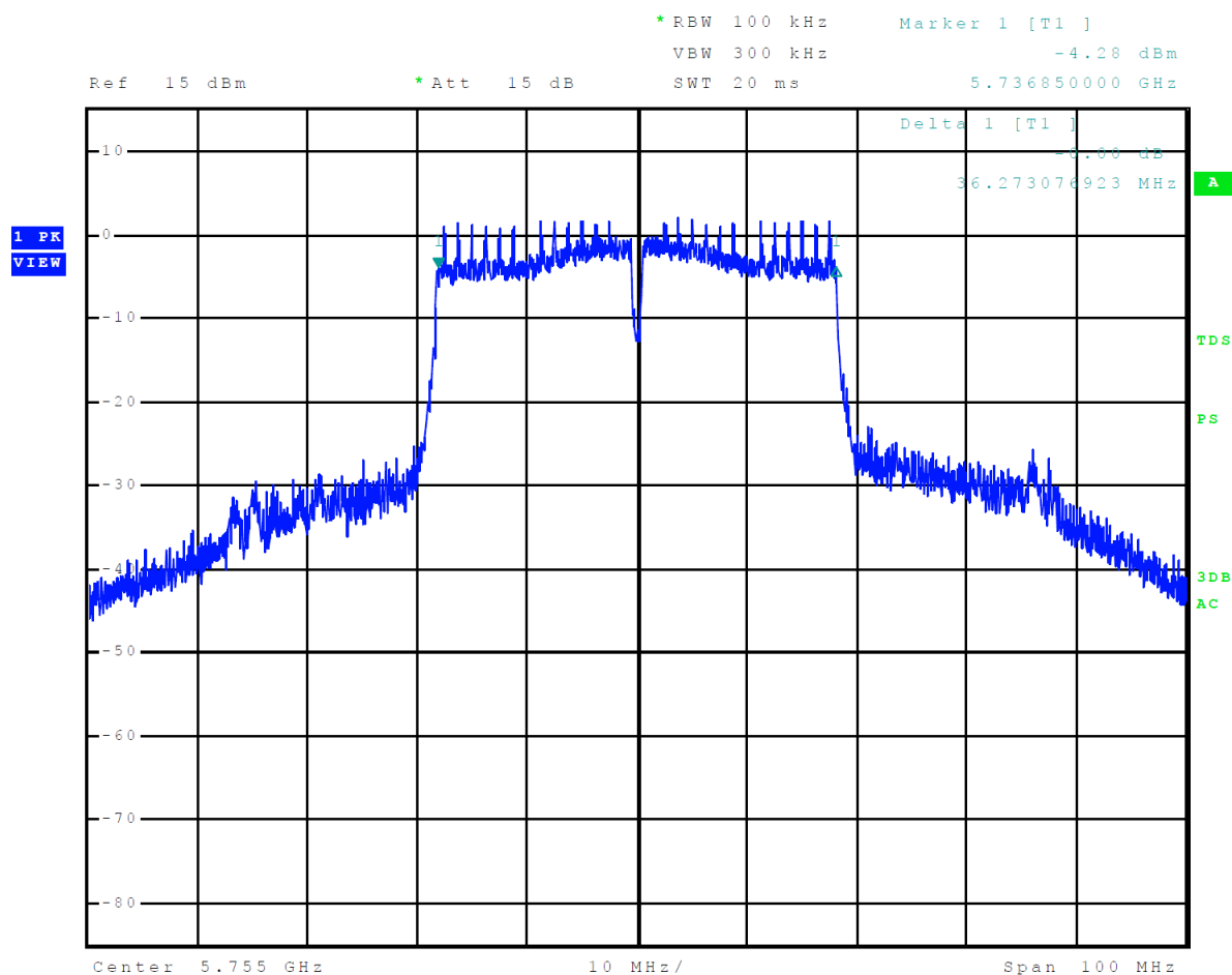
Figure 45 Plot of 6-dB Occupied Bandwidth 5725-5850 MHz Mode 14 U-NII-3 (802.11n40)
