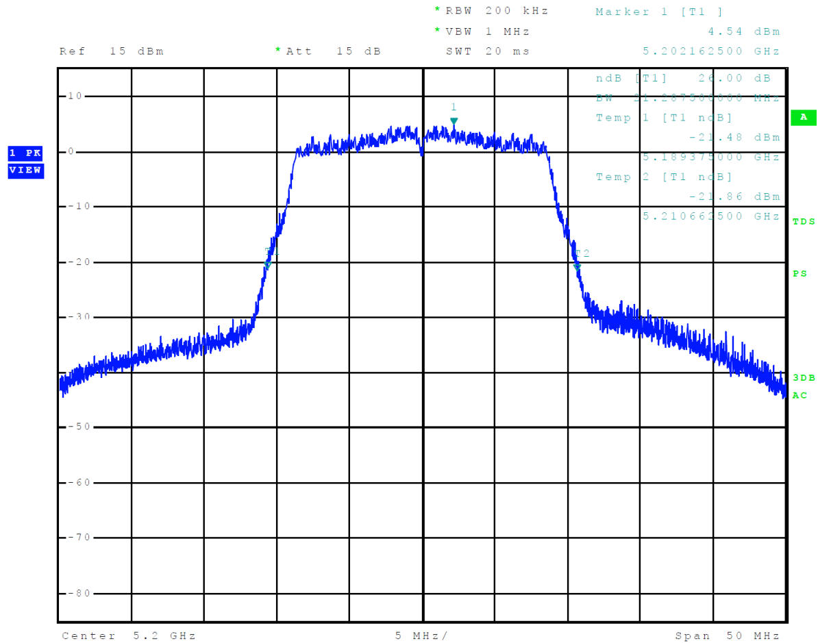
Figure 28 Plot of 26-dB Occupied Bandwidth 5150-5250 MHz Mode 9 U-NII-1 (802.11n)
