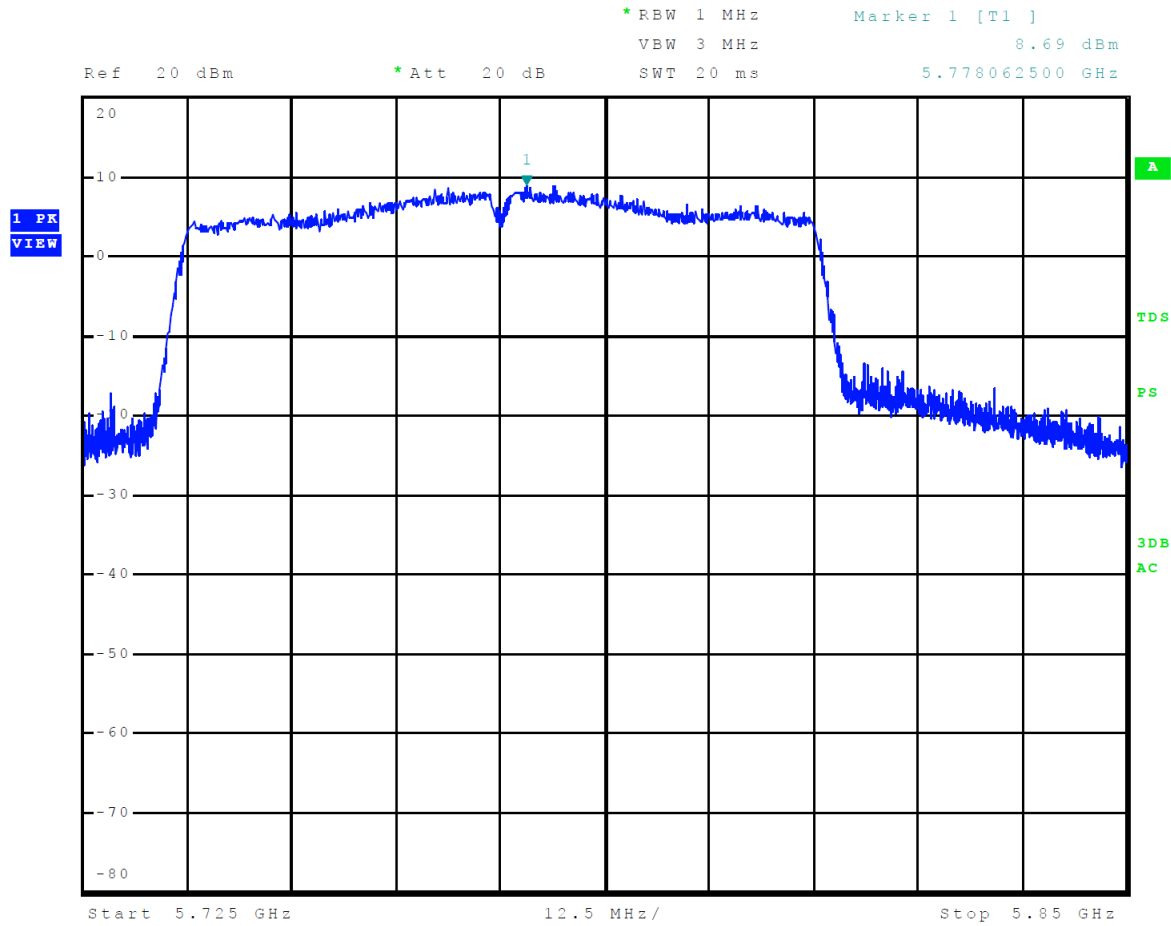
Figure 10 Plot of Transmitter Emissions Across 5725-5850 MHz Mode 12 U-NII-3 (802.11ac80)
