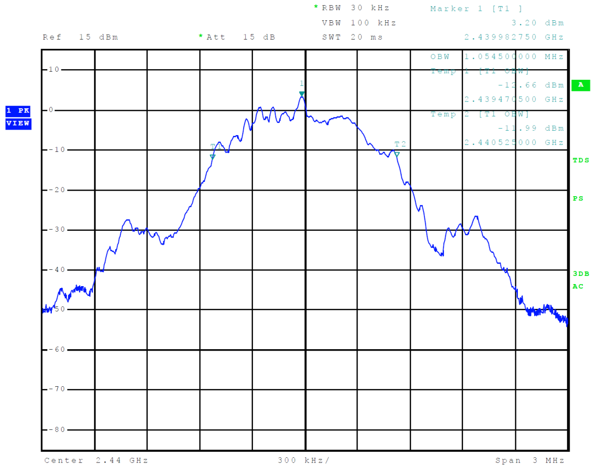
Figure 26 Plot of 99% Occupied Bandwidth Mode 4, BT BLE
