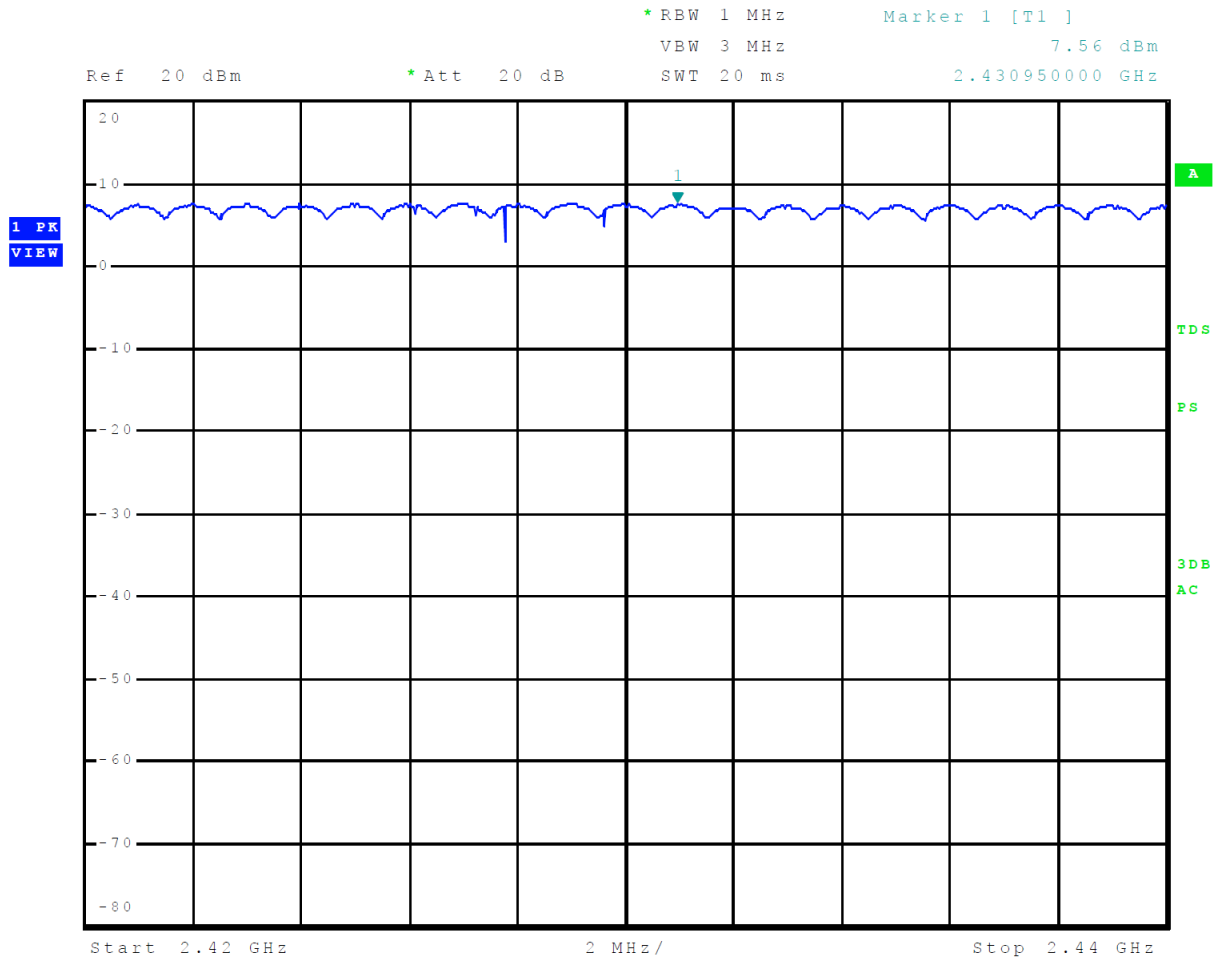
Figure 6a Plot of Number of Hopping Channels Mode 1, BT BR
