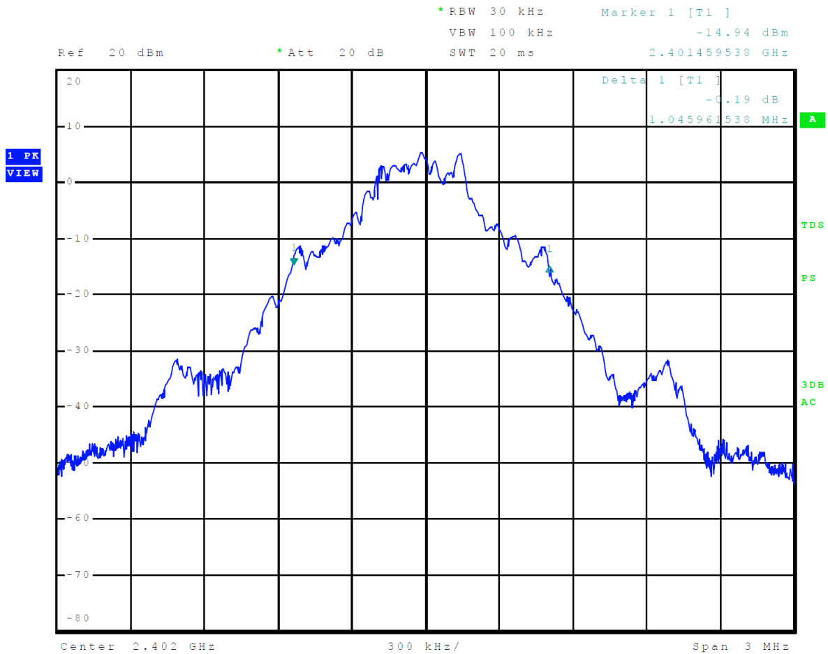
Figure 2 Plot of Transmitter Emissions 20-dB Occupied Bandwidth Mode 1, BT BR
