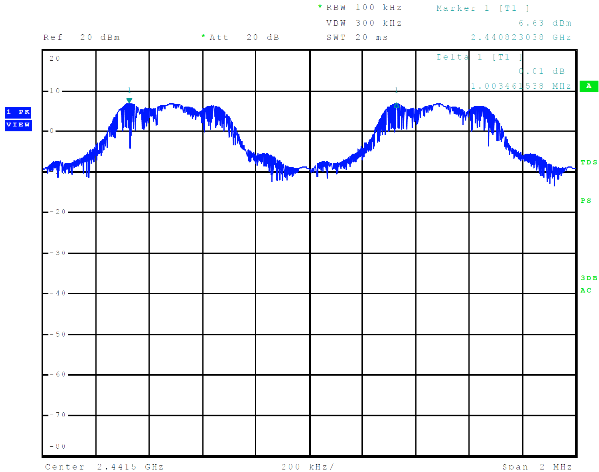
Figure 8 Plot of Channel Separation Mode 1, BT BR
