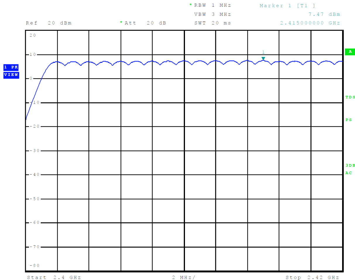
Figure 5 Plot of Number of Hopping Channels Mode 1, BT BR
