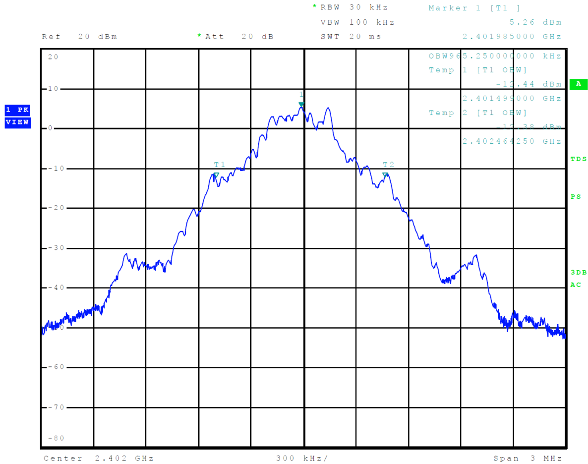
Figure 4 Plot of Transmitter Emissions 99% Occupied Bandwidth Mode 1, BT BR
