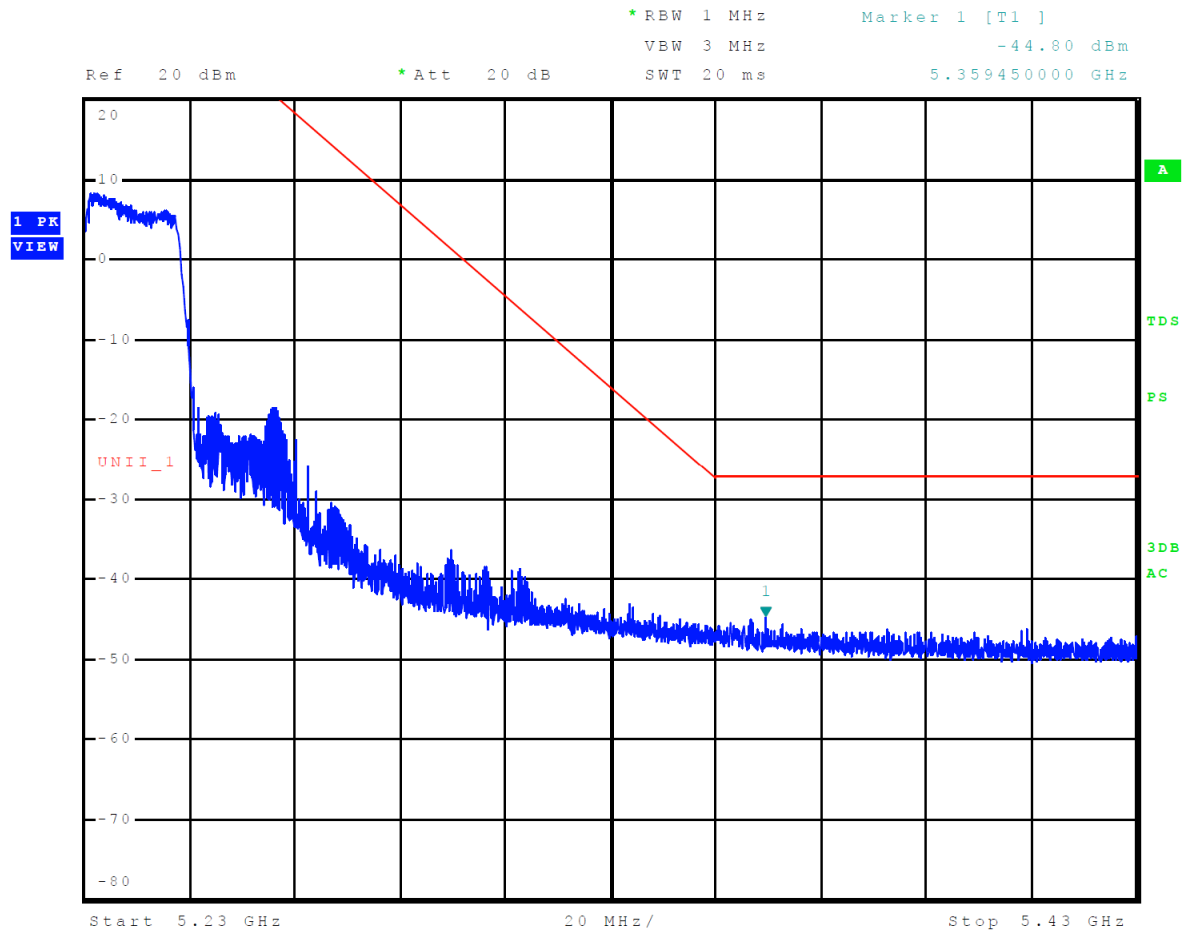
Figure 21 Plot of Upper Band Edge Across 5150-5250 MHz Mode 10 U-NII-1 (802.11n40)
