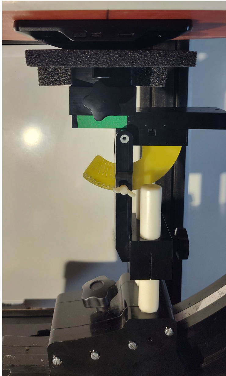
Figure C.3 – Setup Photo, Extremity - Front - Far
