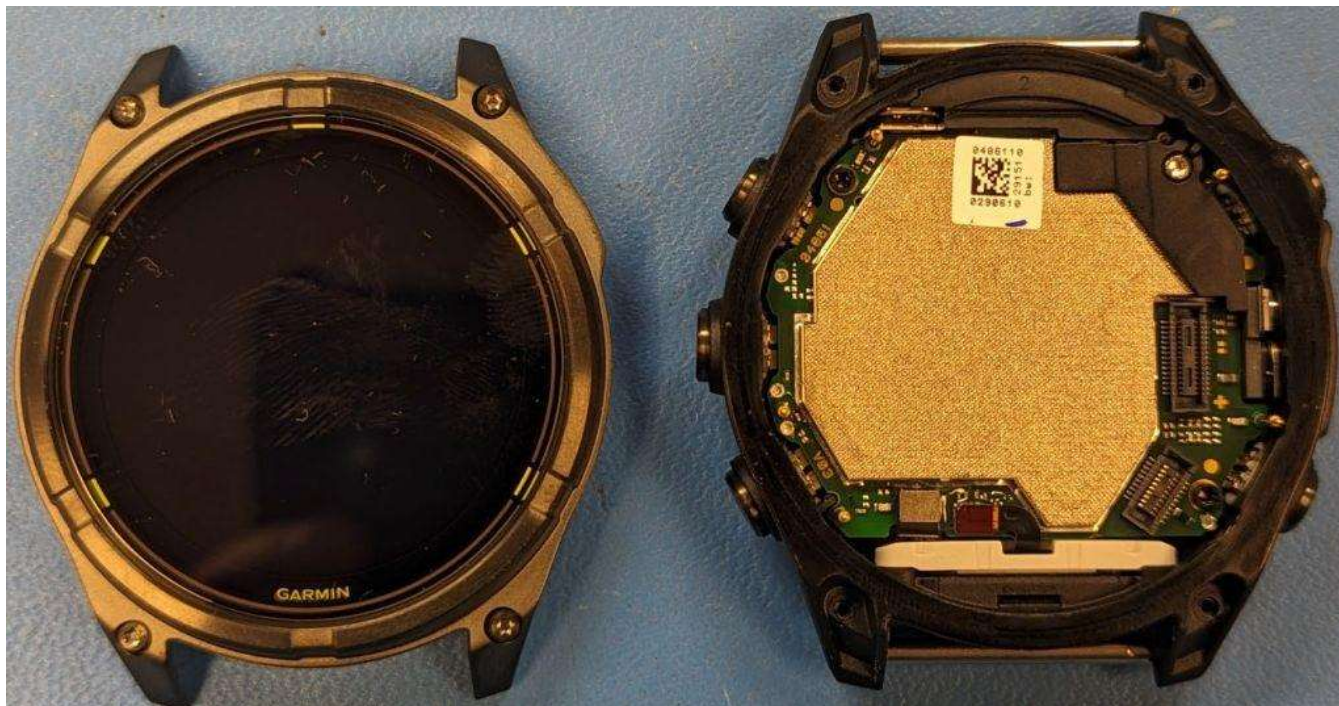
Figure E14.1 – Internal, Front Removed
