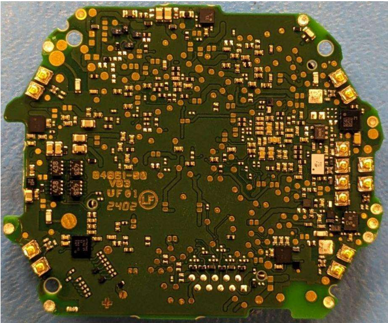
Figure E14.5 – Internal, Main PCB, Bottom Side
