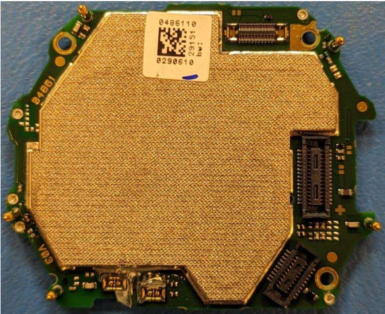
Figure E14.3 – Internal, Main PCB
