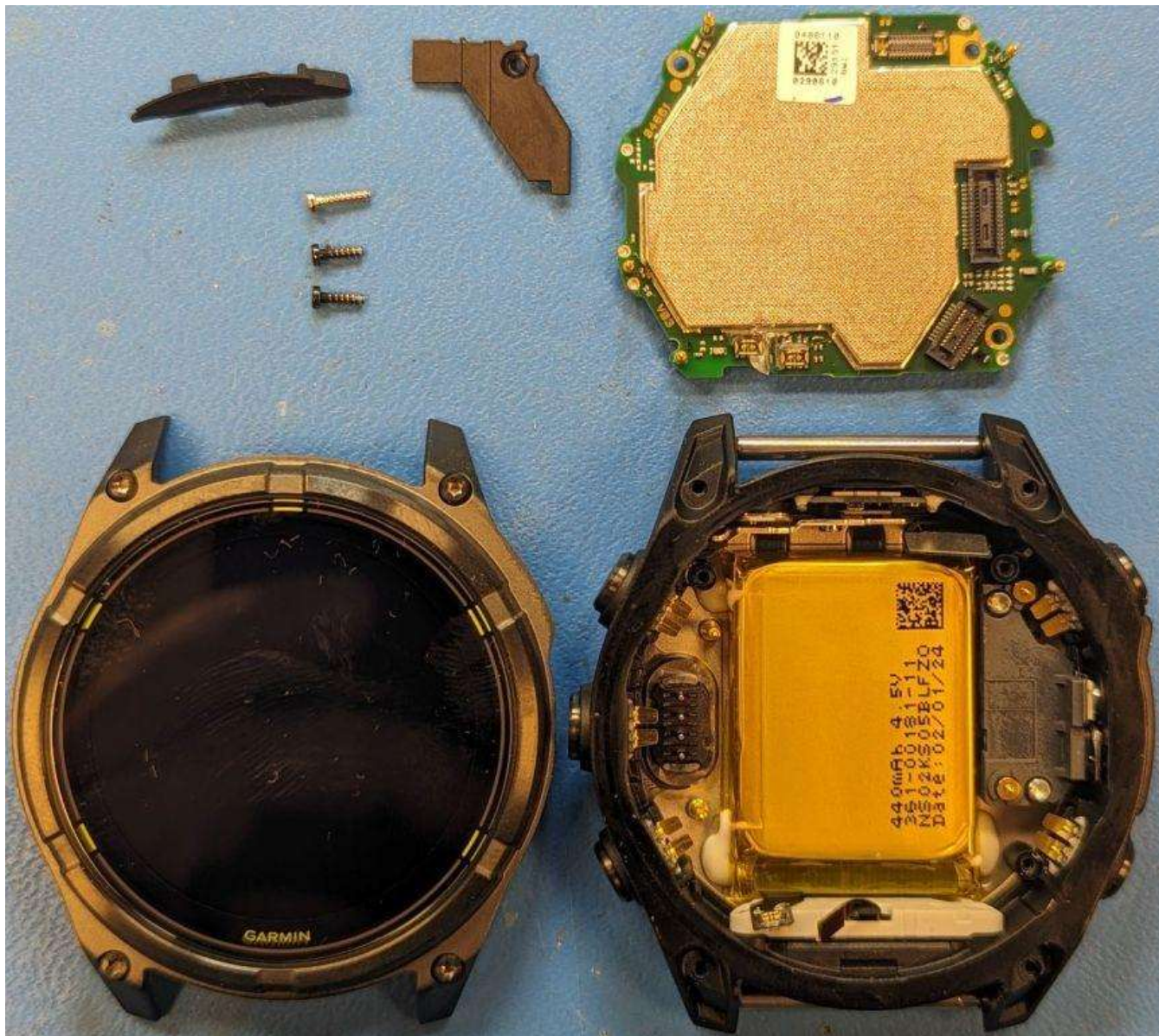
Figure E14.2 – Internal, Main PCB Removed
