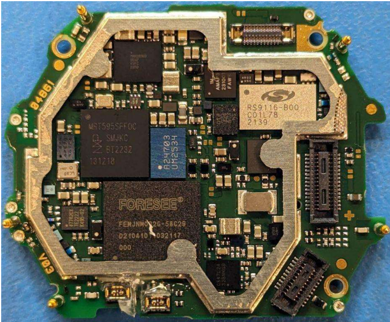
Figure E14.4 – Internal, Main PCB, Shield Removed
