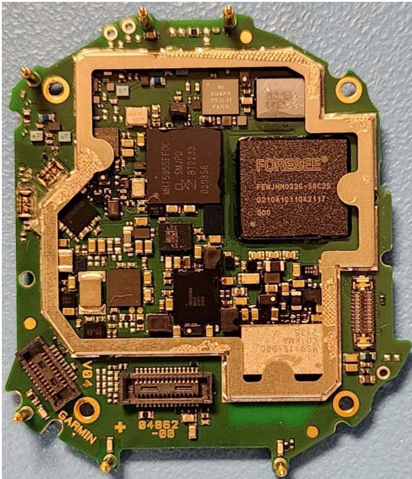
Figure E14.4 – Internal, Main PCB, Shield Removed
