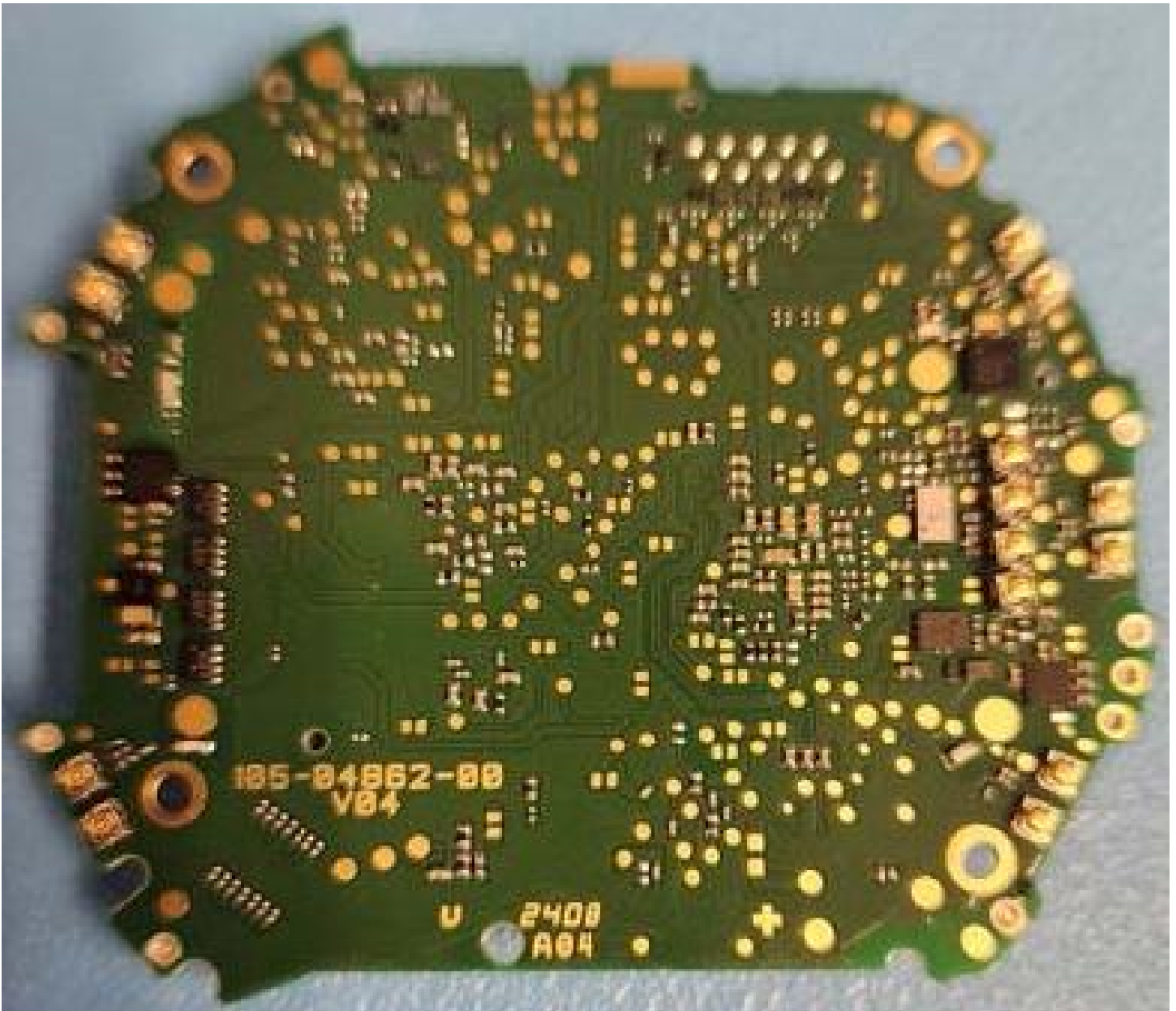
Figure E14.5 – Internal, Main PCB, Bottom Side
