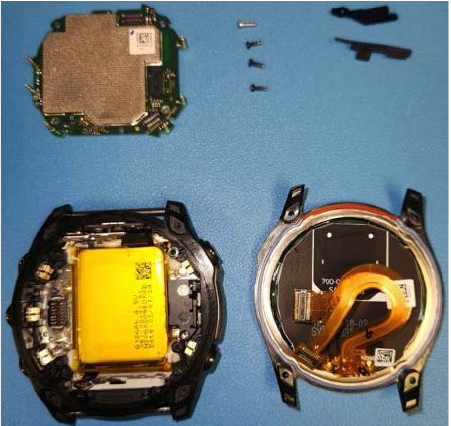
Figure E14.2 – Internal, Main PCB Removed
