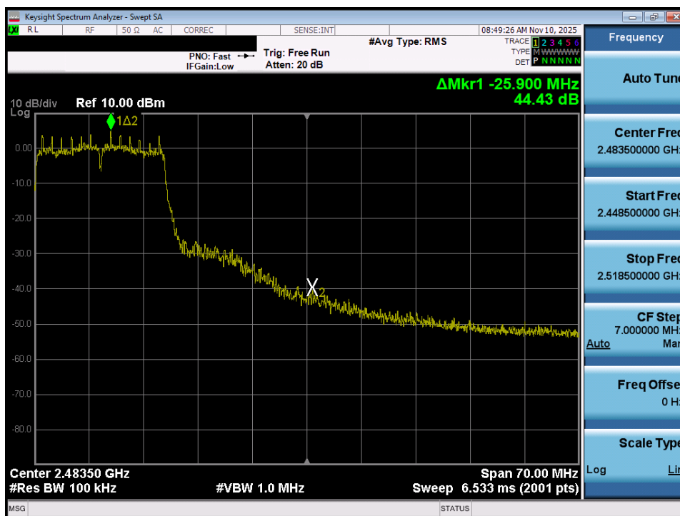
Plot 7-35. Band Edge Plot (802.11g – Ch. 10)
