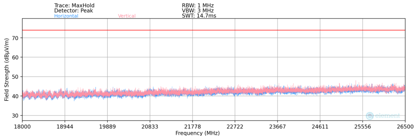
Plot 7-56. Radiated Spurious Plot above 18GHz
