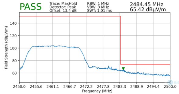
Plot 7-66. Radiated Restricted Upper Band Edge Measurement (Peak)
