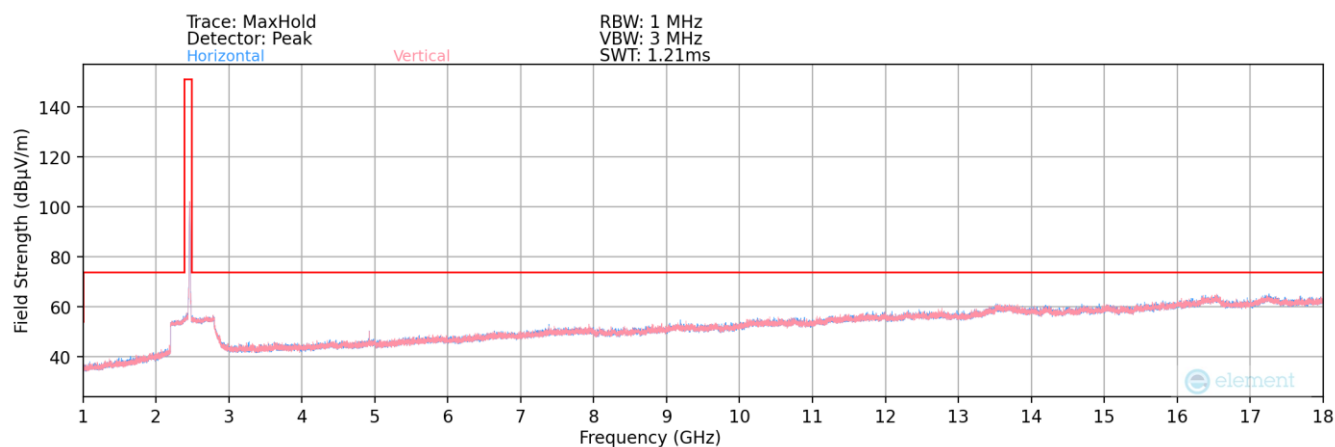
Plot 7-55. Radiated Spurious Plot above 1GHz (802.11b – Ch. 11)
