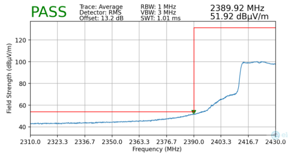
Plot 7-61. Radiated Restricted Lower Band Edge Measurement (Average)
