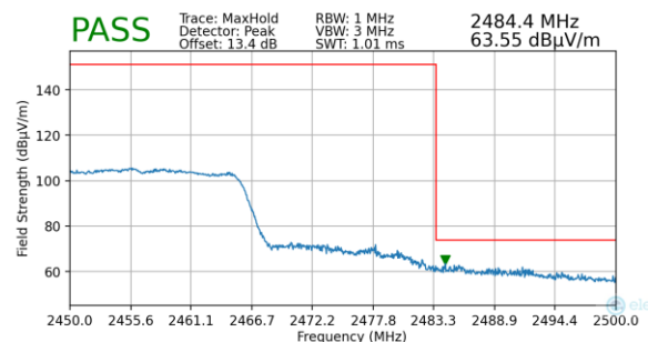
Plot 7-64. Radiated Restricted Upper Band Edge Measurement (Peak)
