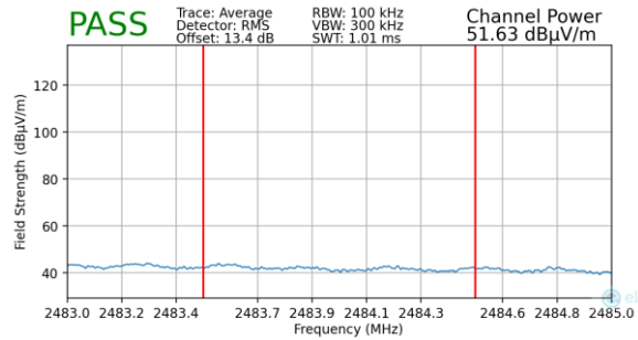
Plot 7-65. Radiated Restricted Upper Band Edge Measurement (Average)
