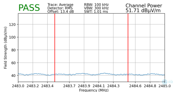
Plot 7-69. Radiated Restricted Upper Band Edge Measurement (Average)
