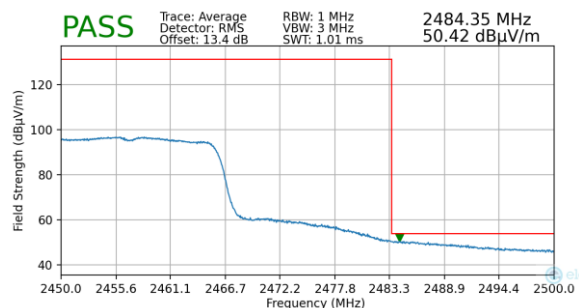
Plot 7-63. Radiated Restricted Upper Band Edge Measurement (Average)
