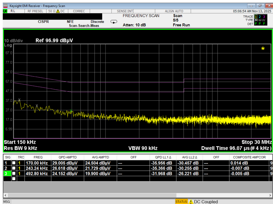
Plot 7-72. Line Conducted Plot with 802.11b (N)
