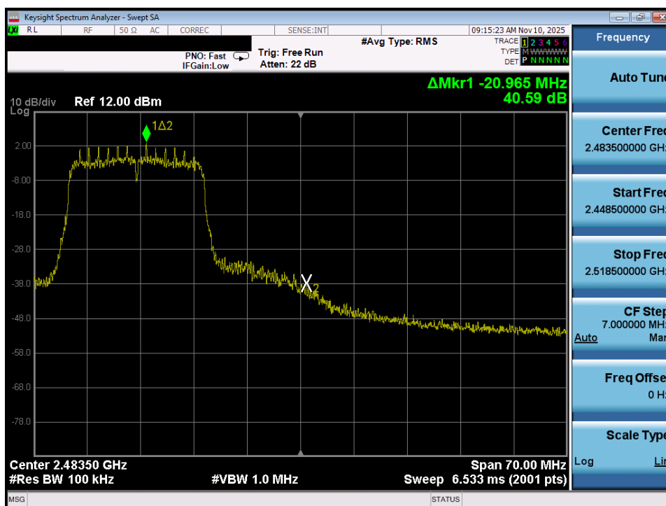
Plot 7-43. Band Edge Plot (802.11n – Ch. 11)
