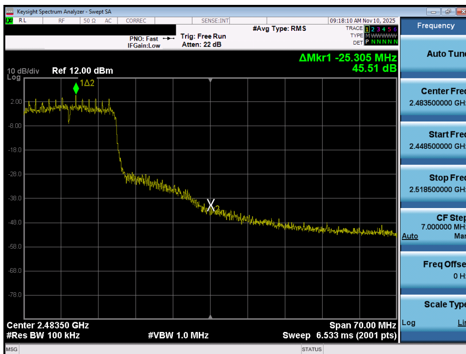
Plot 7-42. Band Edge Plot (802.11n – Ch. 10)
