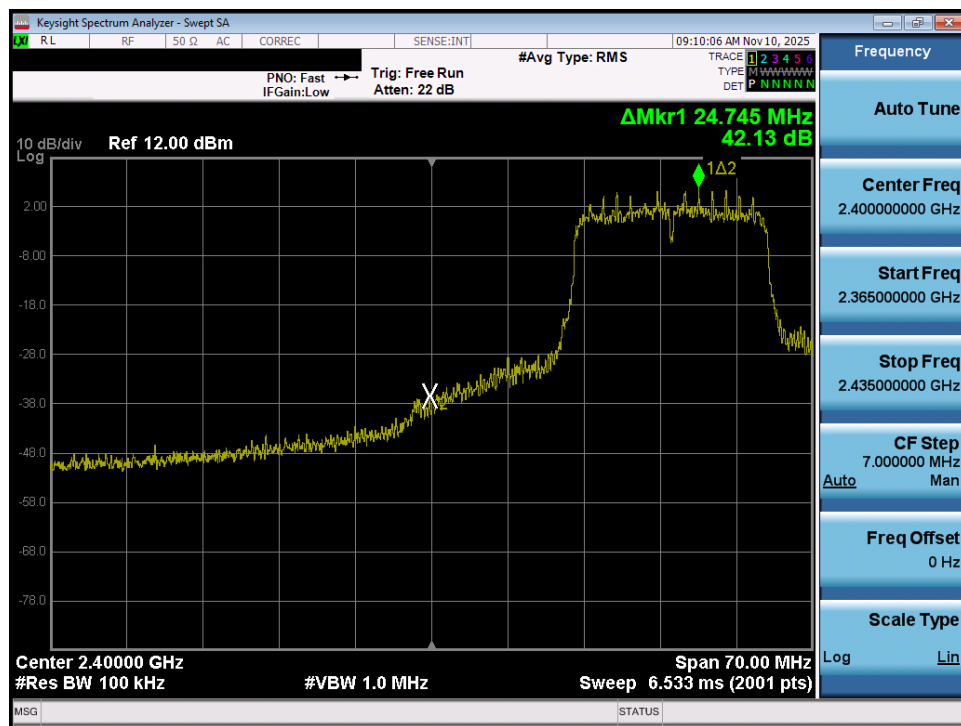
Plot 7-41. Band Edge Plot (802.11n – Ch. 3)
