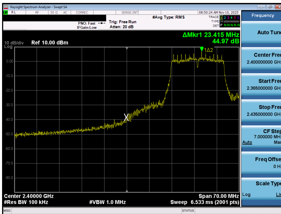
Plot 7-34. Band Edge Plot (802.11g– Ch. 3)
