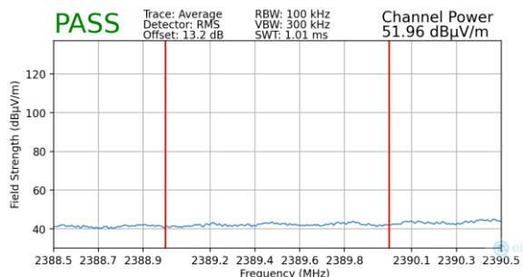
Plot 7-57. Radiated Restricted Lower Band Edge Measurement (Average)
