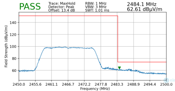
Plot 7-68. Radiated Restricted Upper Band Edge Measurement (Peak)
