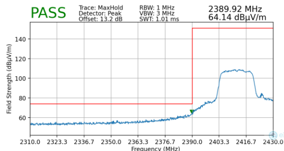
Plot 7-58. Radiated Restricted Lower Band Edge Measurement (Peak)
