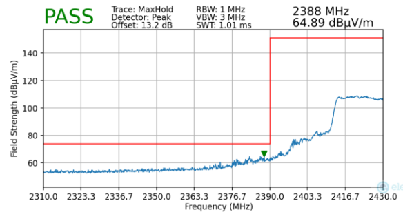
Plot 7-62. Radiated Restricted Lower Band Edge Measurement (Peak)
