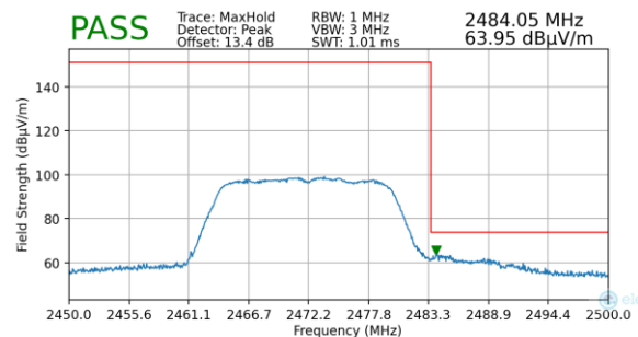
Plot 7-70. Radiated Restricted Upper Band Edge Measurement (Peak)
