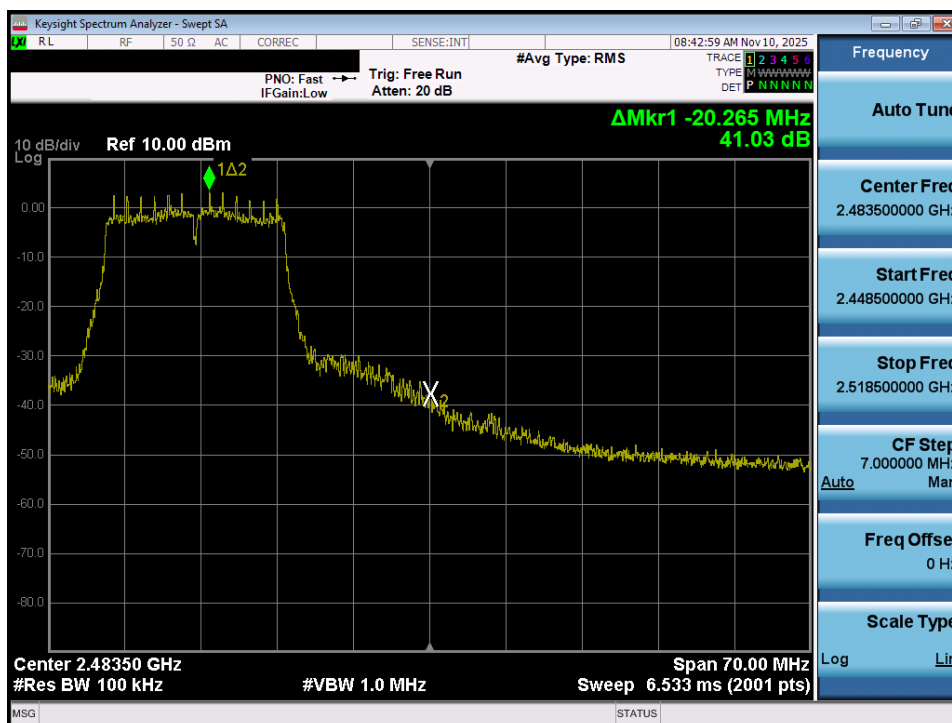
Plot 7-36. Band Edge Plot (802.11g – Ch. 11)
