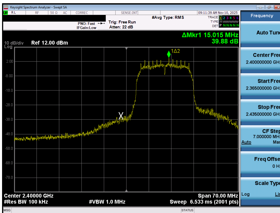
Plot 7-39. Band Edge Plot (802.11n – Ch. 1)
