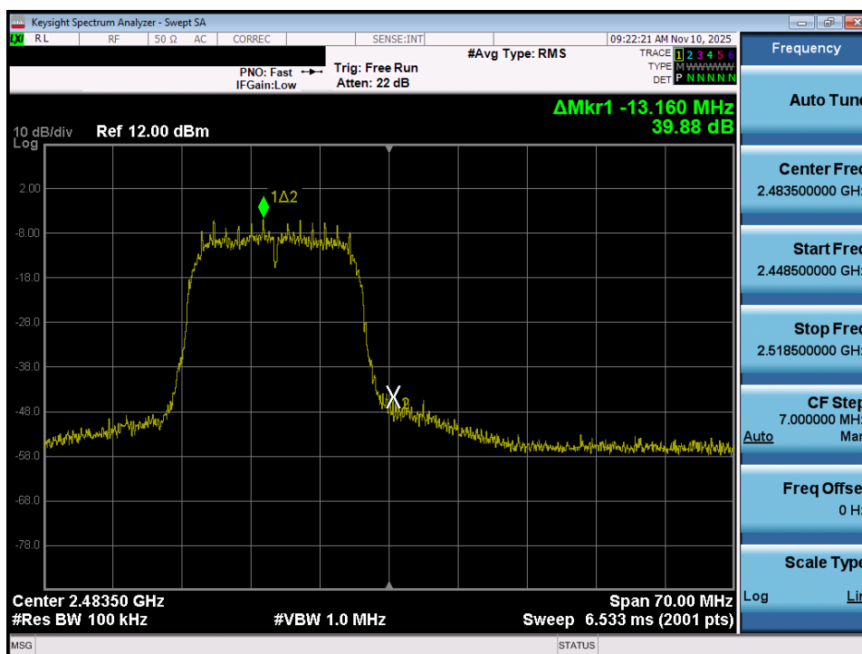
Plot 7-45. Band Edge Plot (802.11n – Ch. 13)
