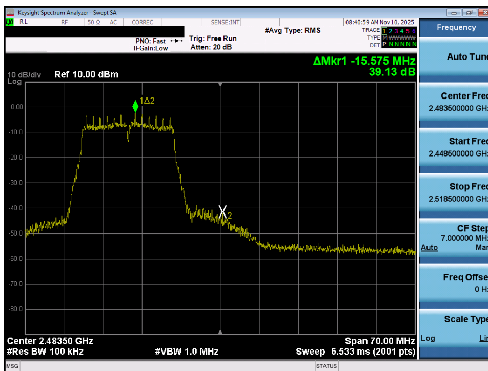
Plot 7-37. Band Edge Plot (802.11g – Ch. 12)
