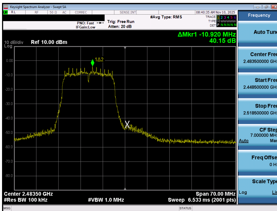
Plot 7-38. Band Edge Plot (802.11g – Ch. 13)
