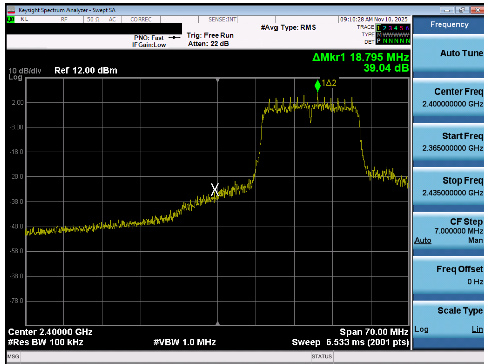
Plot 7-40. Band Edge Plot (802.11n – Ch. 2)
