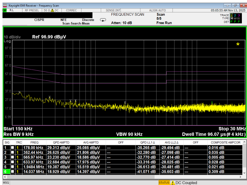
Plot 7-71. Line Conducted Plot with 802.11b (L1)
