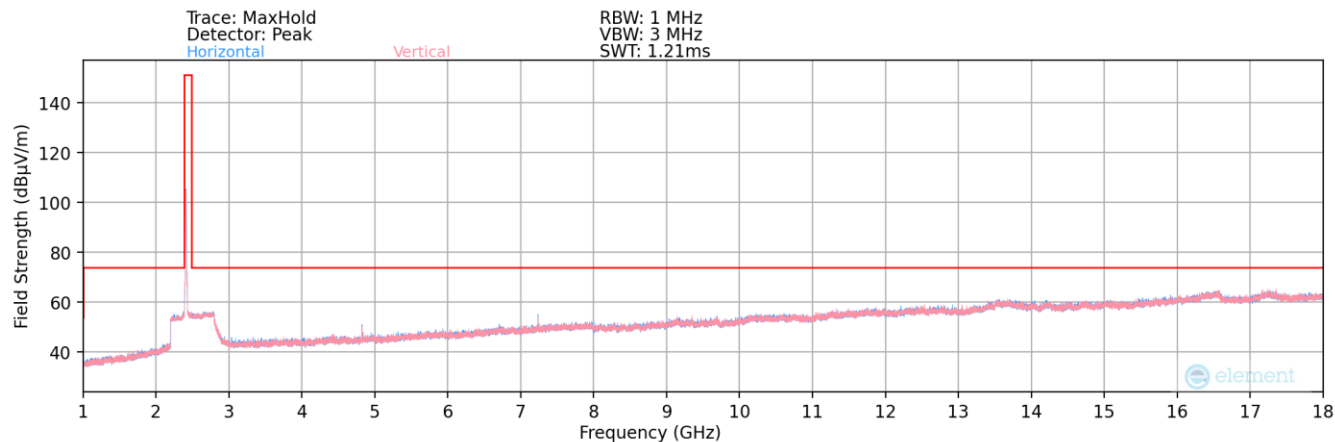
Plot 7-53. Radiated Spurious Plot above 1GHz (802.11b – Ch. 1)
