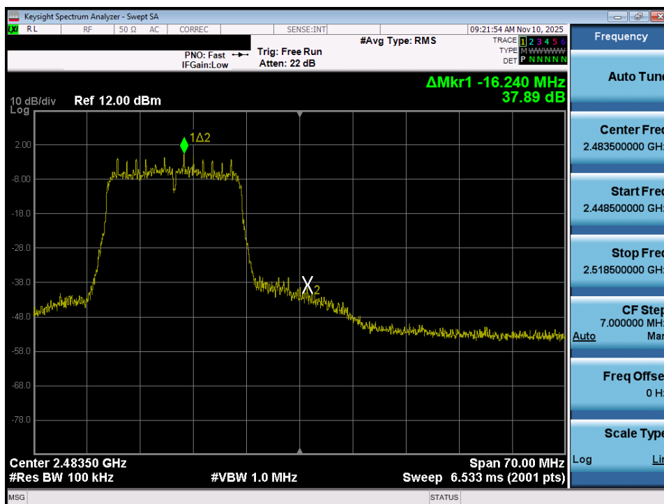
Plot 7-44. Band Edge Plot (802.11n – Ch. 12)
