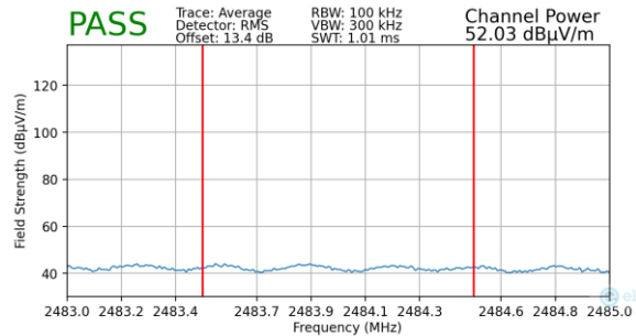
Plot 7-67. Radiated Restricted Upper Band Edge Measurement (Average)
