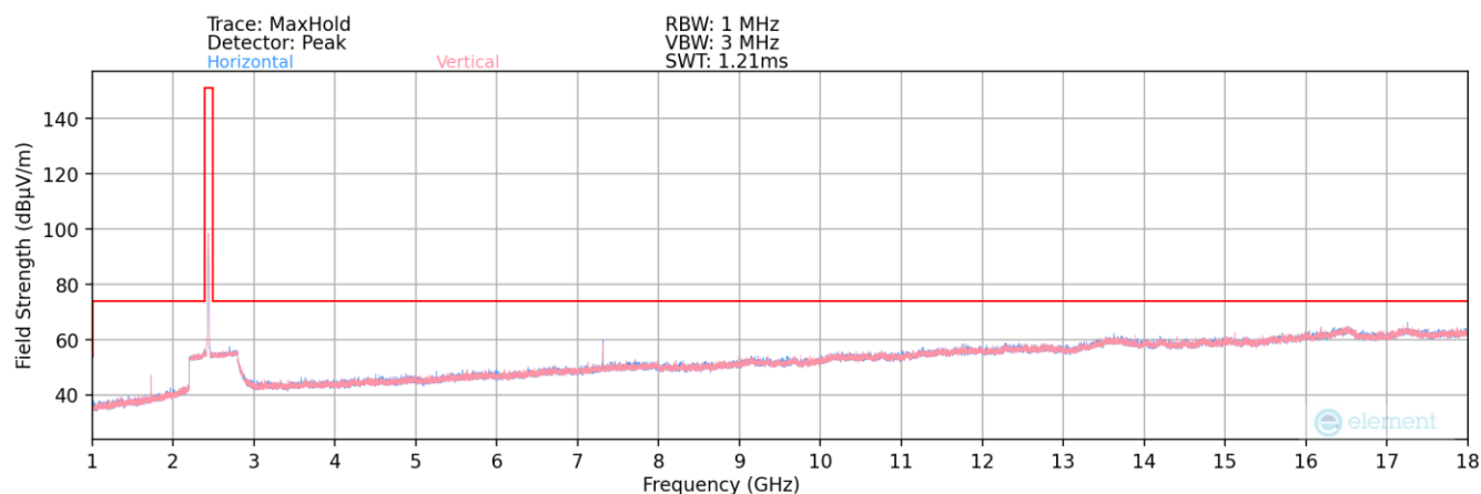
Plot 7-54. Radiated Spurious Plot above 1GHz (802.11b – Ch. 6)
