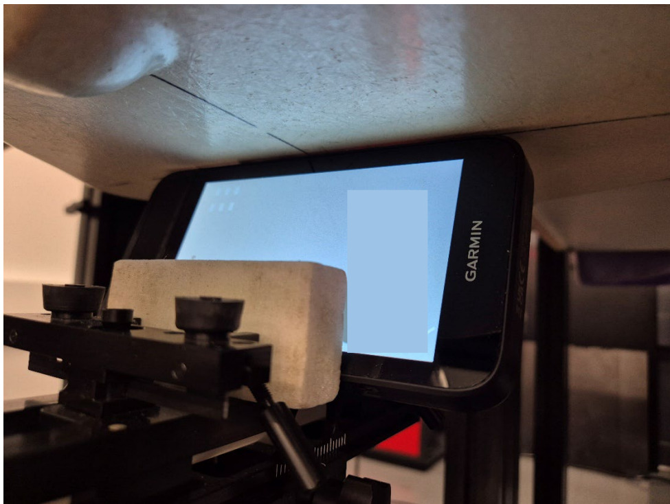
Figure 6 SAR Test Setup – Body/Extremity – Right Edge 0mm
