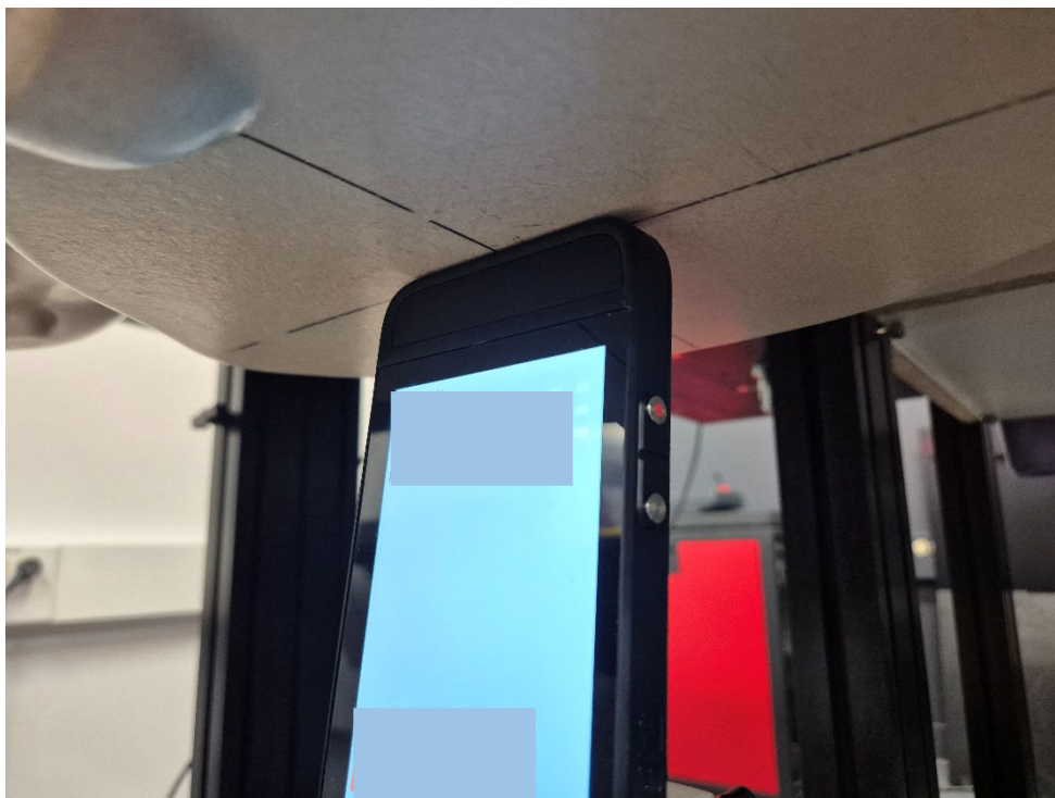
Figure 4 SAR Test Setup – Body/Extremity – Top Edge 0mm
