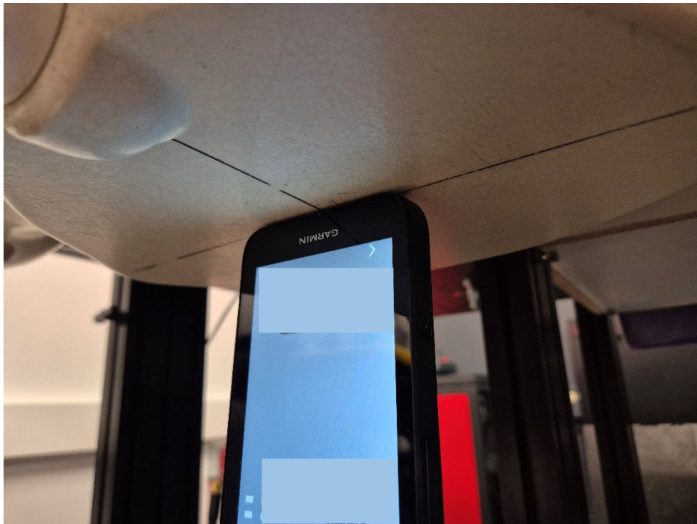
Figure 5 SAR Test Setup – Body/Extremity – Bottom Edge 0mm
