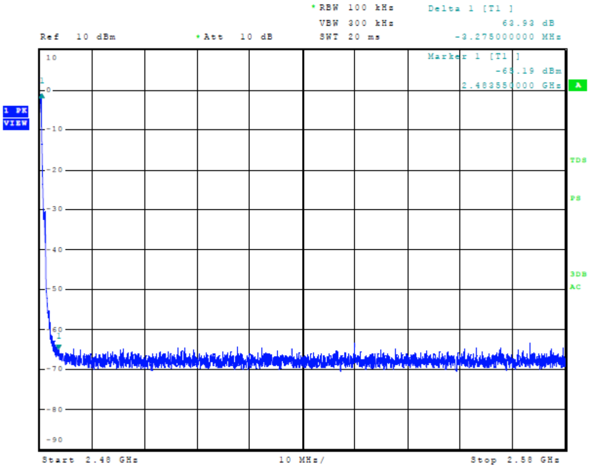
Figure 13 Plot of Transmitter Emissions High Band Edge Mode 1, BT BLE
