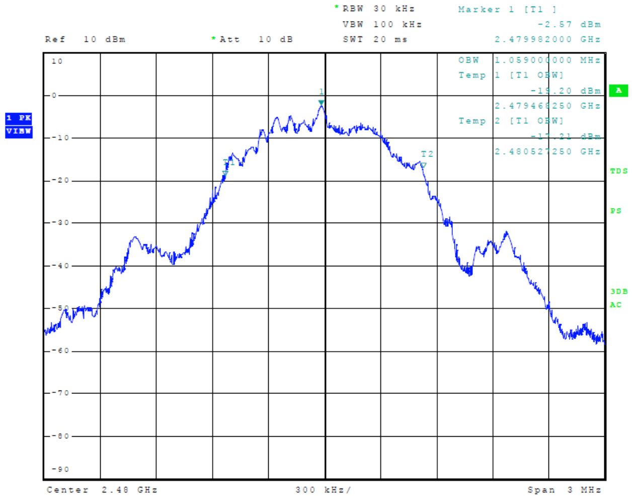
Figure 18 Plot of 99% Occupied Bandwidth Mode 1, BT BLE
