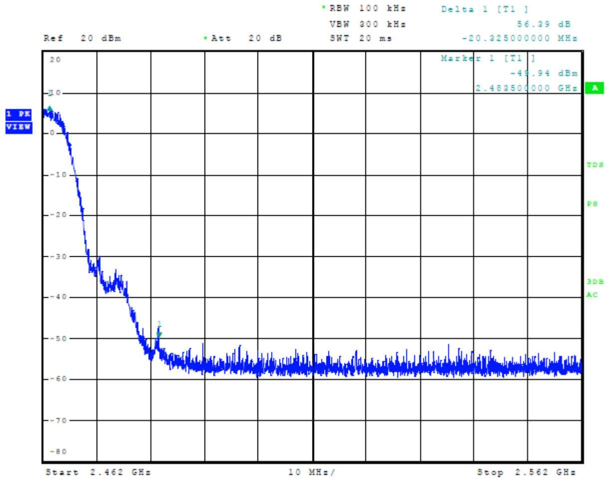
Figure 14 Plot of Transmitter Emissions High Band Edge Mode 2, 802.11b
