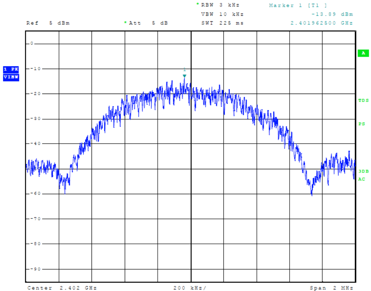
Figure 25 Plot of Transmitter Power Spectral Density Mode 1, BT BLE
