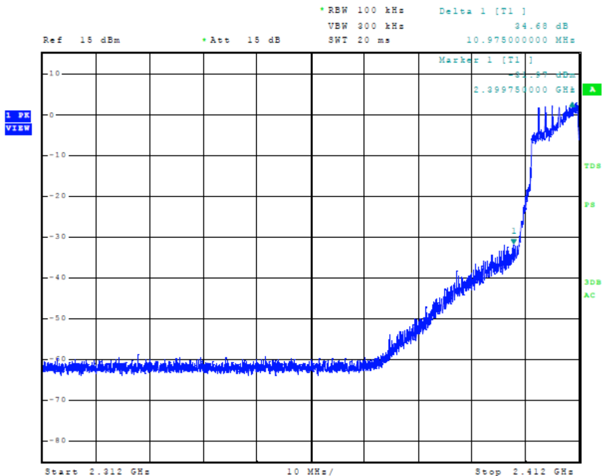
Figure 12 Plot of Emissions Low Band Edge Mode 4, 802.11n
