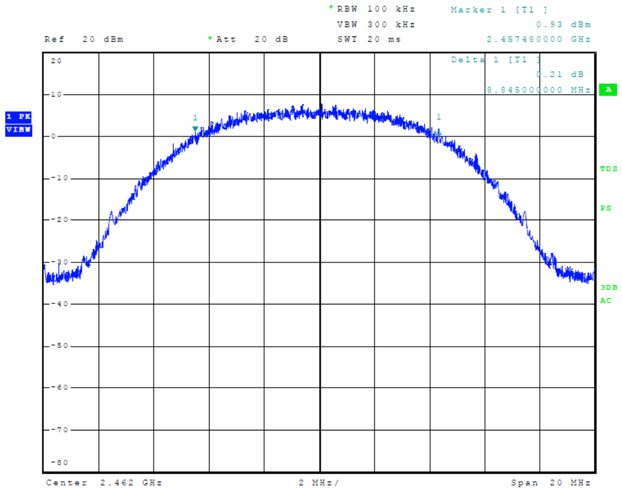
Figure 19 Plot of 6-dB Occupied Bandwidth Mode 2, 802.11b
