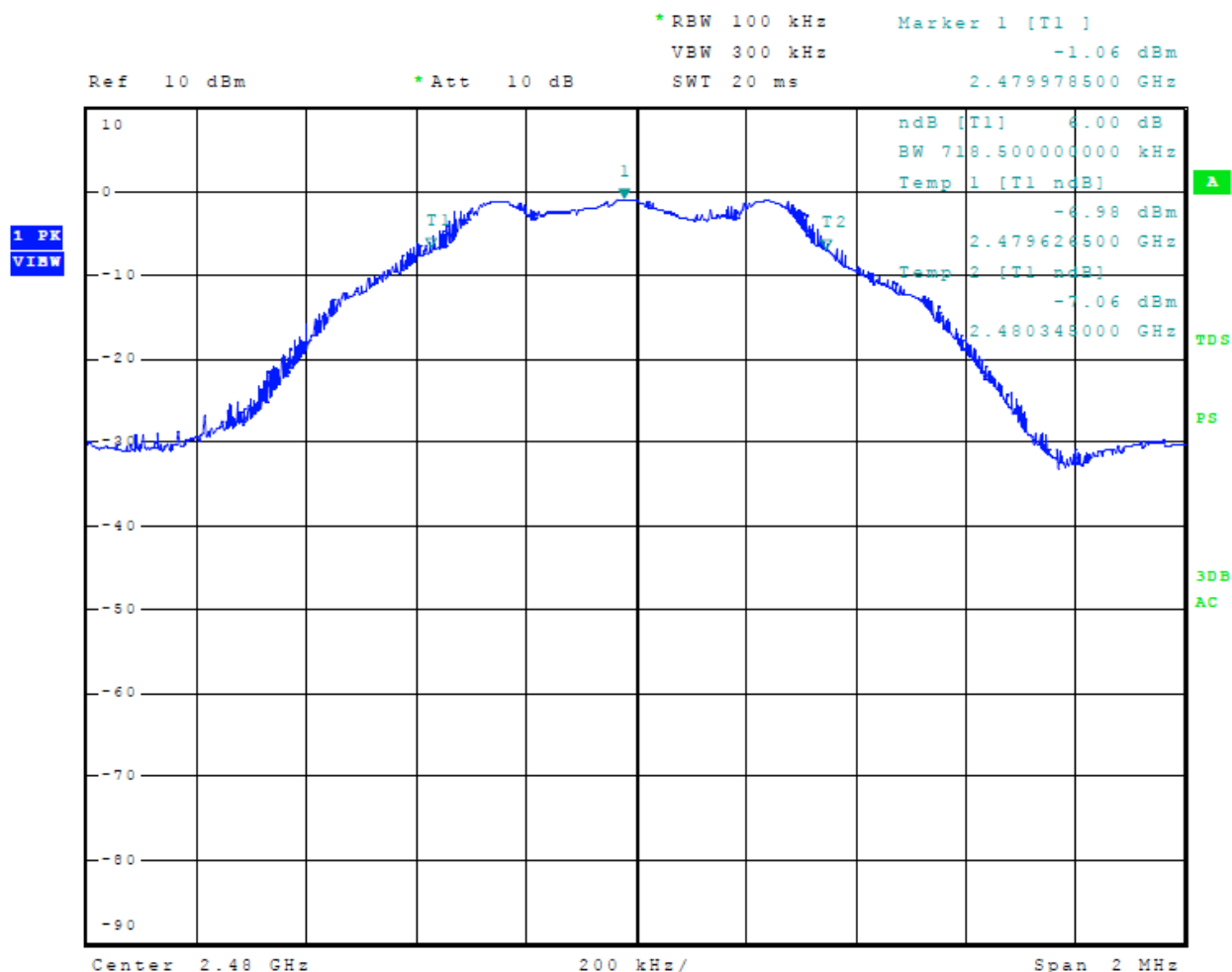
Figure 17 Plot of 6-dB Occupied Bandwidth Mode 1, BT BLE
