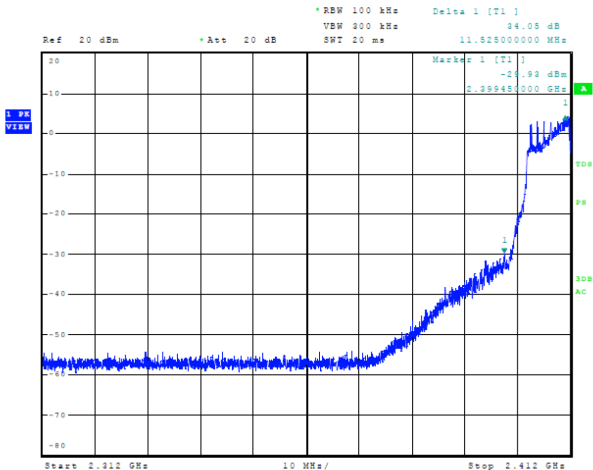
Figure 11 Plot of Emissions Low Band Edge Mode 3, 802.11g
