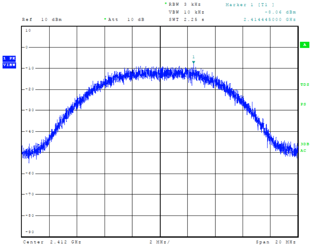
Figure 26 Plot of Transmitter Power Spectral Density Mode 2, 802.11b
