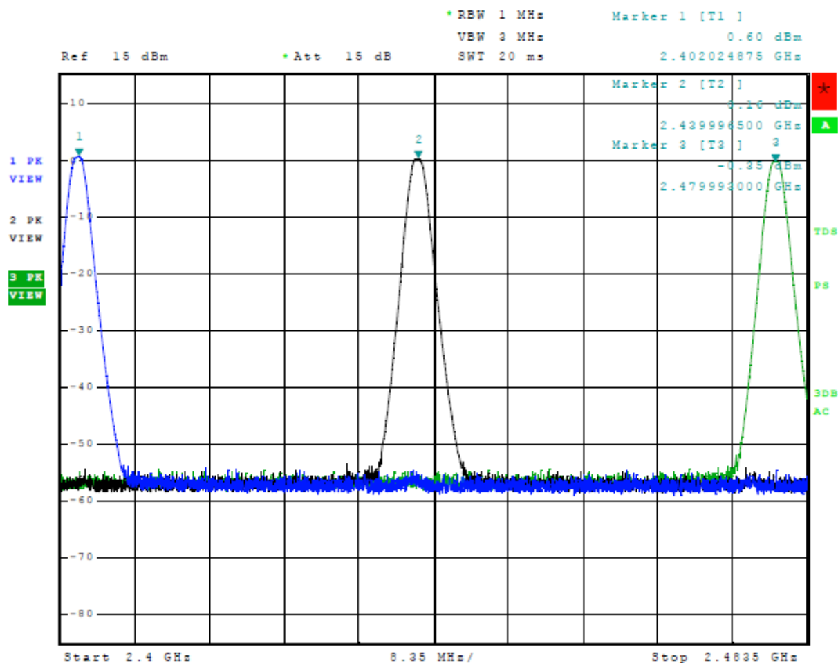
Figure 5 Plot of Transmitter Operation in 2402-2480 MHz Mode 1, BT BLE
