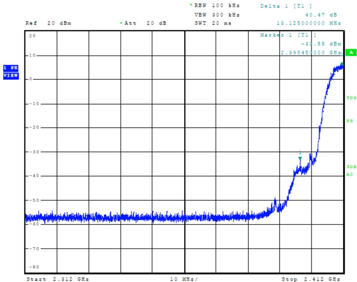
Figure 10 Plot of Emissions Low Band Edge Mode 2, 802.11b
