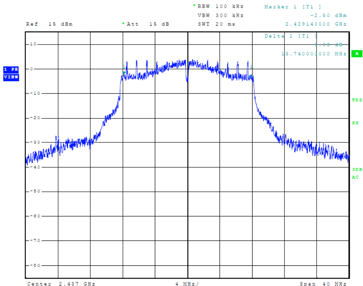
Figure 21 Plot of 6-dB Occupied Bandwidth Mode 3, 802.11g
