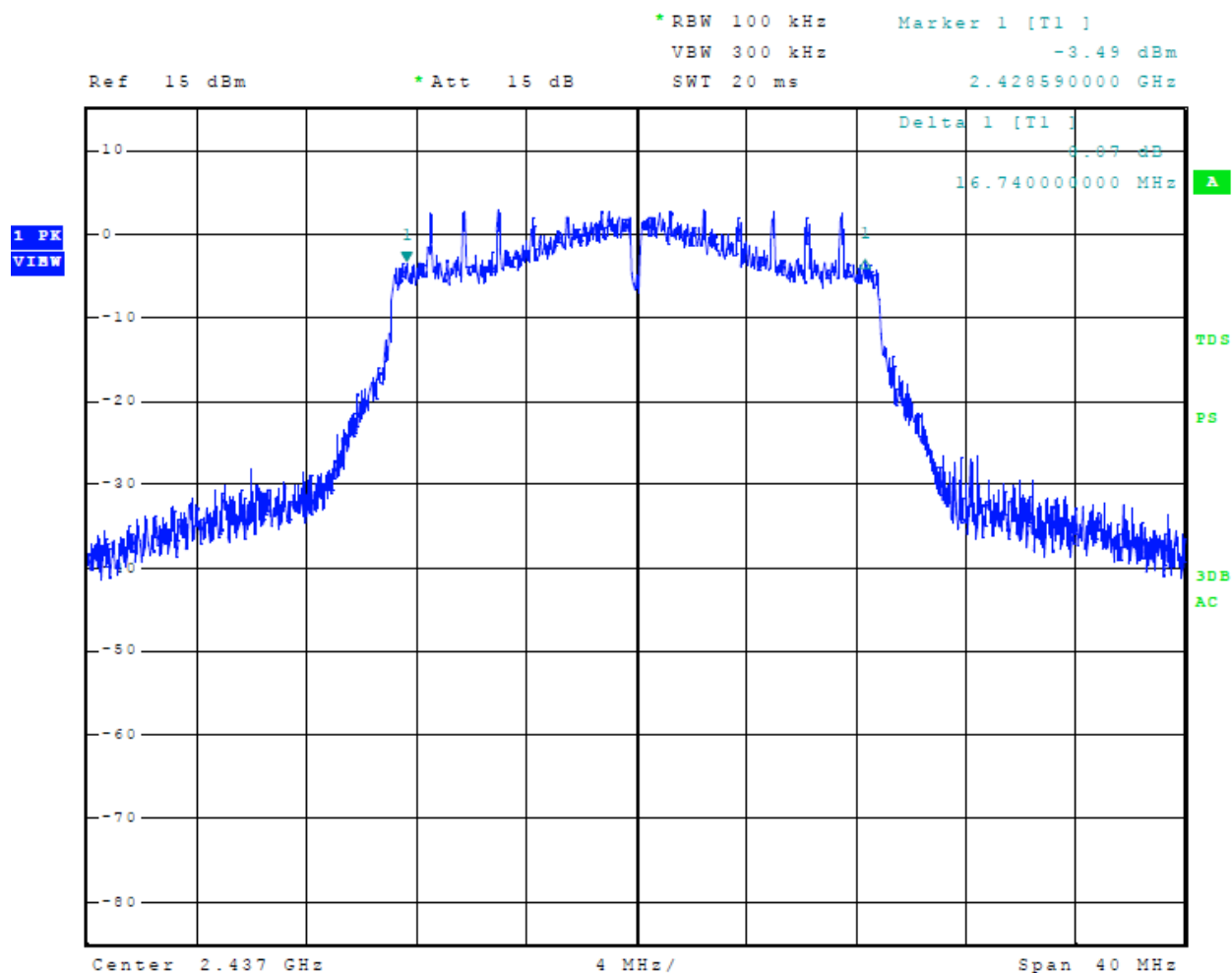
Figure 23 Plot of 6-dB Occupied Bandwidth Mode 4, 802.11n
