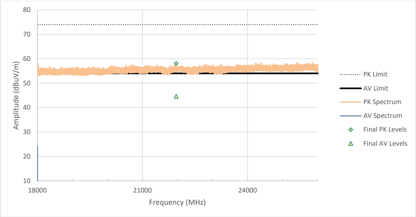
Figure RE23.1: Spectral data
