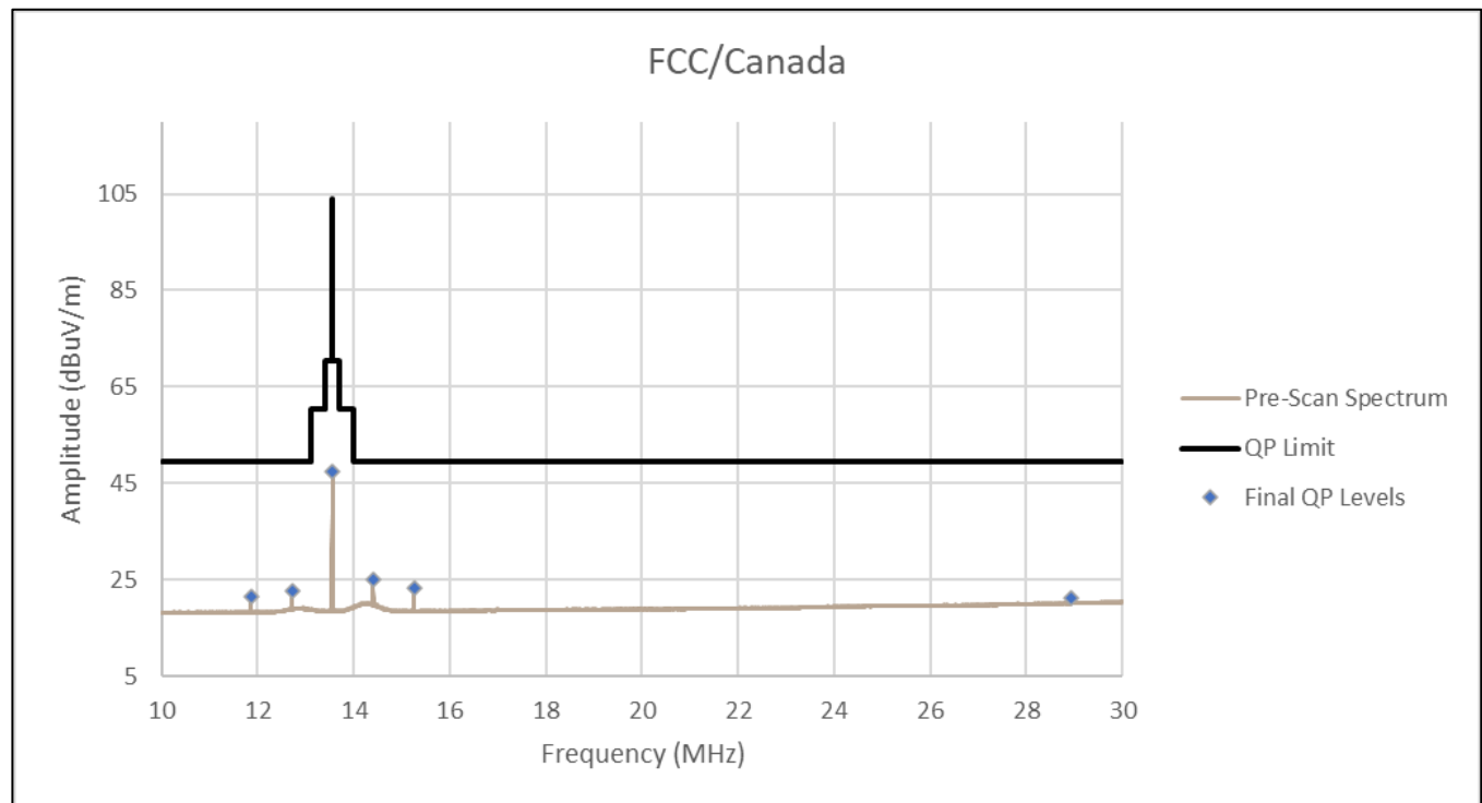
Figure RE19.1: Spectral data
