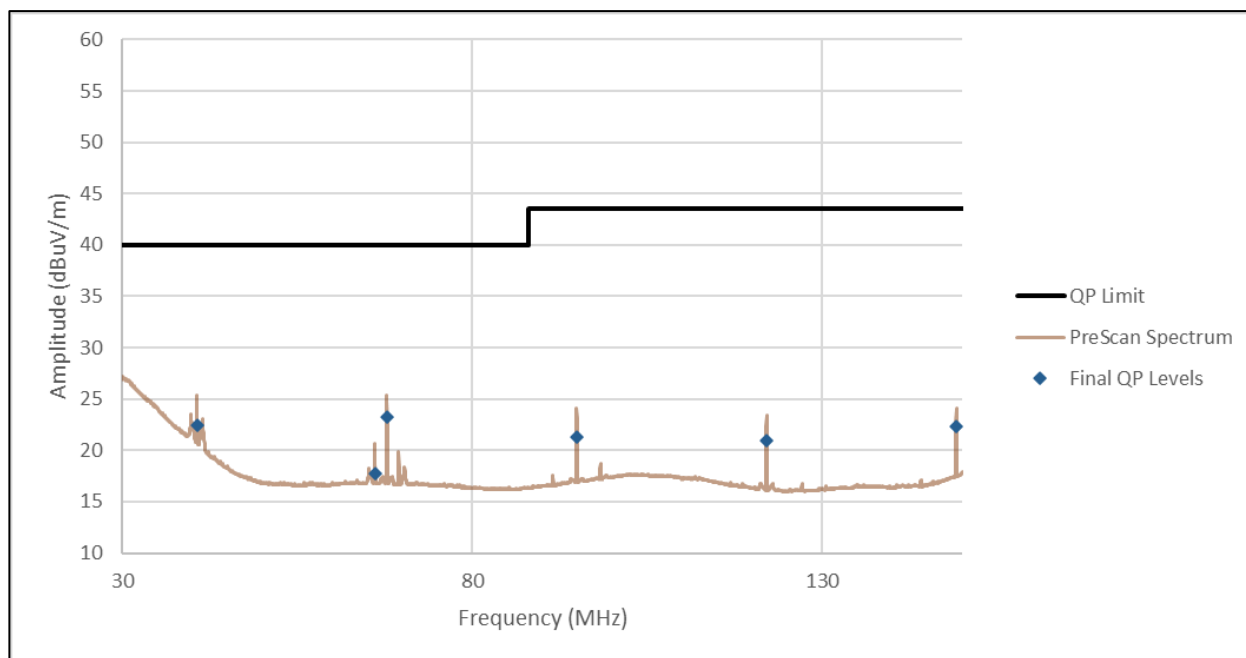
Figure RE20.1: Spectral data
