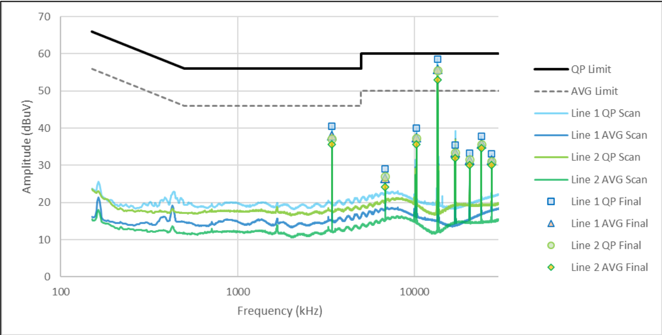
Figure CE04.1: Spectral data (NFC)
