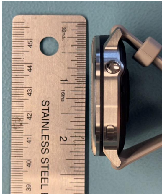
Photograph 7-4 : Right side view of the device
