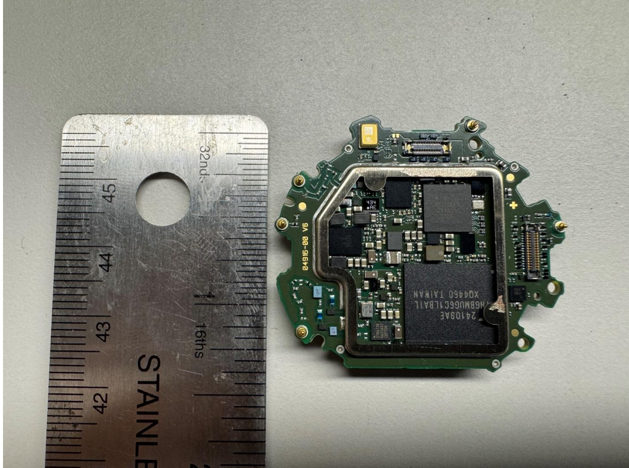
Photograph 6-3 : Front side view of the main board, shields removed
