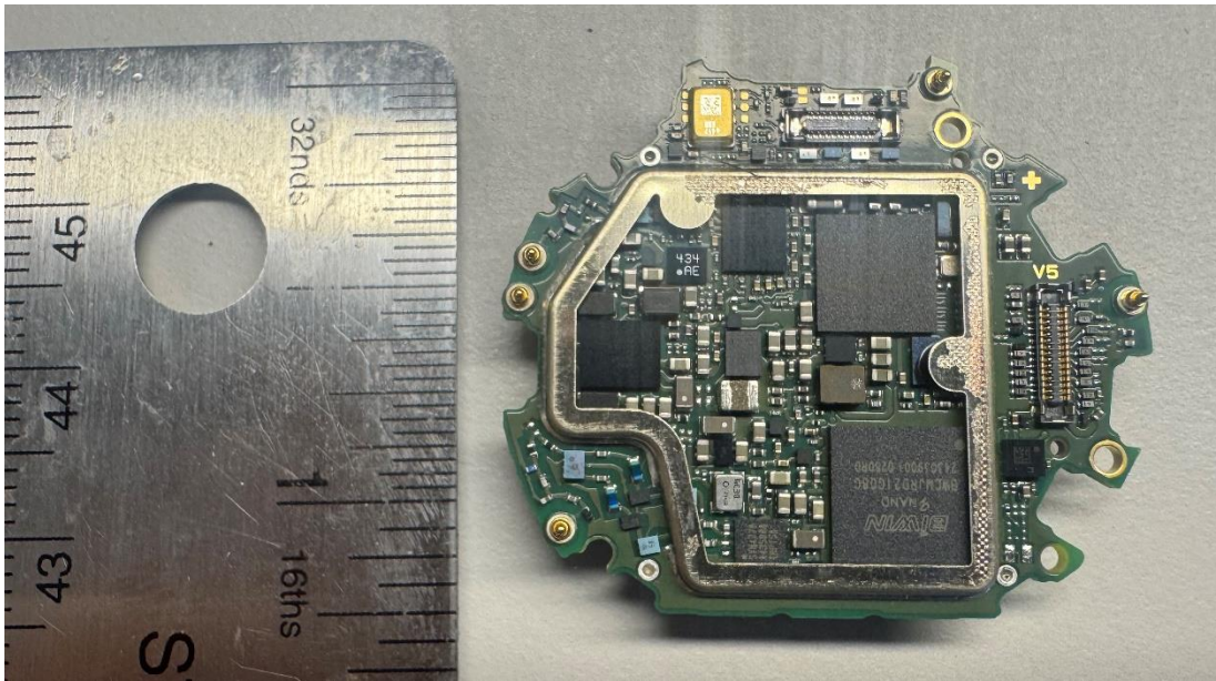
Photograph 6-3 : Front side view of the main board, shields removed
