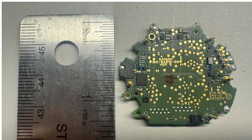
Photograph 6-2 : Back side view of the main board
