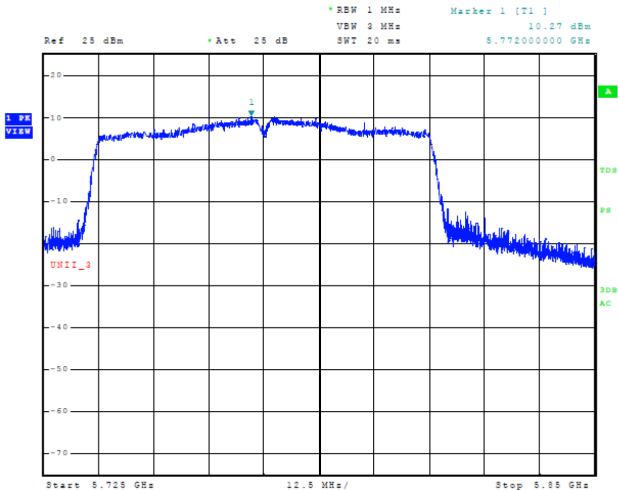
Figure 10 Plot of Transmitter Emissions Across 5725-5850 MHz Mode 15 U-NII-3 (802.11ac80)
