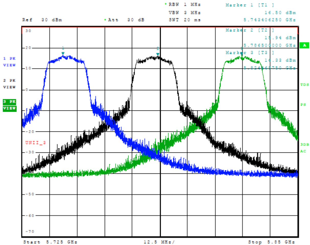
Figure 8 Plot of Transmitter Emissions Across 5725-5850 MHz Mode 13 U-NII-3 (802.11n)
