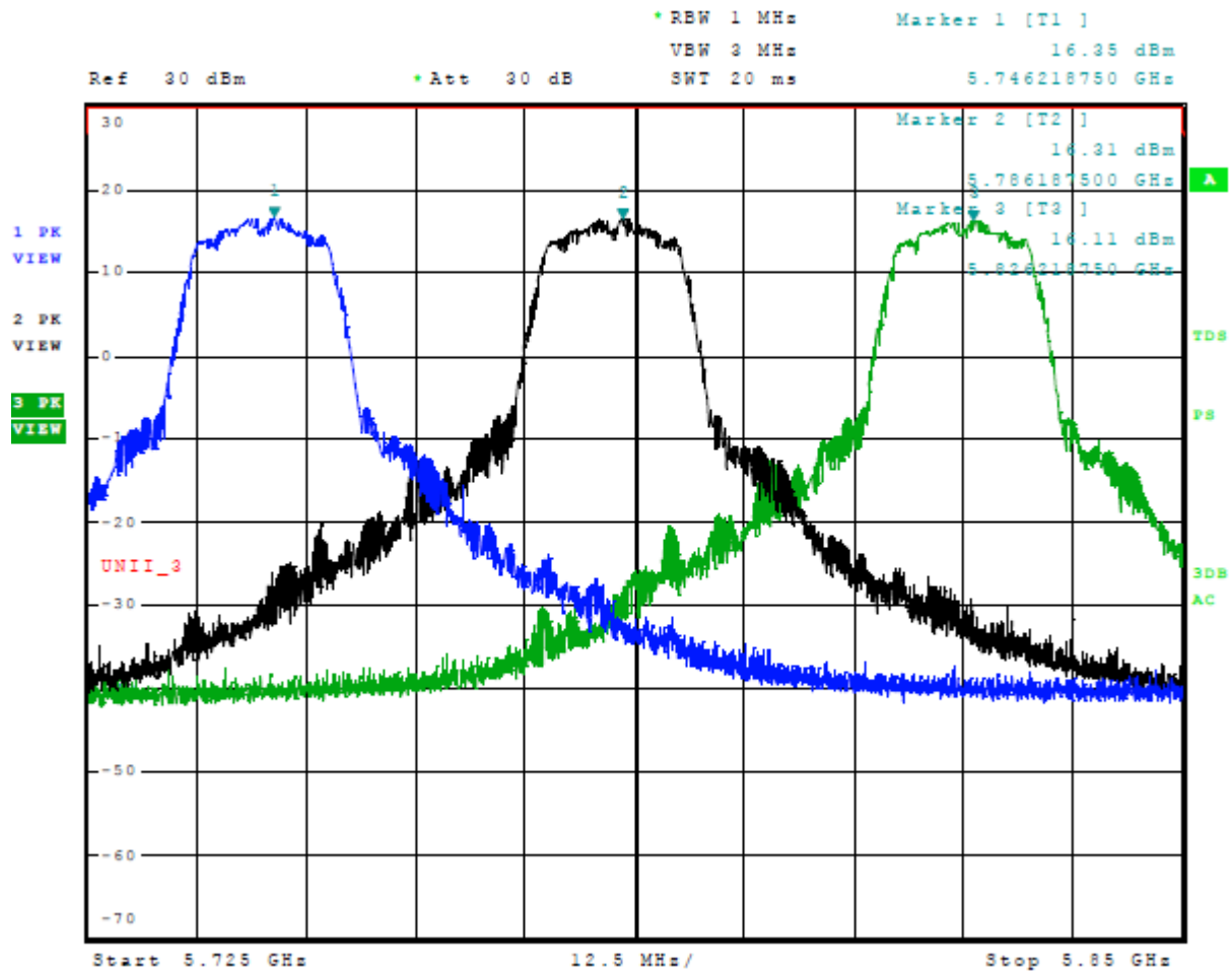
Figure 7 Plot of Transmitter Emissions Across 5725-5850 MHz Mode 12 U-NII-3 (802.11a)
