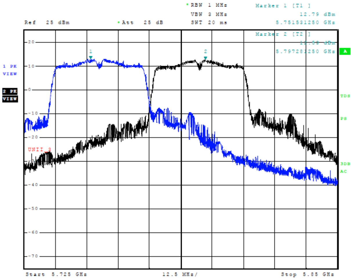
Figure 9 Plot of Transmitter Emissions Across 5725-5850 MHz Mode 14 U-NII-3 (802.11n40)
