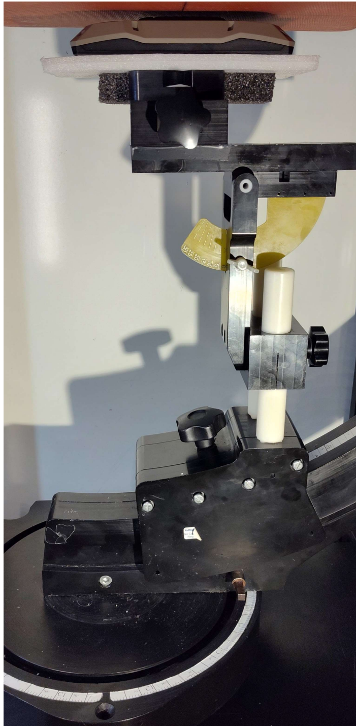
Figure C.7 – Setup Photo, Body - Back - Far
