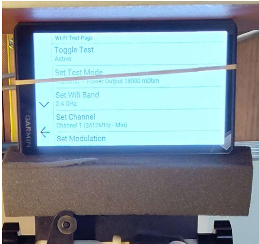
Figure C.6 – Setup Photo, Extremity - Top Edge - Close
