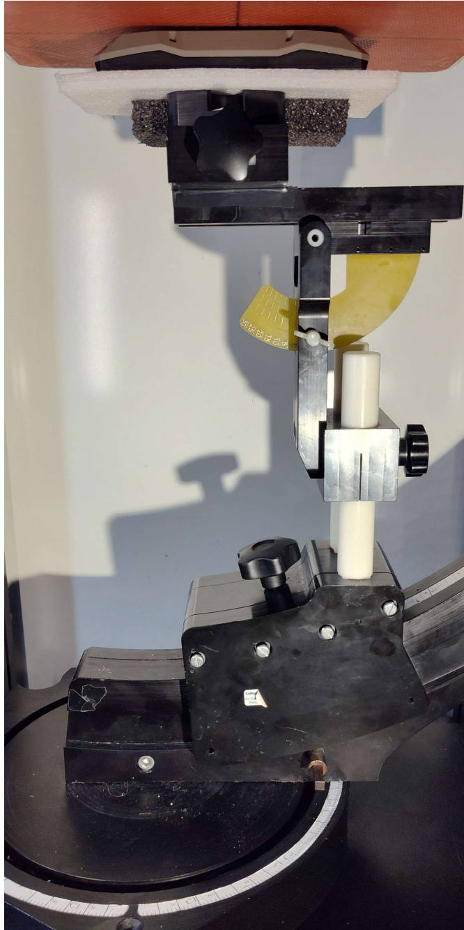
Figure C.1 – Setup Photo, Extremity - Back Touch – Far
