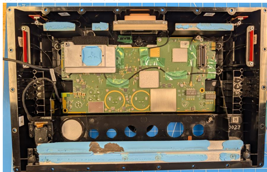
B04946 Back Case with PCBA#2 Removed
