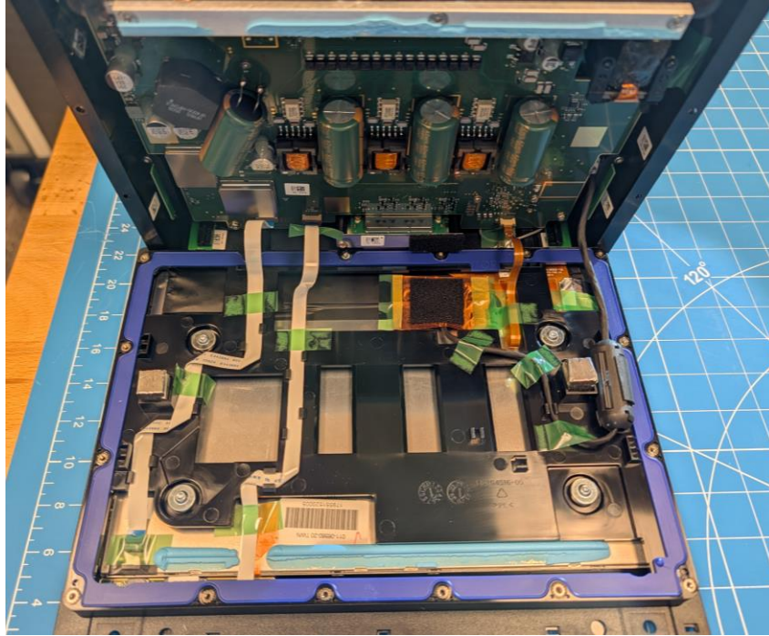
C04946 Case Opened showing Front and Back Case
