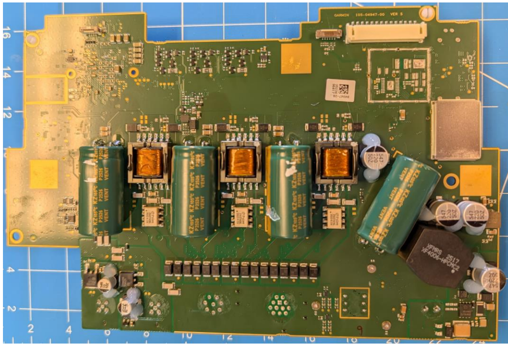
x04946 PCBA#2 Front with Shields
