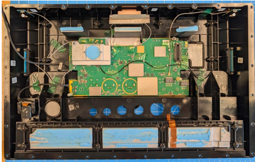
A04946 Back Case showing PCBA#2 Removed
