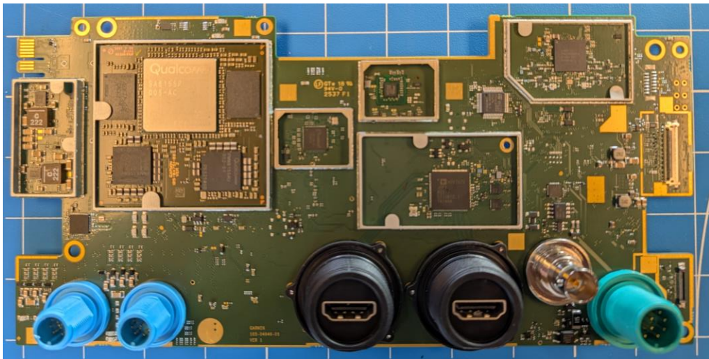
x04946 PCBA#1 Back without Shields and RF Absorber
