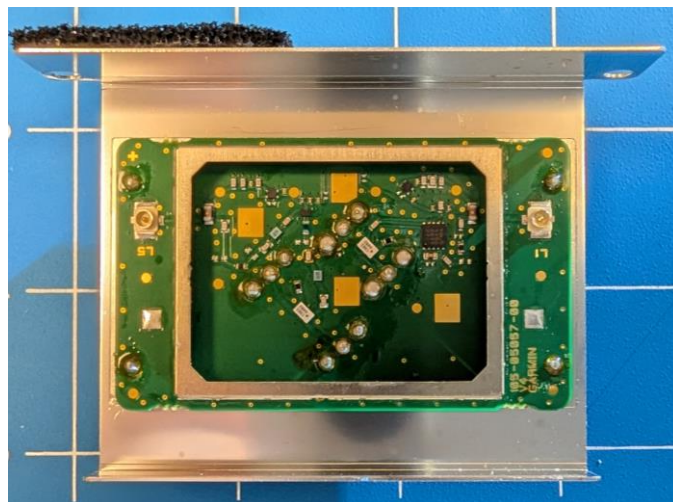
x04946 GPS/GNSS Module Back without Shields
