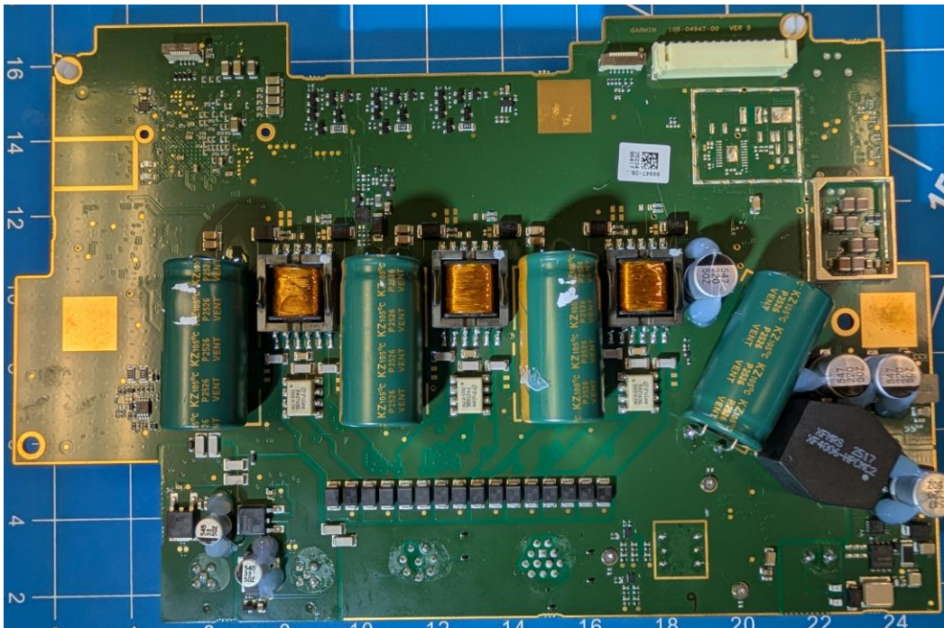
x04946 PCBA#2 Front without Shields
