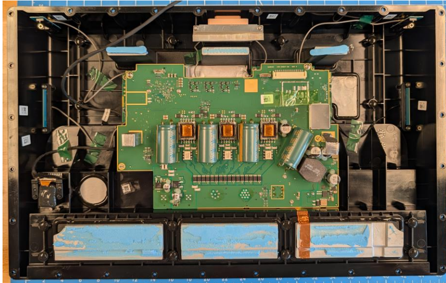
A04946 Back Case with PCBAs Installed, GPS/GNSS Module Installed, and Antennas Installed
