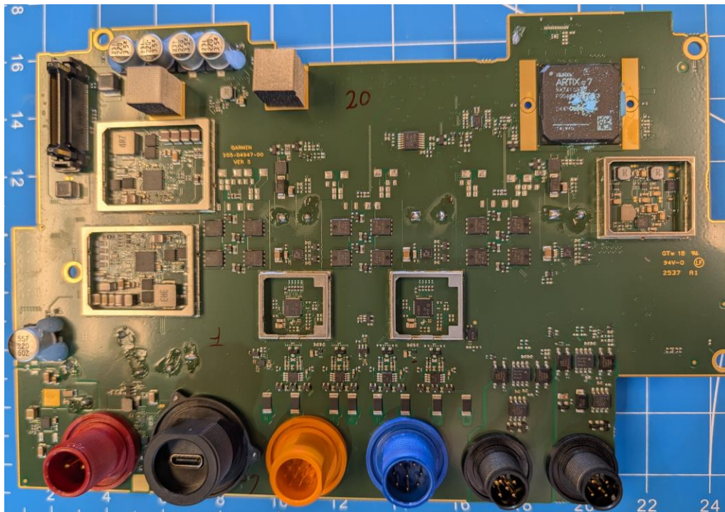
x04946 PCBA#2 Back without Shields
