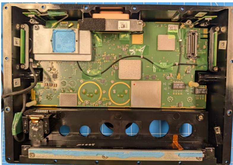
C04946 Back Case with PCBA#2 Removed
