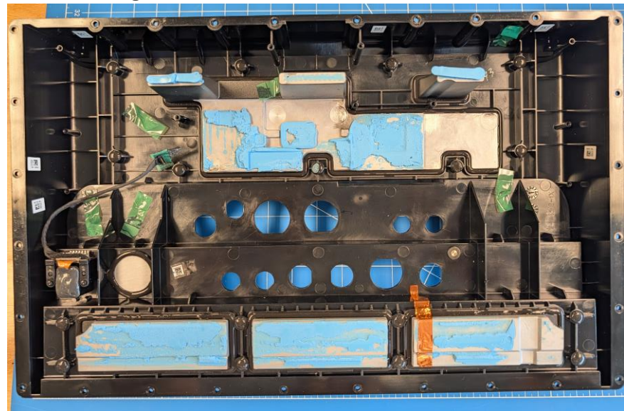
A04946 Back Case showing all PCBAs removed
