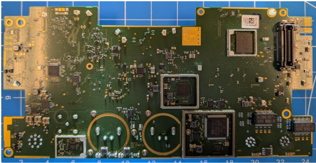
x04946 PCBA#1 Back with Shields and RF Absorber
