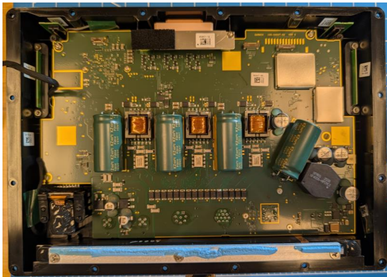
C04946 Back Case with all PCBAs, GPS/GNSS module, and Antennas
