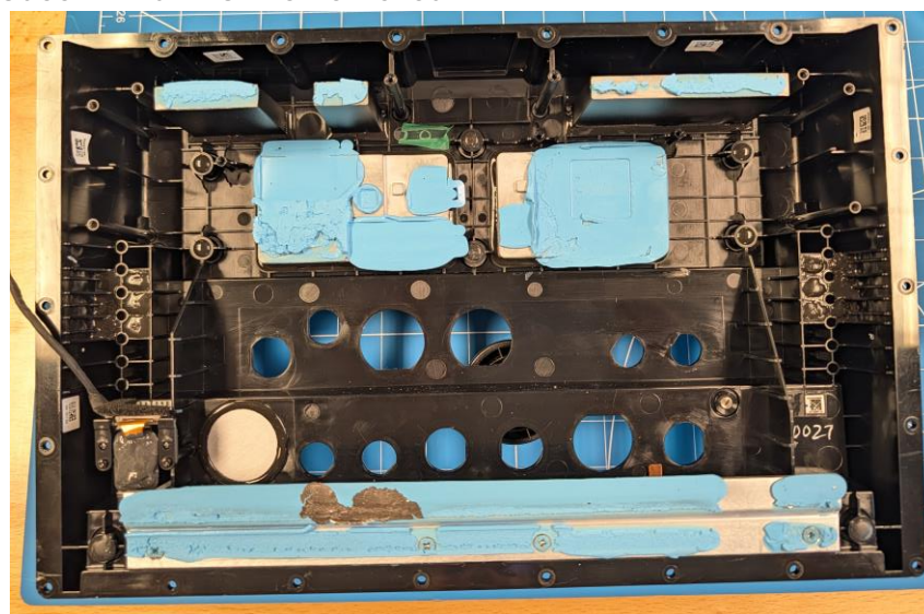
B04946 Back Case with all PCBAs Removed
