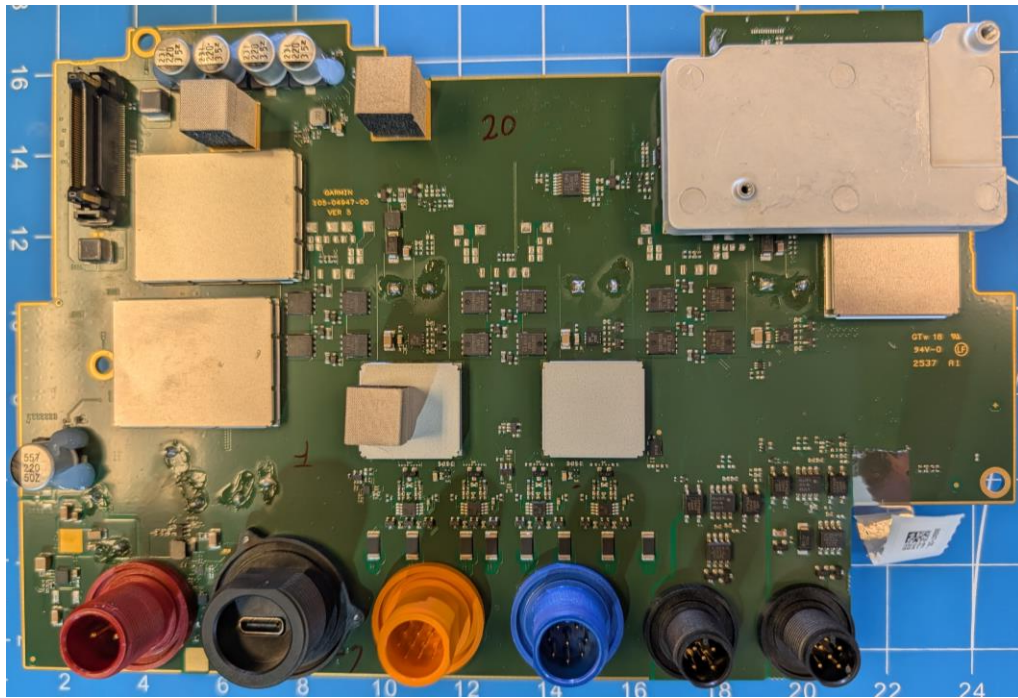
x04946 PCBA#2 Back with Shields
