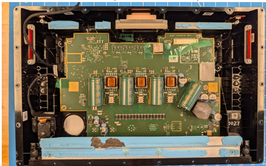
B04946 Inside Back Case with all PCBAs, GPS/GNSS module, and Antennas
