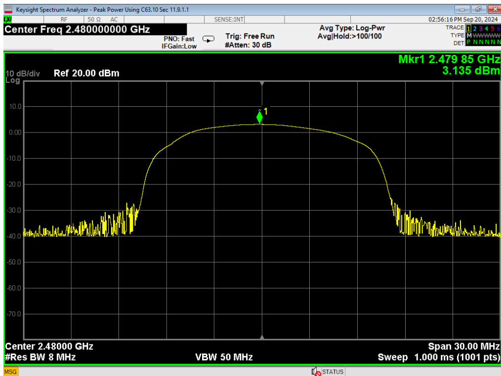
03 Peak Power, BLE 1MB, High
