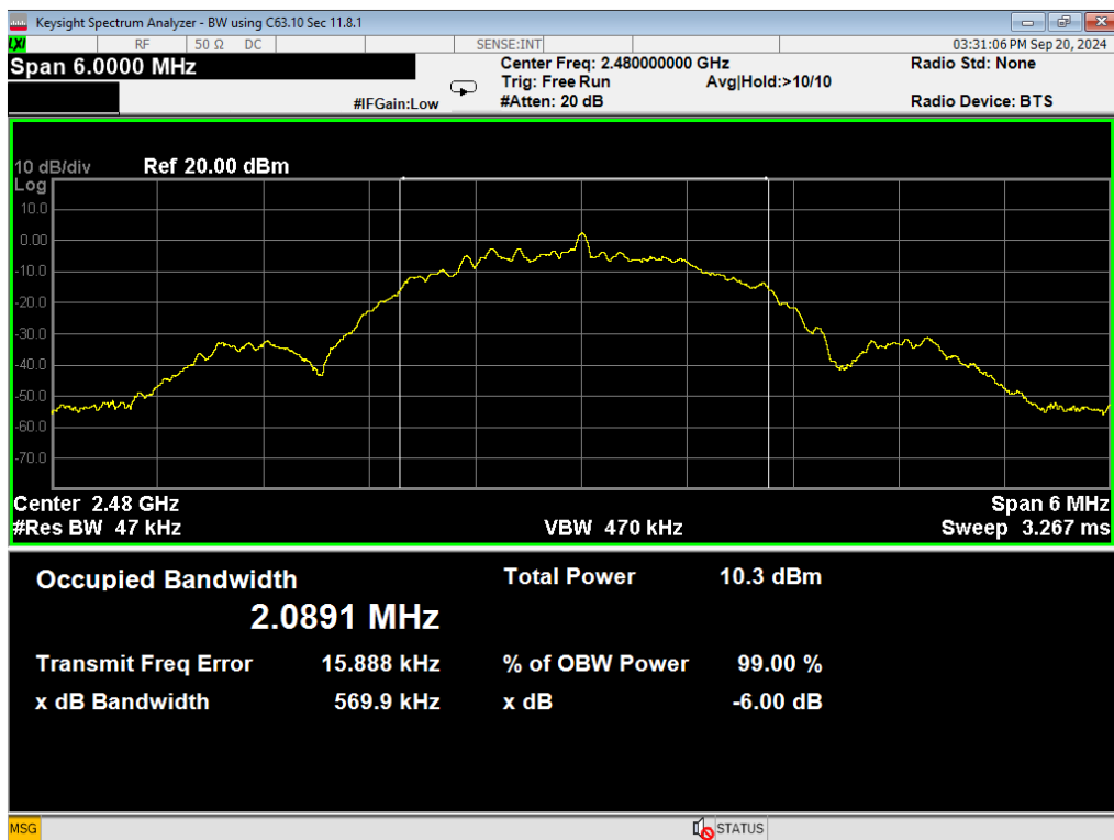
22 Occupied BW, BLE 2MB, High
