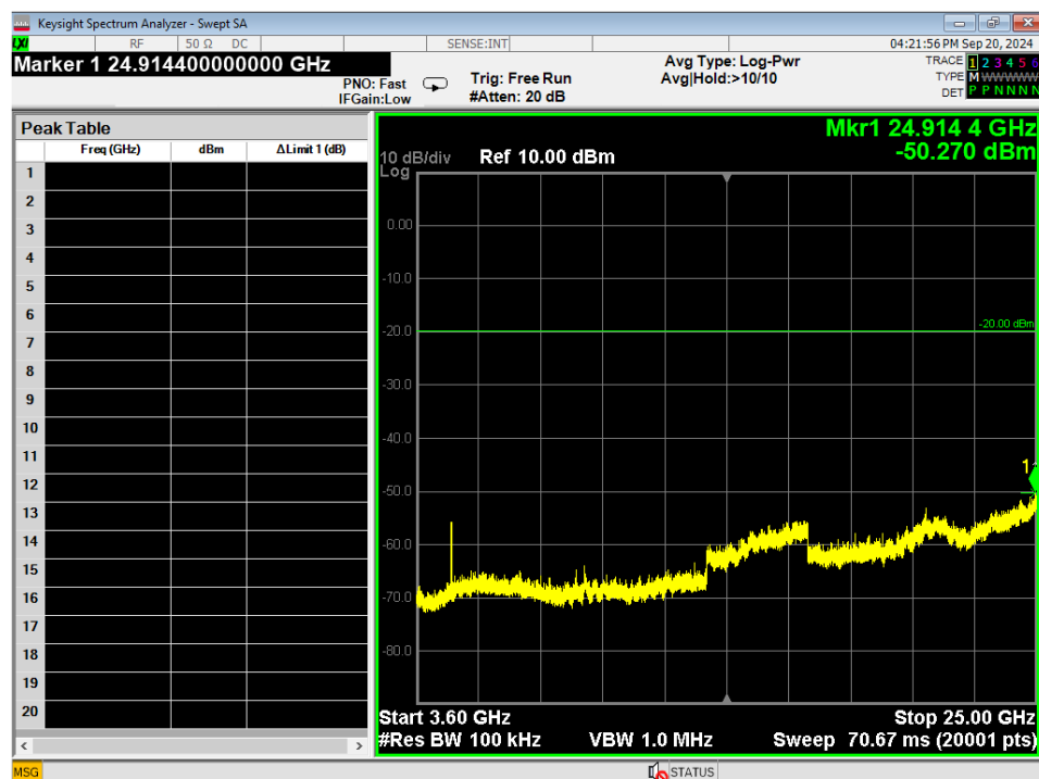
Figure 14 - Radiated Emissions Plot, GMSK 2MB, 3.6GHz – 25GHz, Mid
