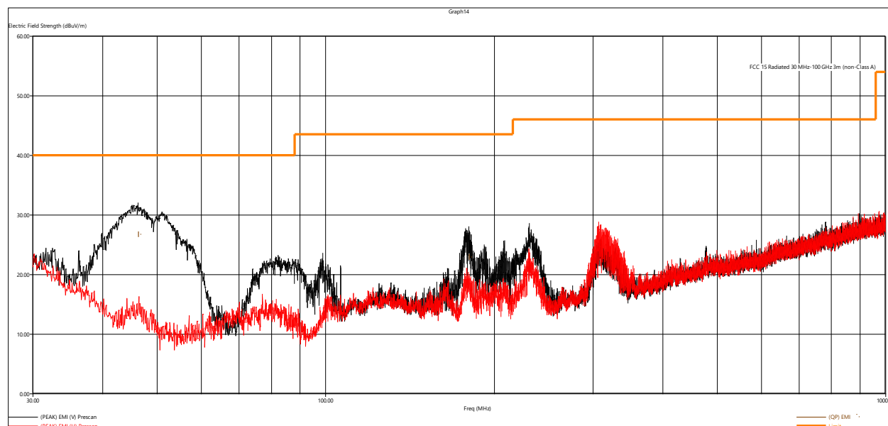
Figure 7 - Radiated Emissions Plot, GMSK 1MB
