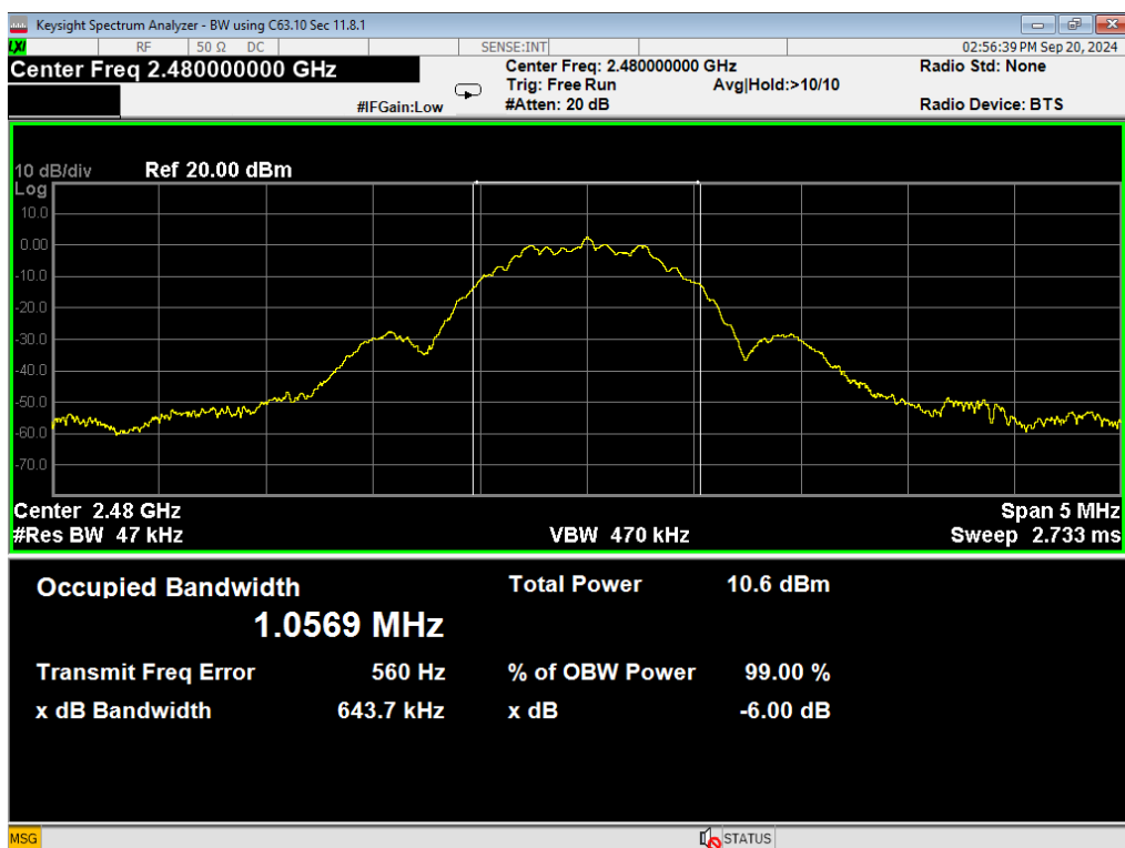
06 Occupied BW, BLE 1MB, High
