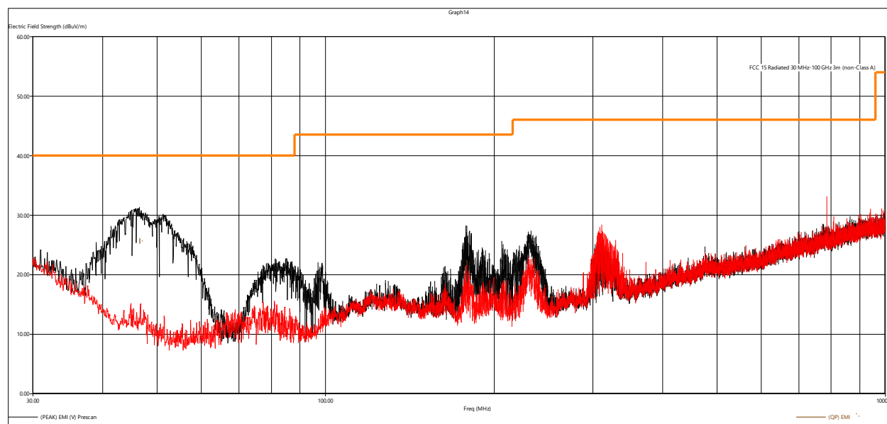
Figure 8 - Radiated Emissions Plot, GMSK 2MB
