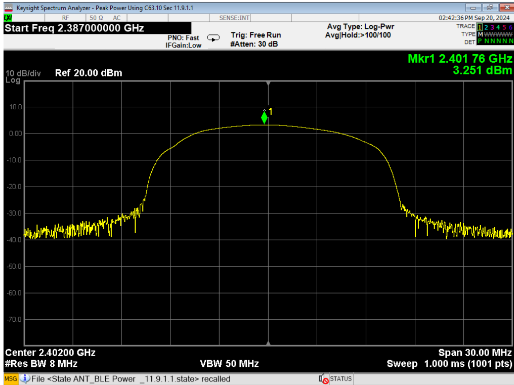
01 Peak Power, BLE 1MB, Low
