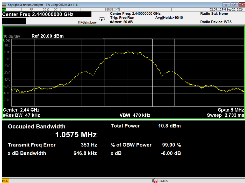
05 Occupied BW, BLE 1MB, Mid
