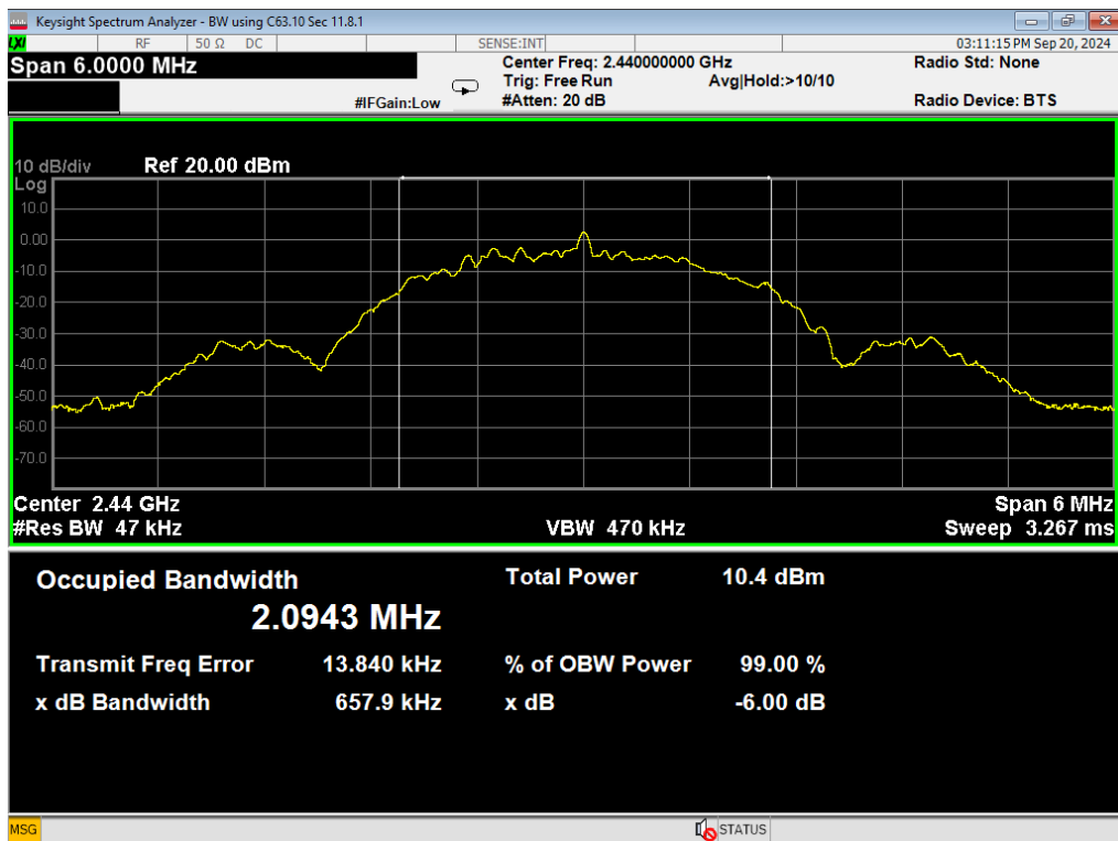
21 Occupied BW, BLE 2MB, Mid
