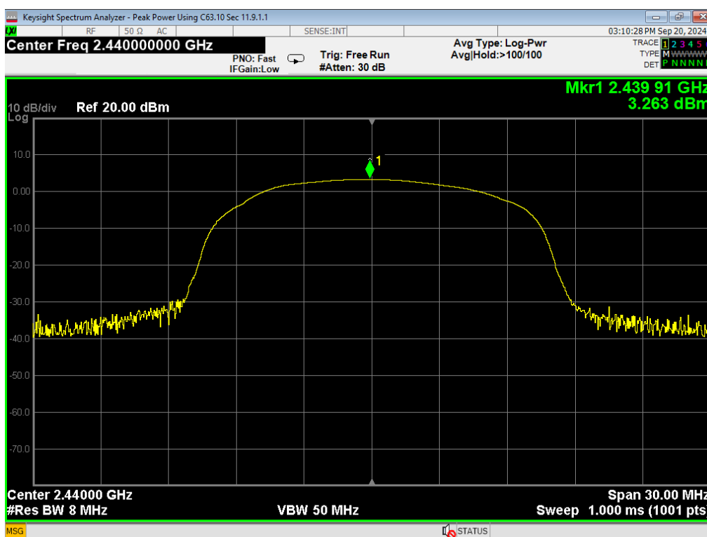
18 Peak Power, BLE 2MB, Mid
