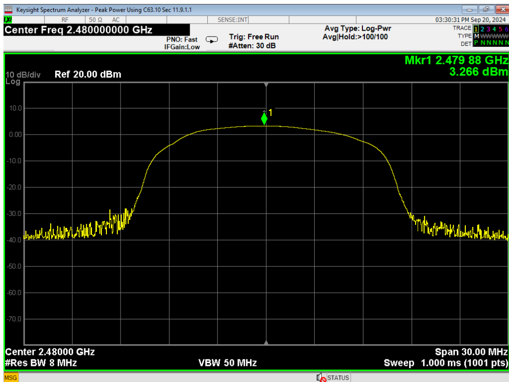
19 Peak Power, BLE 2MB, High
