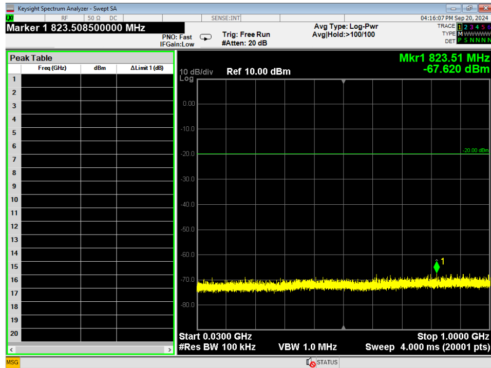
Figure 9 - Radiated Emissions Plot, GMSK 1MB, 30MHz – 1GHz, Mid
