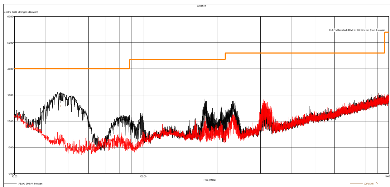
Figure 6 - Radiated Emissions Plot, Receive
