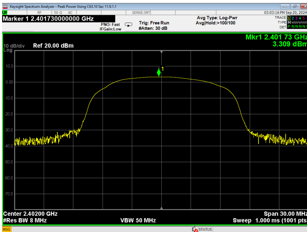
17 Peak Power, BLE 2MB, Low
