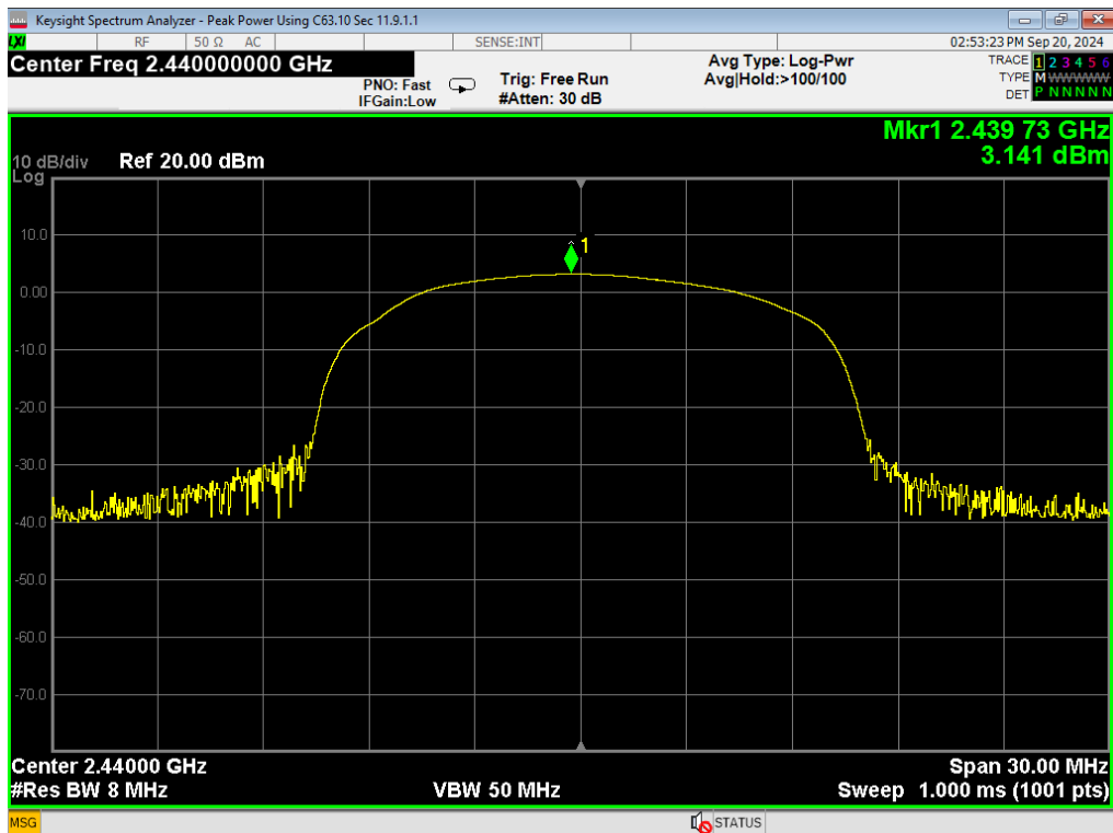
02 Peak Power, BLE 1MB, Mid
