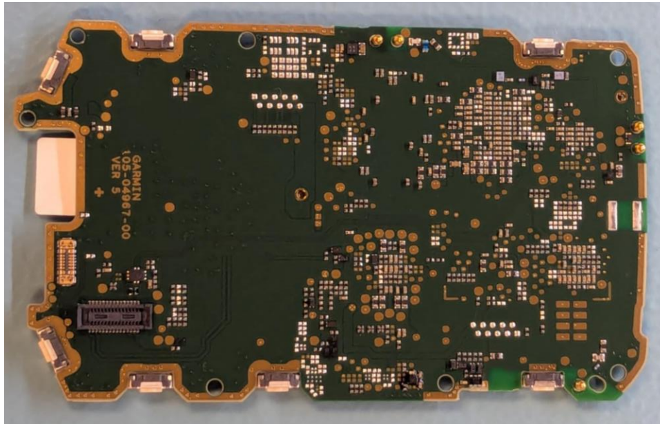
Photograph 07-3: Back side view of the main board
