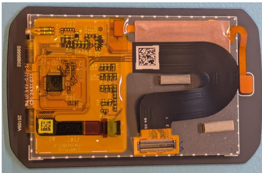
Photograph 07-6: Screen connections
