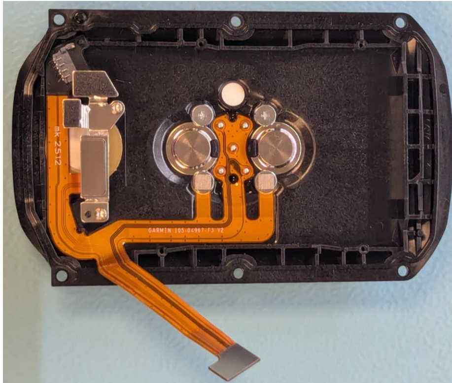
Photograph 07-5: Lower enclosure components – battery removed
