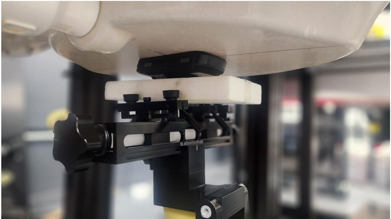
Figure C SAR Test Setup – Body/Extremity – Front 0mm
