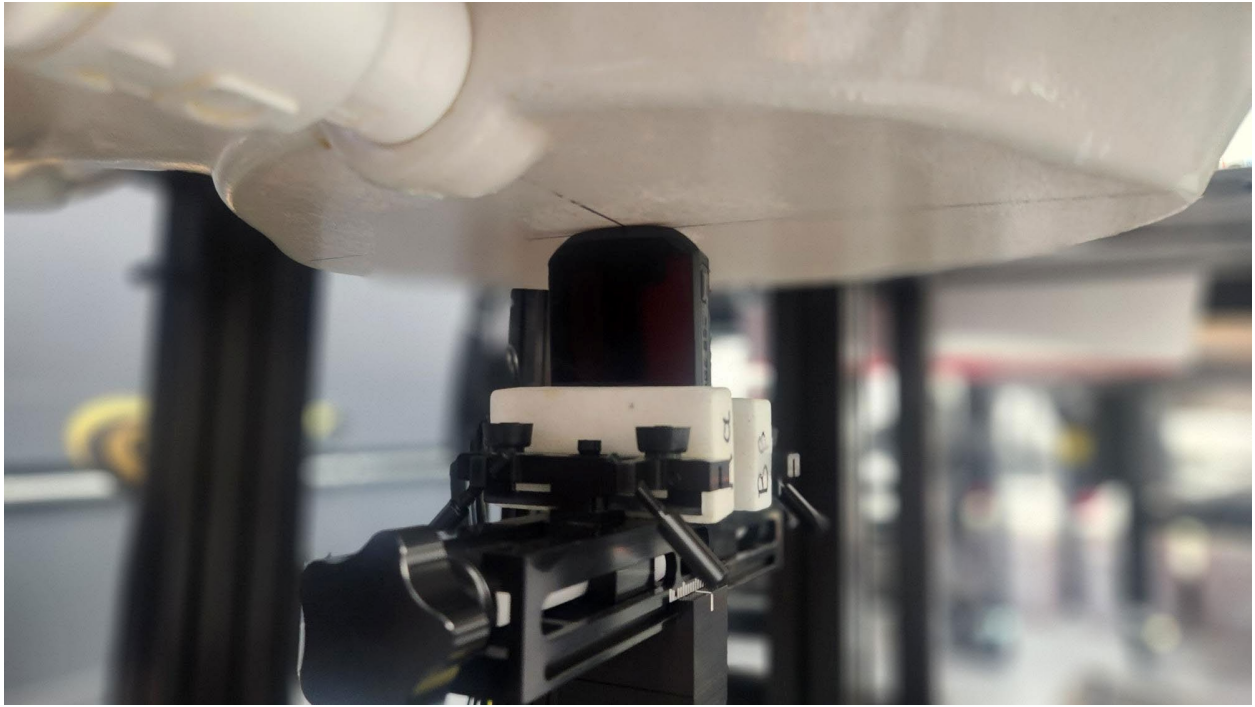
Figure D SAR Test Setup – Body/Extremity – Top 0mm
