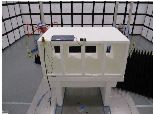
1-40GHz (BACK)
