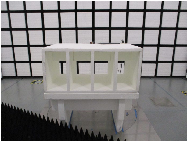
1-40GHz (FRONT)
