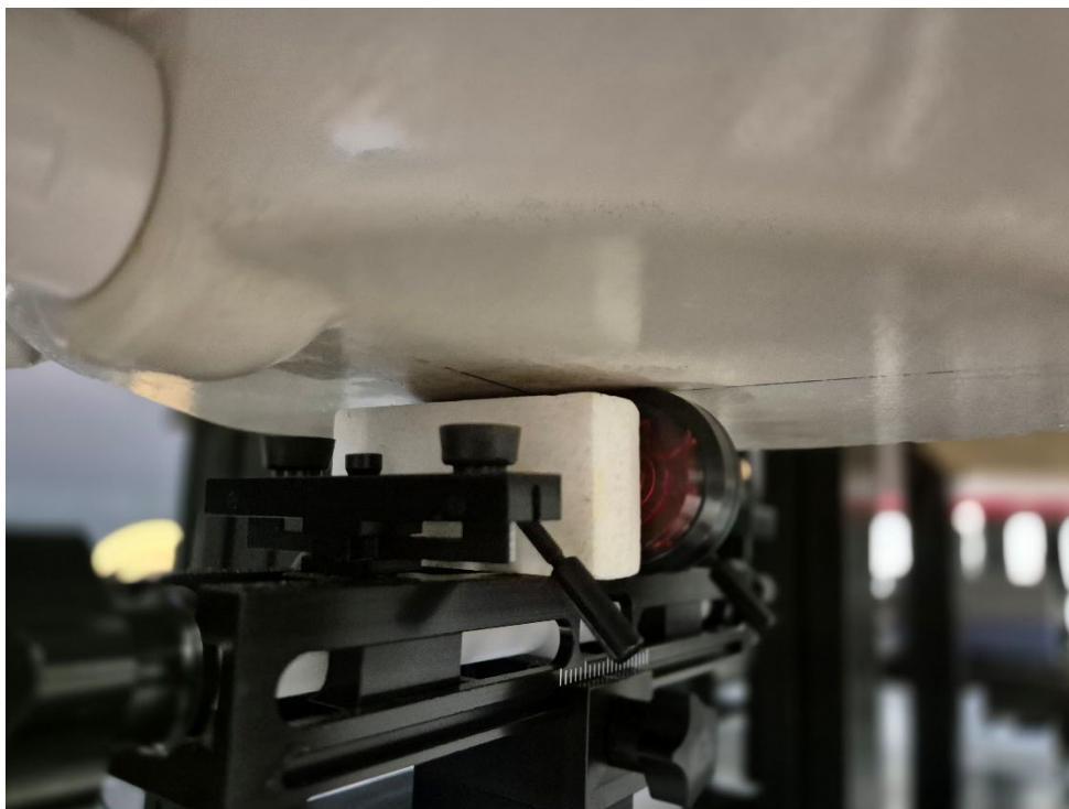
Figure 6 SAR Test Setup – Body/Extremity – Left 0mm
