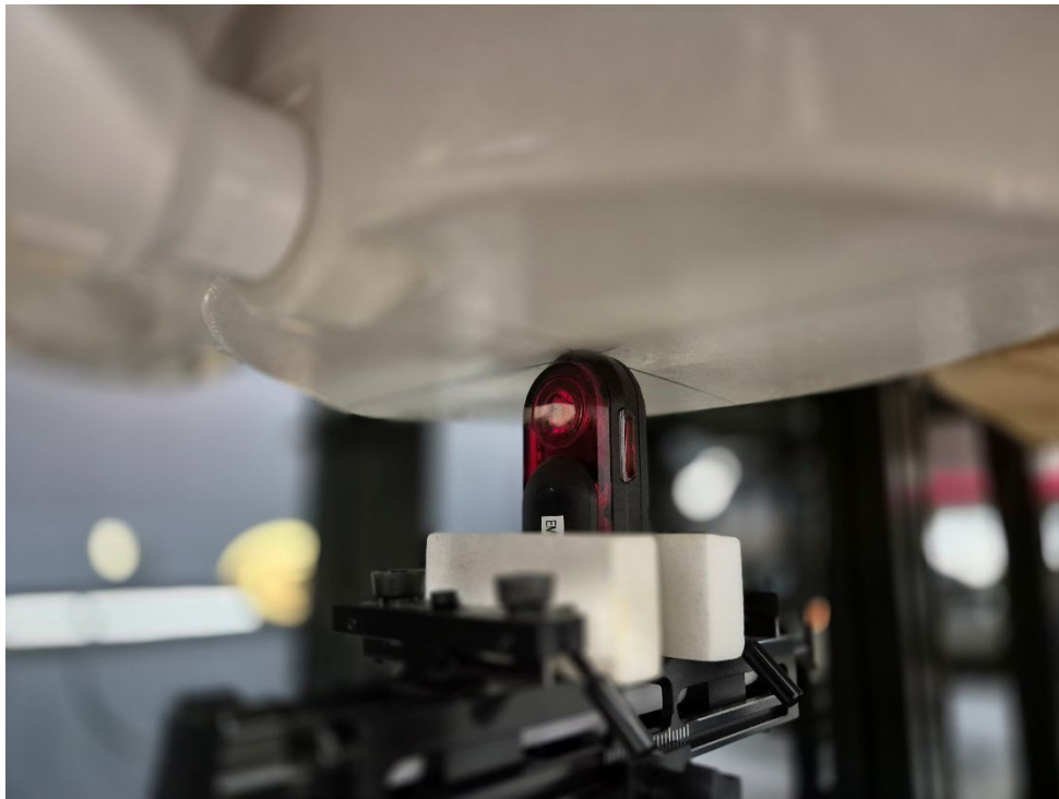
Figure 3 SAR Test Setup – Body/Extremity – Top 0mm
