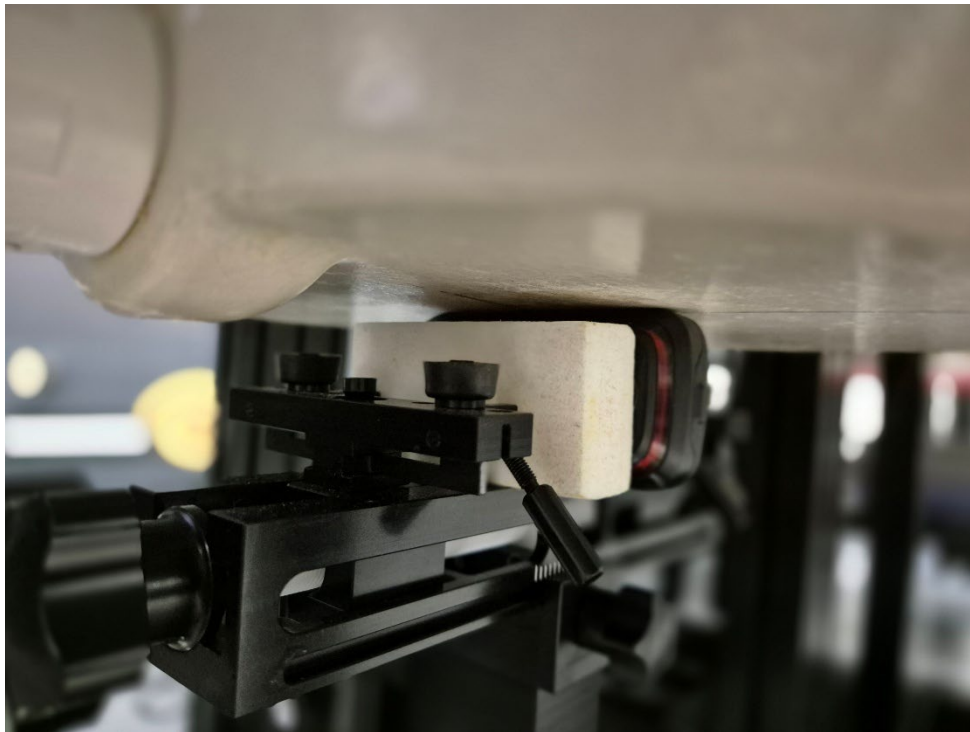
Figure 5 SAR Test Setup – Body/Extremity – Right 0mm
