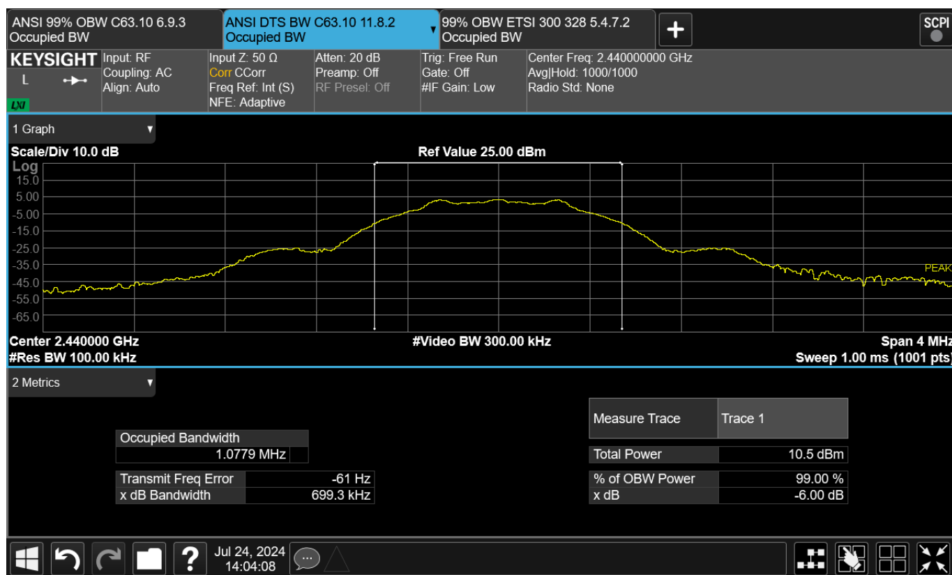
Figure TR06.2: Bandwidth data for BLE 1 at mid channel (2440 MHz)
