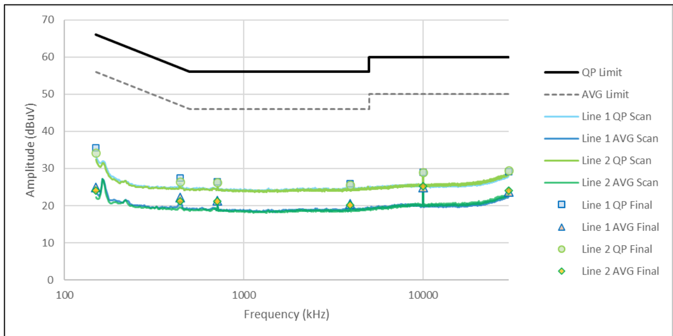
Figure CE01.1: Spectral data (BLE 2 Mbps)
