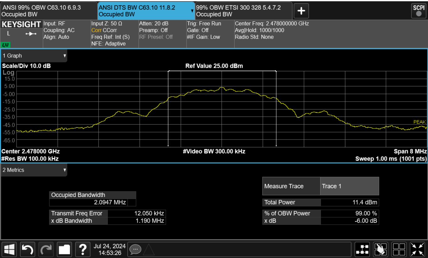
Figure TR06.3: Bandwidth data for BLE 2 at high channel (2478 MHz)
