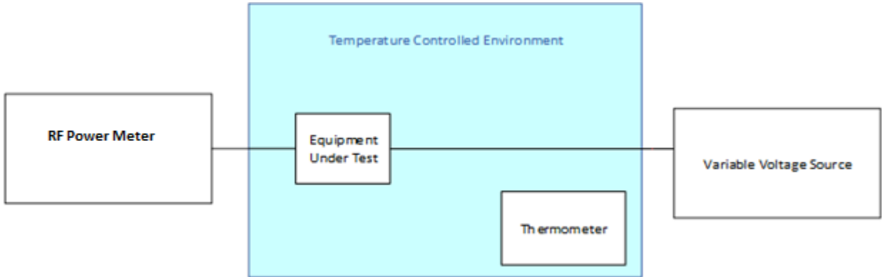
Figure TR02.2: Transmit Power over temperature test equipment setup
