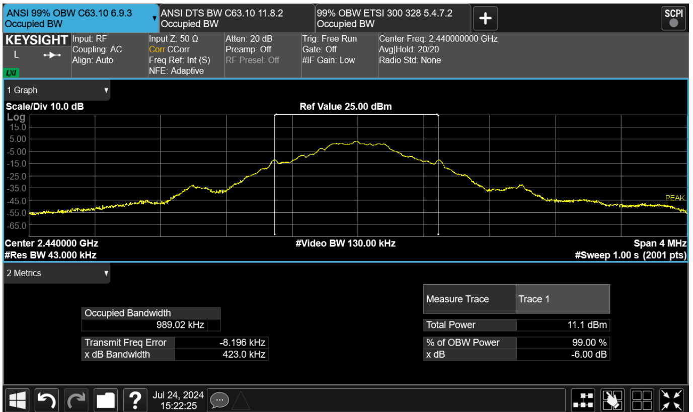
Figure TR10.4: Occupied bandwidth data for ANT at mid channel (2440 MHz)
