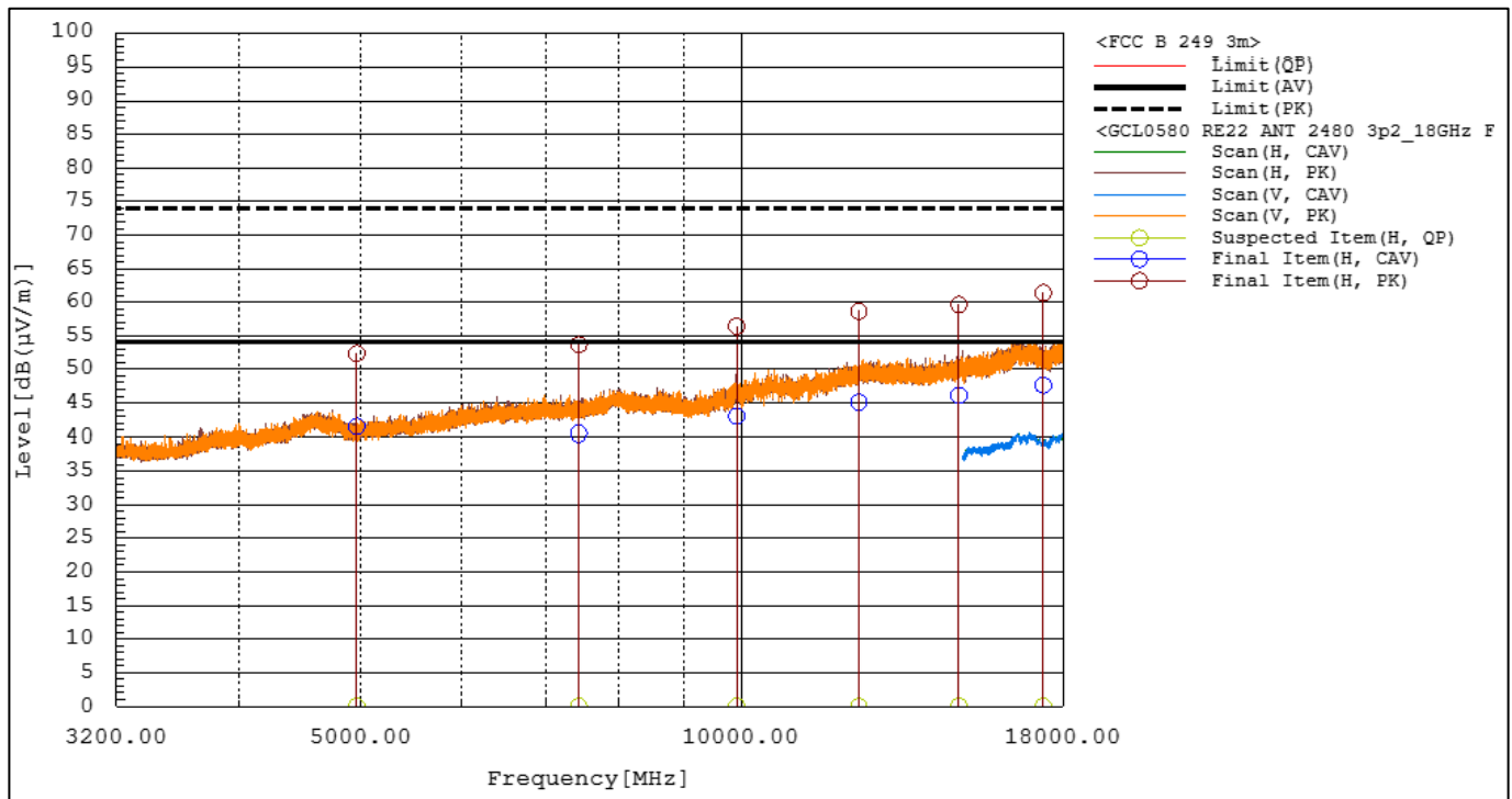
Figure RE22.3: Spectral data (ANT 2480MHz, X orientation)
