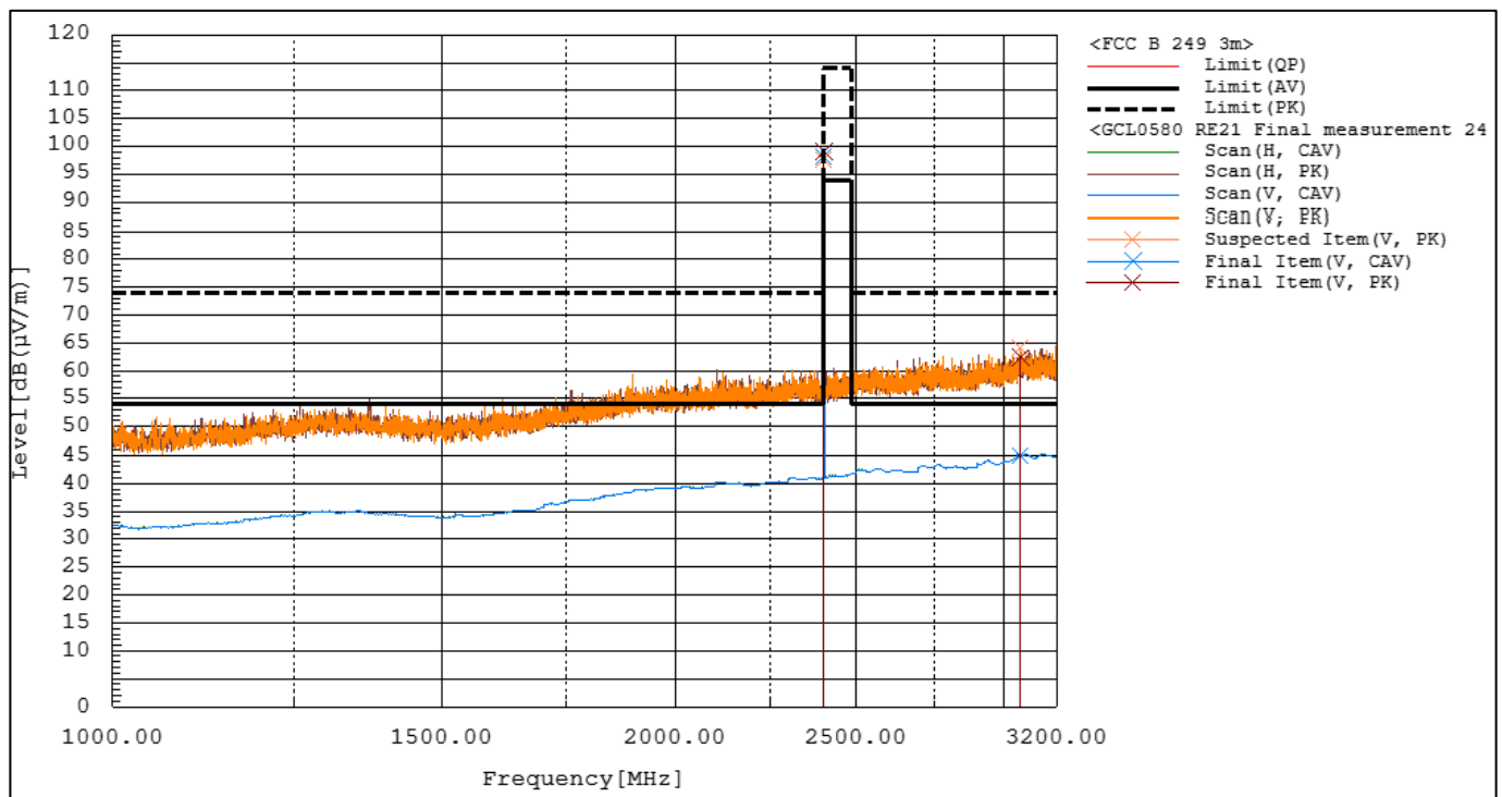
Figure RE21.1: Spectral data ((ANT, 2402MHz X orientation)
