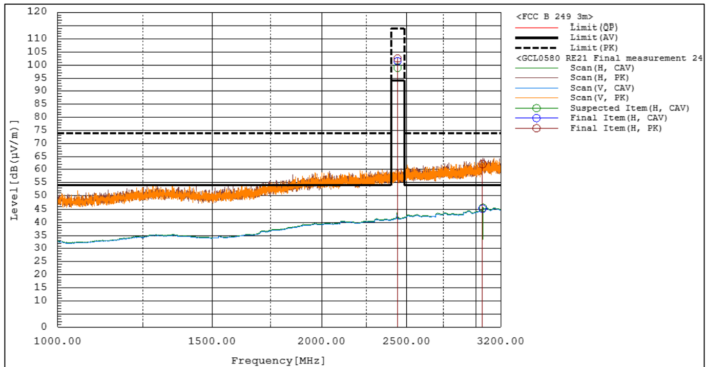
Figure RE21.2: Spectral data (ANT, 2440MHz X orientation)
