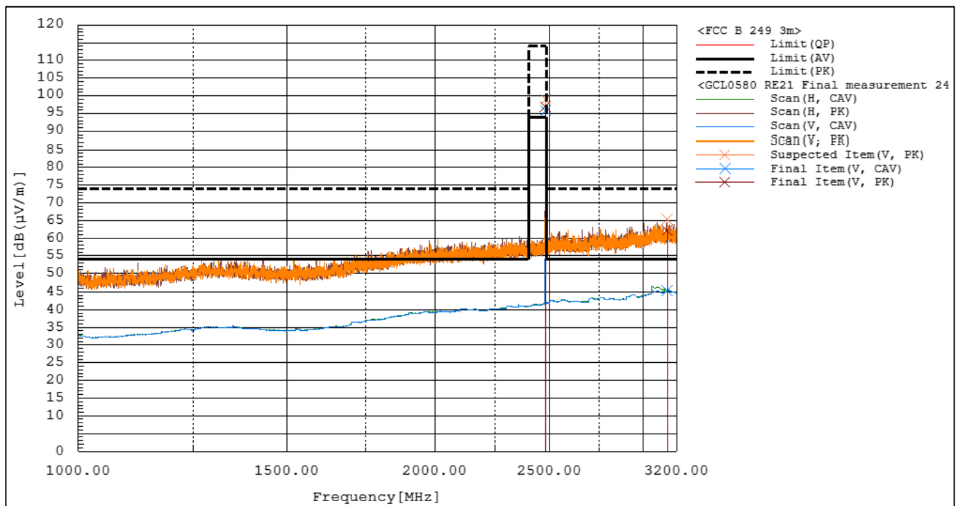
Figure RE21.3: Spectral data (ANT, 2480MHz X orientation)
