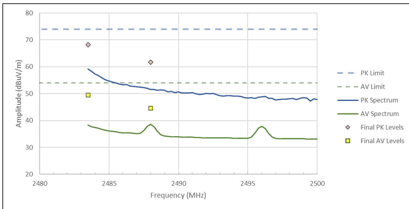
Figure RE04.2: FCC restricted band spectral data from 2483.5 to 2500 MHz
