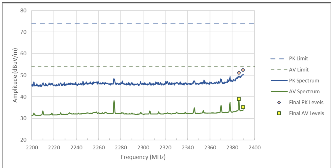
Figure RE04.1: FCC restricted band spectral data from 2200 to 2390 MHz
