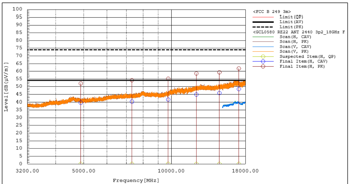
Figure RE22.2: Spectral data (ANT 2440MHz, X orientation)
