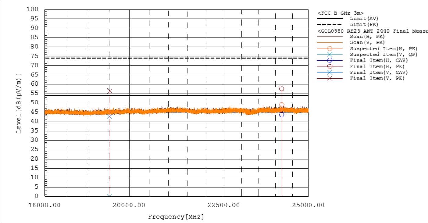
Figure RE23.1: Spectral data graph
