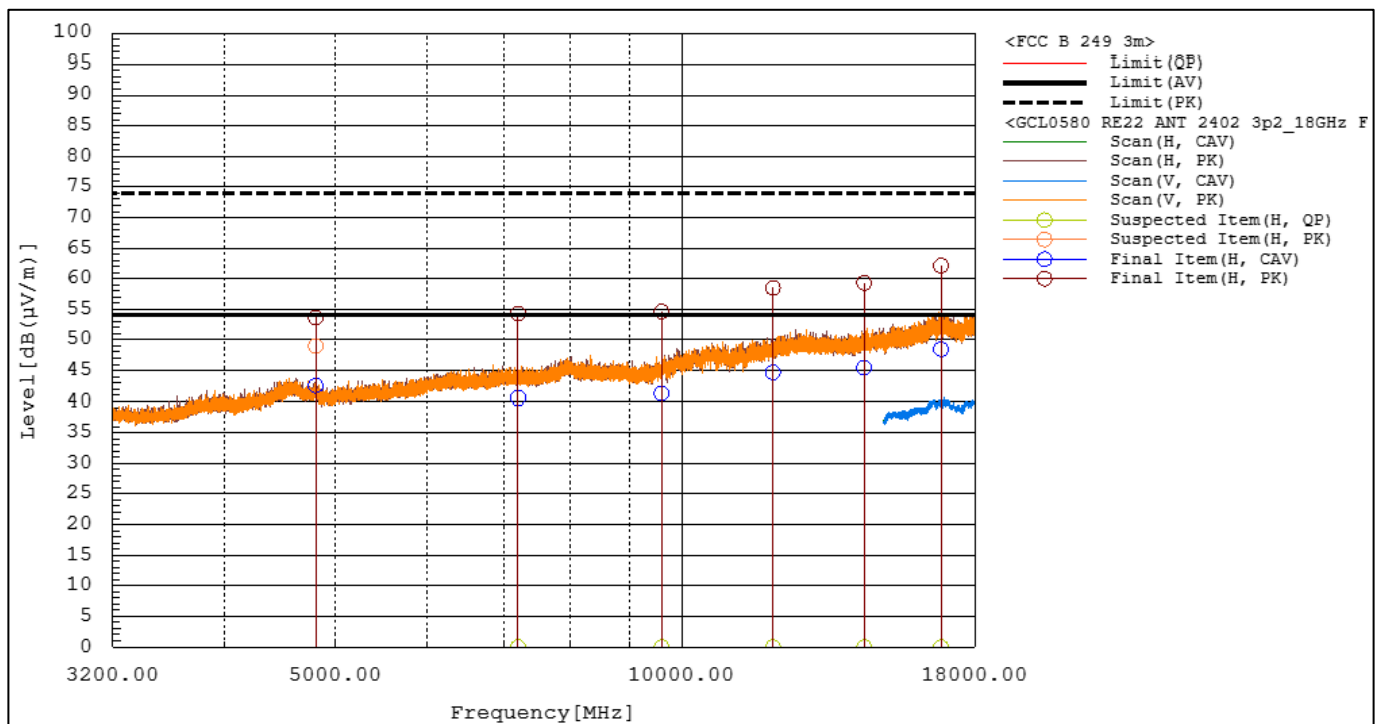
Figure RE22.1: Spectral data (ANT 2402MHz, X orientation)
