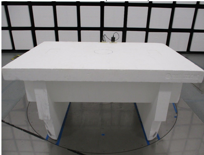
RADIATED EMISSIONS SETUP (30-1000MHz)
