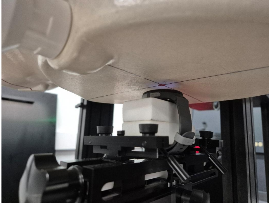
Figure 1 SAR Test Setup – Head – Front 10mm
