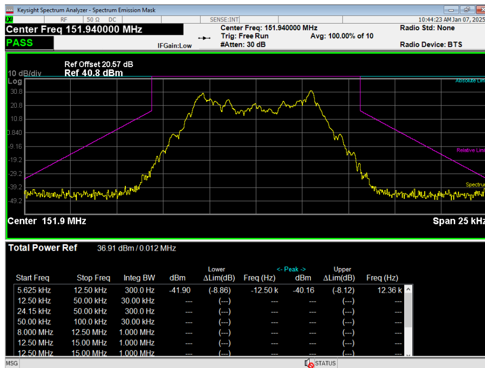
Figure 19 - Emissions Mask, Ch3, 95.2779(b)(1)
