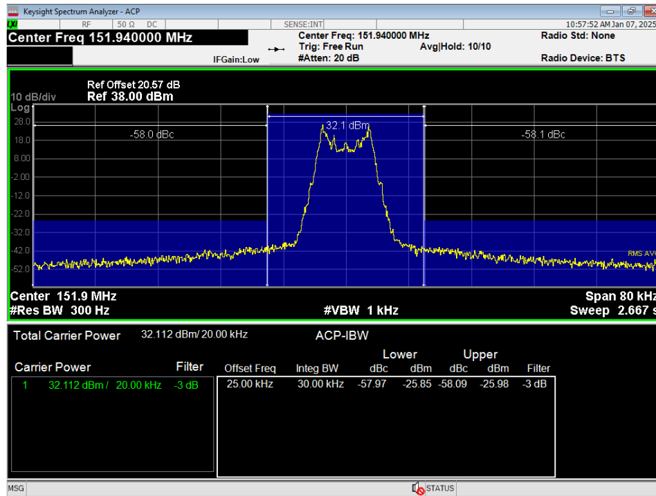
Figure 20 - Emissions Mask, Ch3, 95.2779(b)(2)
