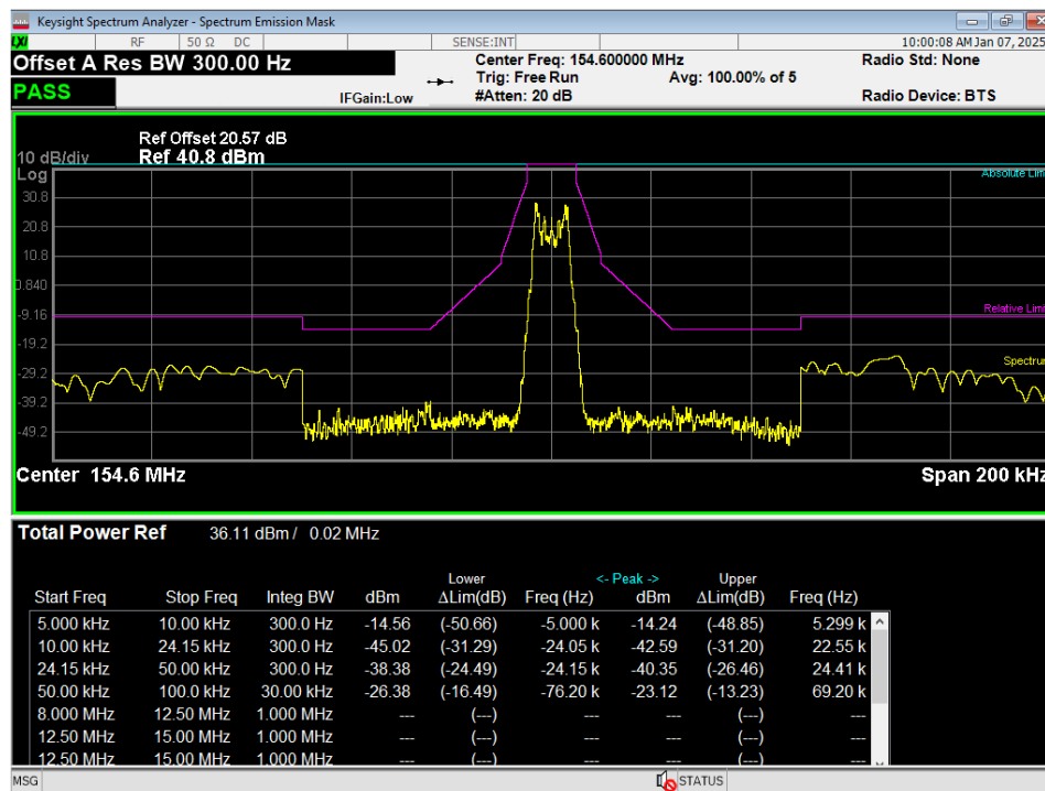
Figure 21 - Emissions Mask, Ch5, 95.2779(b)(5,6,7)
