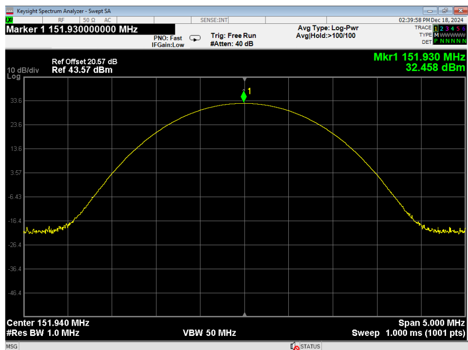
Figure 12 –Output Power, 151.940 MHz
