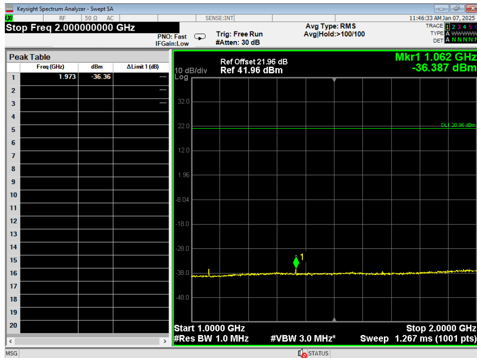
Figure 6 - Conducted Spurious emissions, VHF, Ch1, 1GHz – 2GHz
