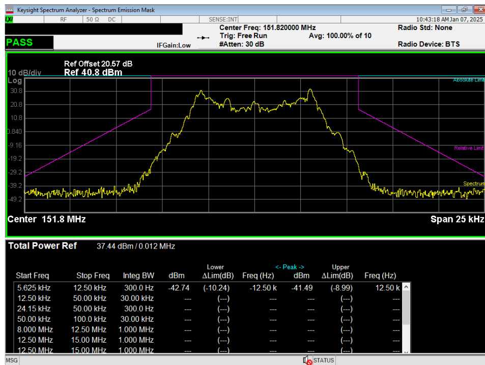
Figure 17 - Emissions Mask, Ch1, 95.2779(b)(1)
