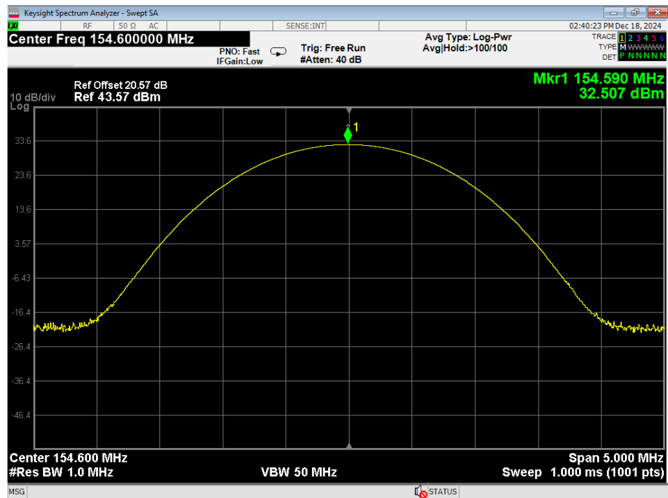
Figure 13 –Output Power, 154.600 MHz
