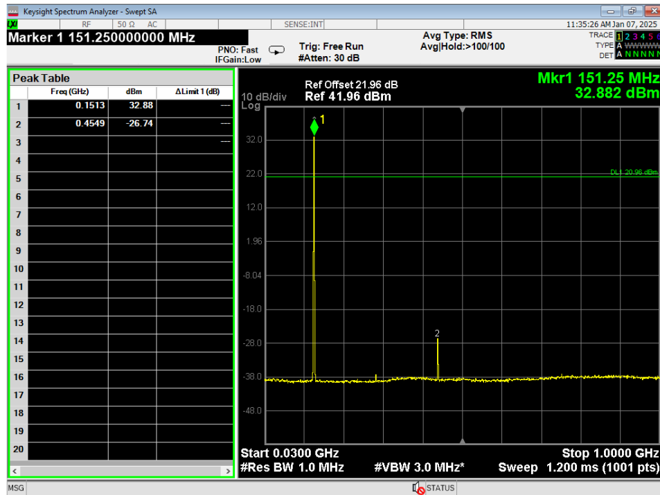
Figure 5 - Conducted Spurious emissions, VHF, Ch1, 30MHz – 1GHz
