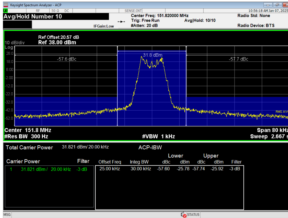
Figure 18 - Emissions Mask, Ch1, 95.2779(b)(2)
