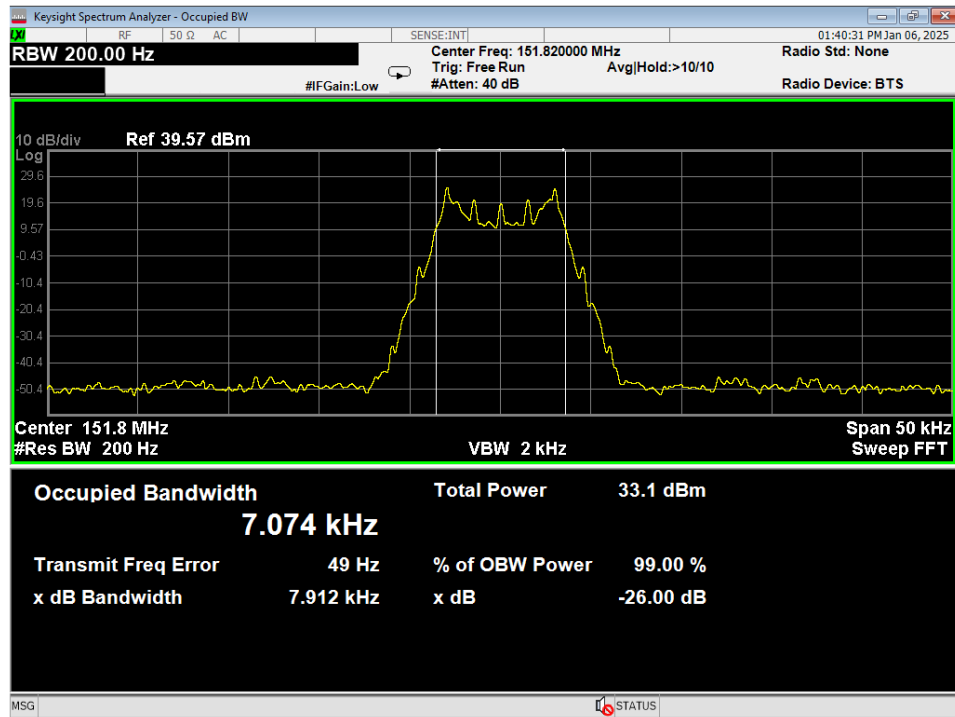
Figure 14 - Bandwidth, 151.820 MHz
