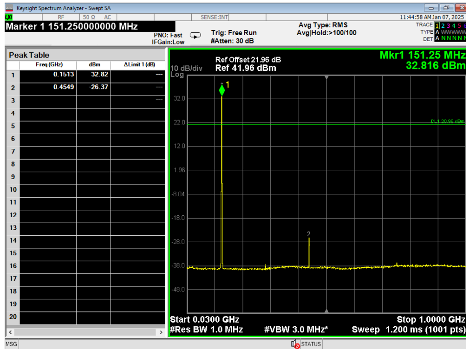
Figure 7 - Conducted Spurious emissions, VHF, Ch3, 30MHz – 1GHz
