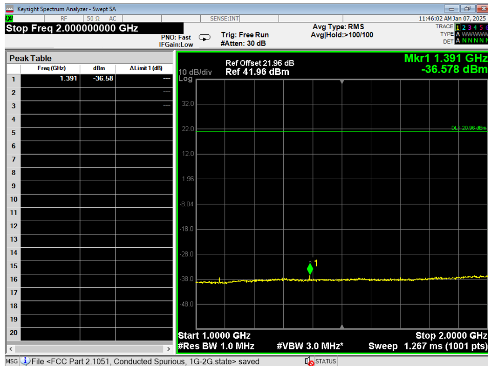
Figure 10 - Conducted Spurious emissions, VHF, Ch5, 1GHz – 2GHz
