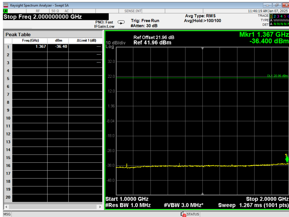
Figure 8 - Conducted Spurious emissions, VHF, Ch3, 1GHz – 2GHz
