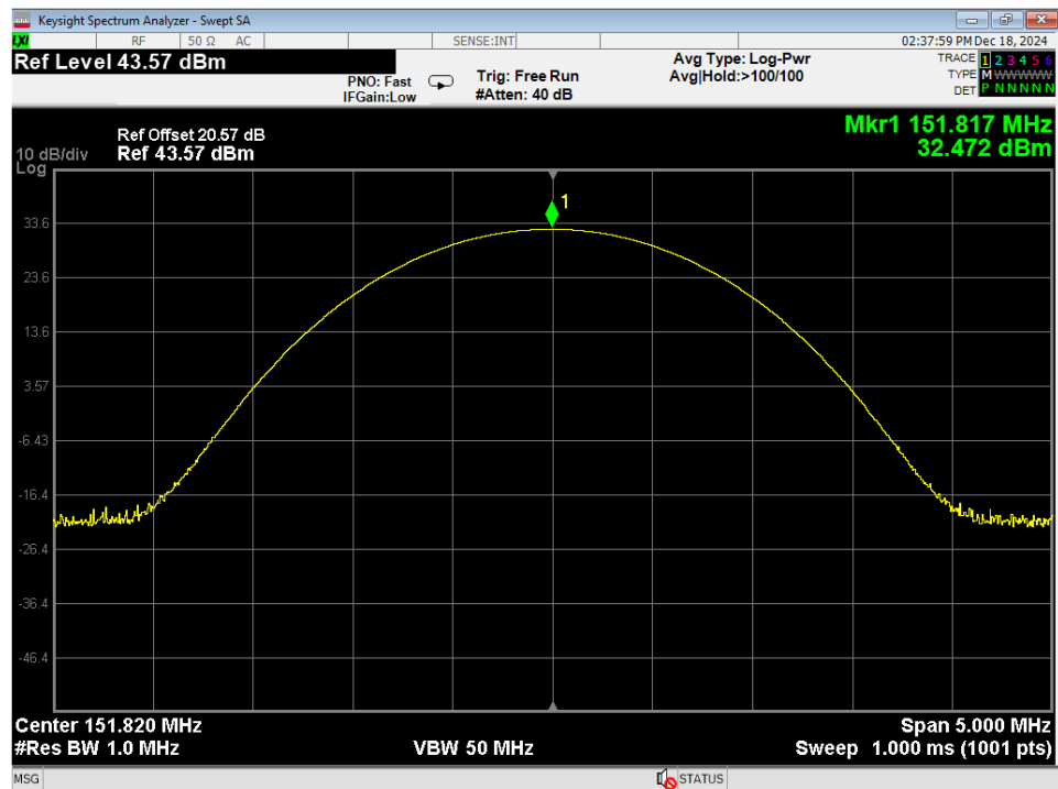
Figure 11 –Output Power, 151.820 MHz
