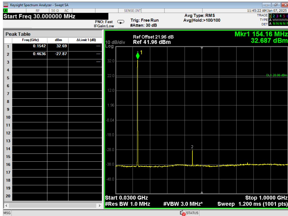
Figure 9 - Conducted Spurious emissions, VHF, Ch5, 30MHz – 1GHz
