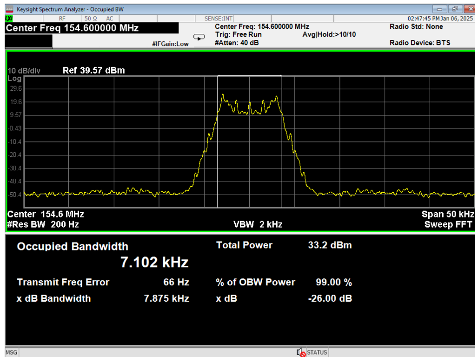
Figure 16 - Bandwidth, 154.600 MHz
