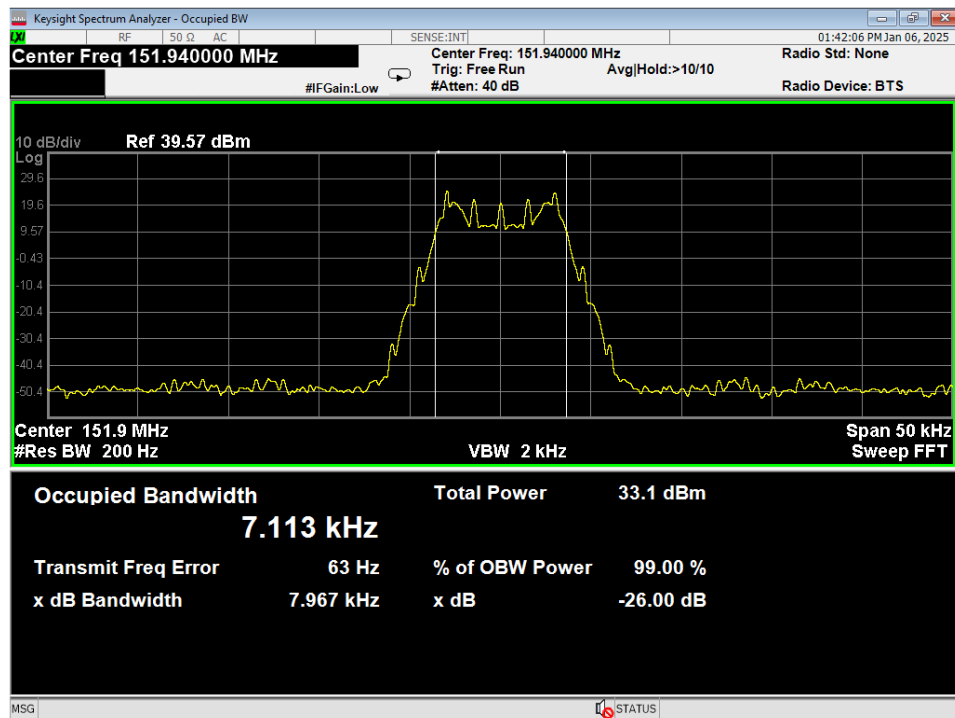
Figure 15 - Bandwidth, 151.940 MHz
