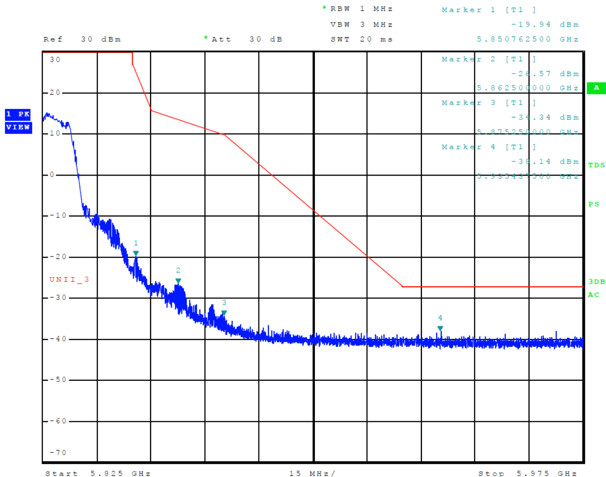
Figure 25 Plot of Upper Band Edge Across 5725-5850 MHz Mode 13 U-NII-3 (802.11a)
