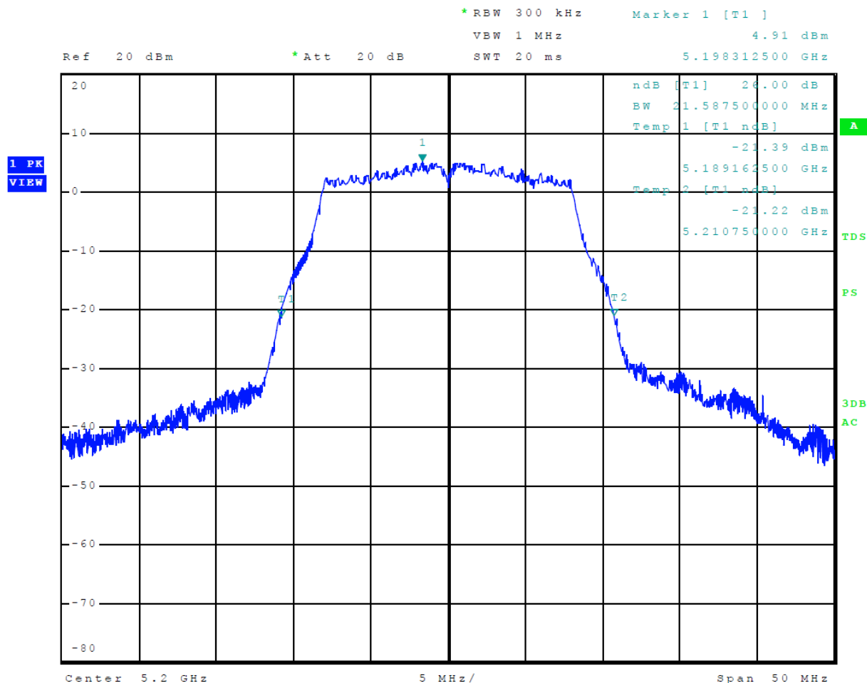
Figure 29 Plot of 26-dB Occupied Bandwidth 5150-5250 MHz Mode 9 U-NII-1 (802.11a)
