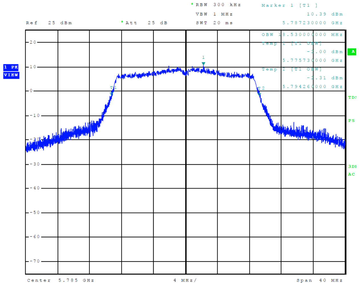
Figure 42 Plot of 99% Occupied Bandwidth 5725-5850 MHz Mode 14 U-NII-3 (802.11n)
