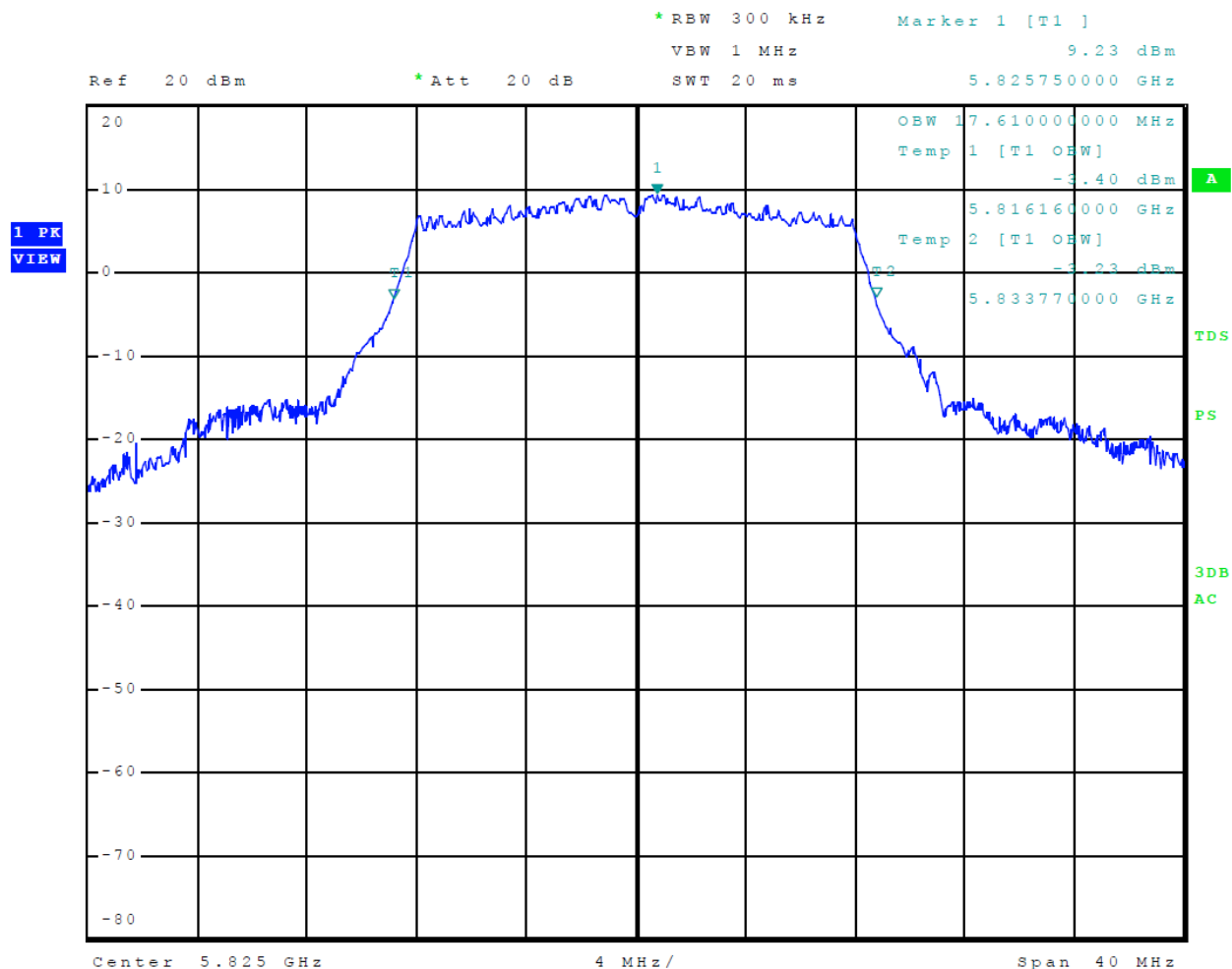
Figure 41 Plot of 99% Occupied Bandwidth 5725-5850 MHz Mode 13 U-NII-3 (802.11a)
