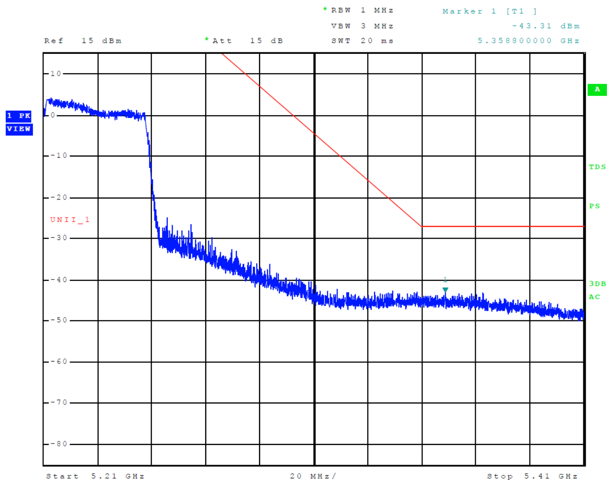
Figure 24 Plot of Upper Band Edge Across 5150-5250 MHz Mode 12 U-NII-1 (802.11ac80)
