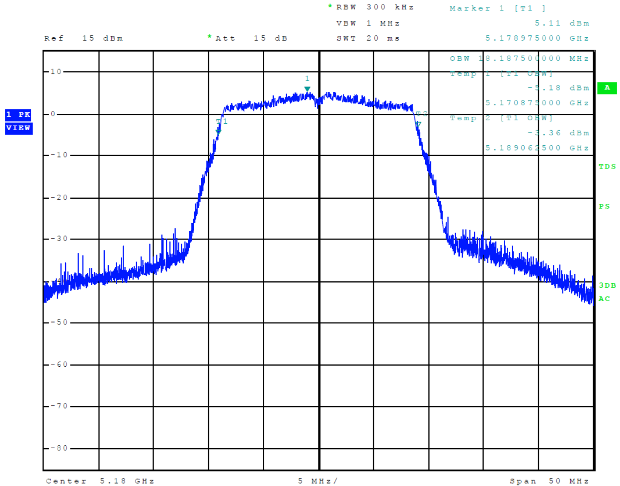
Figure 38 Plot of 99% Occupied Bandwidth 5150-5250 MHz Mode 10 U-NII-1 (802.11n)
