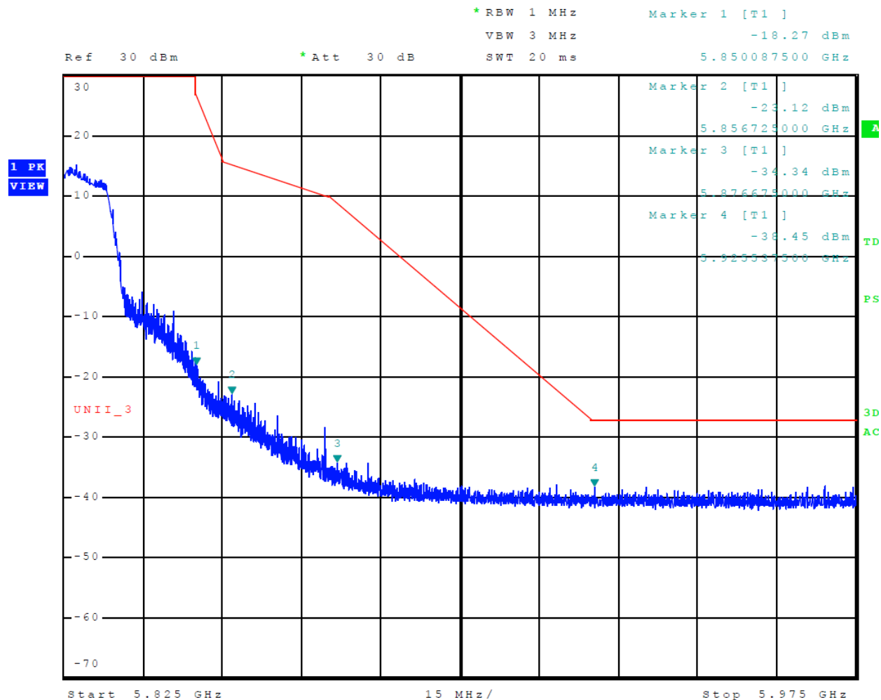
Figure 26 Plot of Upper Band Edge Across 5725-5850 MHz Mode 14 U-NII-3 (802.11n)
