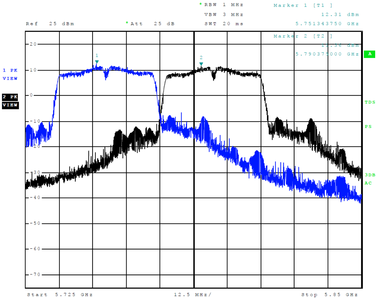
Figure 11 Plot of Transmitter Emissions Across 5725-5850 MHz Mode 15 U-NII-3 (802.11n40)
