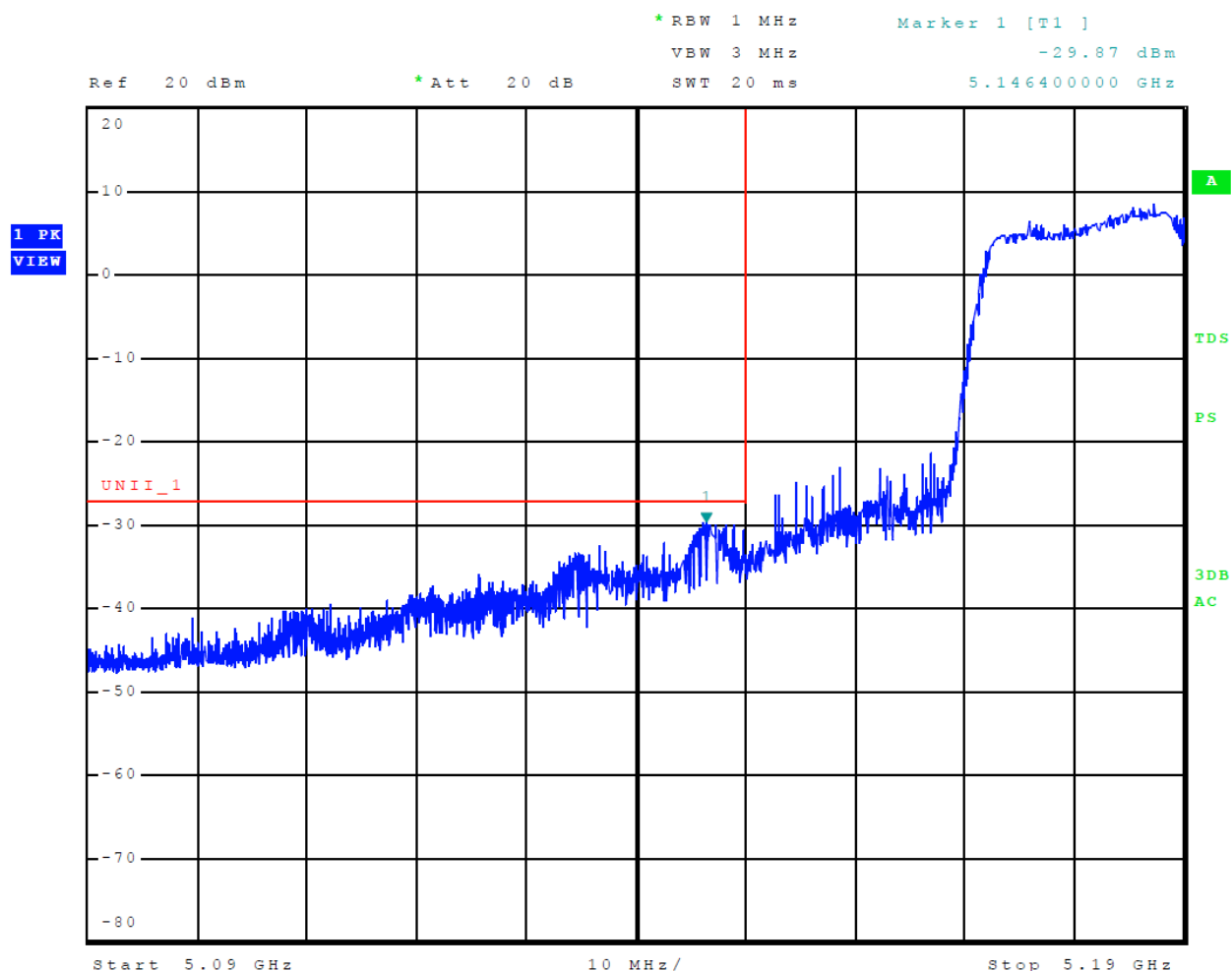
Figure 15 Plot of Lower Band Edge Across 5150-5250 MHz Mode 11 U-NII-1 (802.11n40)
