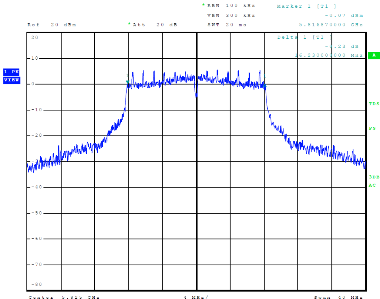
Figure 45 Plot of 6-dB Occupied Bandwidth 5725-5850 MHz Mode 13 U-NII-3 (802.11a)
