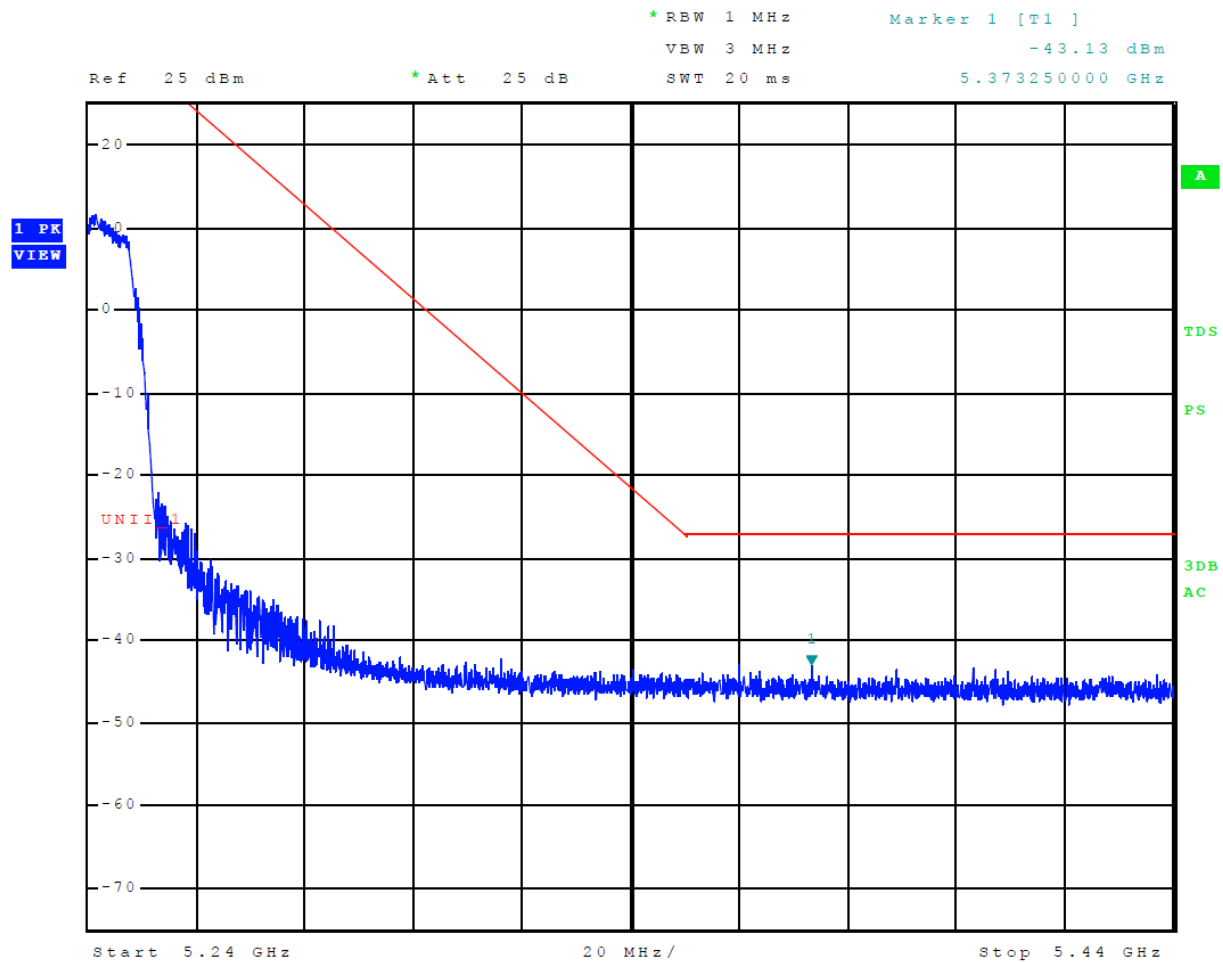
Figure 21 Plot of Upper Band Edge Across 5150-5250 MHz Mode 9 U-NII-1 (802.11a)
