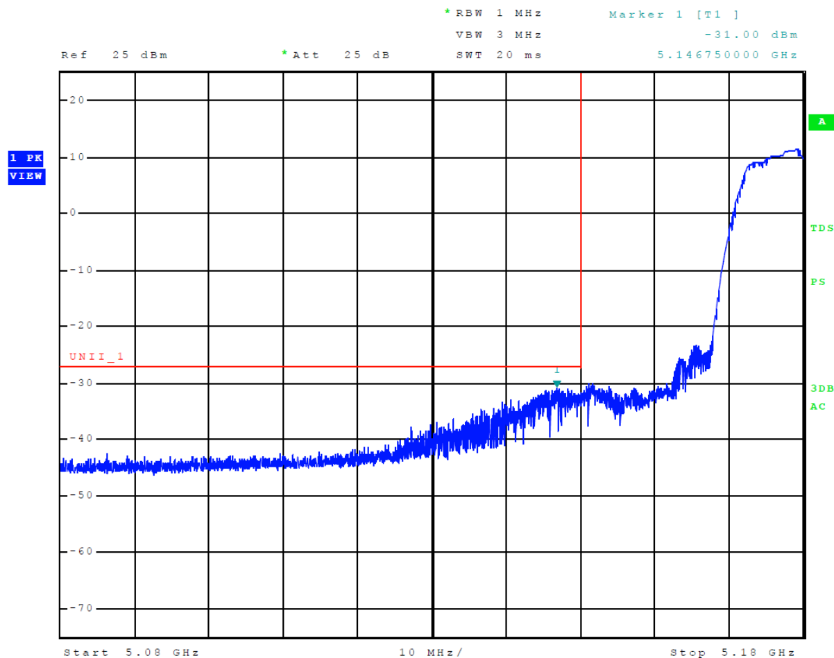
Figure 13 Plot of Lower Band Edge Across 5150-5250 MHz Mode 9 U-NII-1 (802.11a)
