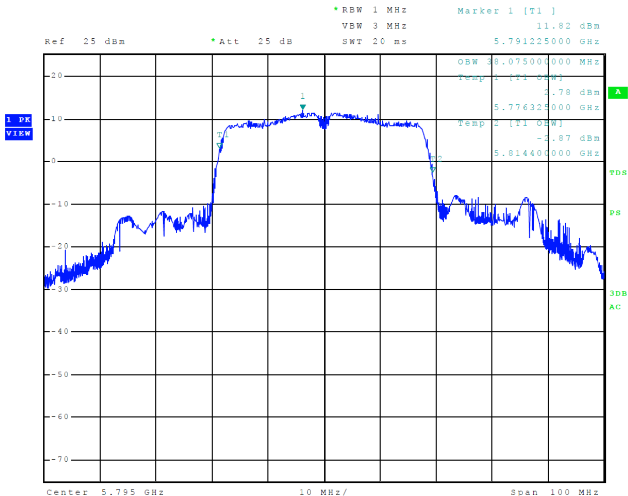
Figure 43 Plot of 99% Occupied Bandwidth 5725-5850 MHz Data Mode 15 U-NII-3 (802.11n40)
