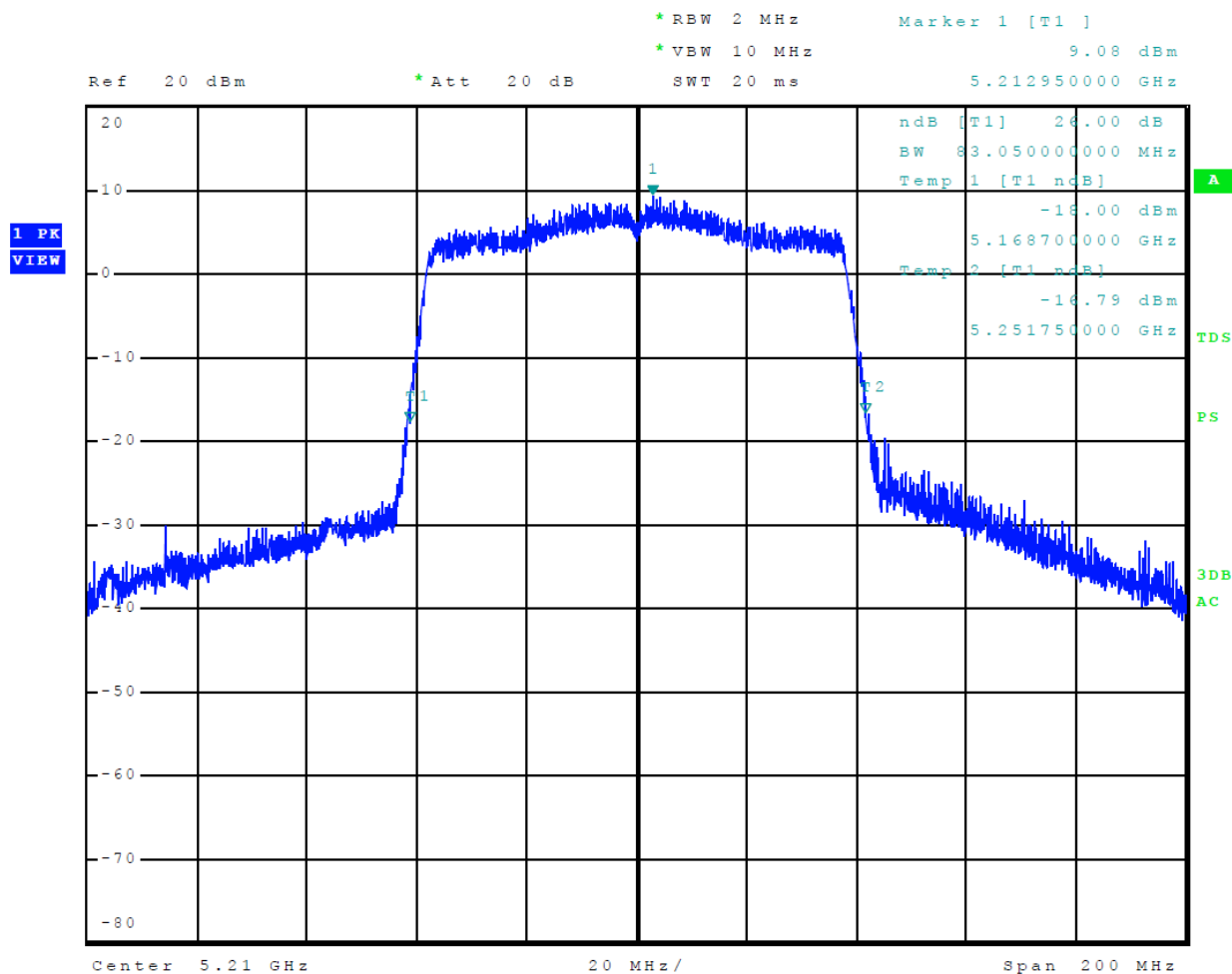
Figure 32 Plot of 26-dB Occupied Bandwidth 5150-5250 MHz Mode 12 U-NII-1 (802.11ac80)
