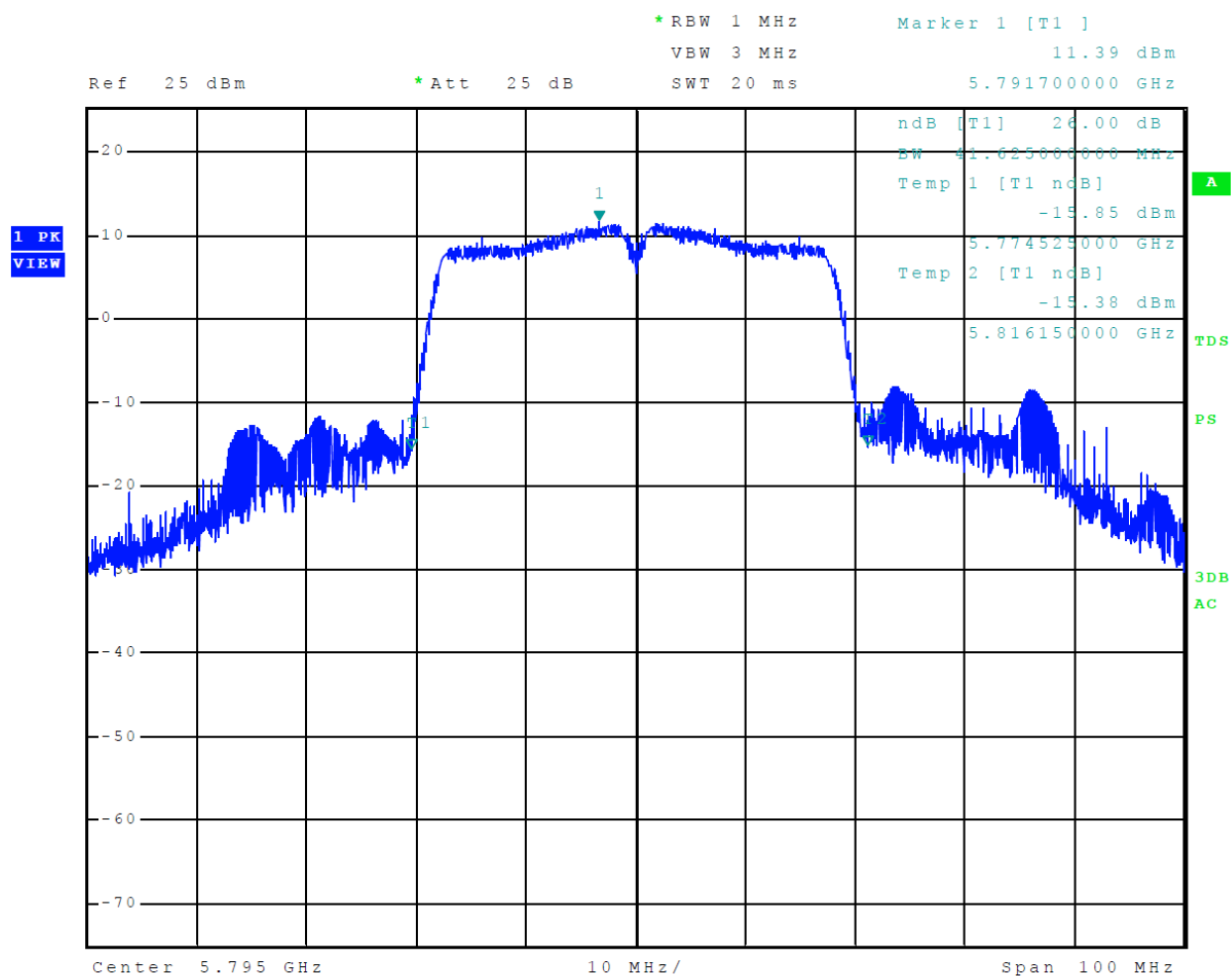
Figure 35 Plot of 26-dB Occupied Bandwidth 5725-5850 MHz Data Mode 15 U-NII-3 (802.11n40)
