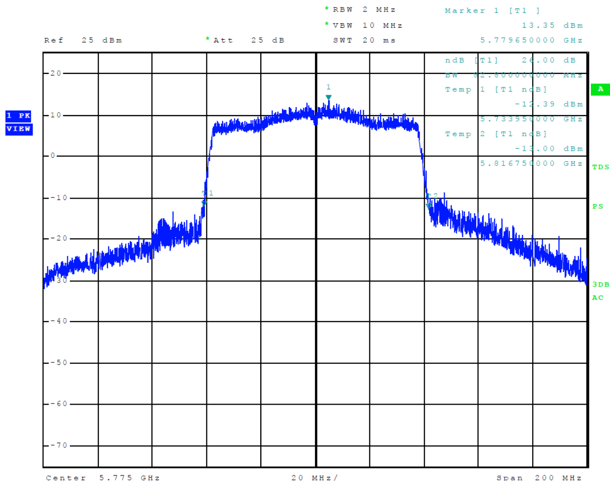
Figure 36 Plot of 26-dB Occupied Bandwidth 5725-5850 MHz Mode 16 U-NII-3 (802.11ac80)
