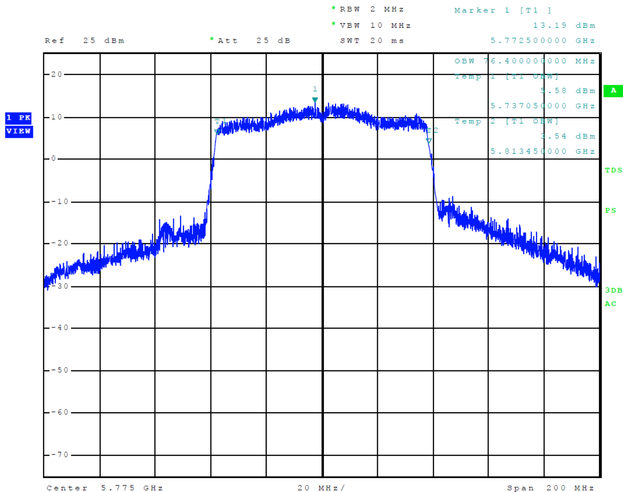
Figure 44 Plot of 99% Occupied Bandwidth 5725-5850 MHz Mode 16 U-NII-3 (802.11ac80)
