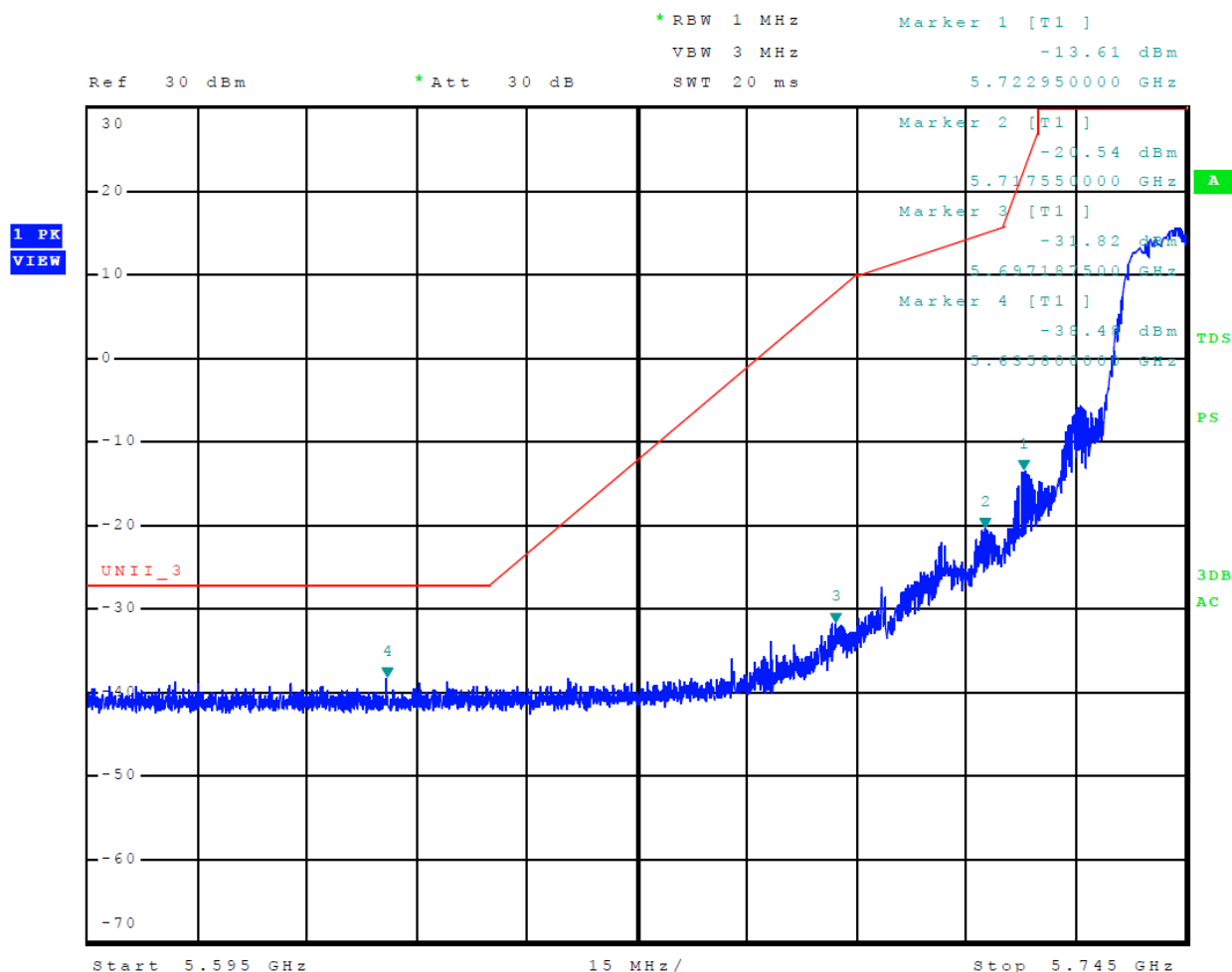
Figure 17 Plot of Lower Band Edge Across 5725-5850 MHz Mode 13 U-NII-3 (802.11a)
