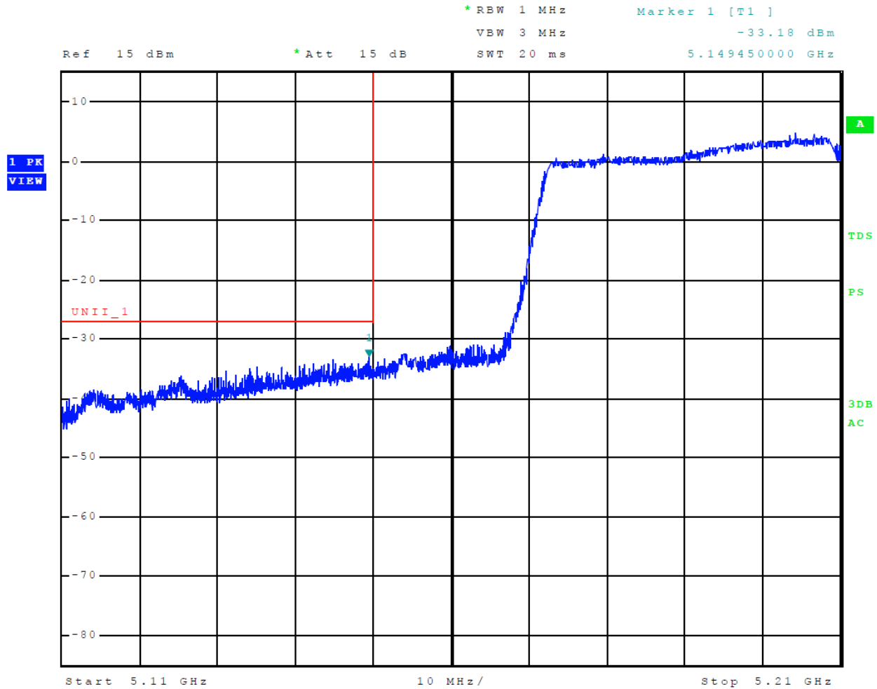
Figure 16 Plot of Lower Band Edge Across 5150-5250 MHz Mode 12 U-NII-1 (802.11ac80)
