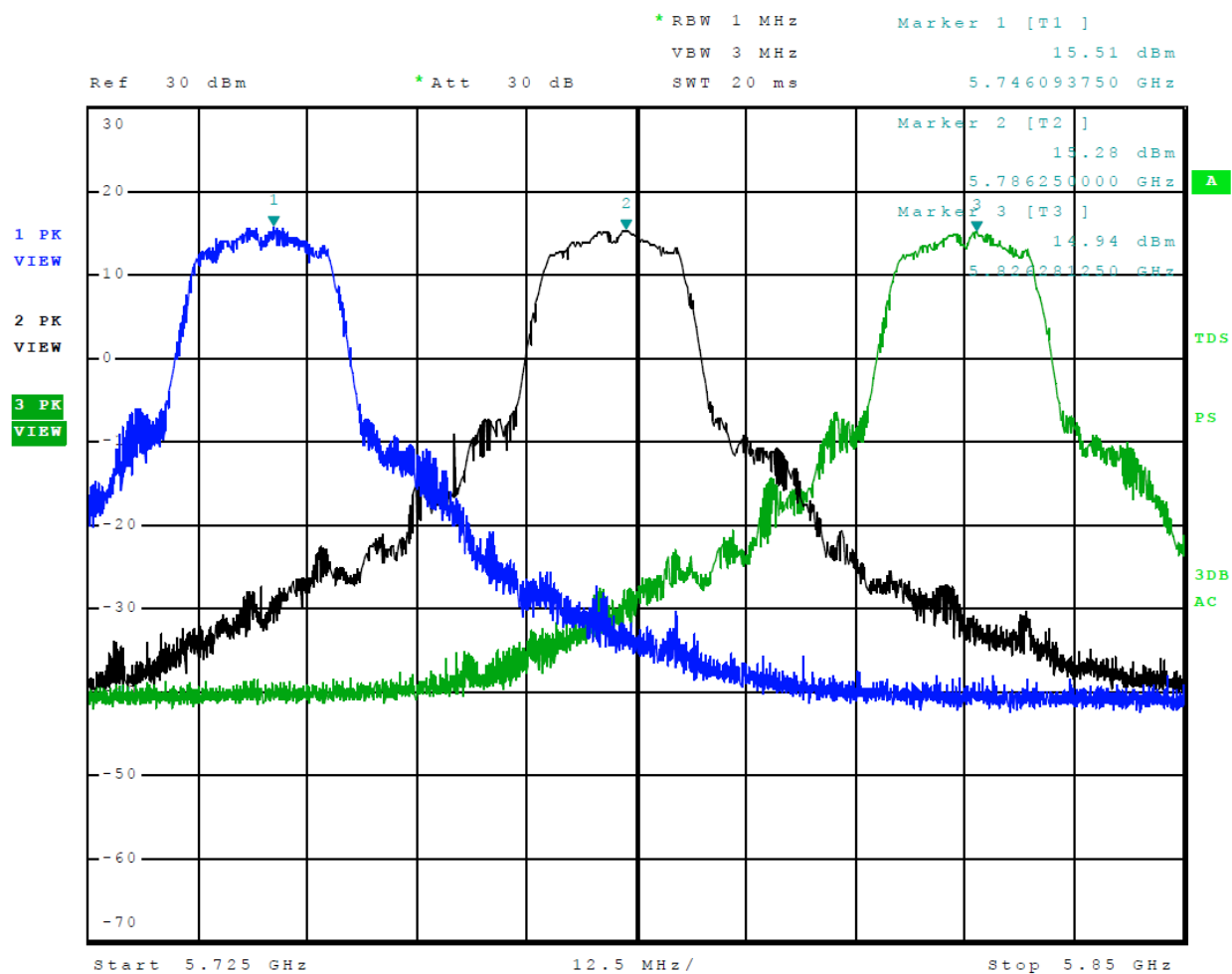
Figure 9 Plot of Transmitter Emissions Across 5725-5850 MHz Mode 13 U-NII-3 (802.11a)
