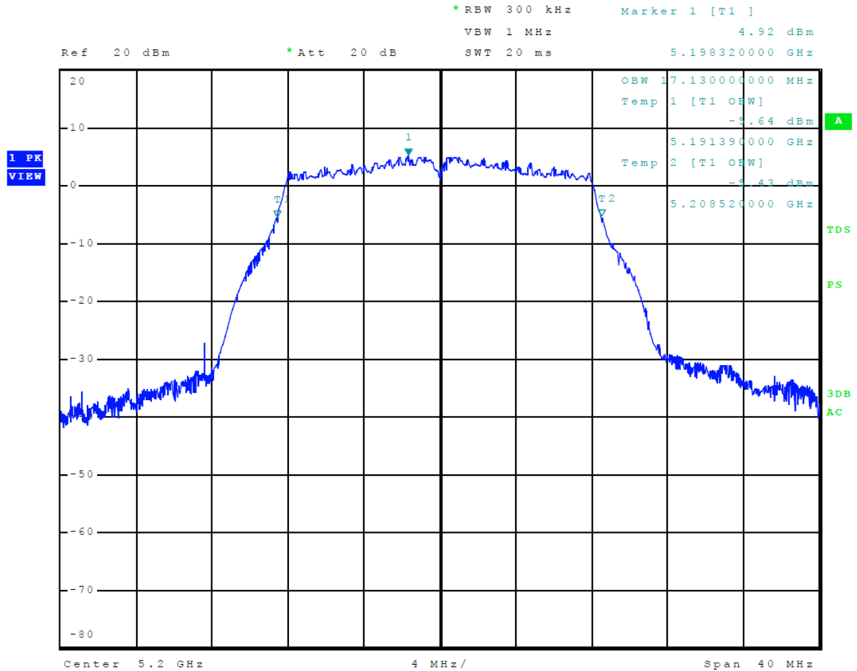
Figure 37 Plot of 99% Occupied Bandwidth 5150-5250 MHz Mode 9 U-NII-1 (802.11a)
