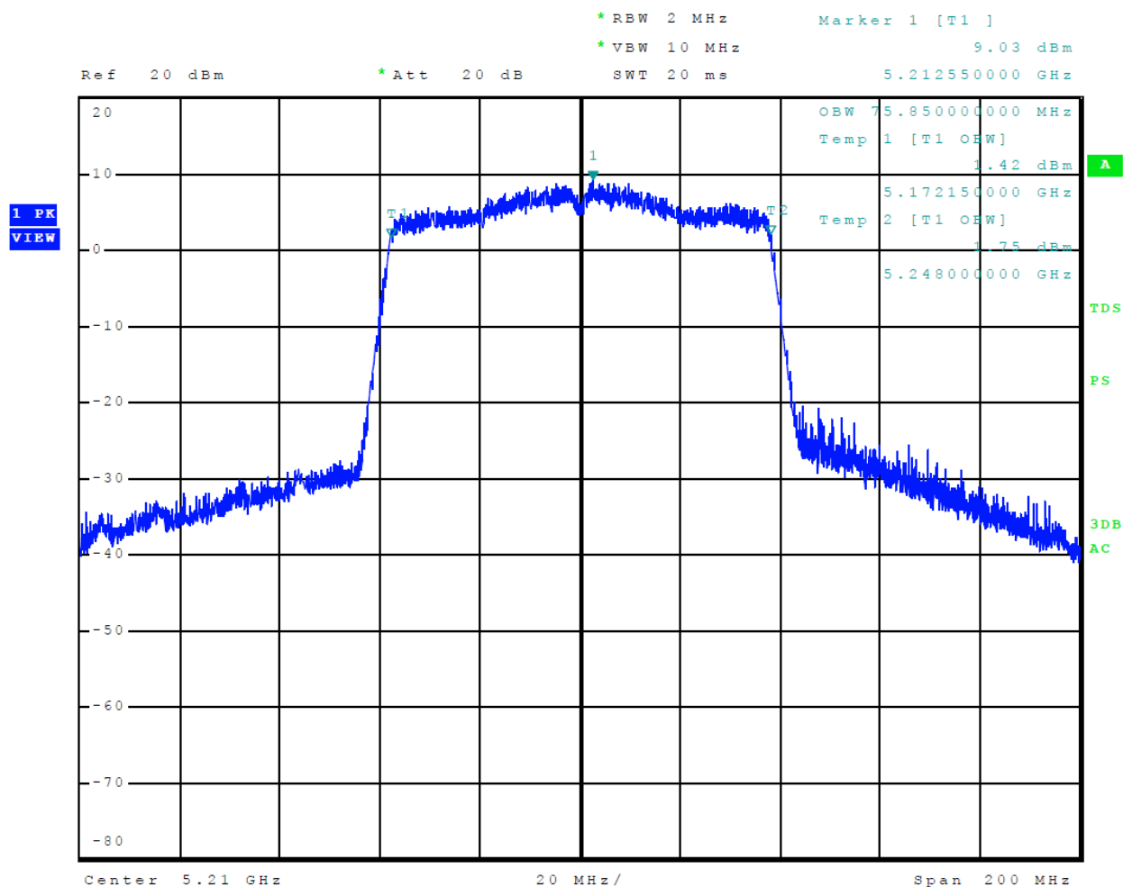
Figure 40 Plot of 99% Occupied Bandwidth 5150-5250 MHz Mode 12 U-NII-1 (802.11ac80)
