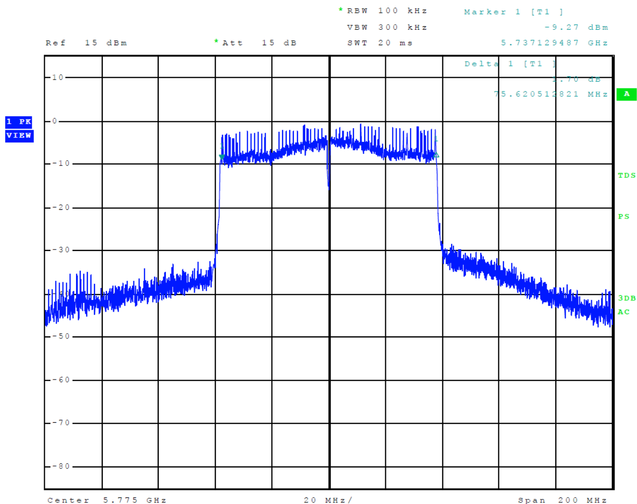
Figure 48 Plot of 6-dB Occupied Bandwidth 5725-5850 MHz Mode 16 U-NII-3 (802.11ac80)
