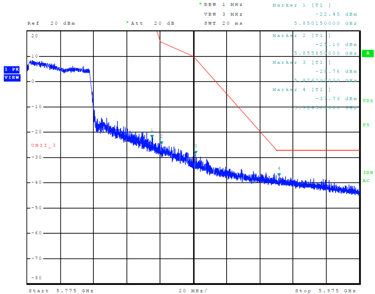
Figure 28 Plot of Upper Band Edge Across 5725-5850 MHz Mode 16 U-NII-3 (802.11ac80)
