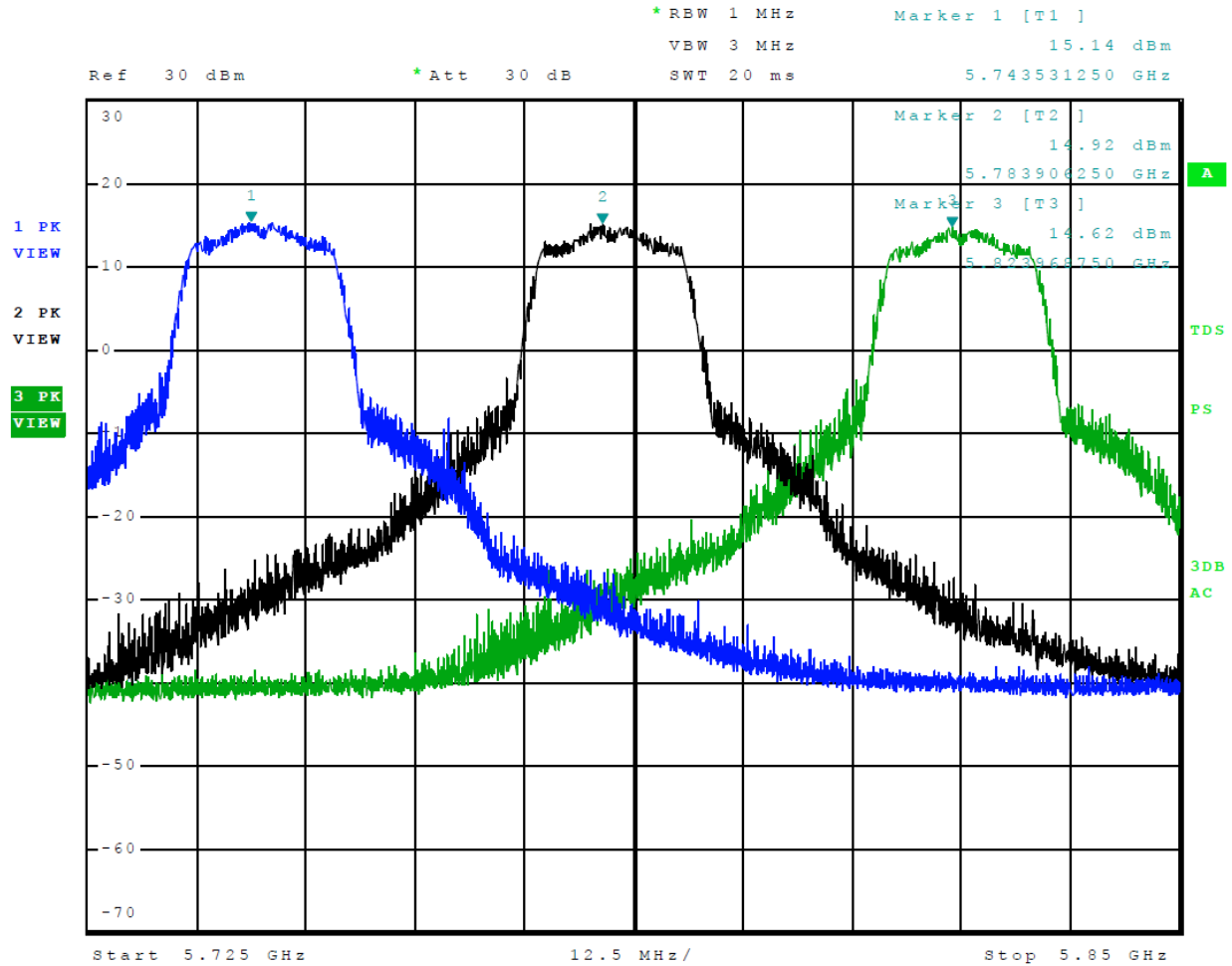
Figure 10 Plot of Transmitter Emissions Across 5725-5850 MHz Mode 14 U-NII-3 (802.11n)
