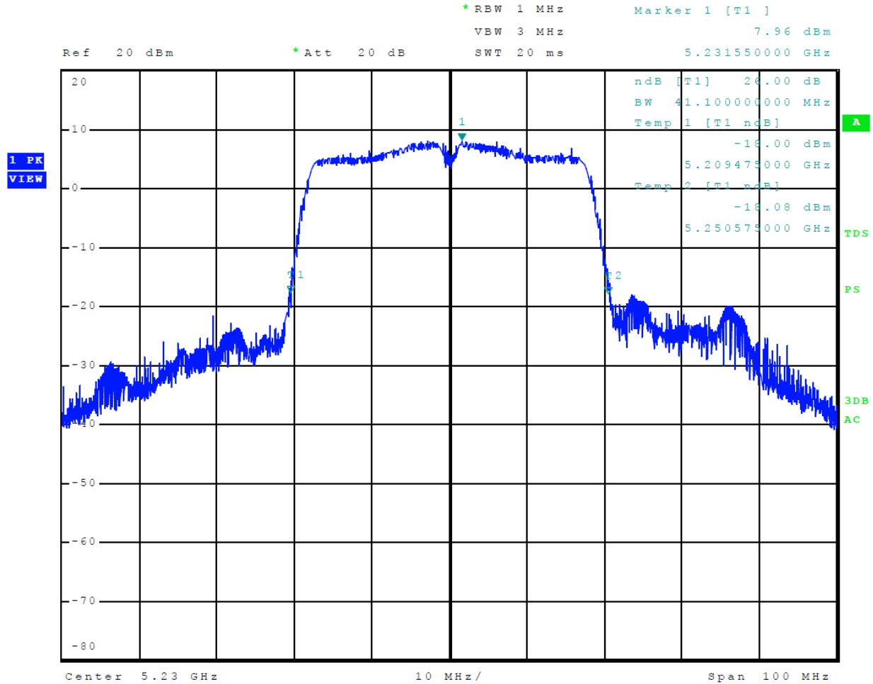
Figure 31 Plot of 26-dB Occupied Bandwidth 5150-5250 MHz Mode 11 U-NII-1 (802.11n40)
