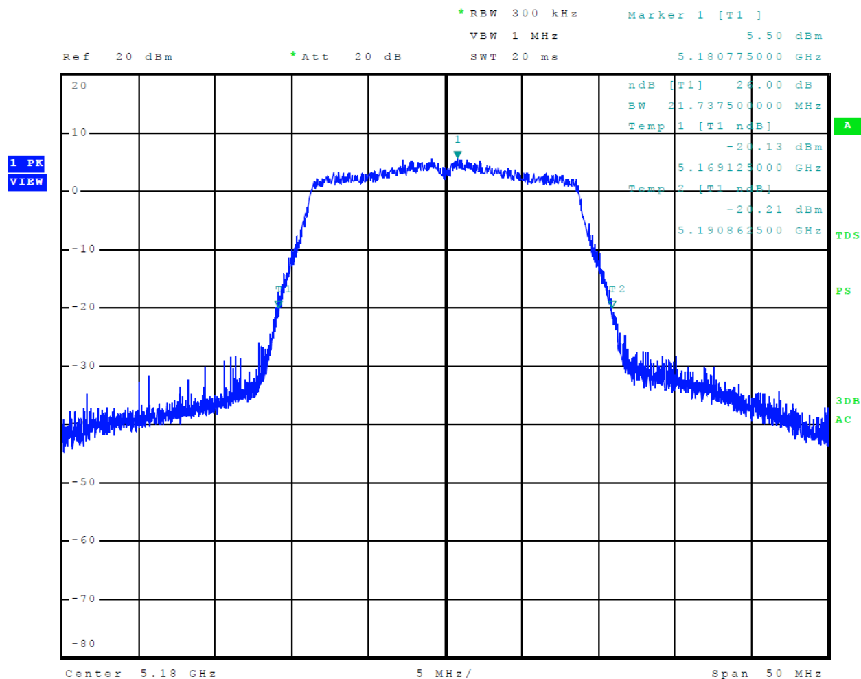
Figure 30 Plot of 26-dB Occupied Bandwidth 5150-5250 MHz Mode 10 U-NII-1 (802.11n)
