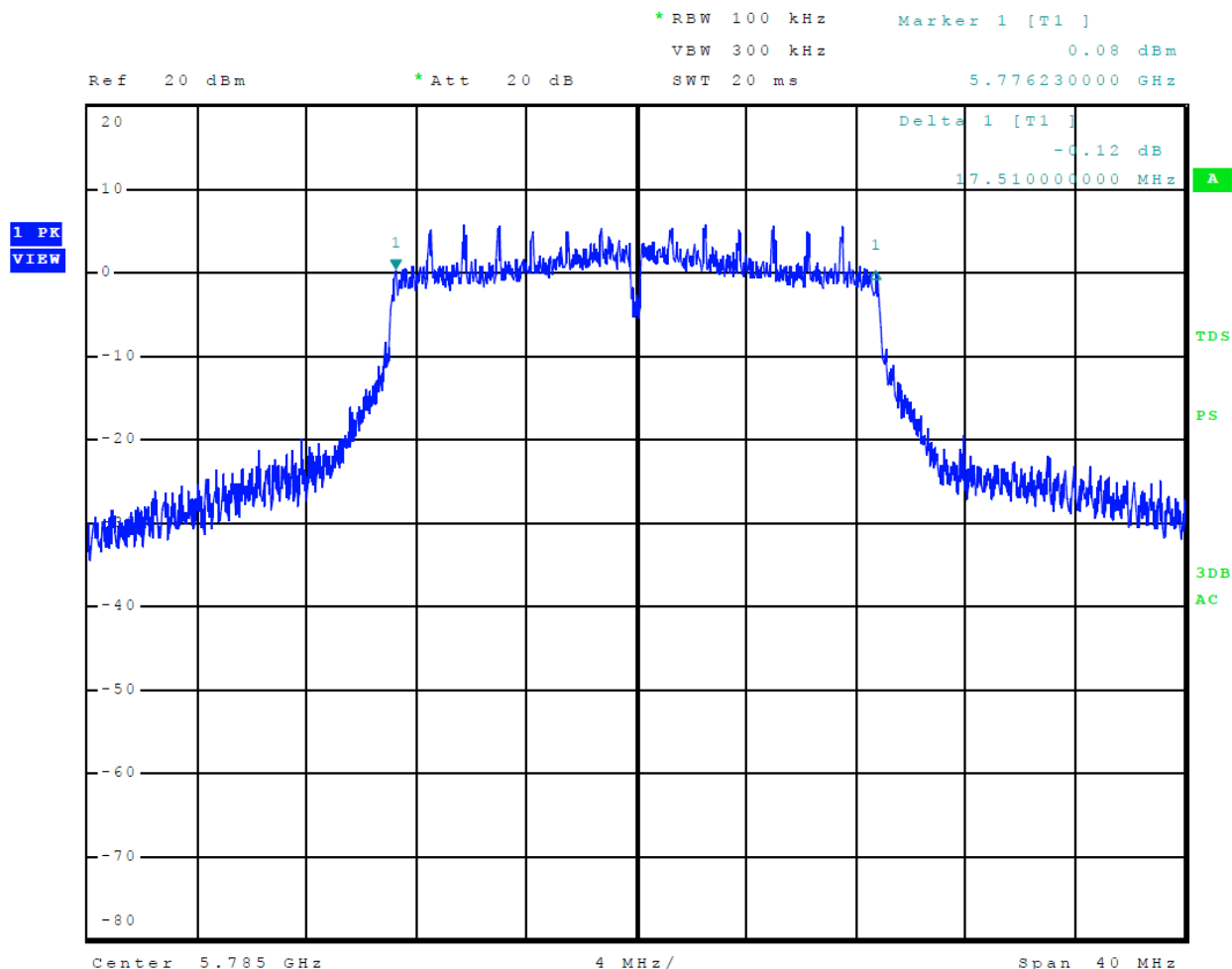
Figure 46 Plot of 6-dB Occupied Bandwidth 5725-5850 MHz Mode 14 U-NII-3 (802.11n)
