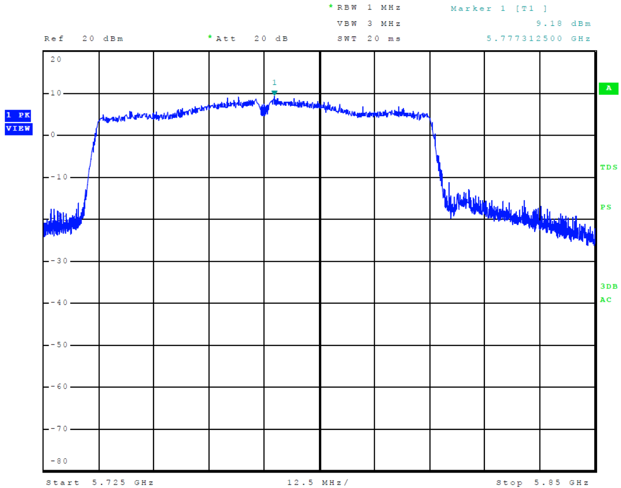
Figure 12 Plot of Transmitter Emissions Across 5725-5850 MHz Mode 16 U-NII-3 (802.11ac80)
