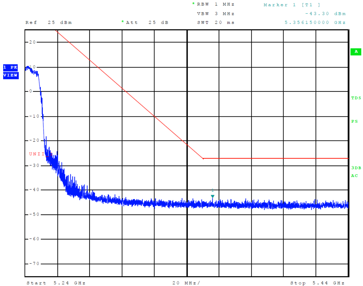
Figure 22 Plot of Upper Band Edge Across 5150-5250 MHz Mode 10 U-NII-1 (802.11n)
