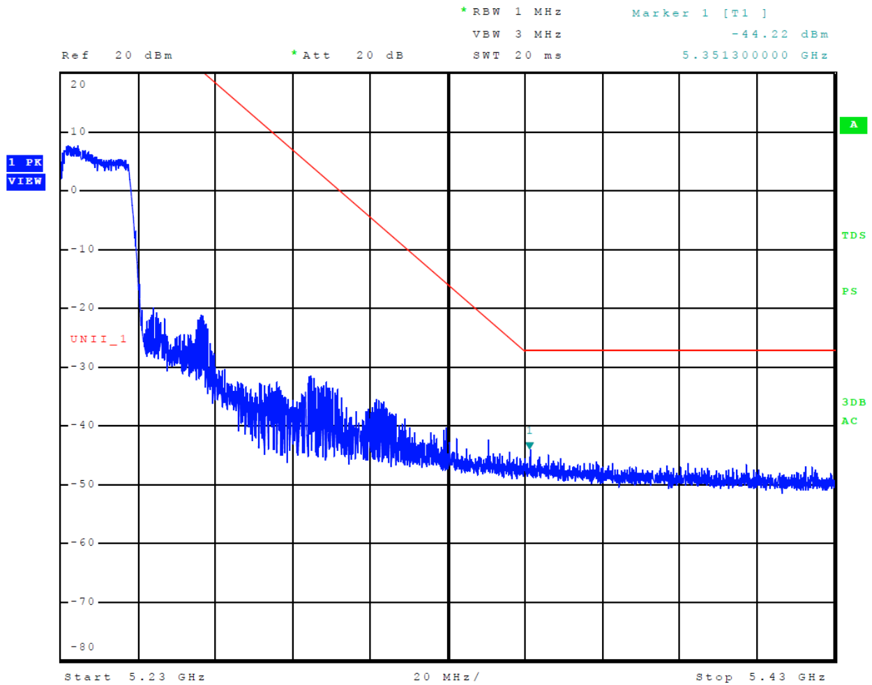
Figure 23 Plot of Upper Band Edge Across 5150-5250 MHz Mode 11 U-NII-1 (802.11n40)
