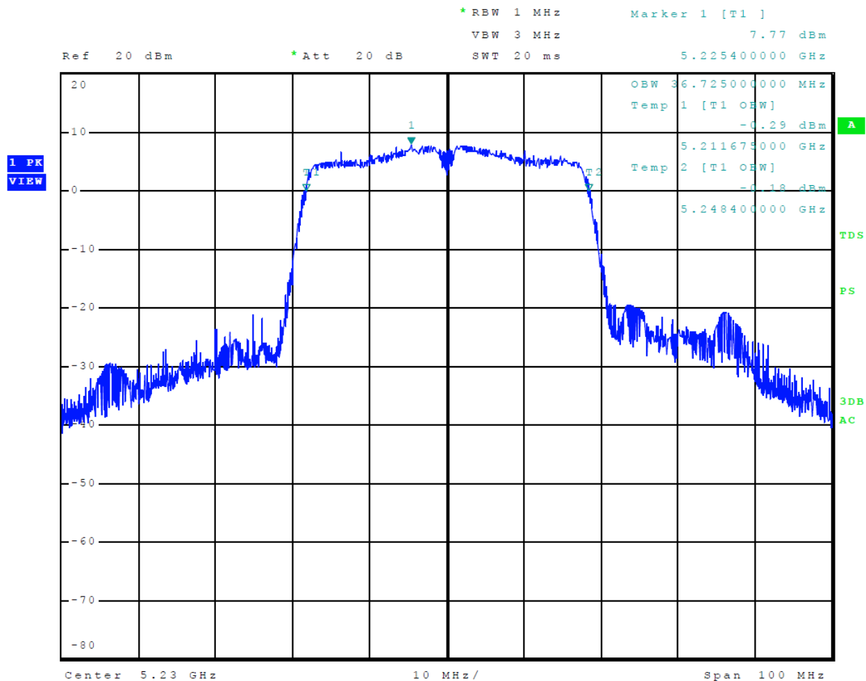
Figure 39 Plot of 99% Occupied Bandwidth 5150-5250 MHz Mode 11 U-NII-1 (802.11n40)
