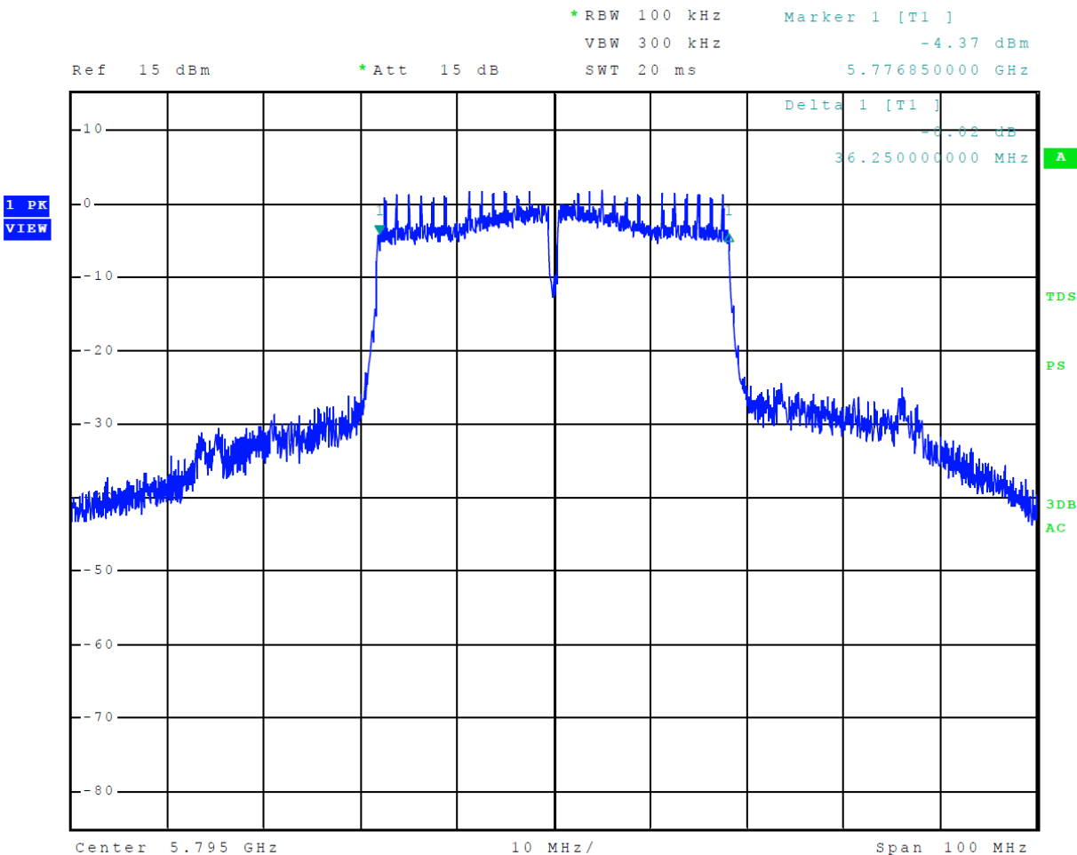
Figure 47 Plot of 6-dB Occupied Bandwidth 5725-5850 MHz Data Mode 15 U-NII-3 (802.11n40)
