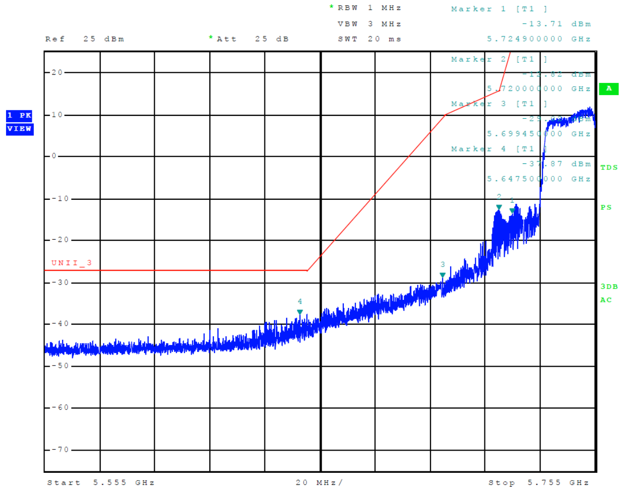
Figure 19 Plot of Lower Band Edge Across 5725-5850 MHz Data Mode 15 U-NII-3 (802.11n40)
