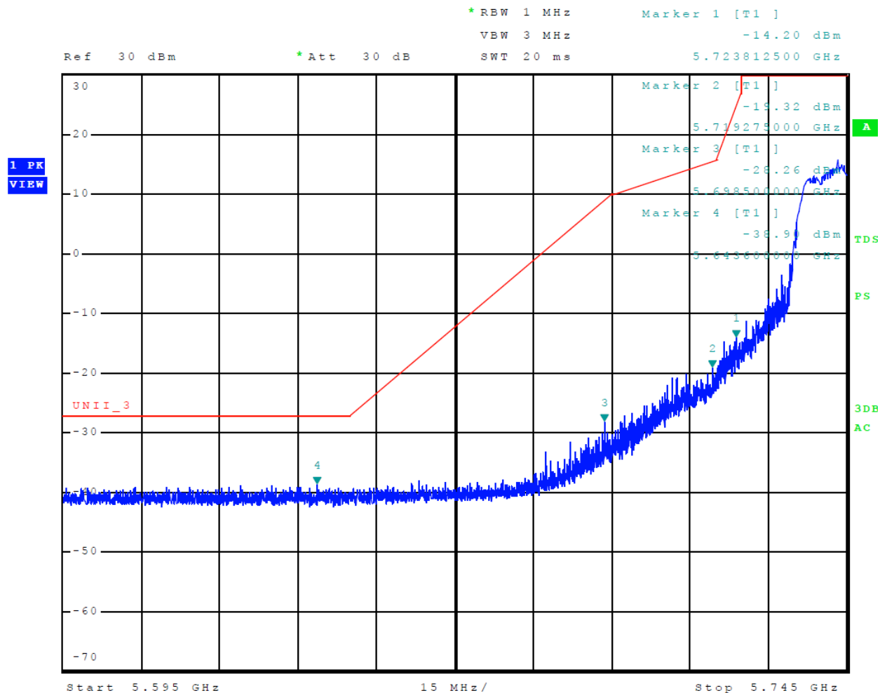
Figure 18 Plot of Lower Band Edge Across 5725-5850 MHz Mode 14 U-NII-3 (802.11n)
