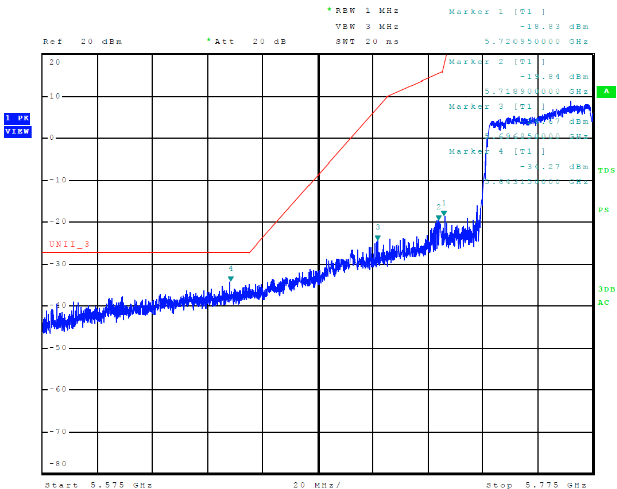
Figure 20 Plot of Lower Band Edge Across 5725-5850 MHz Mode 16 U-NII-3 (802.11ac80)
