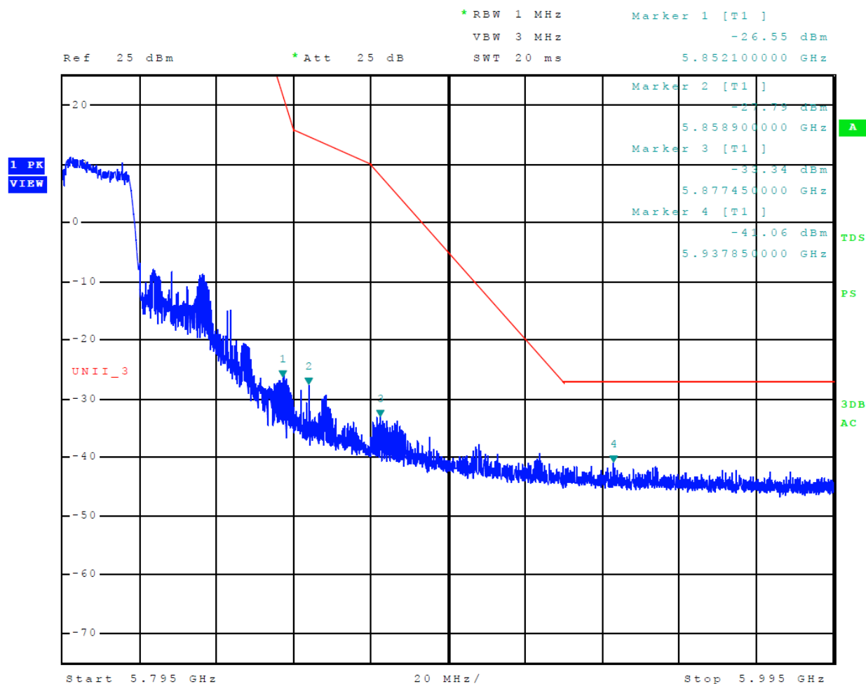
Figure 27 Plot of Upper Band Edge Across 5725-5850 MHz Data Mode 15 U-NII-3 (802.11n40)
