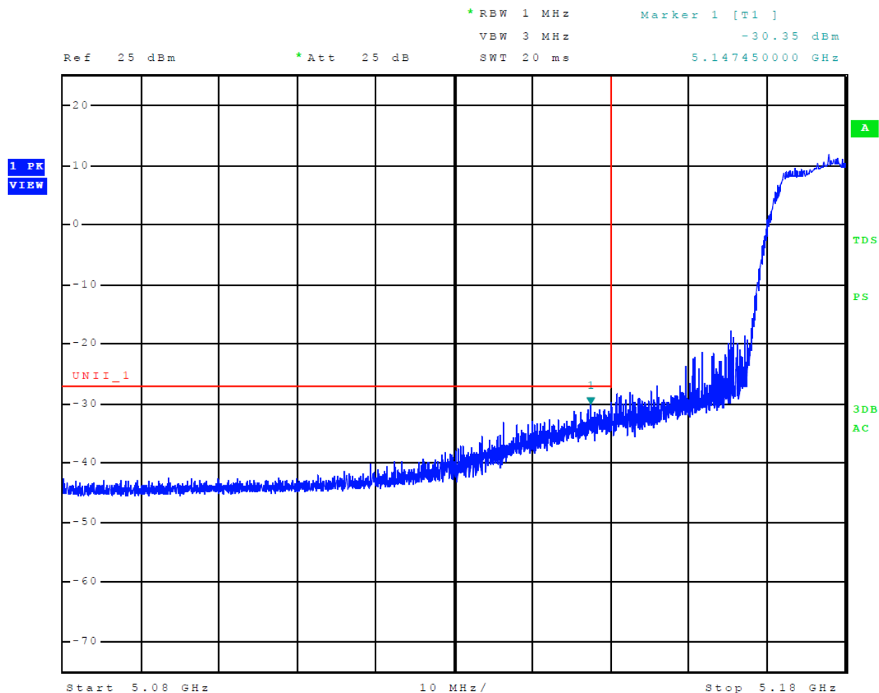
Figure 14 Plot of Lower Band Edge Across 5150-5250 MHz Mode 10 U-NII-1 (802.11n)
