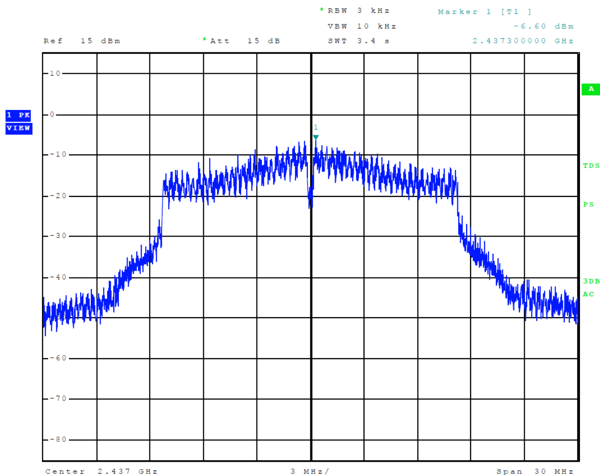
Figure 39 Plot of Transmitter Power Spectral Density Mode 7, 802.11g
