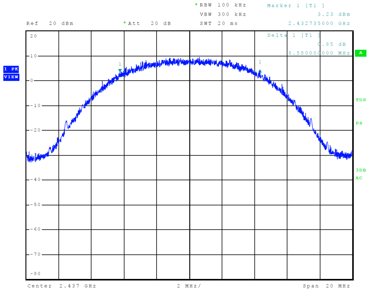
Figure 29 Plot of 6-dB Occupied Bandwidth Mode 6, 802.11b
