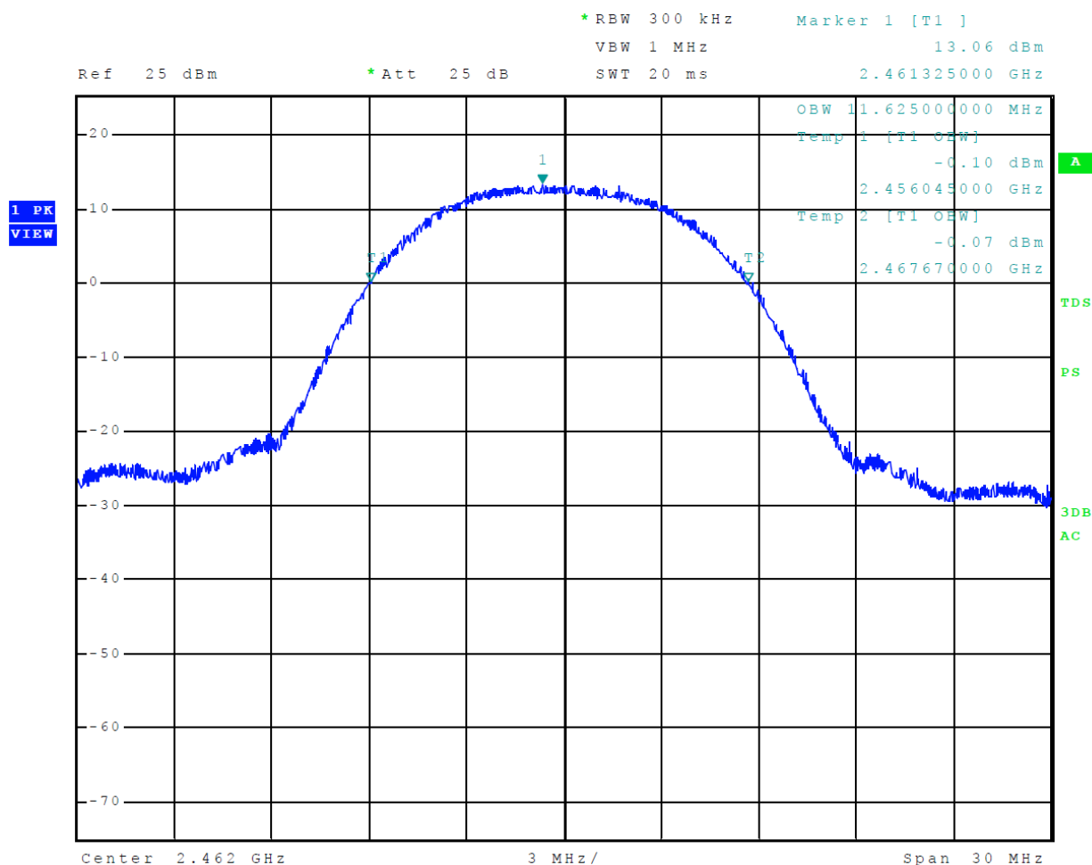
Figure 30 Plot of 99% Occupied Bandwidth Mode 6, 802.11b
