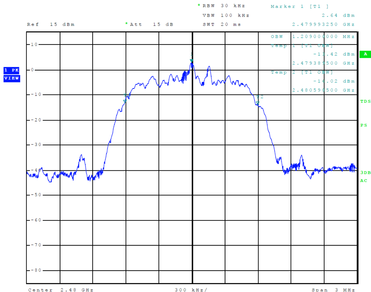
Figure 24 Plot of 99% Occupied Bandwidth Mode 3, BT 2EDR
