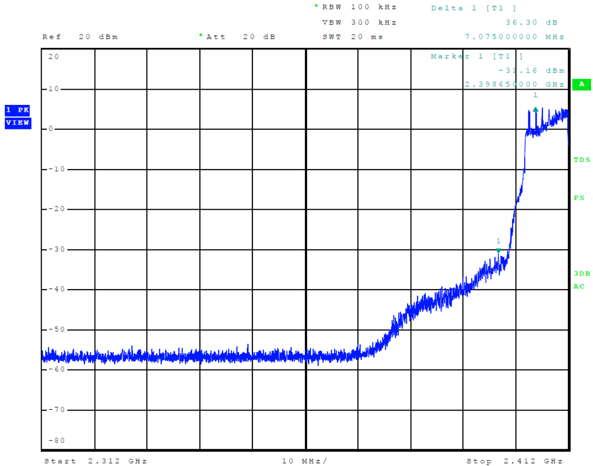
Figure 15 Plot of Emissions Low Band Edge Mode 4, 802.11g
