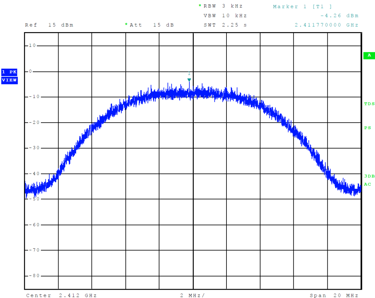
Figure 38 Plot of Transmitter Power Spectral Density Mode 6, 802.11b
