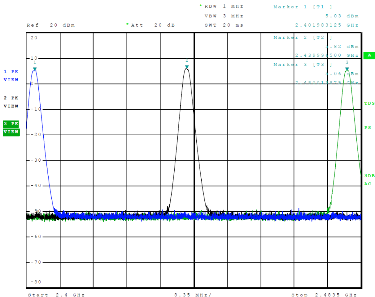
Figure 7 Plot of Transmitter Operation in 2402-2480 MHz Mode 5, BT BLE
