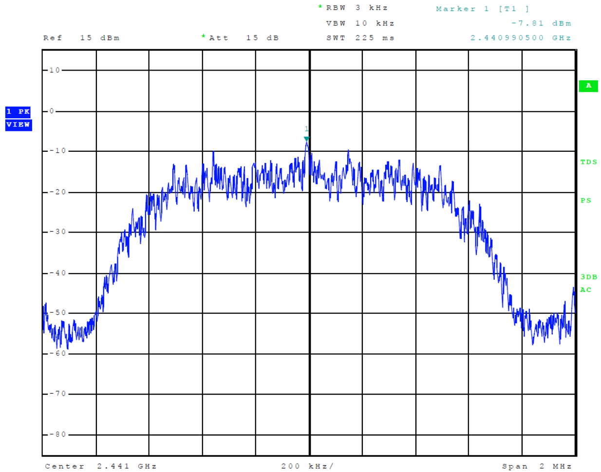
Figure 35 Plot of Transmitter Power Spectral Density Mode 3, BT 2EDR
