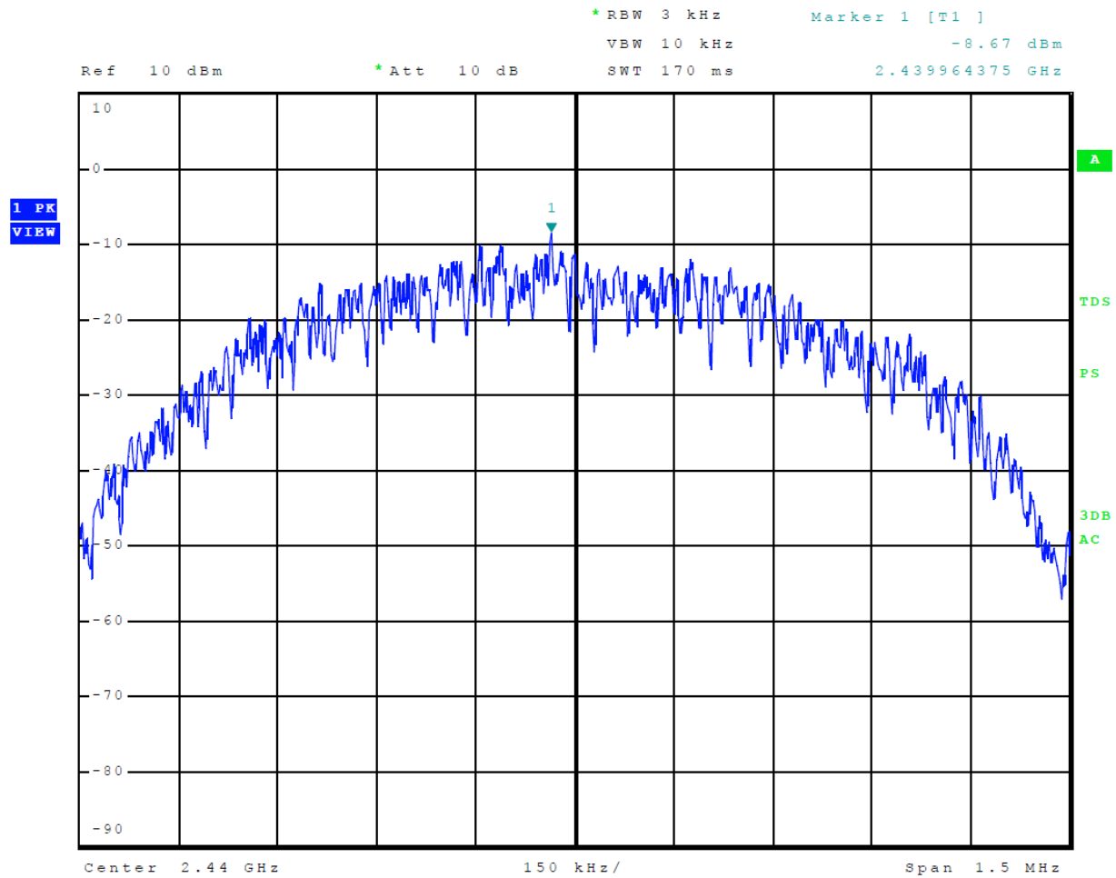
Figure 37 Plot of Transmitter Power Spectral Density Mode 5, BT BLE
