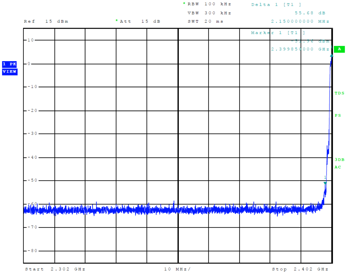
Figure 11 Plot of Emissions Low Band Edge Mode 3, BT 2EDR
