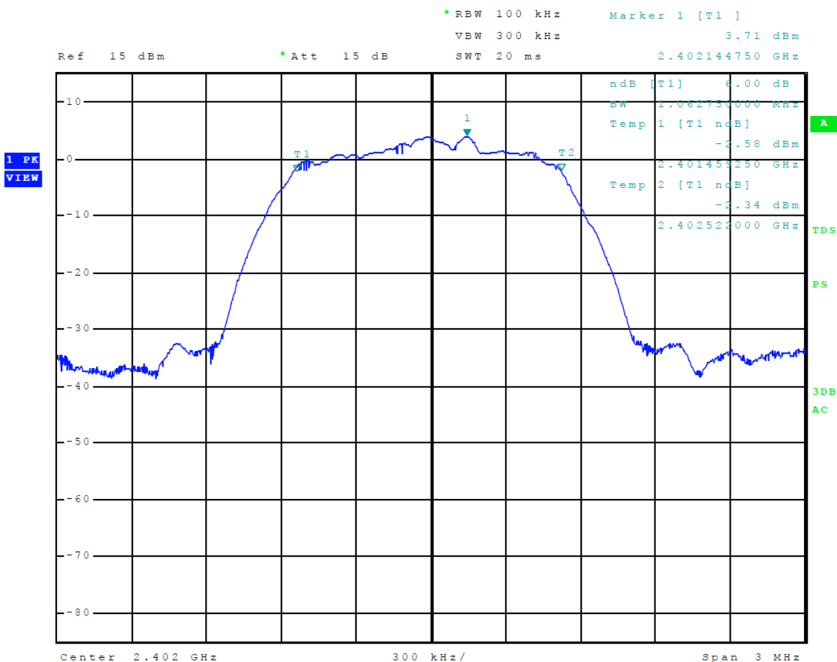
Figure 23 Plot of 6-dB Occupied Bandwidth Mode 3, BT 2EDR
