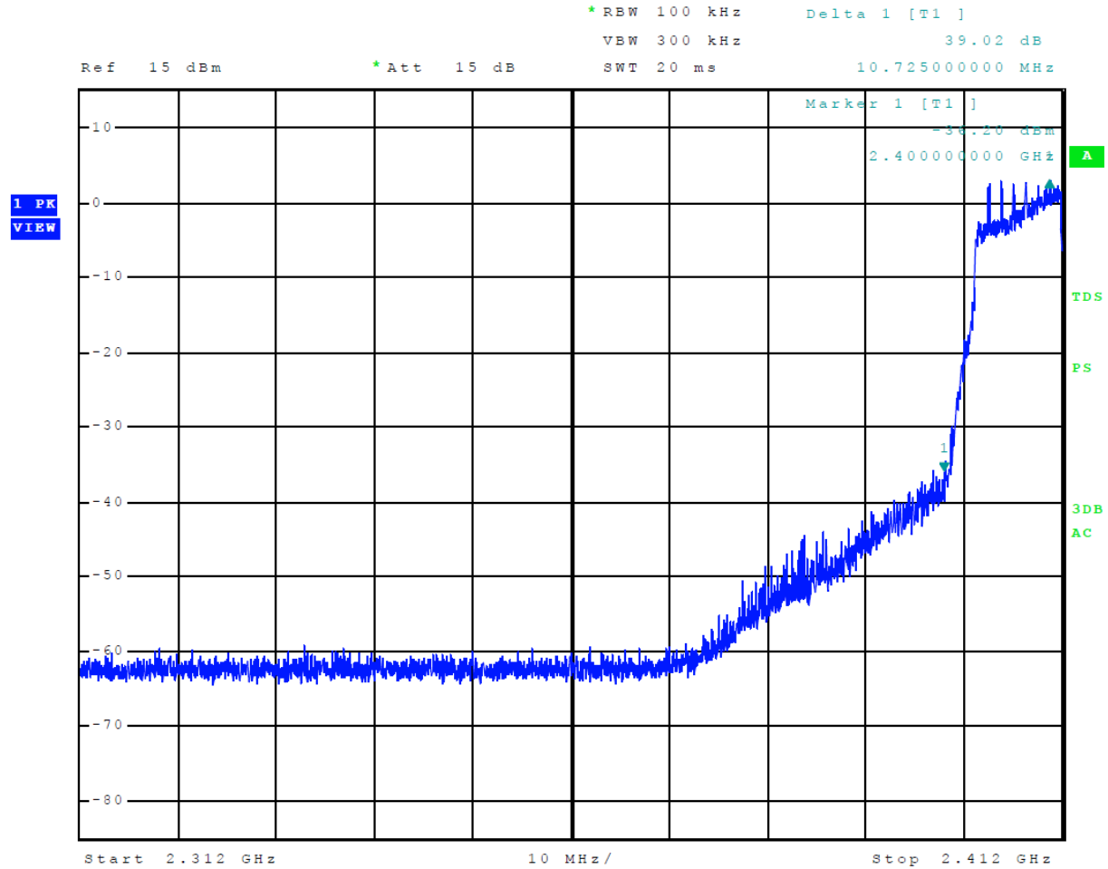
Figure 16 Plot of Emissions Low Band Edge Mode 4, 802.11n
