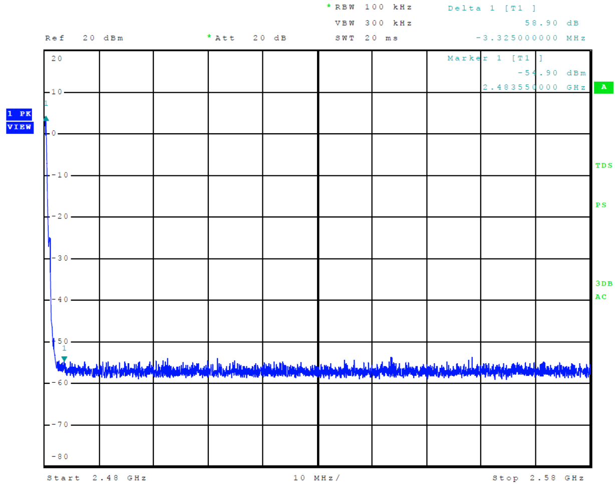
Figure 19 Plot of Transmitter Emissions High Band Edge Mode 5, BT BLE
