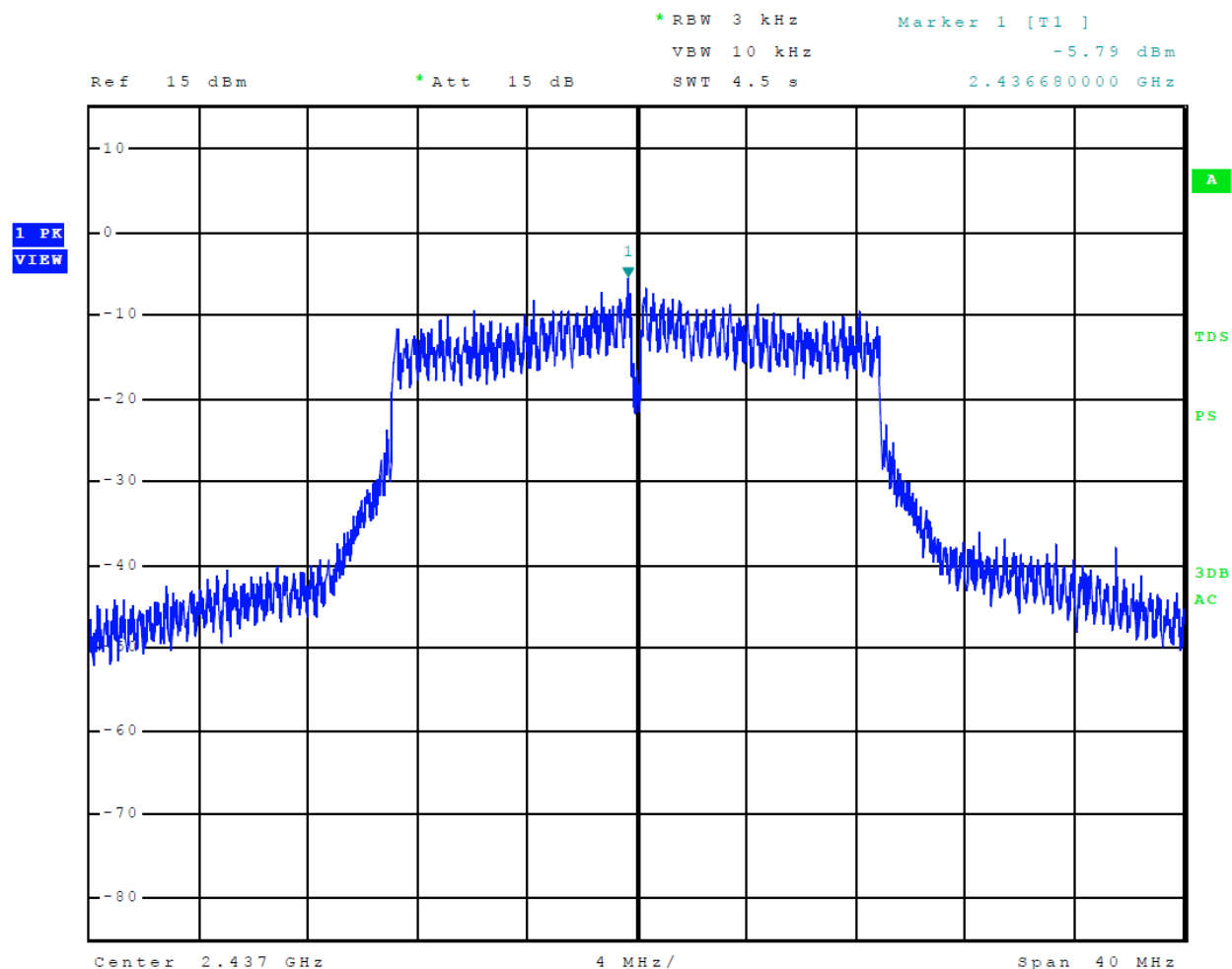
Figure 40 Plot of Transmitter Power Spectral Density Mode 8, 802.11n
