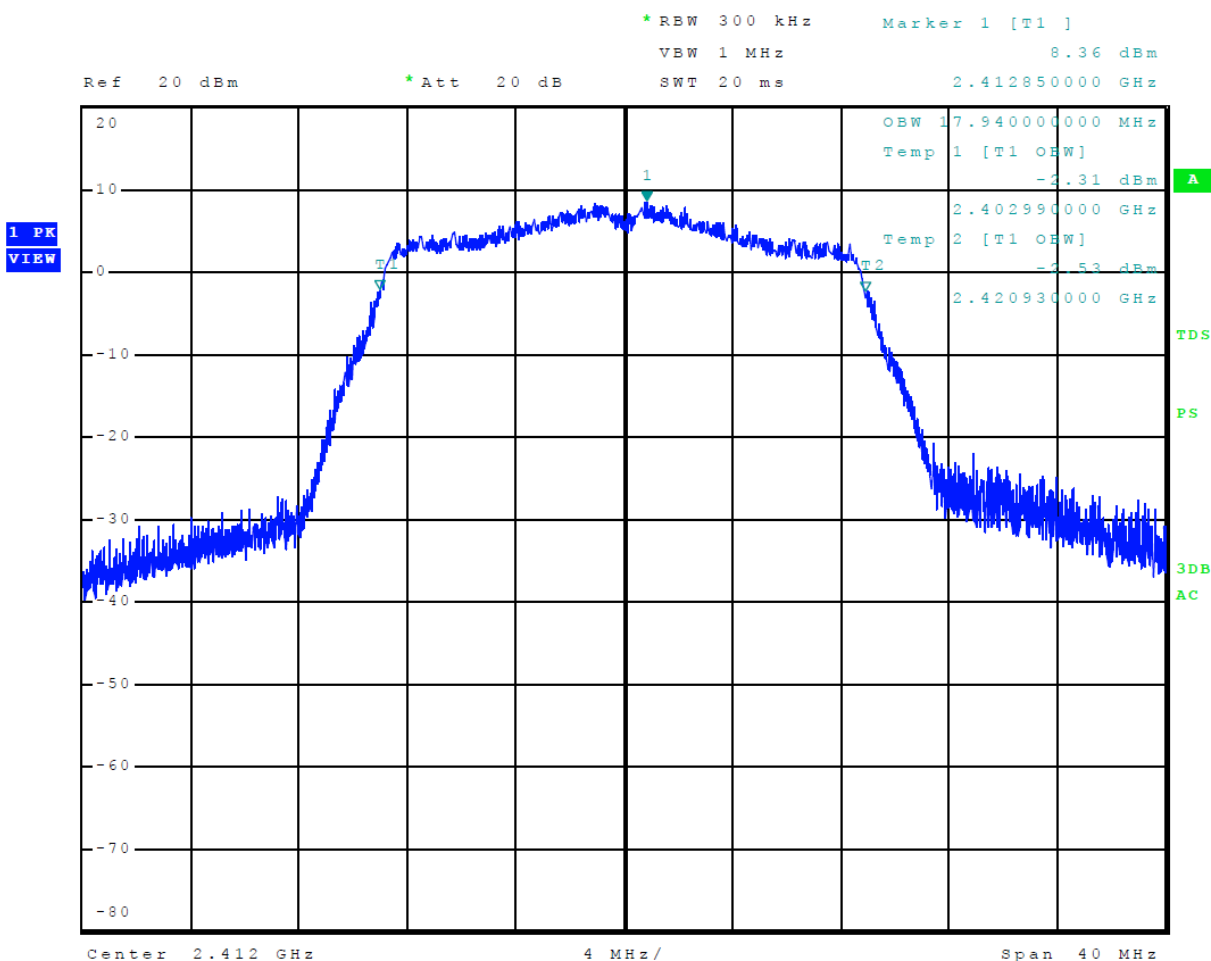
Figure 34 Plot of 99% Occupied Bandwidth Mode 8, 802.11n
