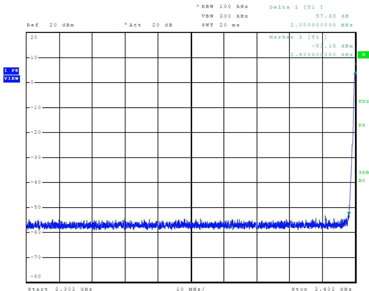
Figure 13 Plot of Emissions Low Band Edge Mode 5, BT BLE
