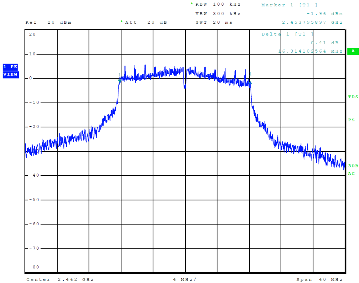
Figure 31 Plot of 6-dB Occupied Bandwidth Mode 7, 802.11g
