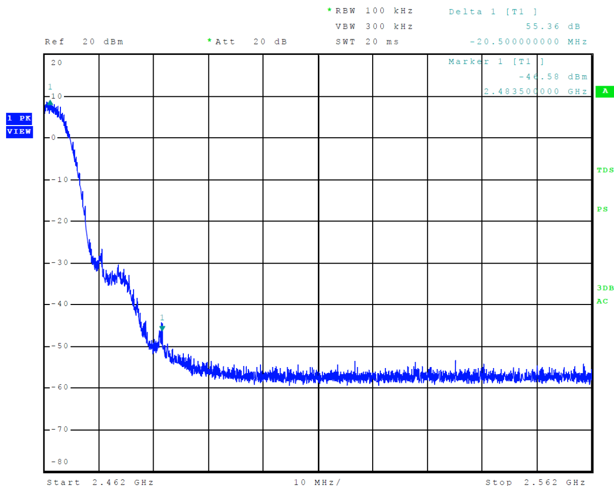
Figure 20 Plot of Transmitter Emissions High Band Edge Mode 6, 802.11b
