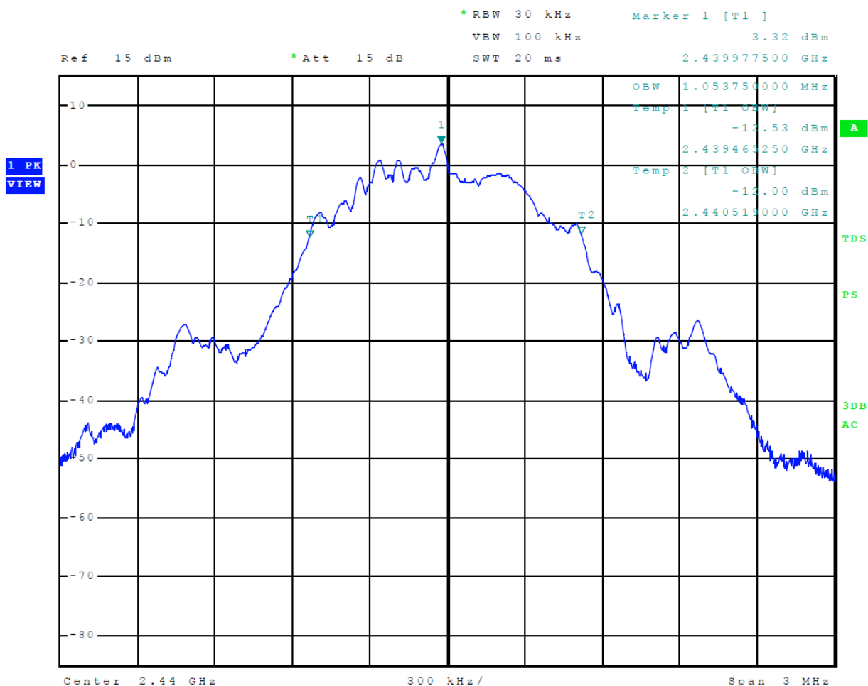
Figure 28 Plot of 99% Occupied Bandwidth Mode 5, BT BLE
