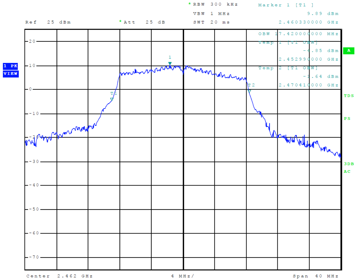
Figure 32 Plot of 99% Occupied Bandwidth Mode 7, 802.11g
