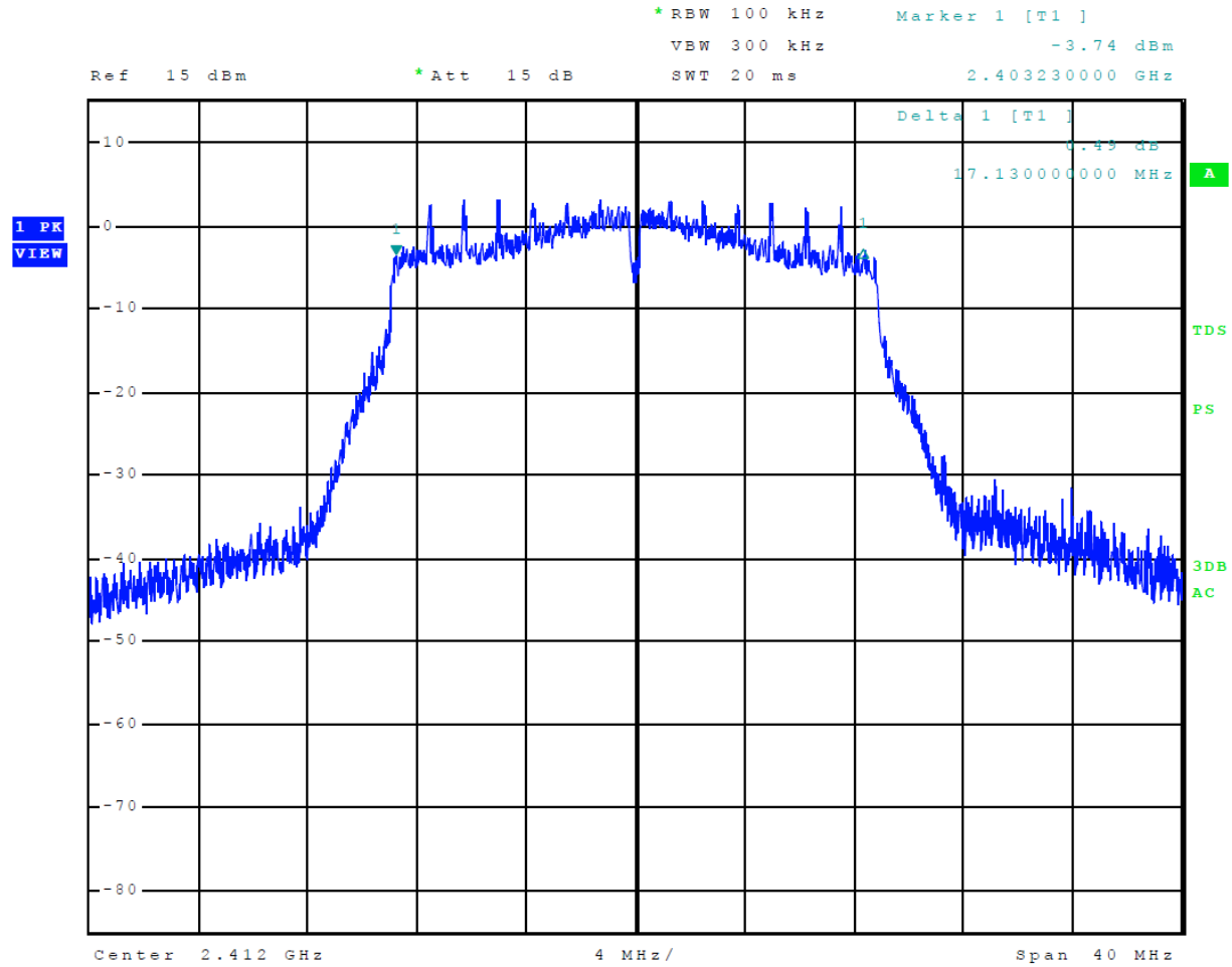
Figure 33 Plot of 6-dB Occupied Bandwidth Mode 8, 802.11n
