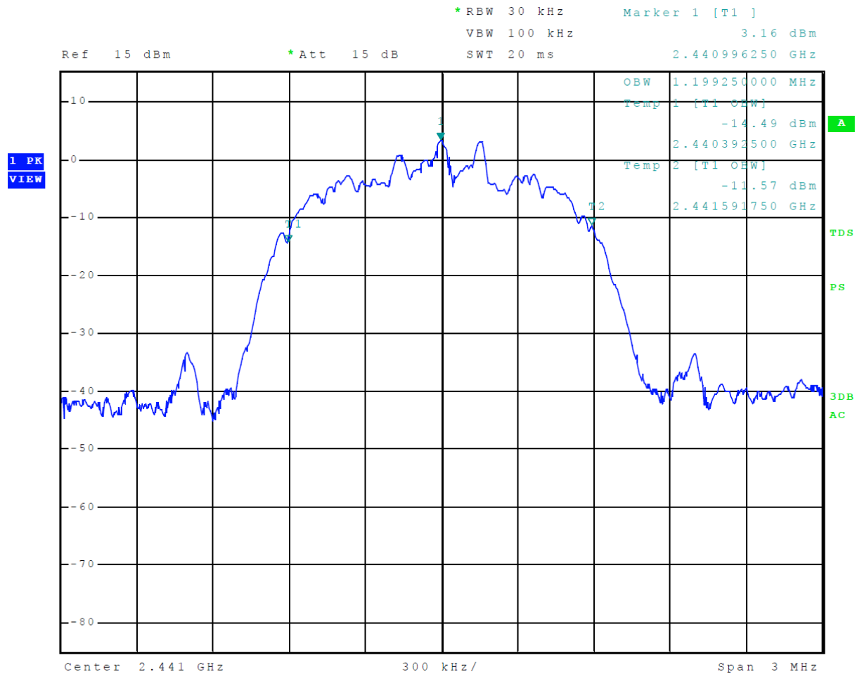
Figure 26 Plot of 99% Occupied Bandwidth Mode 4, BT 3EDR
