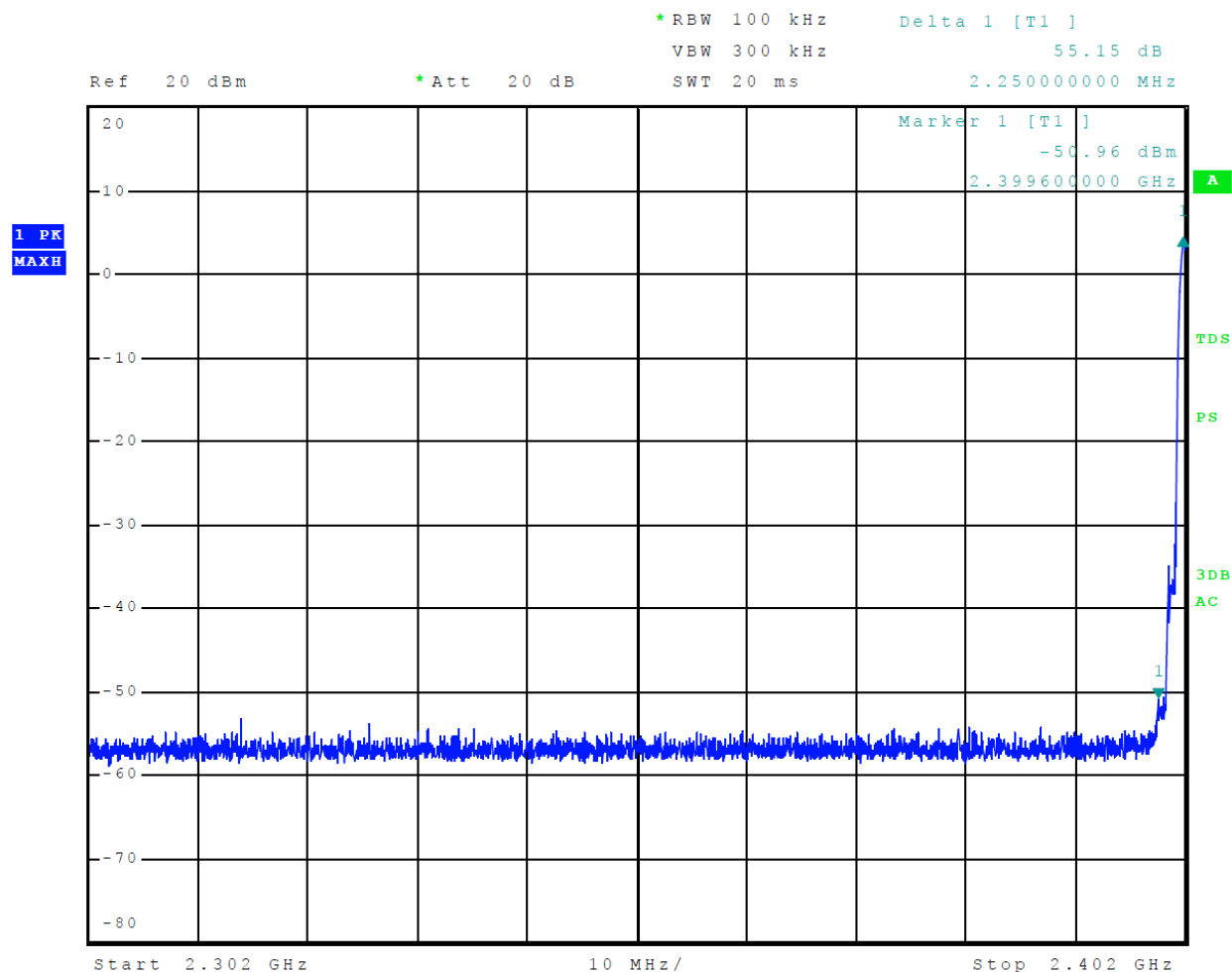
Figure 12 Plot of Emissions Low Band Edge Mode 4, BT 3EDR
