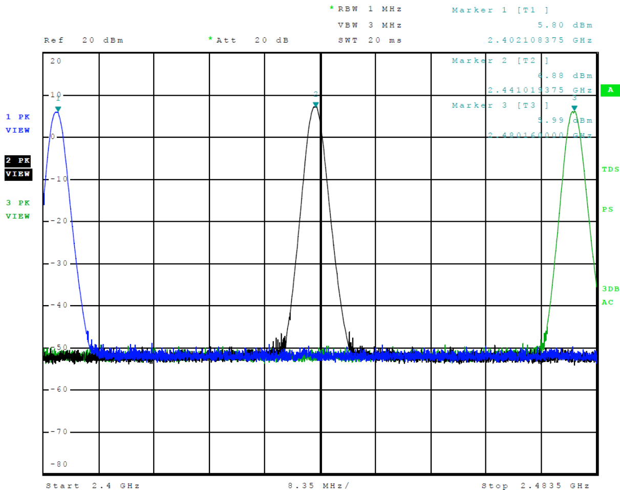
Figure 5 Plot of Transmitter Operation in 2402-2480 MHz Mode 3, BT 2EDR
