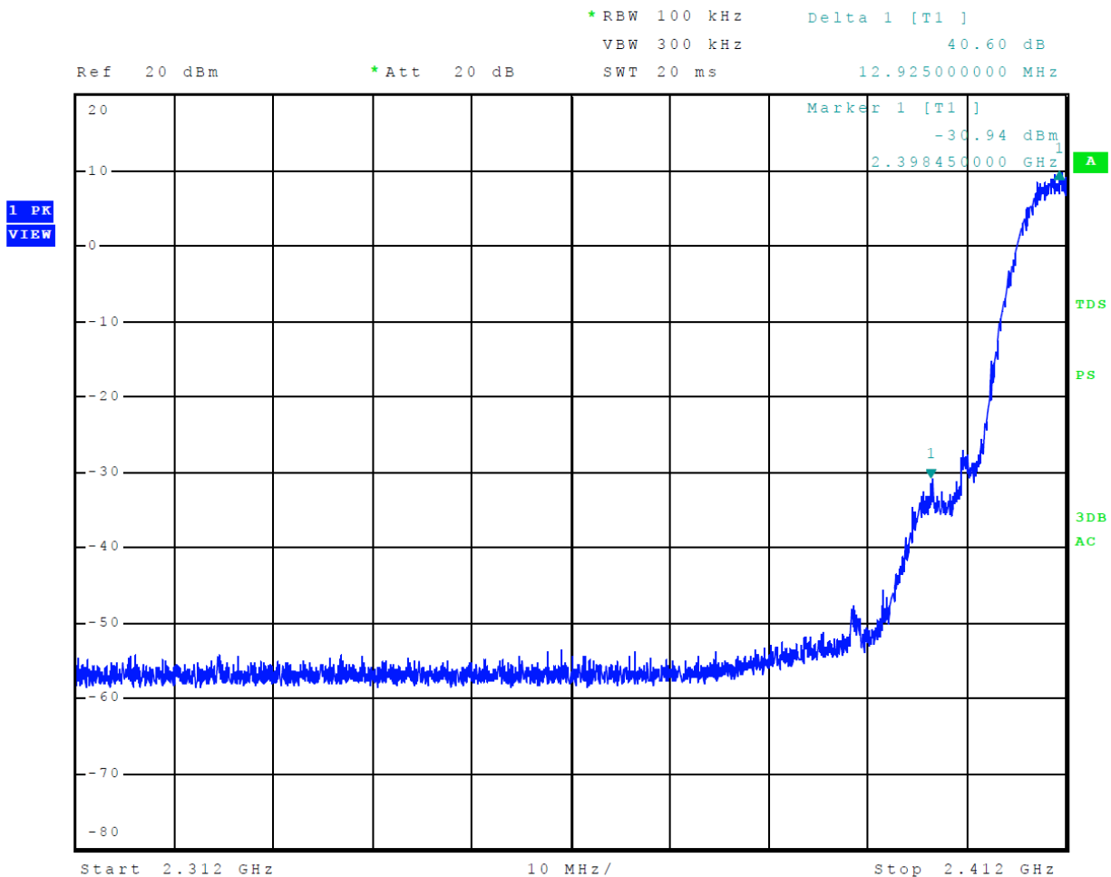
Figure 14 Plot of Emissions Low Band Edge Mode 4, 802.11b
