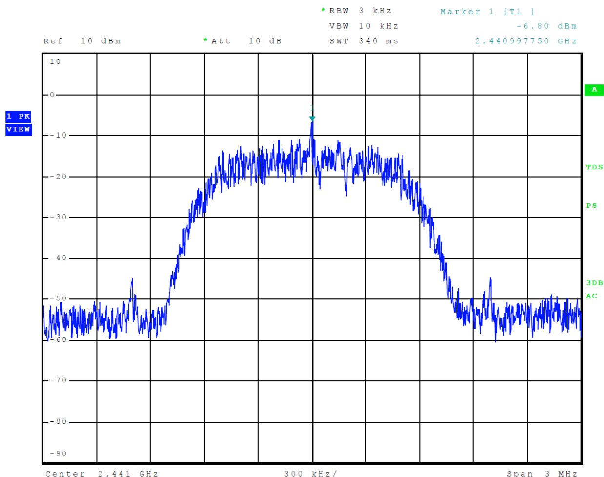
Figure 36 Plot of Transmitter Power Spectral Density Mode 4, BT 3EDR
