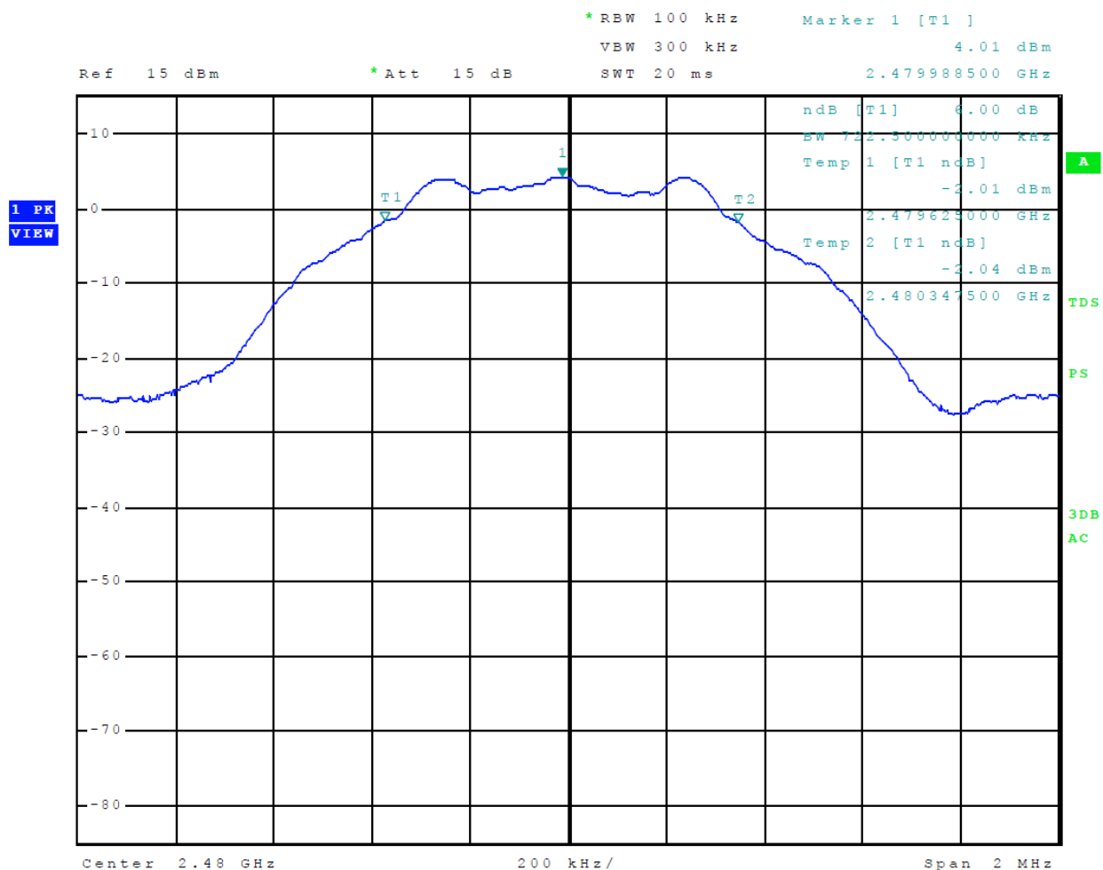
Figure 27 Plot of 6-dB Occupied Bandwidth Mode 5, BT BLE
