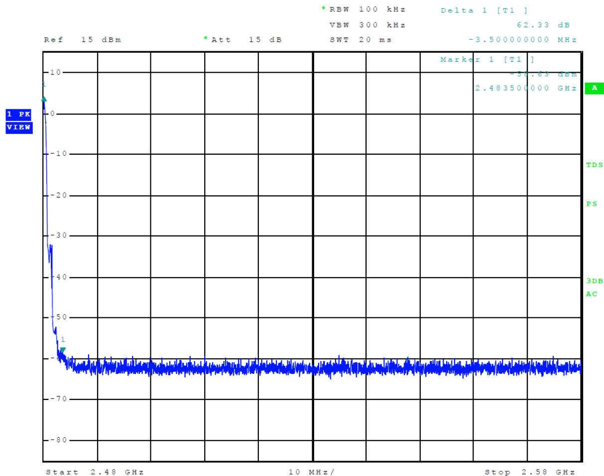
Figure 17 Plot of Transmitter Emissions High Band Edge Mode 3, BT 2EDR
