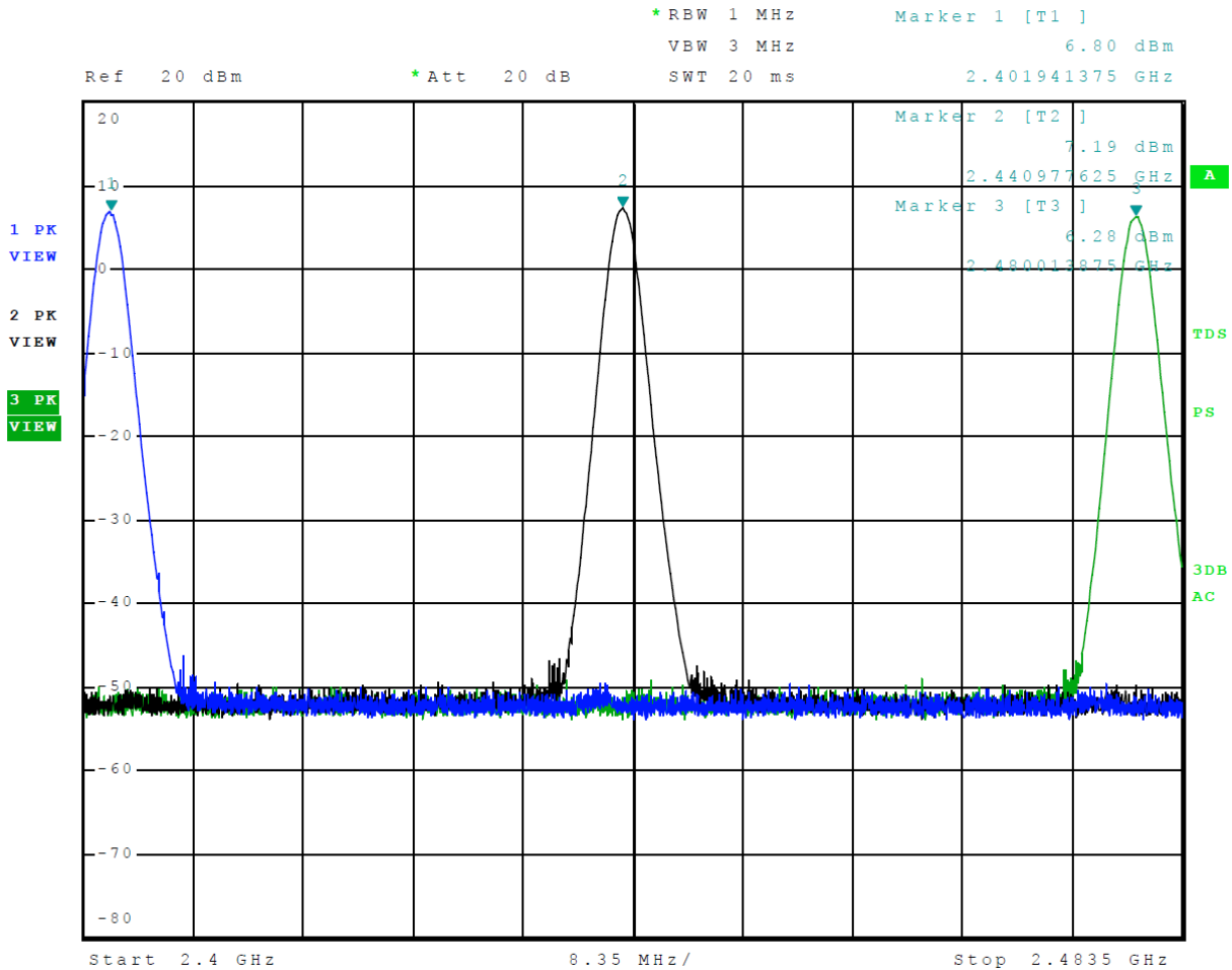
Figure 6 Plot of Transmitter Operation in 2402-2480 MHz Mode 4, BT 3EDR
