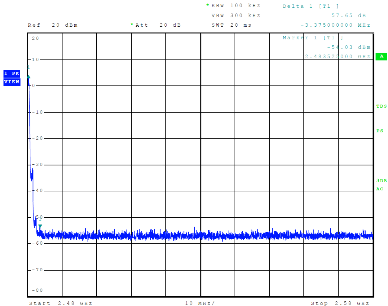
Figure 18 Plot of Transmitter Emissions High Band Edge Mode 4, BT 3EDR
