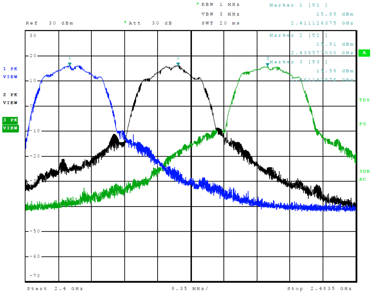
Figure 9 Plot of Transmitter Operation in 2402-2480 MHz Mode 7, 802.11g
