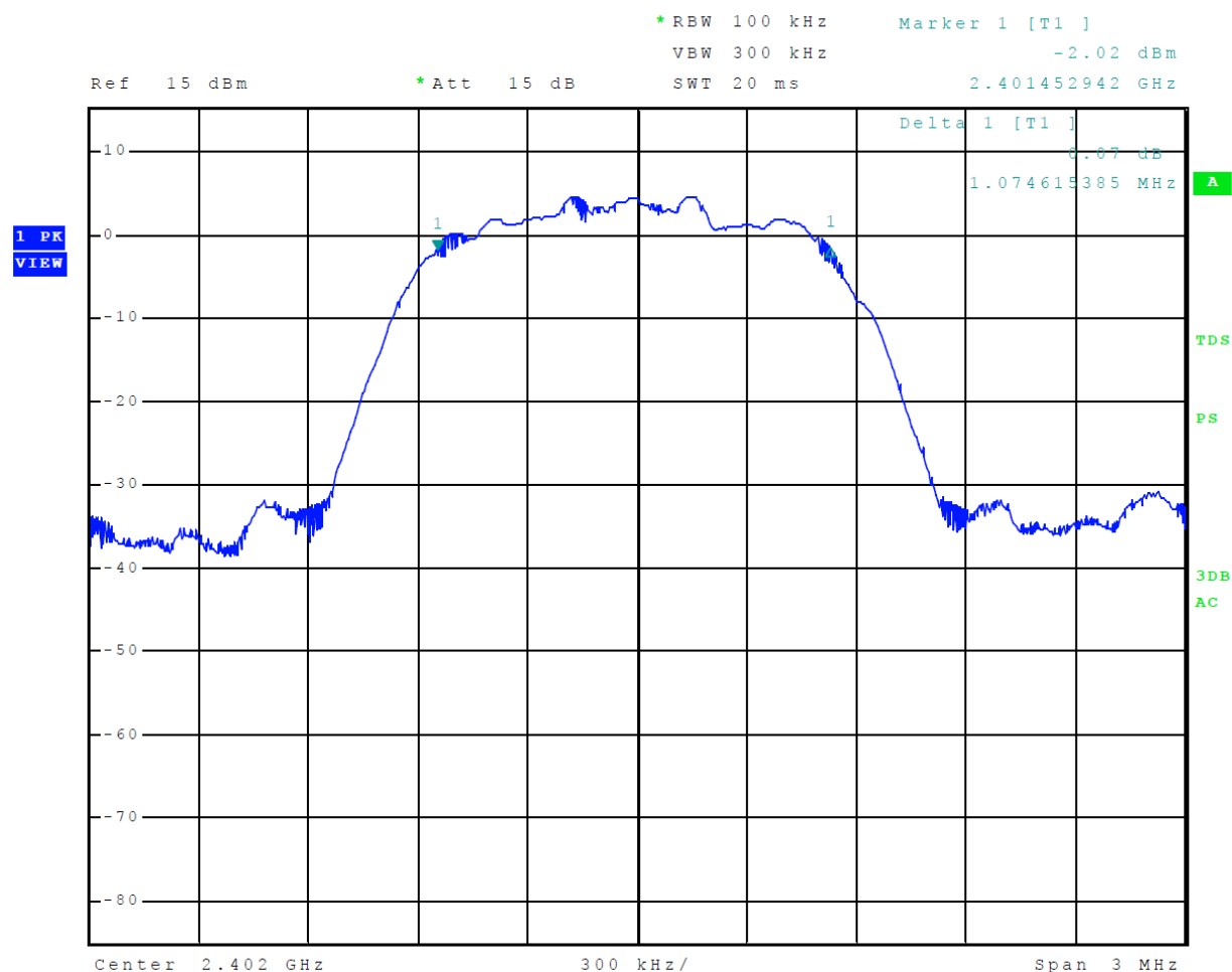
Figure 25 Plot of 6-dB Occupied Bandwidth Mode 4, BT 3EDR
