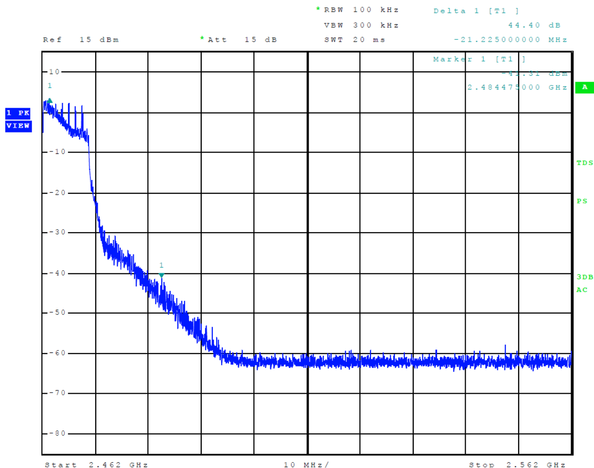
Figure 22 Plot of Transmitter Emissions High Band Edge Mode 8, 802.11n
