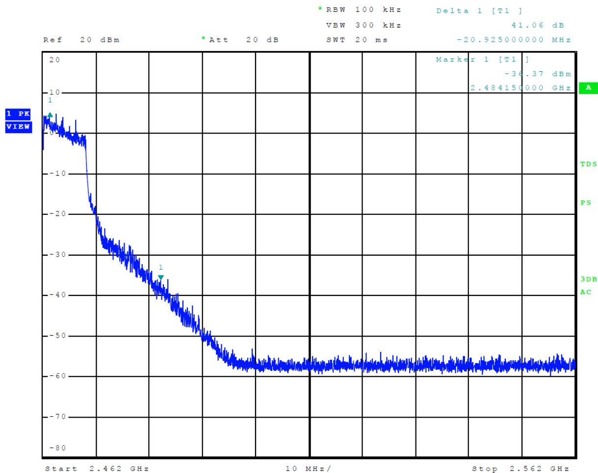
Figure 21 Plot of Transmitter Emissions High Band Edge Mode 7, 802.11g
