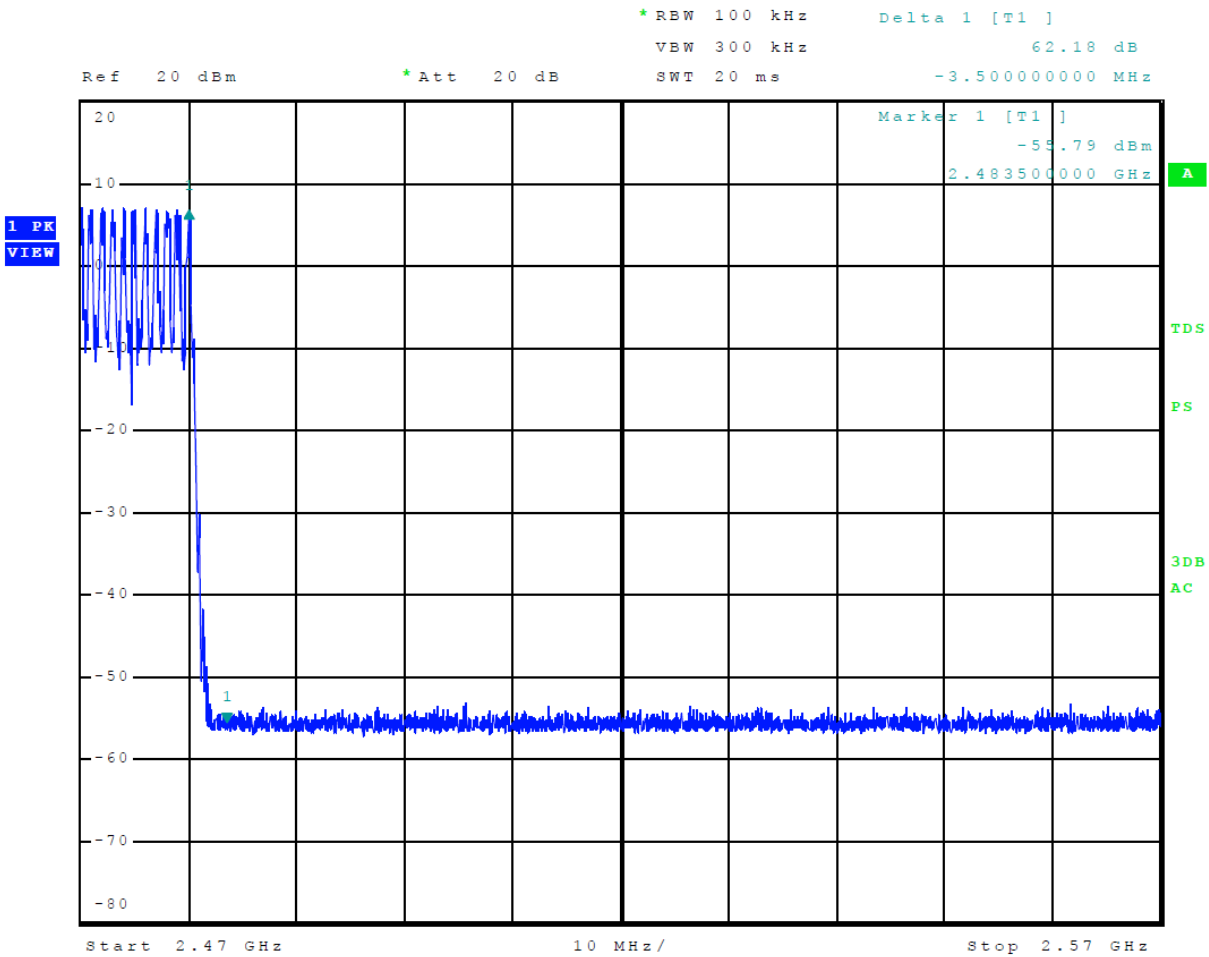
Figure 12 Plot of Transmitter Emissions High Band Edge Mode 2, BT BR
