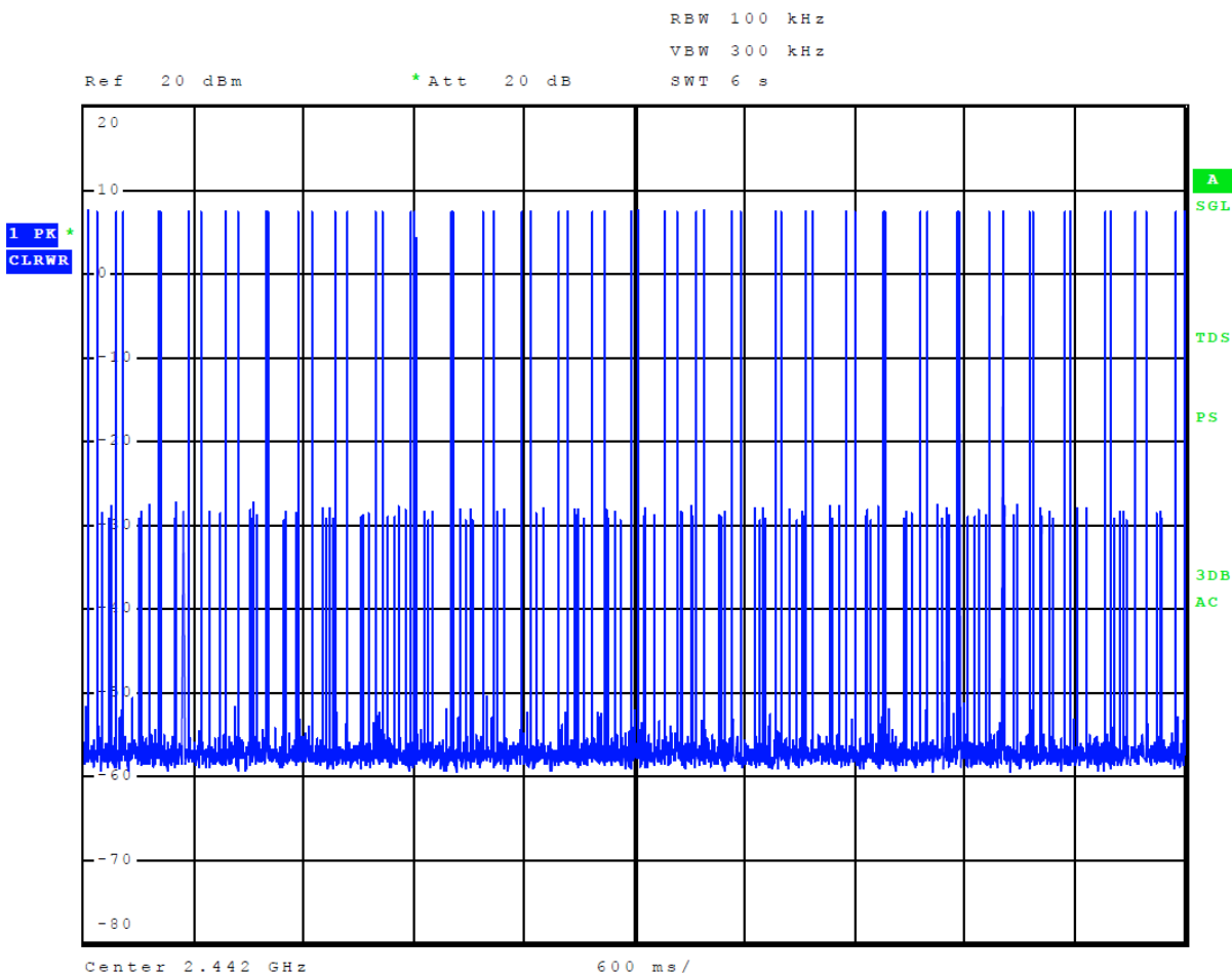
Figure 10 Plot of Number of Times on Channel over 6 Second Period Mode 2, BT BR
