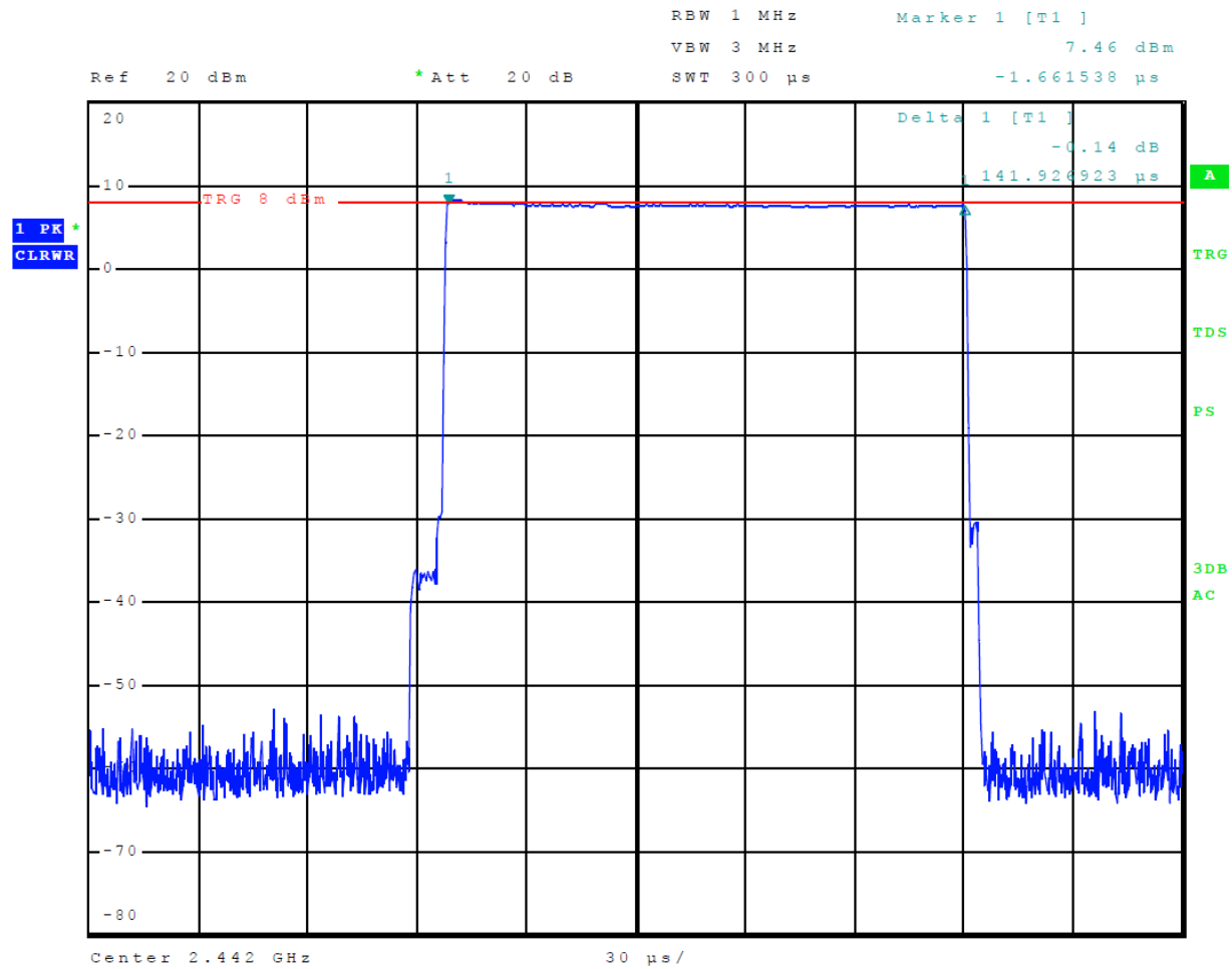
Figure 9 Plot of Dwell time On Channel Mode 2, BT BR
