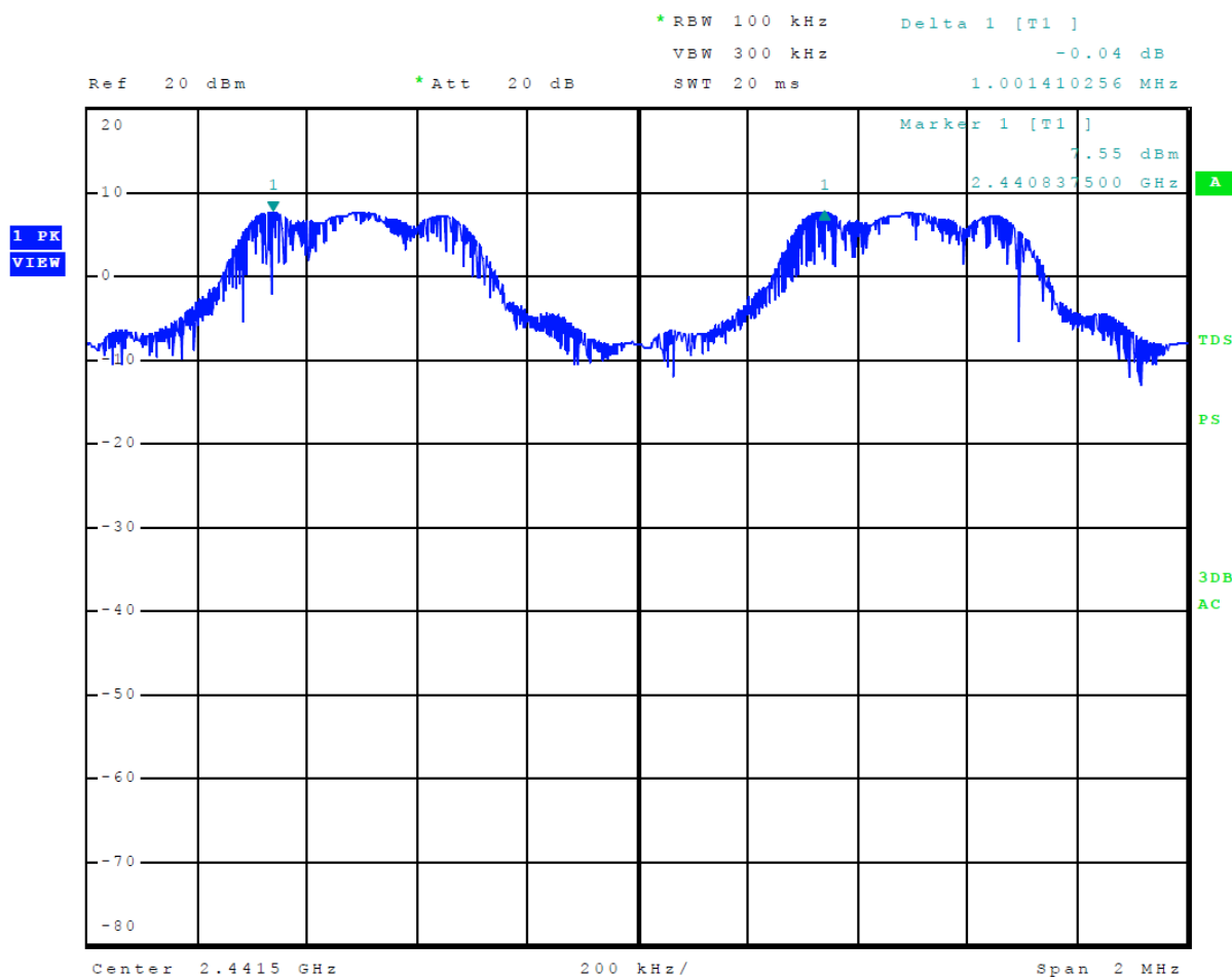
Figure 10 Plot of Channel Separation Mode 2, BT BR
