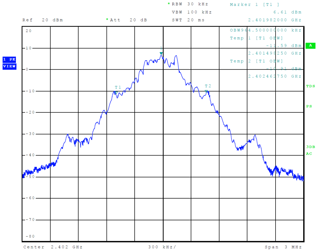
Figure 5 Plot of Transmitter Emissions 99% Occupied Bandwidth Mode 2, BT BR
