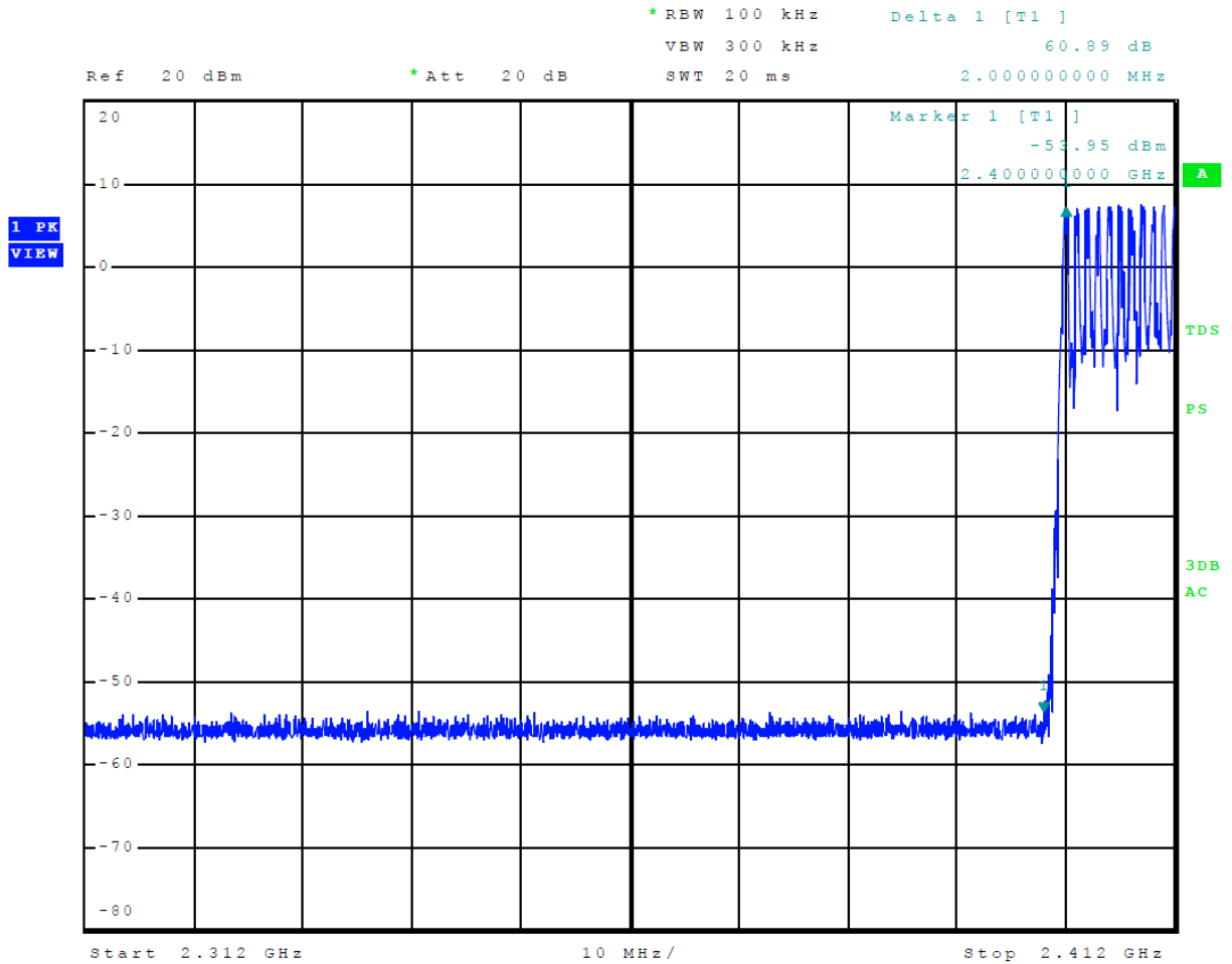
Figure 11 Plot of Transmitter Emissions Low Band Edge Mode 2, BT BR
