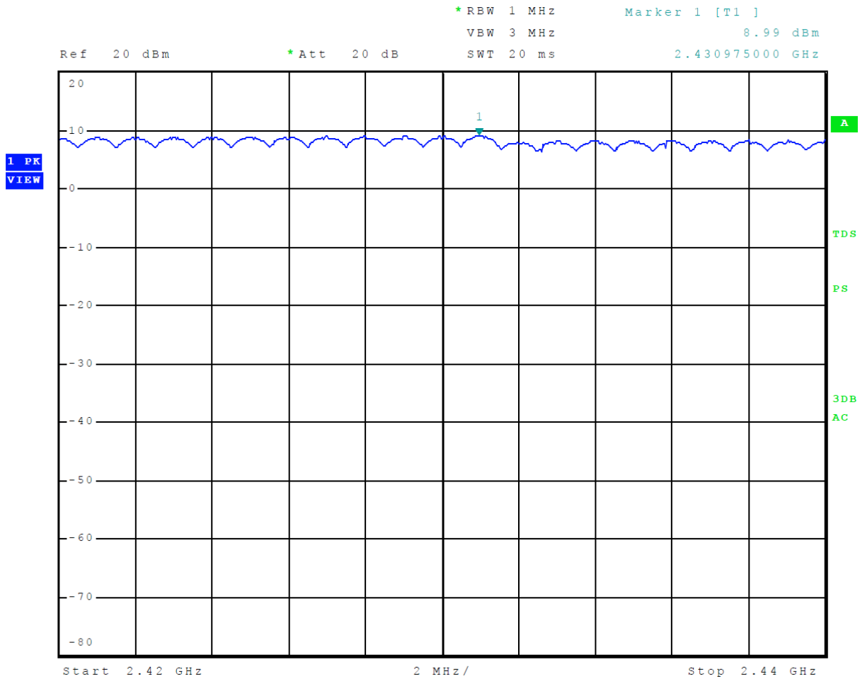
Figure 7 Plot of Number of Hopping Channels Mode 2, BT BR
