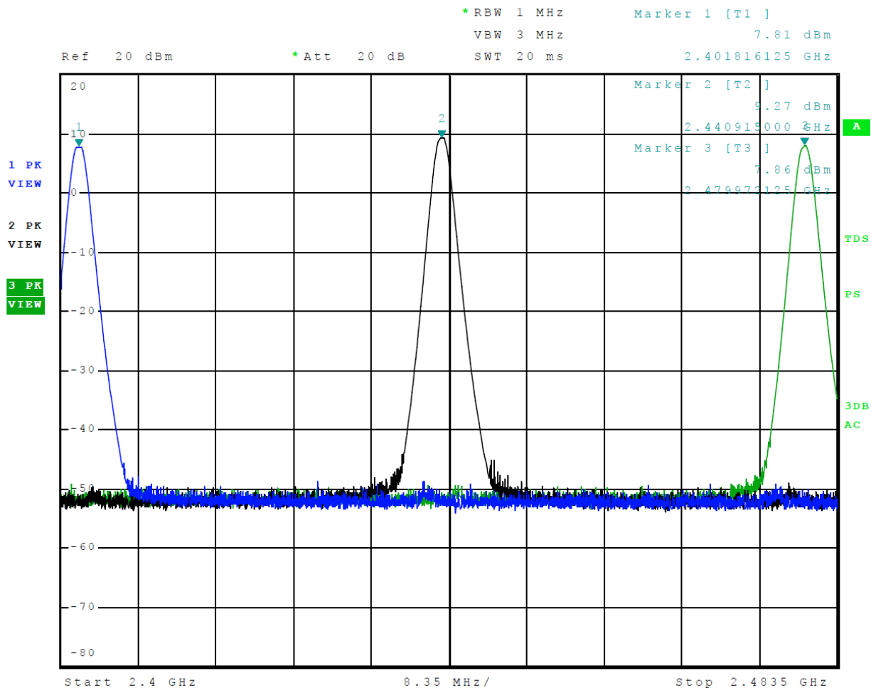
Figure 3 Plot of Transmitter Emissions Operation in 2402-2480 MHz Mode 2, BT BR
