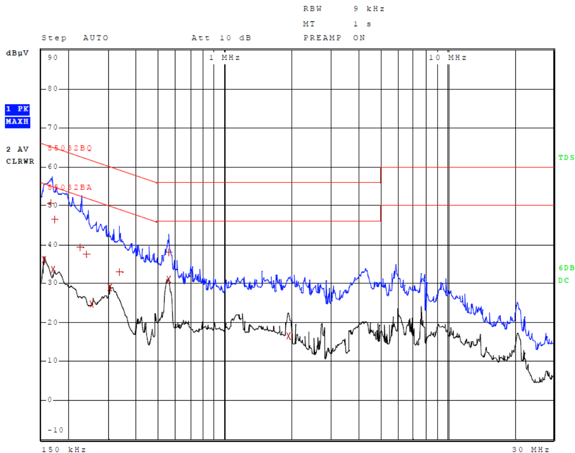
Figure 1 AC Line Conducted Emissions Data L1 (#5, EUT – Computer)
