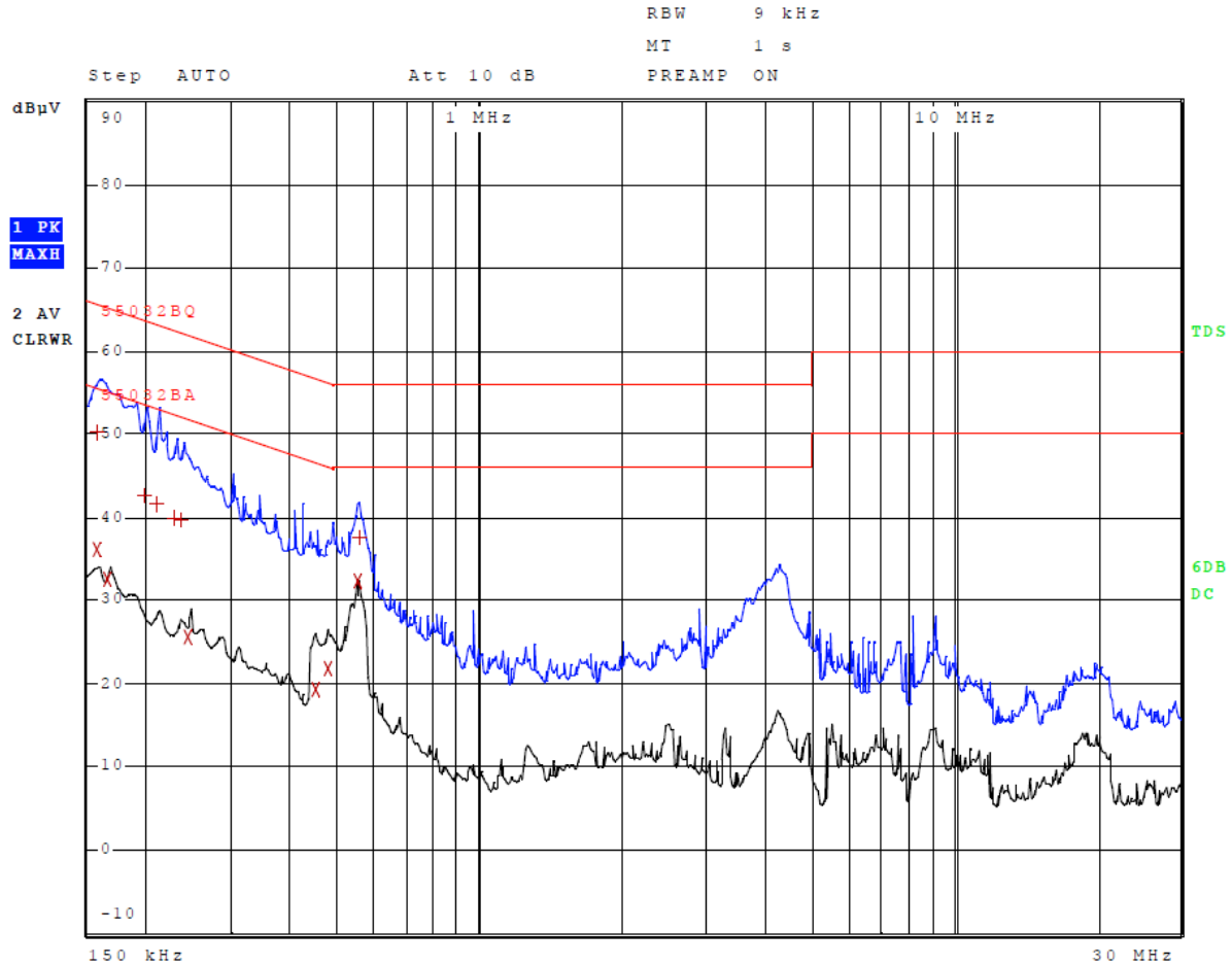
Figure 2 AC Line Conducted Emissions Data L2 (#5, EUT – Computer)
