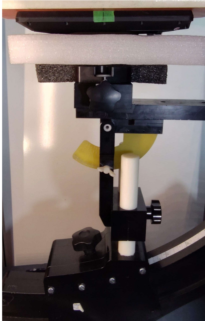
Figure C.3 – Setup Photo, Extremity - Front
