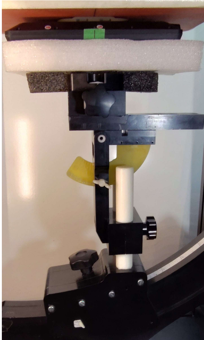
Figure C.1 – Setup Photo, Extremity - Back Touch
