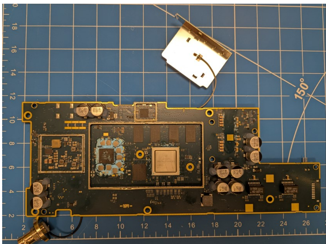
Rear: PCBA#1
