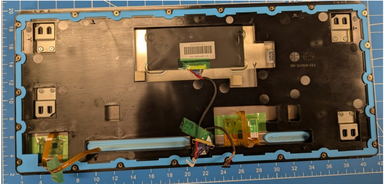
Front with boards in Chassis:
