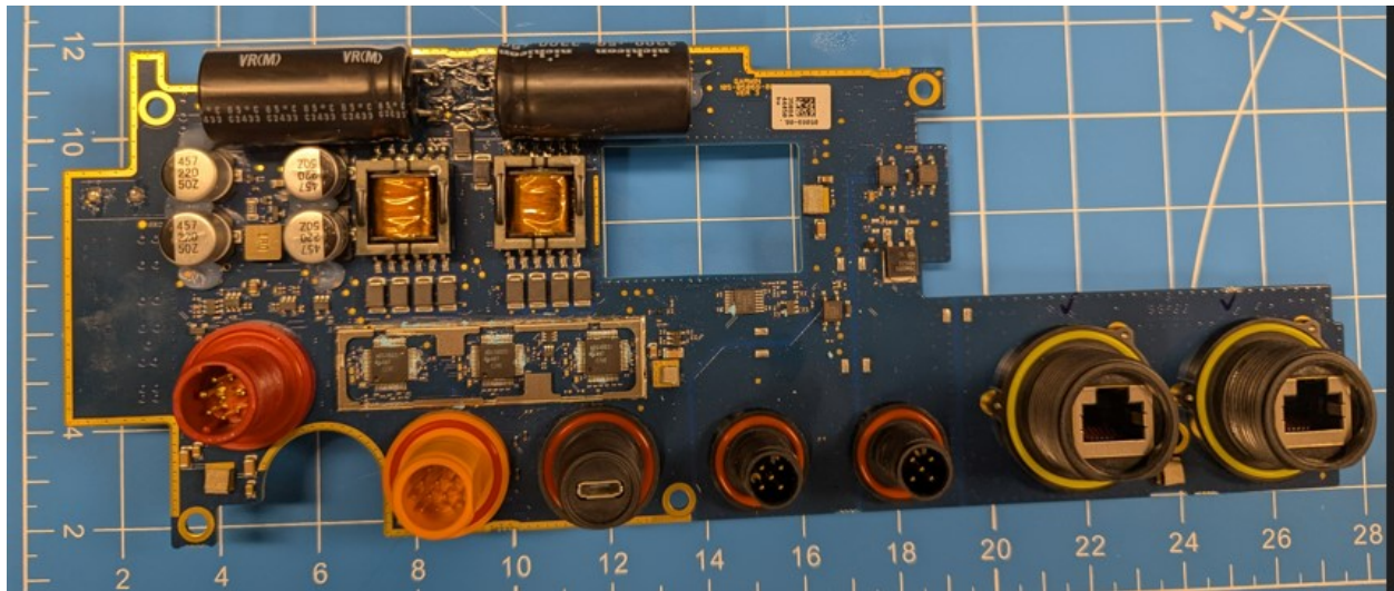
Back PCBA#2
