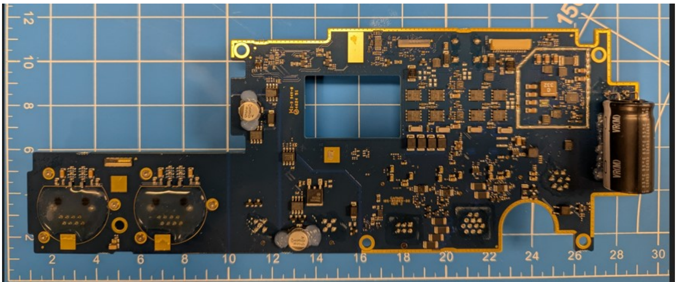
Front PCBA#2
