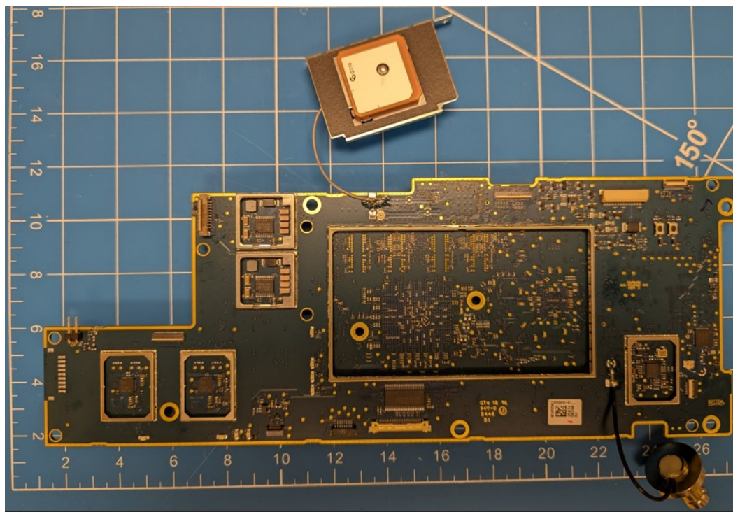
Front PCBA#1
