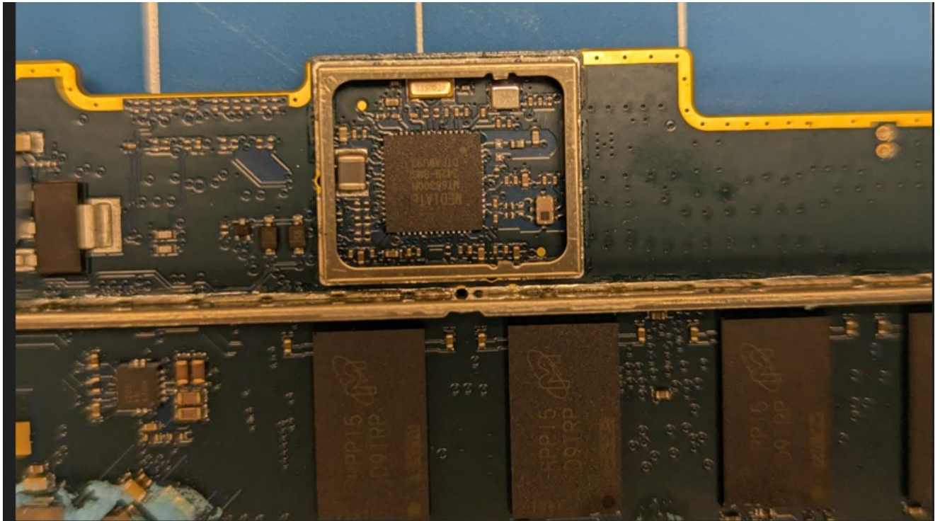
Rear: PCBA#1 (Close-up – Wifi/BLE transmitter)
