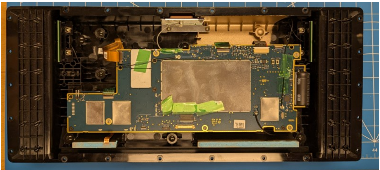
Rear with boards in Chassis:
