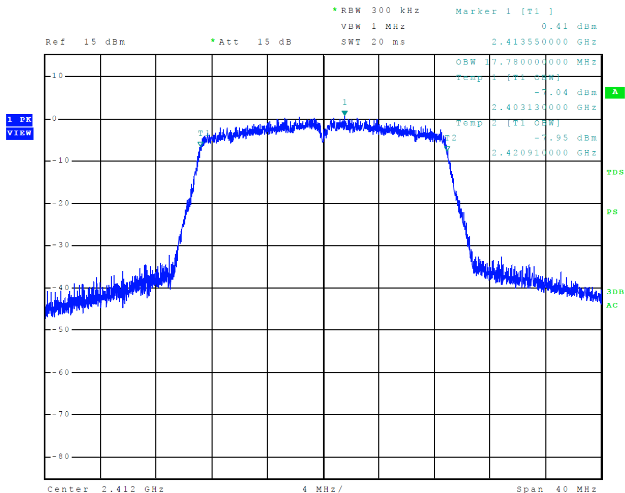
Figure 24 Plot of 99% Occupied Bandwidth Mode 5, 802.11n
