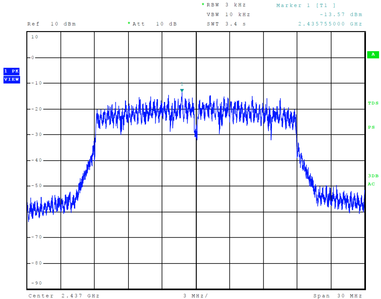
Figure 28 Plot of Transmitter Power Spectral Density Mode 5, 802.11n
