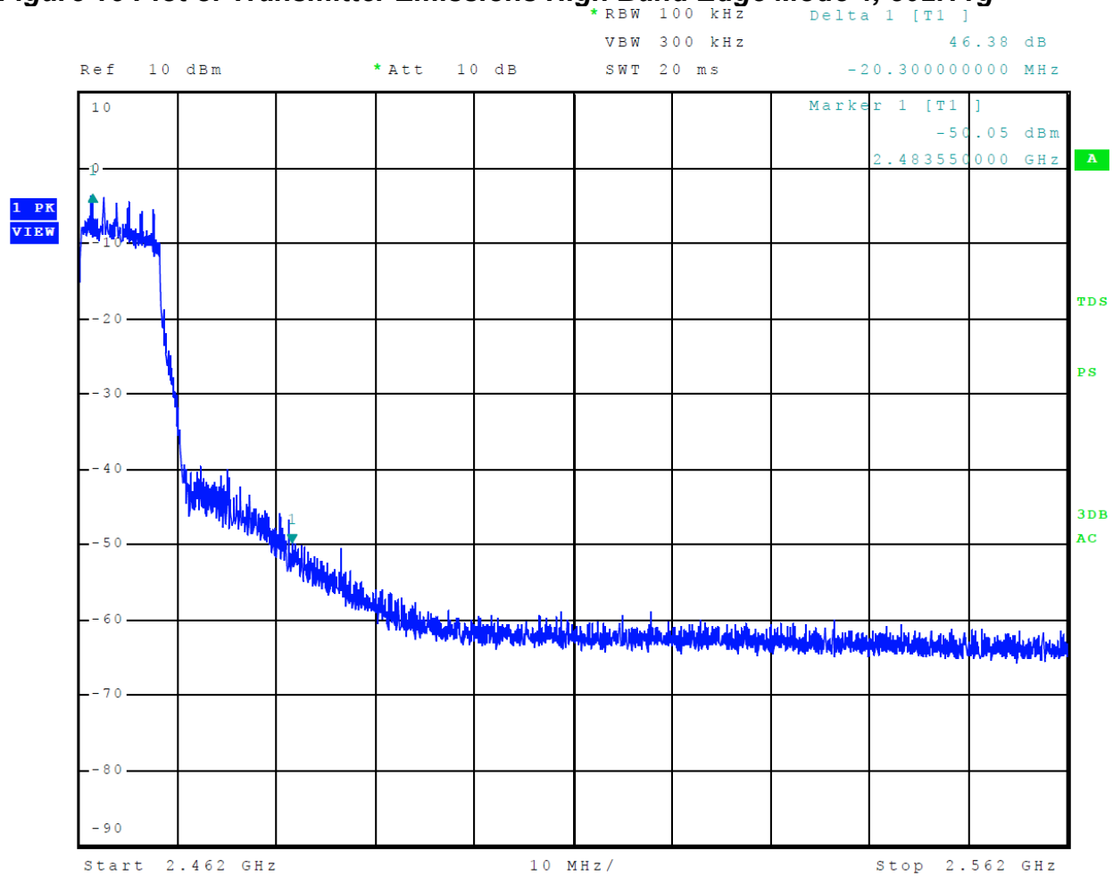
Figure 15 Plot of Transmitter Emissions High Band Edge Mode 4, 802.11g
