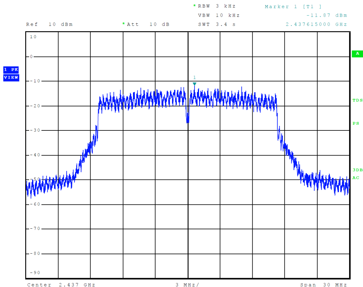
Figure 27 Plot of Transmitter Power Spectral Density Mode 4, 802.11g
