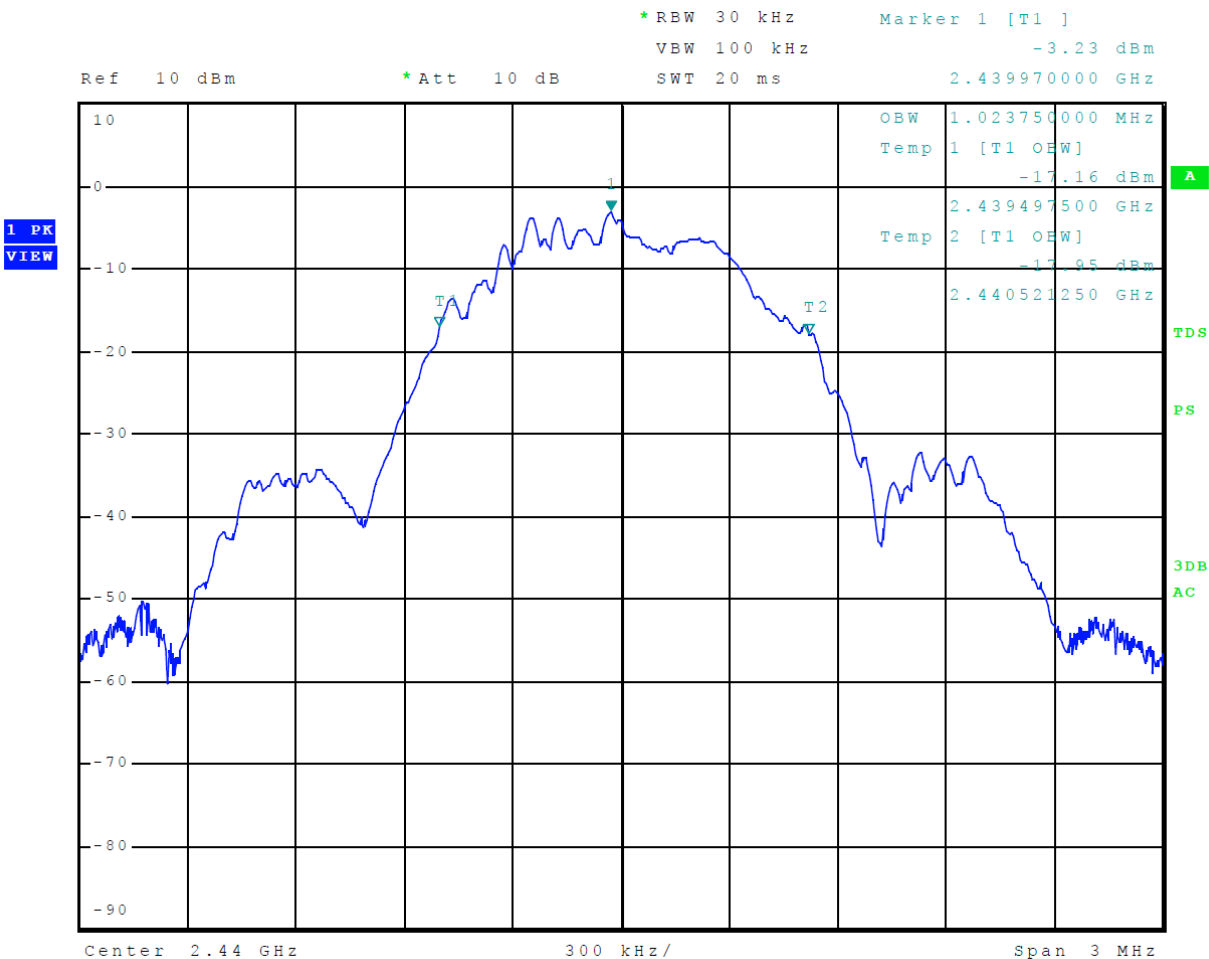
Figure 18 Plot of 99% Occupied Bandwidth Mode 2, BT BLE (GMSK)
