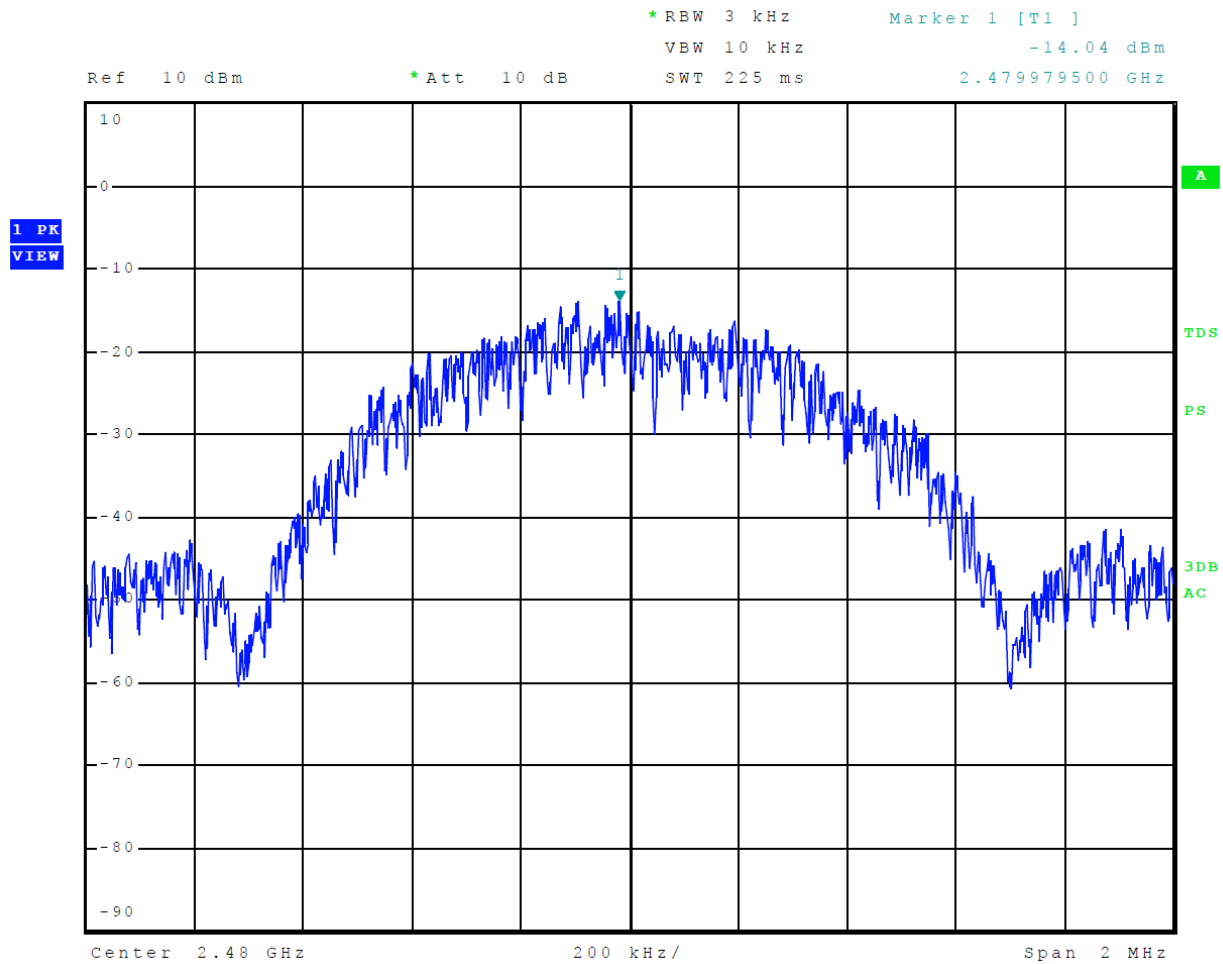
Figure 25 Plot of Transmitter Power Spectral Density Mode 2, BT BLE (GMSK)
