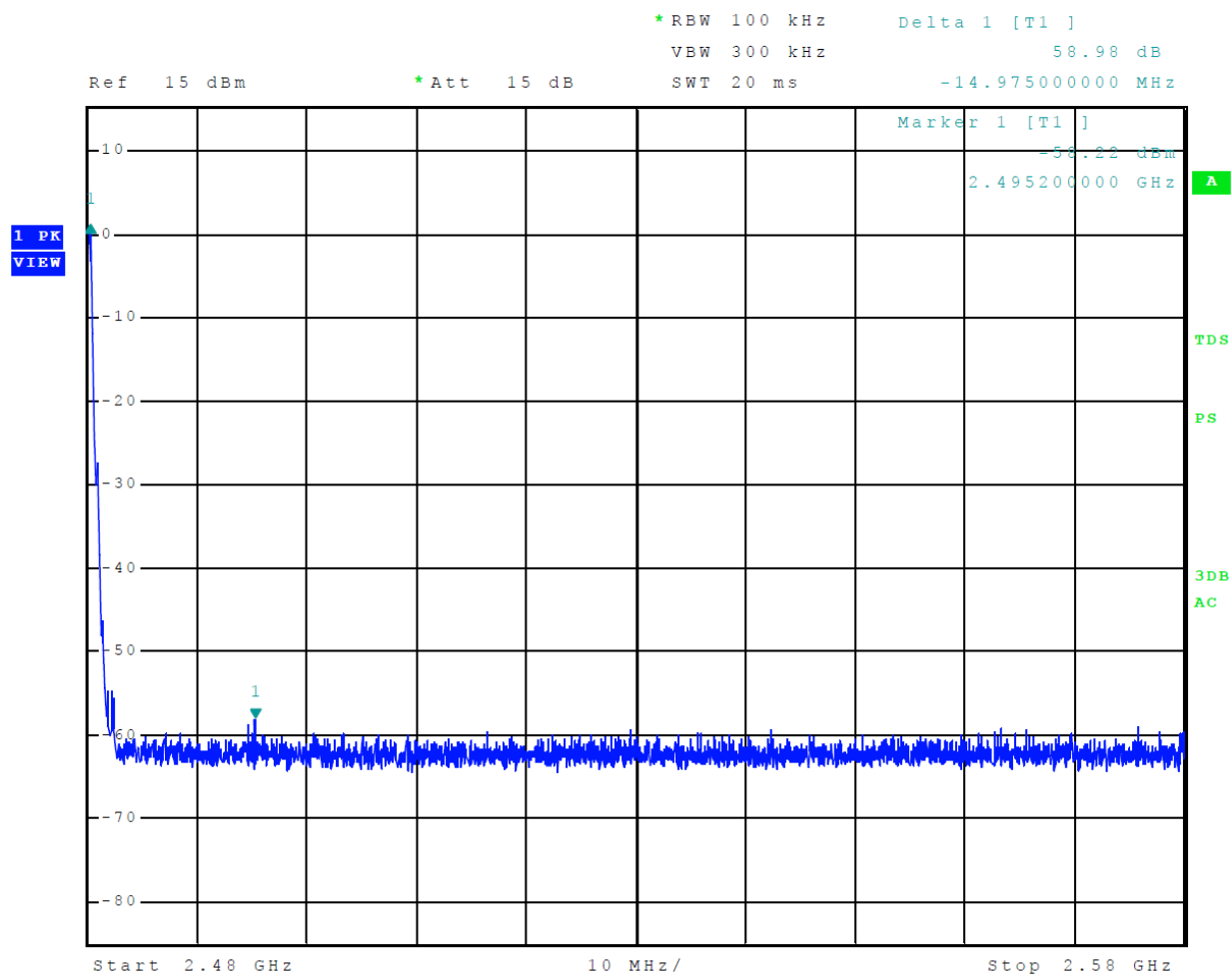
Figure 13 Plot of Transmitter Emissions High Band Edge Mode Mode 2, BT BLE (GMSK)
