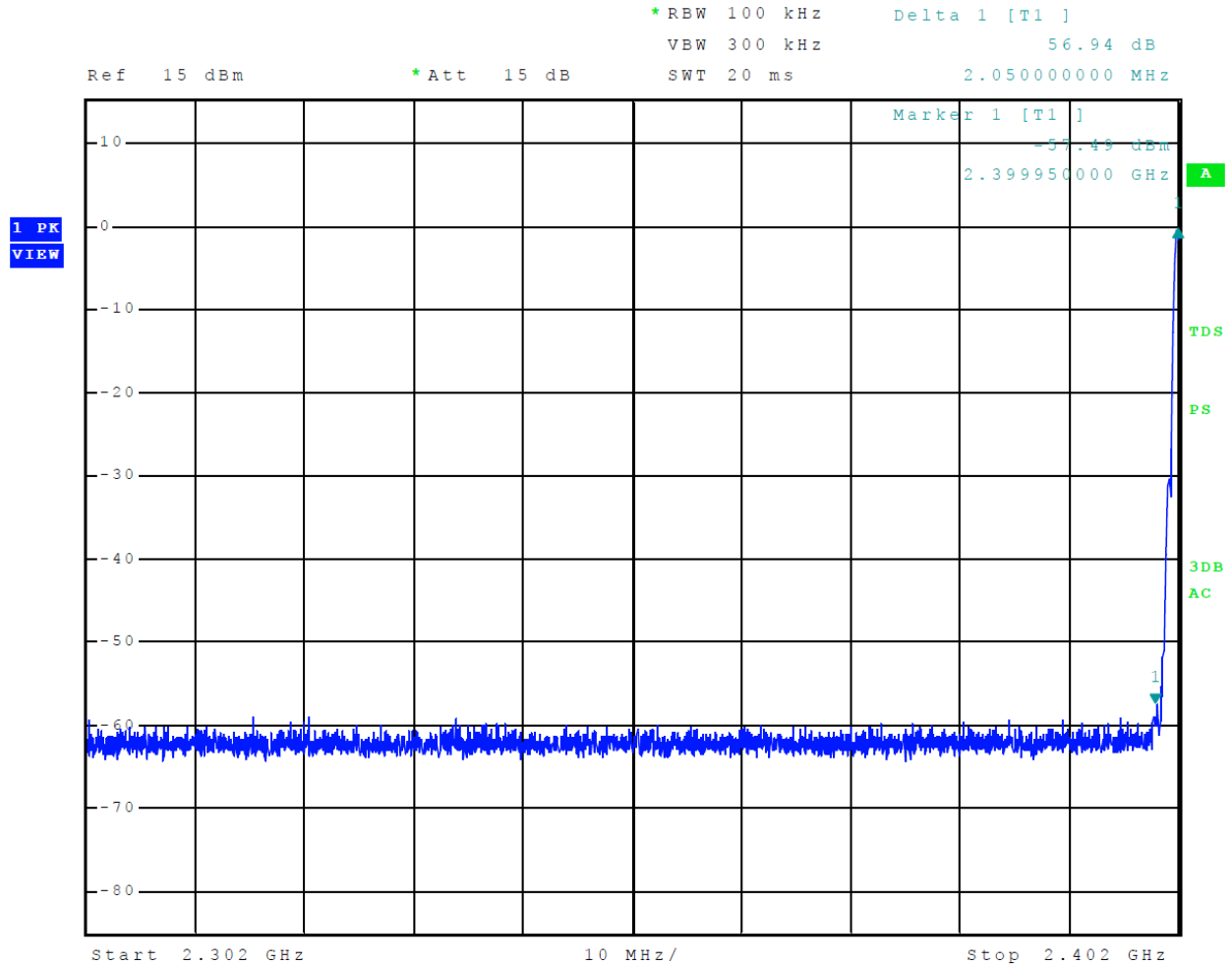
Figure 9 Plot of Emissions Low Band Edge Mode 2, BT BLE (GMSK)
