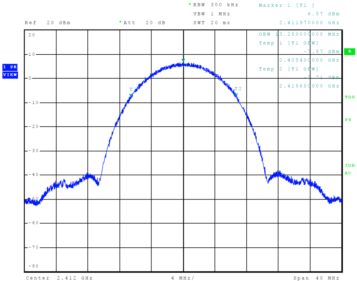
Figure 20 Plot of 99% Occupied Bandwidth Mode 3, 802.11b
