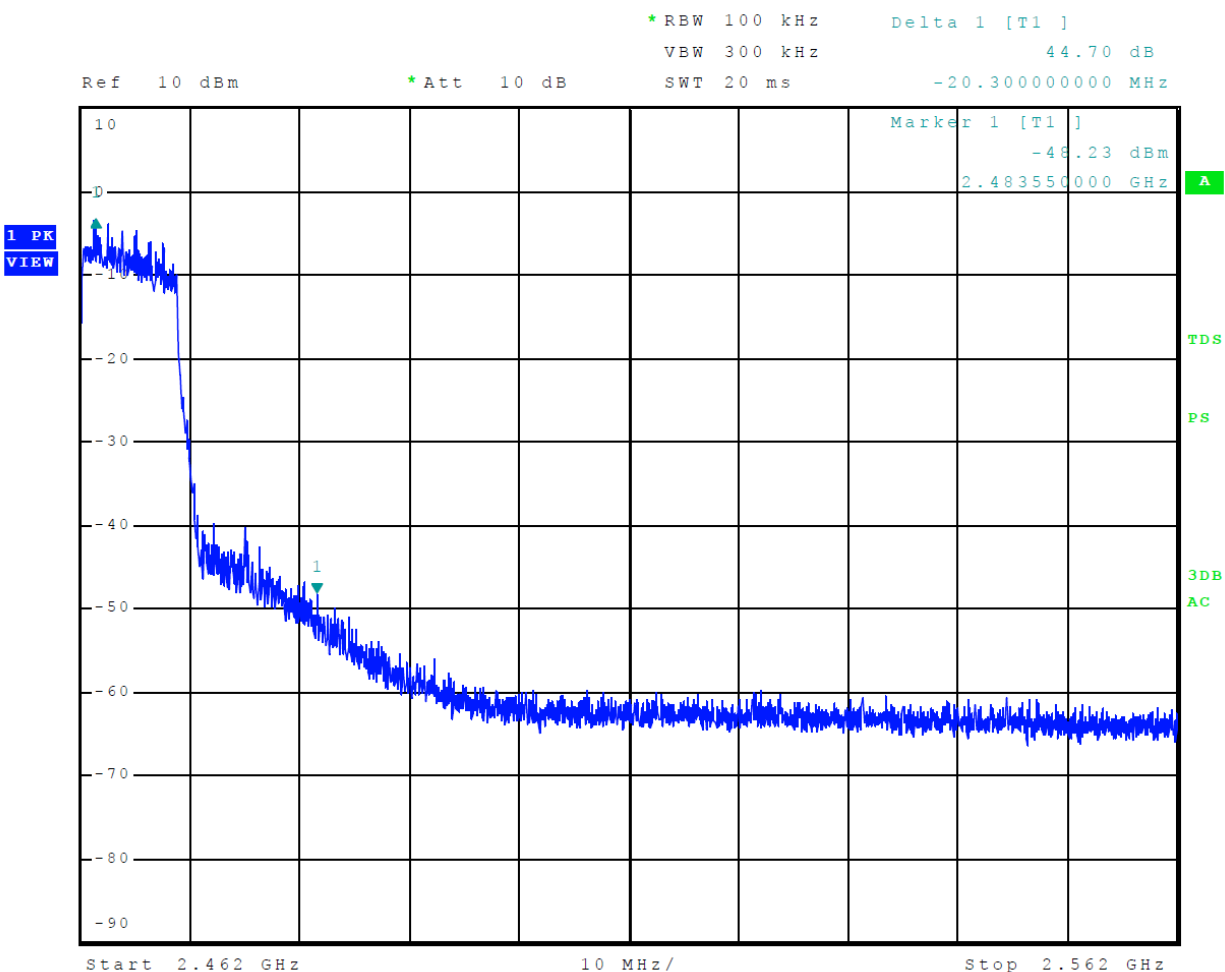
Figure 16 Plot of Transmitter Emissions High Band Edge Mode 5, 802.11n
