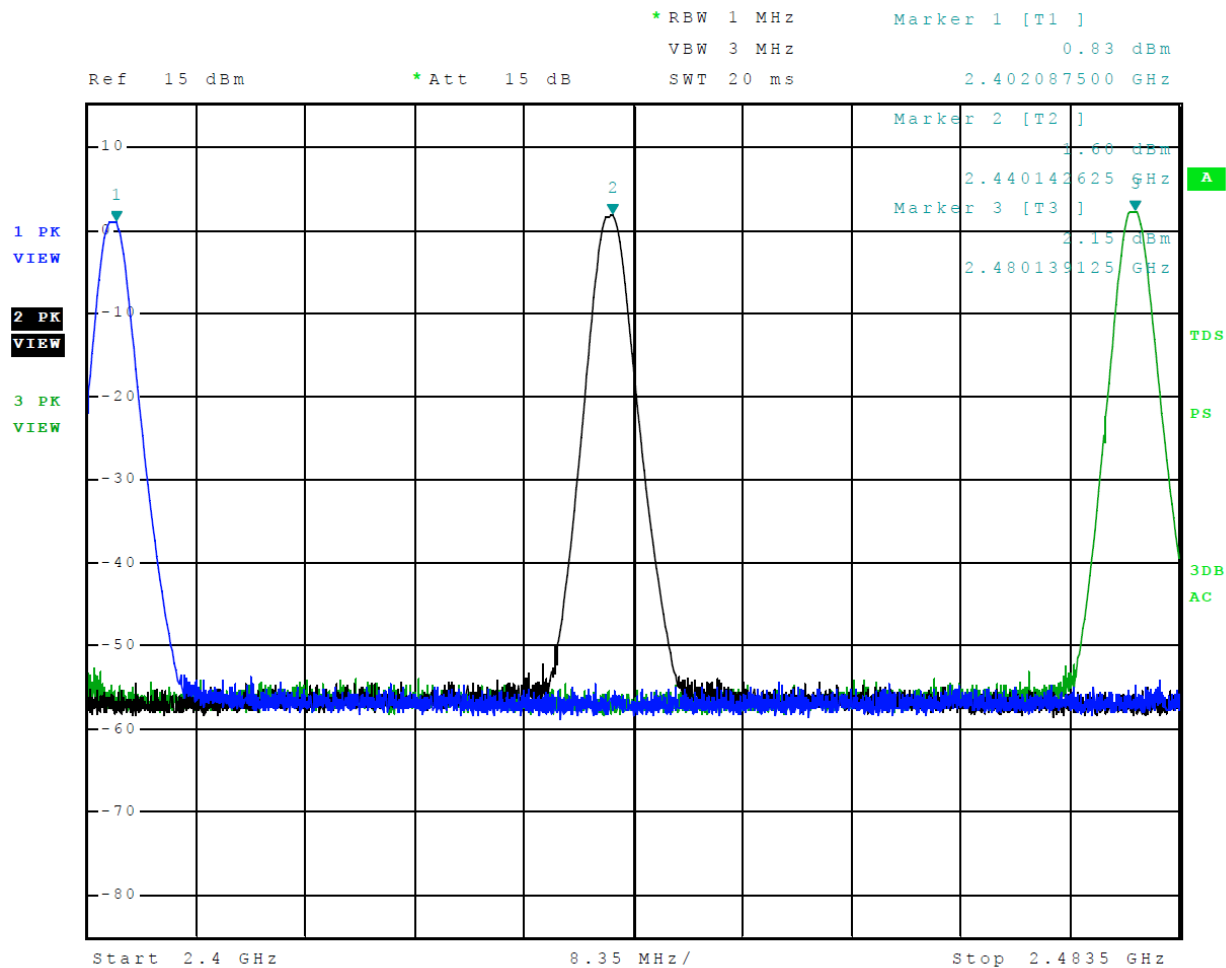
Figure 5 Plot of Transmitter Operation in 2402-2480 MHz Mode 2, BT BLE (GMSK)
