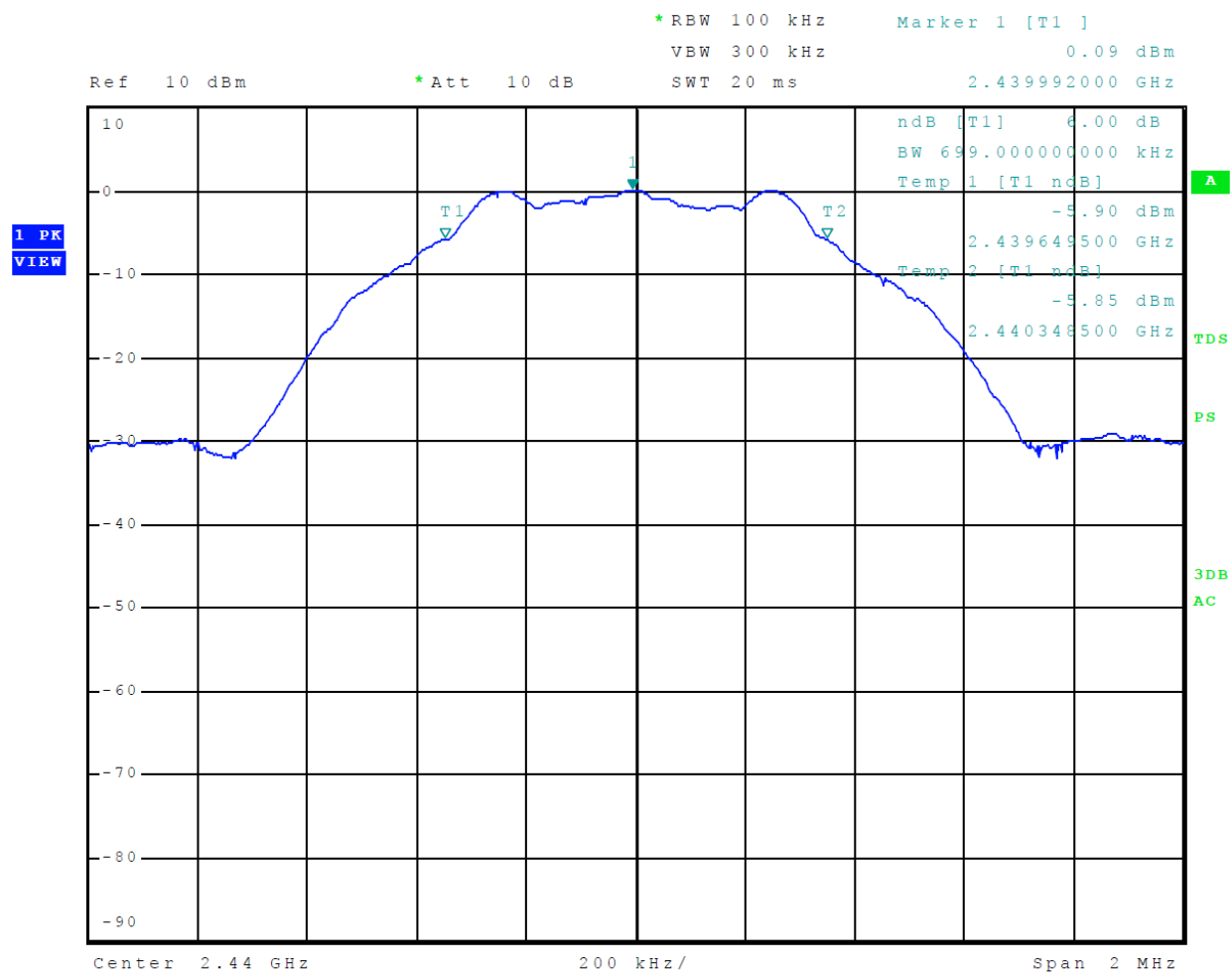
Figure 17 Plot of 6-dB Occupied Bandwidth Mode 2, BT BLE (GMSK)
