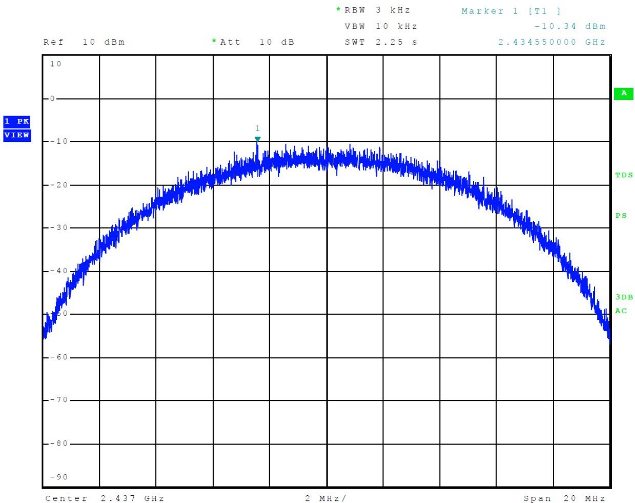
Figure 26 Plot of Transmitter Power Spectral Density Mode 3, 802.11b
