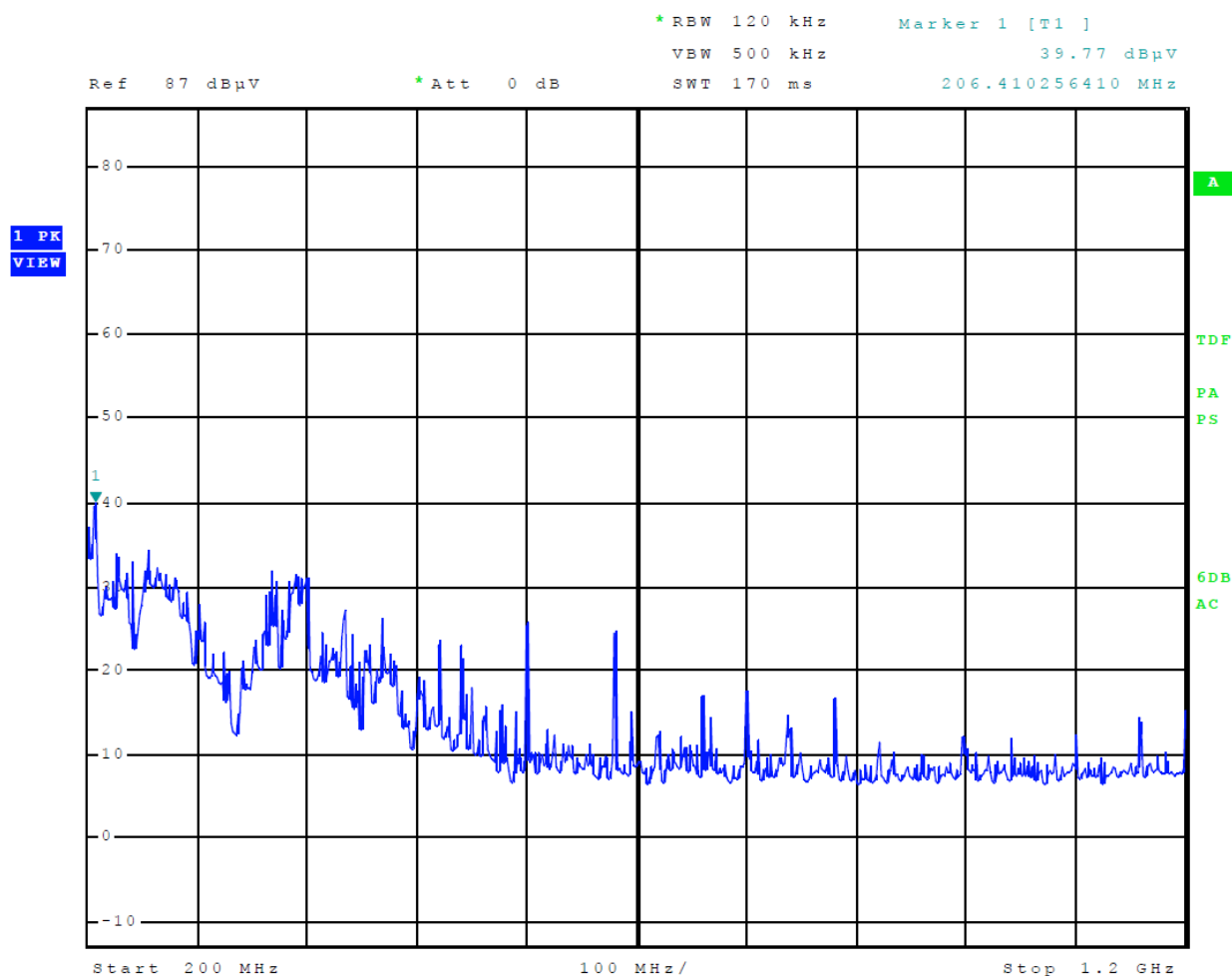
Figure 2 Plot of General Radiated Emissions (200 MHz – 1.2 GHz)
