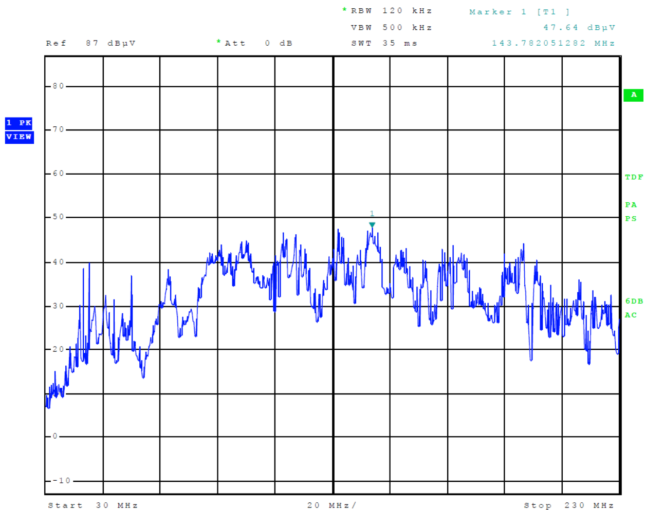
Figure 1 Plot of General Radiated Emissions (30 MHz – 230 MHz)
