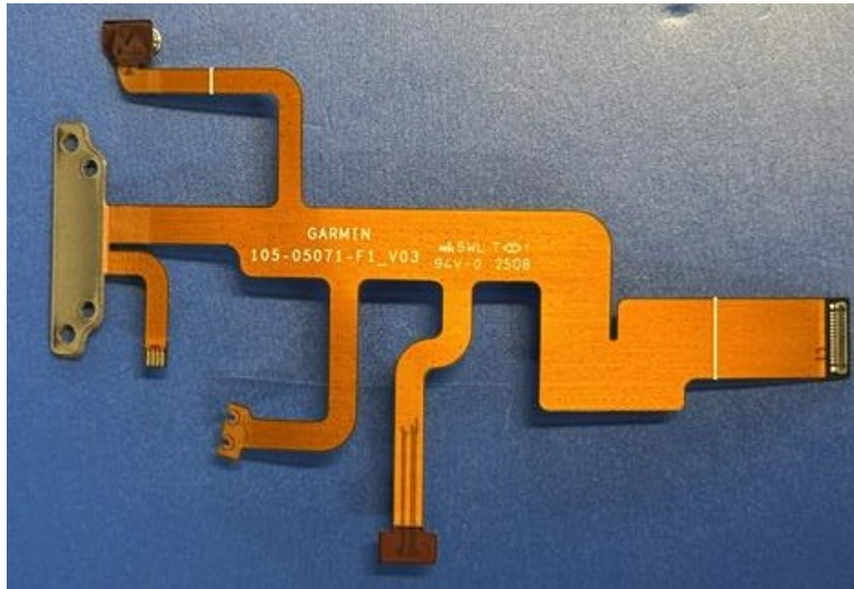
Front FPCBA#2
