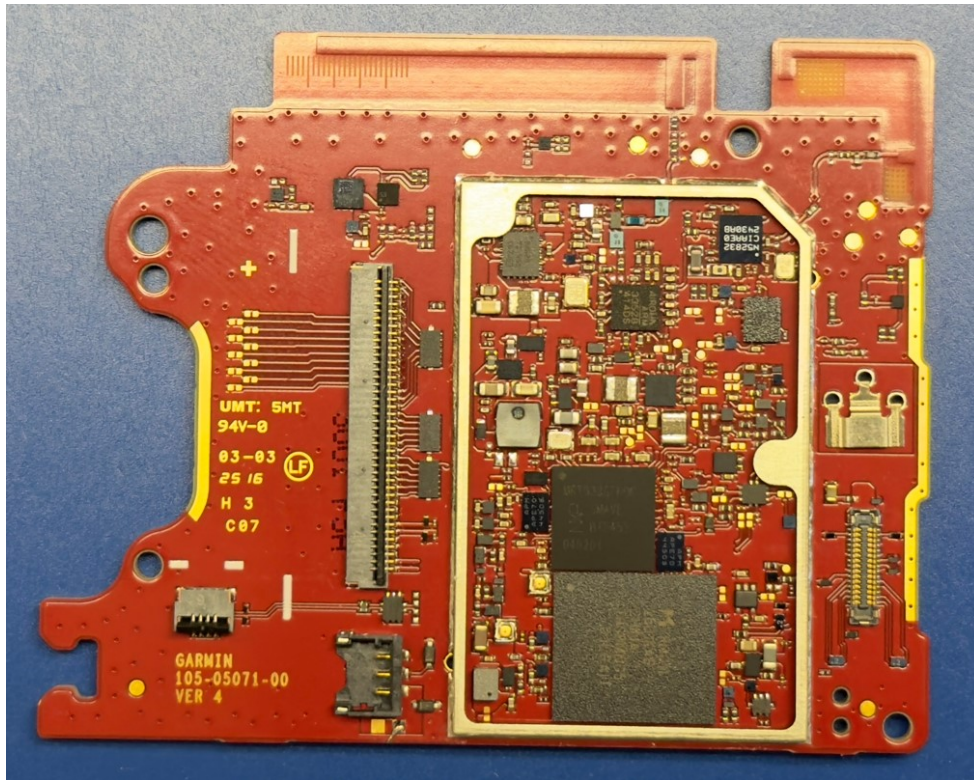
Front PCBA#2
