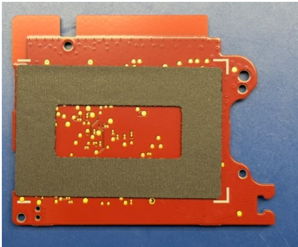
Rear: PCBA#1
