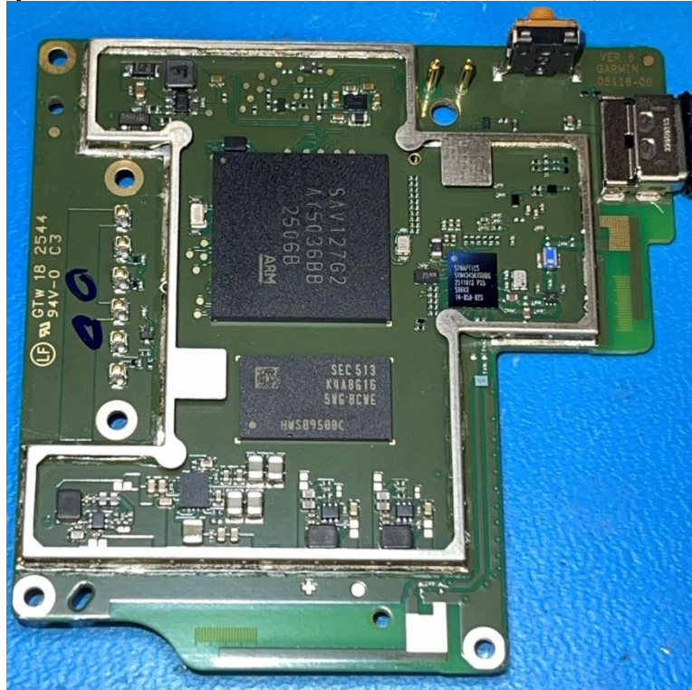
Photograph 07-3: Back side view of the main board, shield removed
