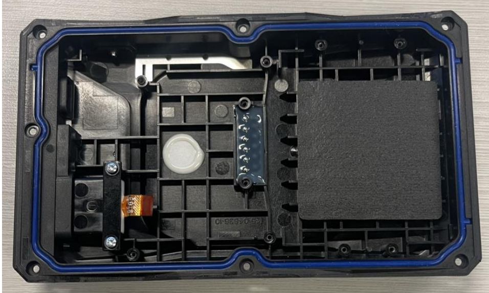
Photograph 07-5: Lower enclosure components – battery removed
