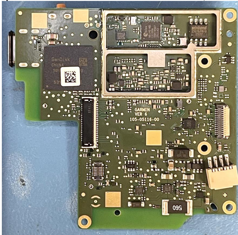
Photograph 07-2: Front side view of the main board, shield removed
