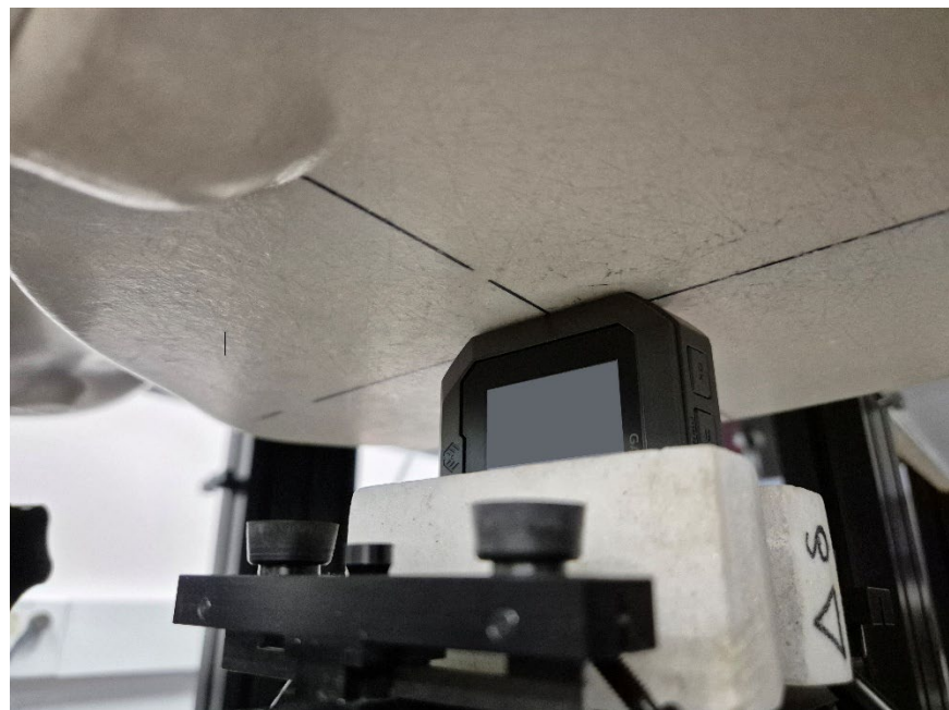
Figure 6 SAR Test Setup – Body/Extremity – Left Edge 0mm
