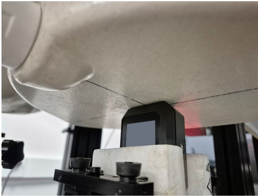
Figure 5 SAR Test Setup – Body/Extremity – Right Edge 0mm
