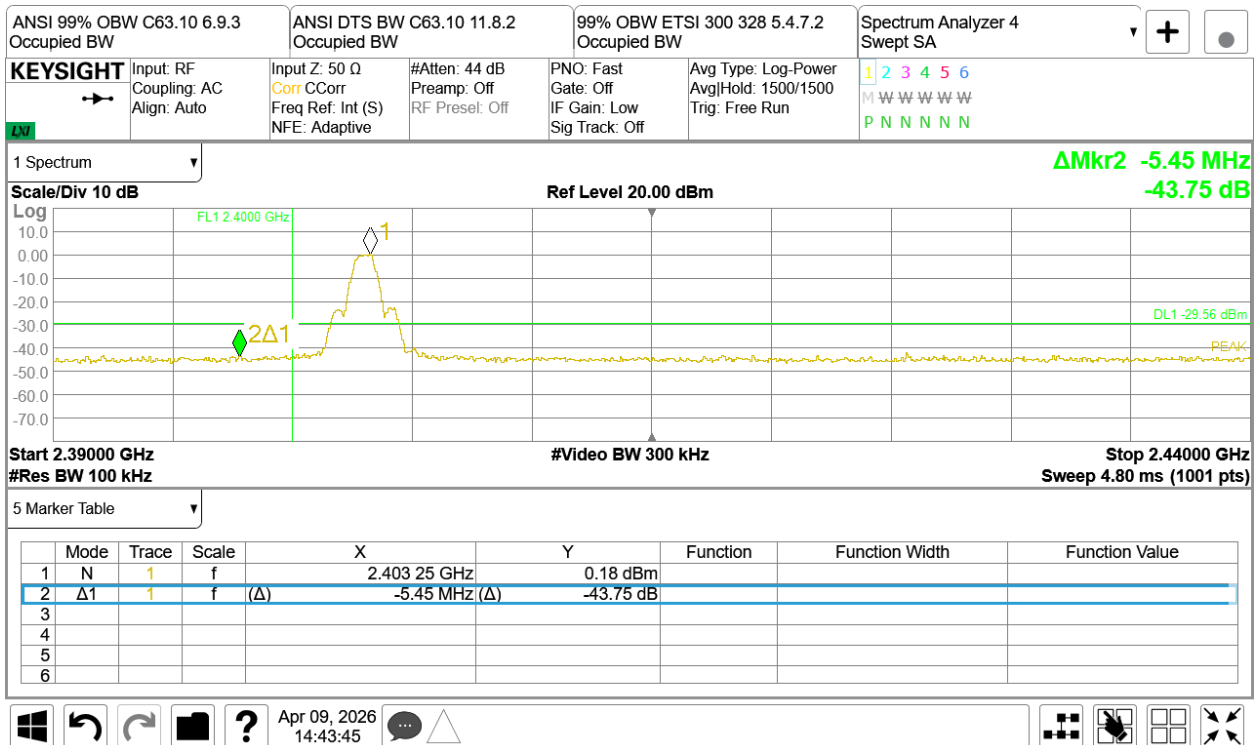
Figure TR67.6: Band edge gap measurement for ANT, 2403 MHz
