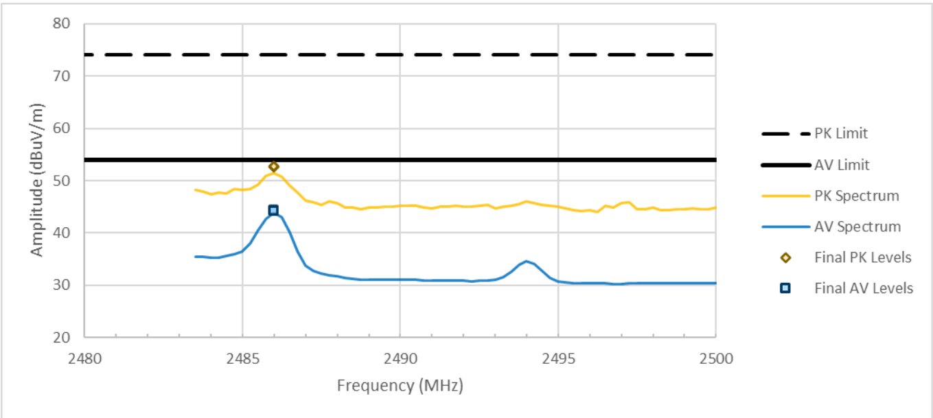
Figure RE06.2: FCC restricted band spectral data from 2483.5 to 2500 MHz (ANT, 2478 MHz)
