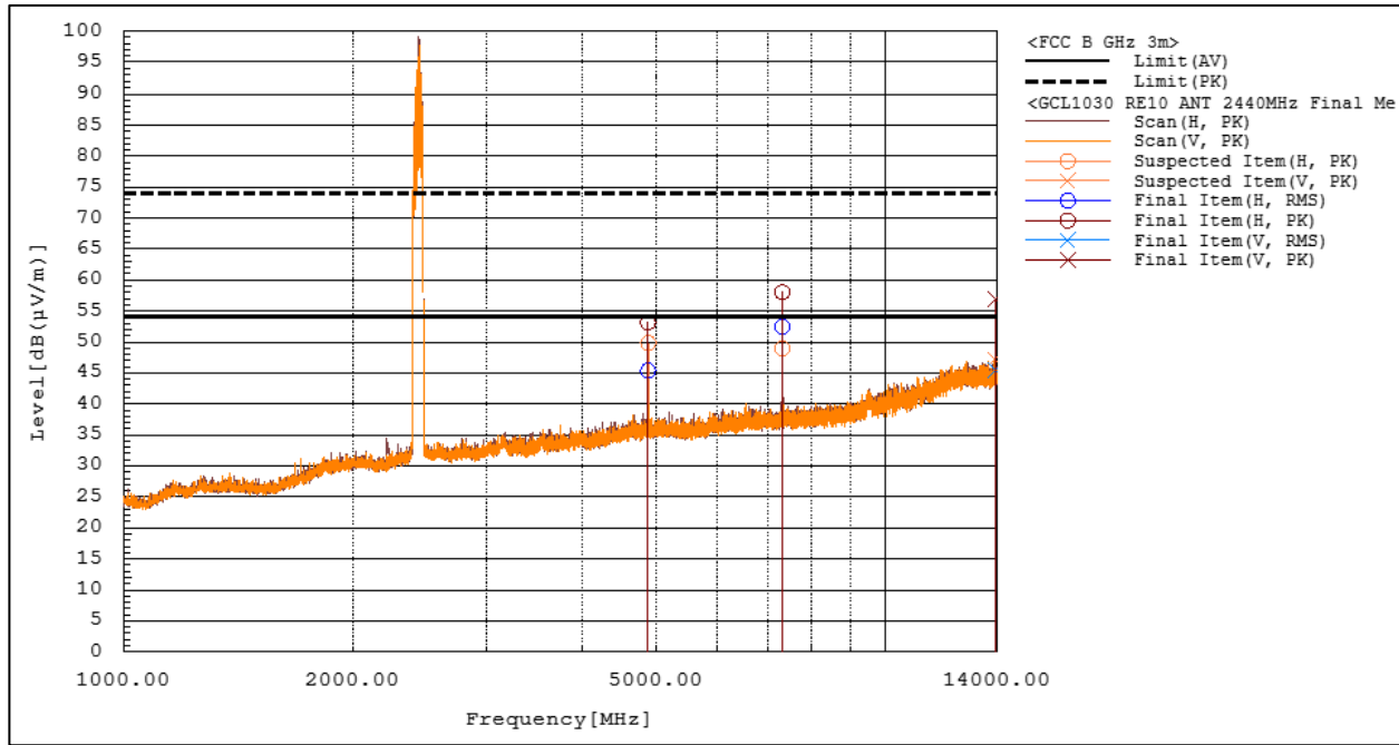
Figure RE10.2: Spectral data (ANT, 2440 MHz)
