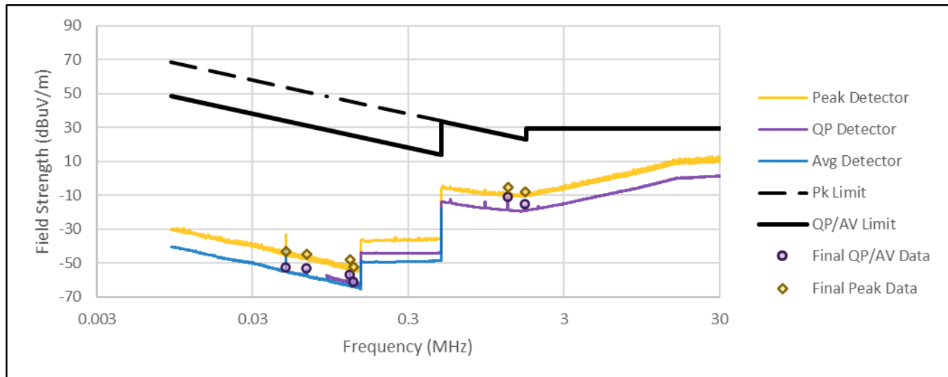
Figure RE29.1: Spectral data (ANT, 2440 MHz)
