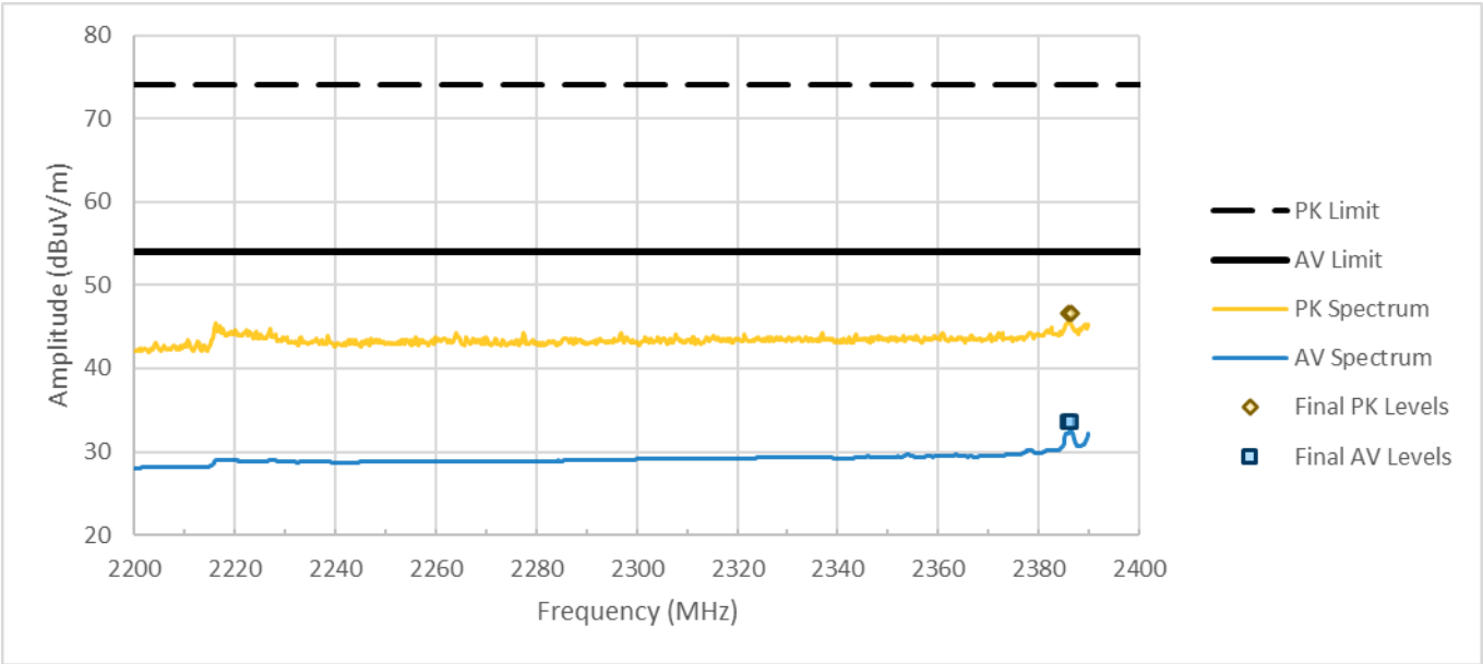
Figure RE06.1: FCC restricted band spectral data from 2200 to 2390 MHz (ANT, 2402 MHz)
