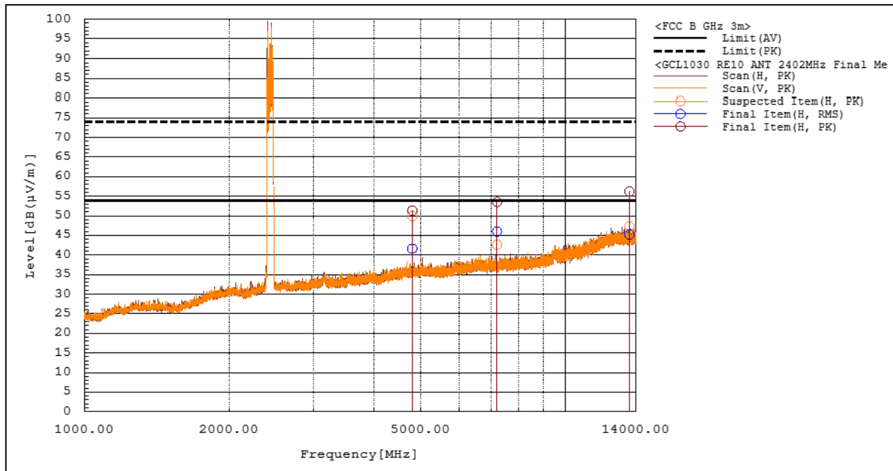
Figure RE10.1: Spectral data (ANT, 2402 MHz)
