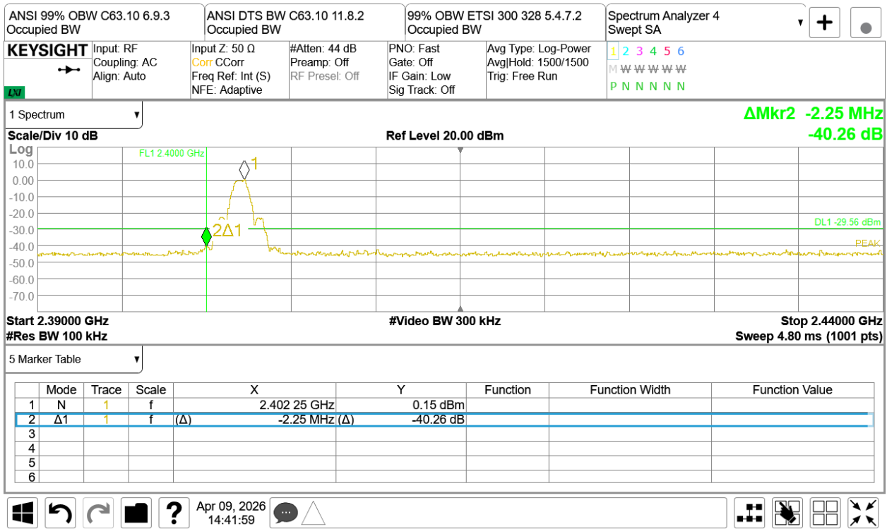
Figure TR67.5: Band edge gap measurement for ANT, 2402 MHz
