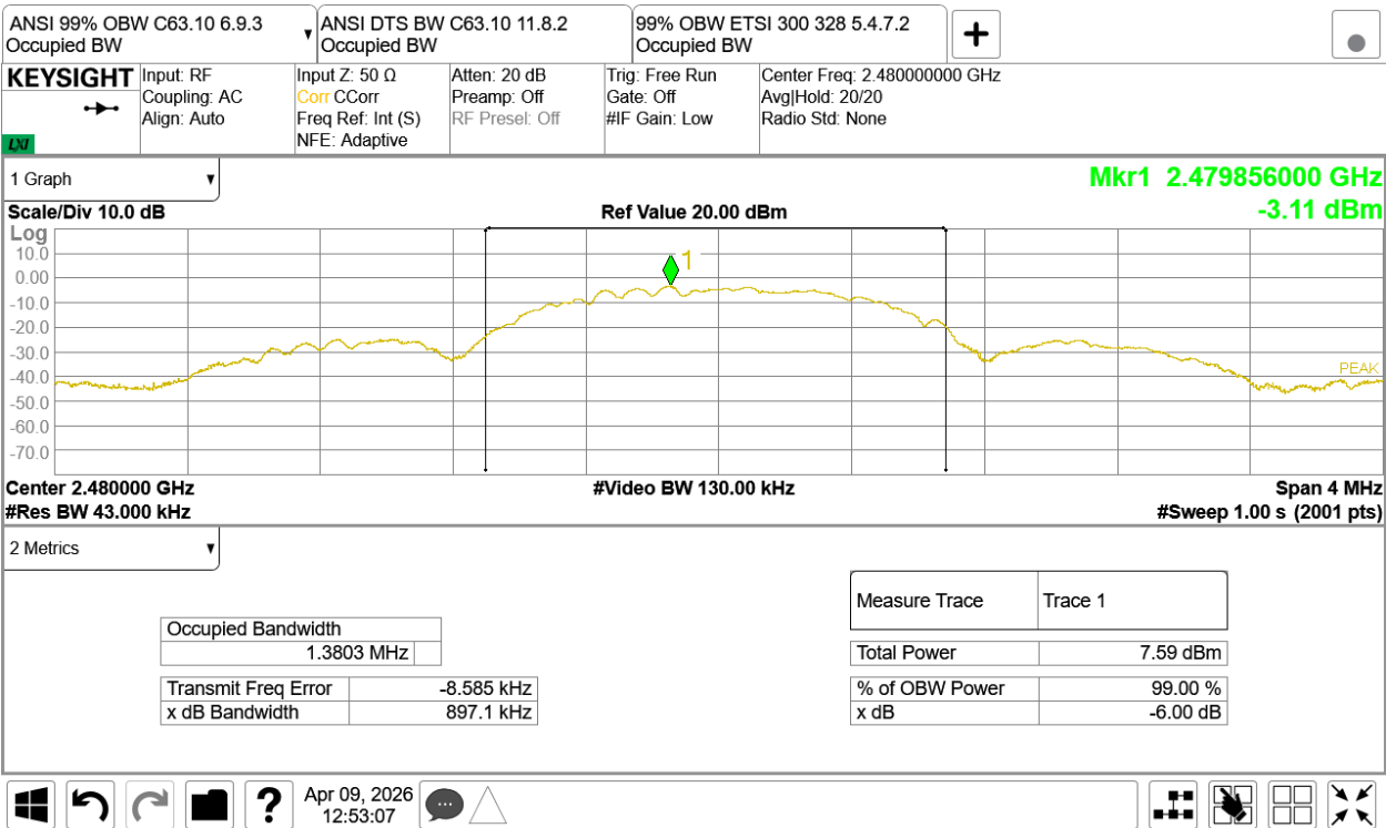
Figure TR35.1: Occupied bandwidth data for ANT at high channel (2480 MHz)
