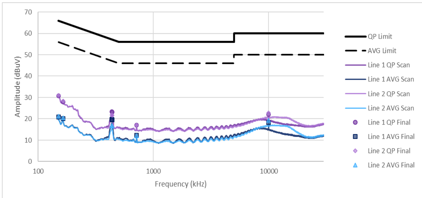
Figure CE03.1: Spectral data (ANT, 2440 MHz)
