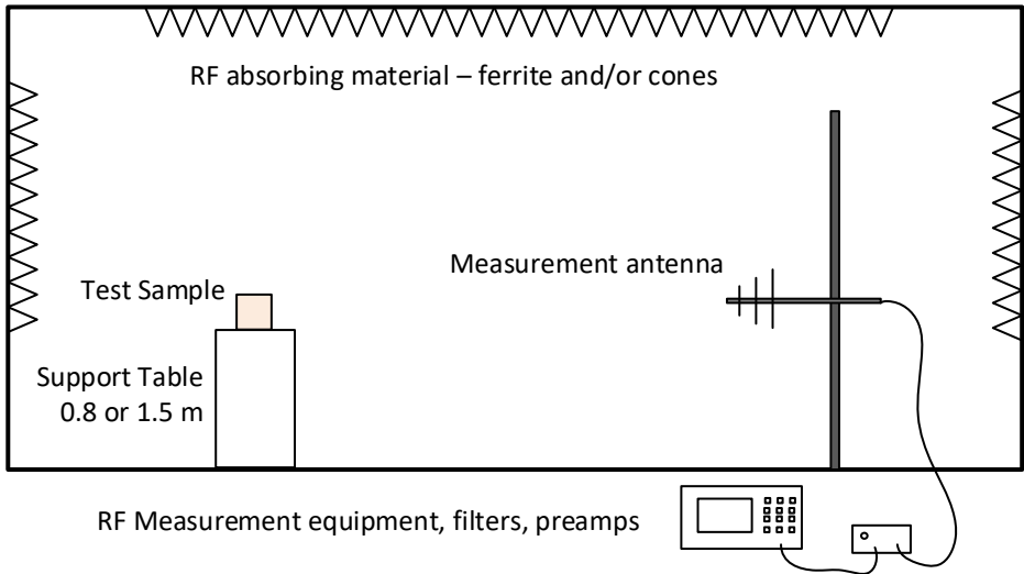
Figure 1: Typical configuration for measurements below 1 GHz
