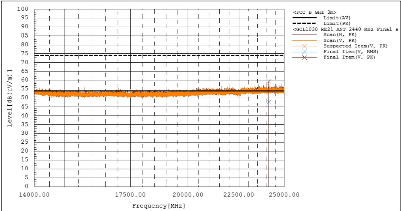
Figure RE21.1: Spectral data (3 meter, 2440 MHz)
