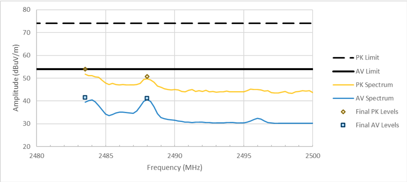
Figure RE06.3: FCC restricted band spectral data from 2483.5 to 2500 MHz (ANT, 2480 MHz)
