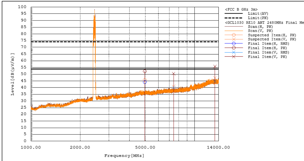
Figure RE10.3: Spectral data (ANT, 2480 MHz)
