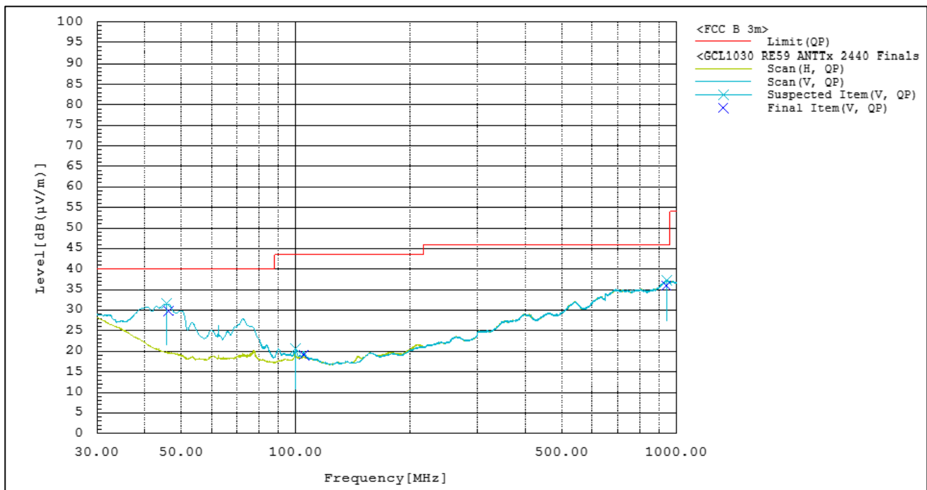
Figure RE59.1: Spectral data (ANT, 2440 MHz)
