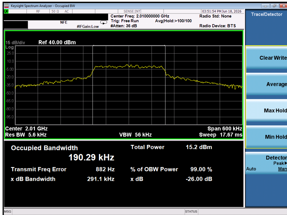
Plot 7-2. Occupied Bandwidth Plot (Band 23/255, Mid Channel) - QPSK
