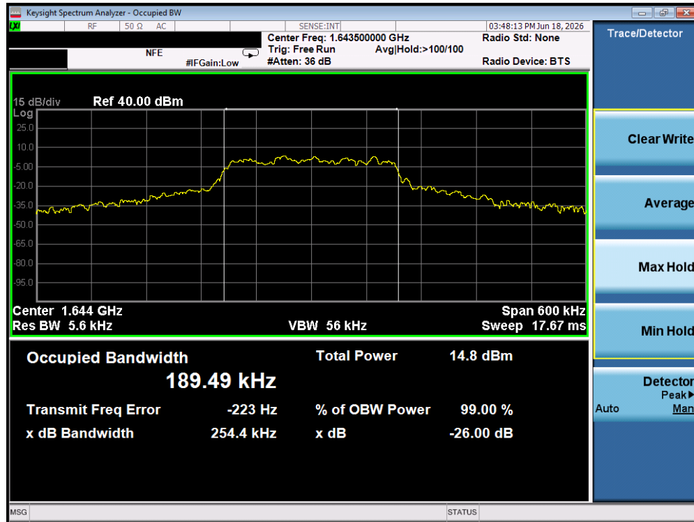
Plot 7-1. Occupied Bandwidth Plot (Band 255, Mid Channel) - QPSK
