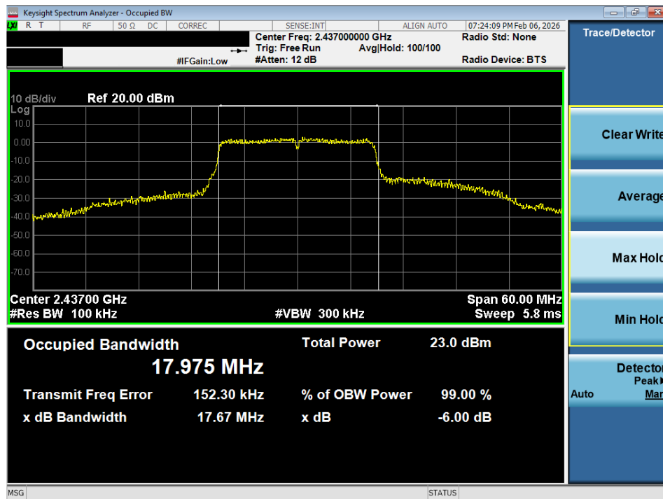
Plot 7-8 6dB BW (20MHz BW 802.11n - Ch.6)
