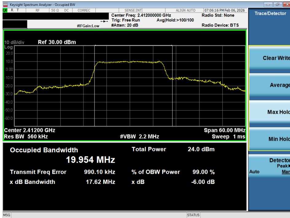
Plot 7-15 99% OBW Plot (20MHz BW 802.11n - Ch.1)
