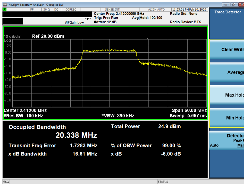
Plot 7-12 99% OBW Plot (20MHz BW 802.11g - Ch.1)
