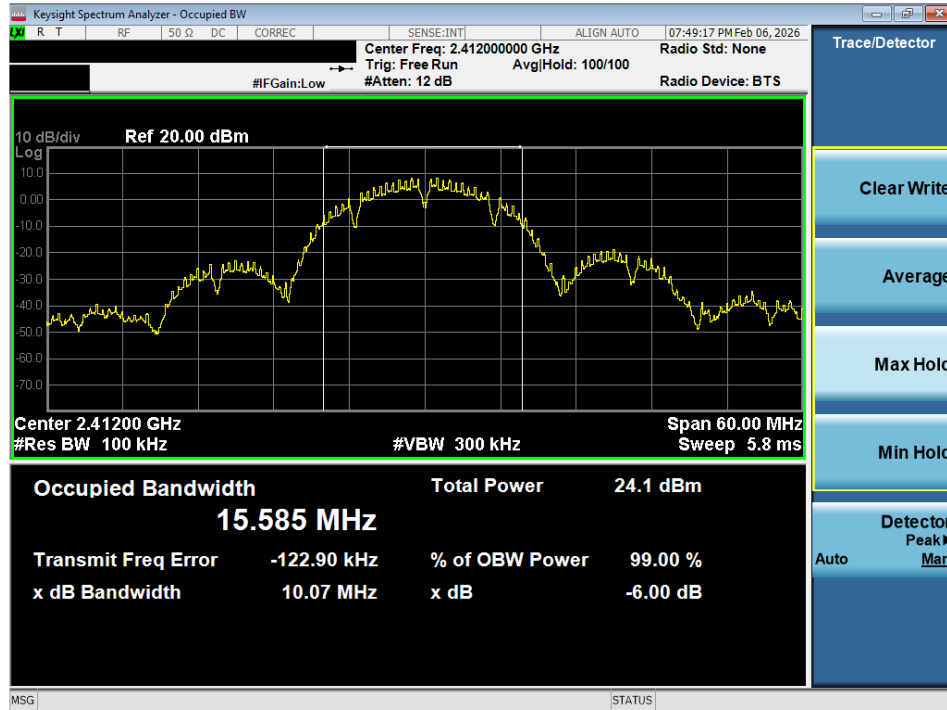
Plot 7-1 6dB BW (20MHz BW 802.11b - Ch.1)
