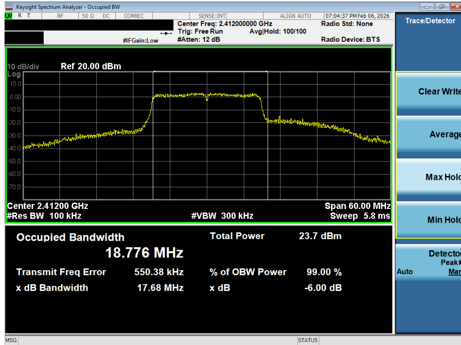
Plot 7-7 6dB BW (20MHz BW 802.11n - Ch.1)
