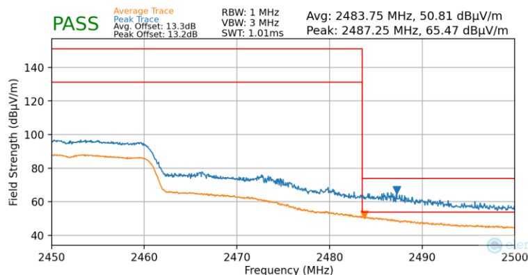
Plot 7-65. Radiated Restricted Upper Band Edge Measurement (Average & Peak)
