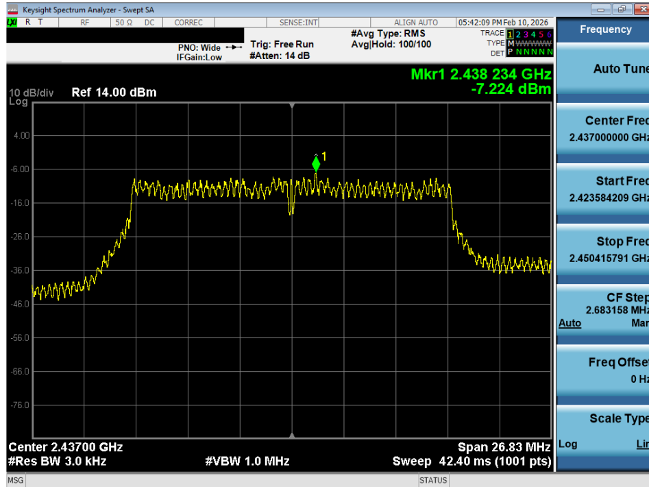
Plot 7-22 PSD (20MHz BW 802.11g - Ch.6)
