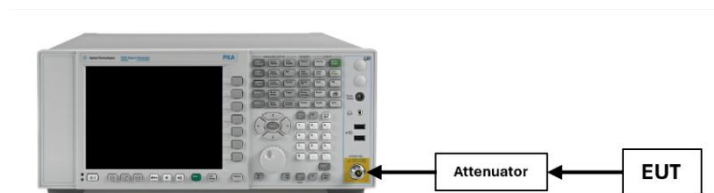
Figure 7-5. Test Instrument & Measurement Setup
