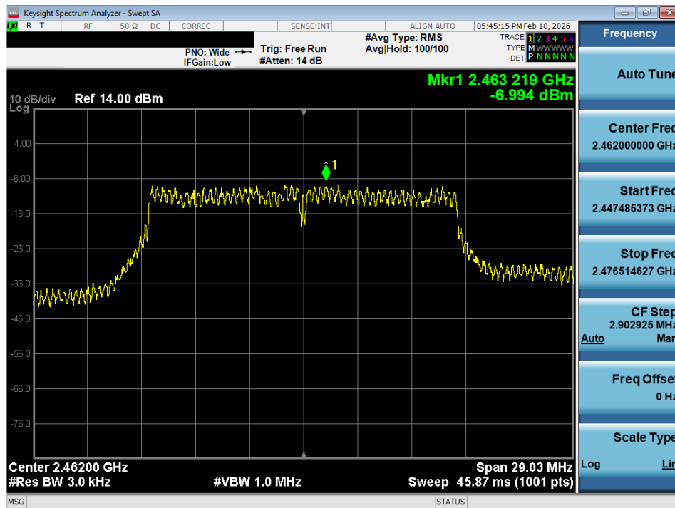
Plot 7-23 PSD (20MHz BW 802.11g - Ch.11)
