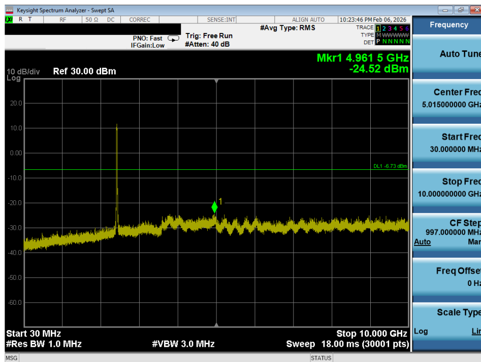
Plot 7-55. Conducted Spurious Plot (802.11n – Ch. 6)
