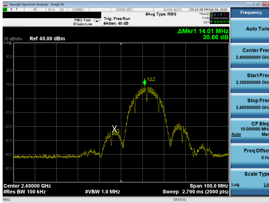
Plot 7-27. Band Edge Plot (802.11b – Ch. 1)
