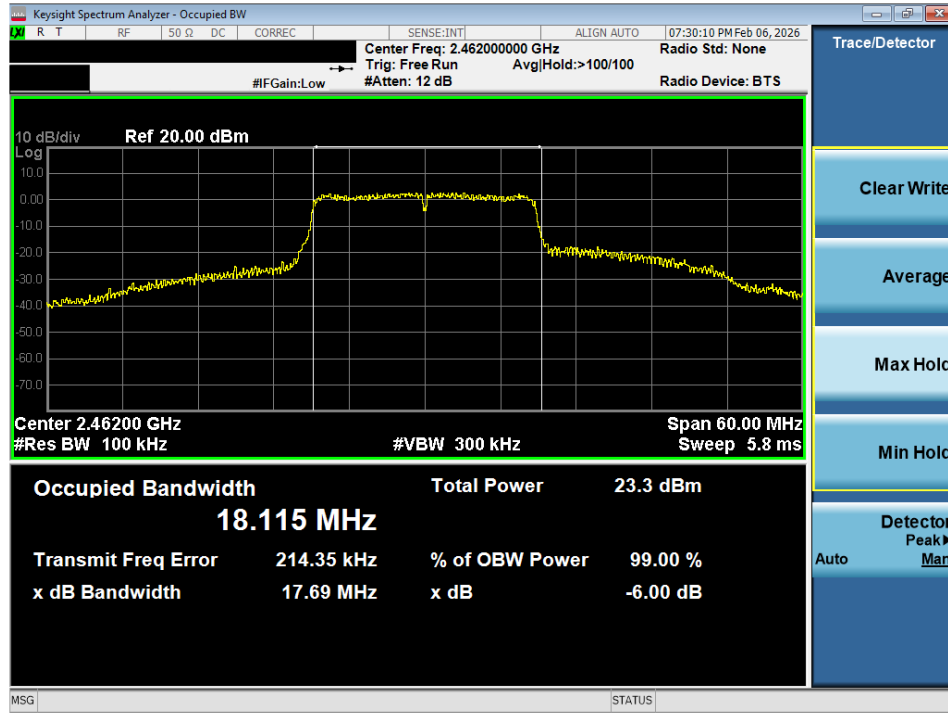
Plot 7-9 6dB BW (20MHz BW 802.11n - Ch.11)
