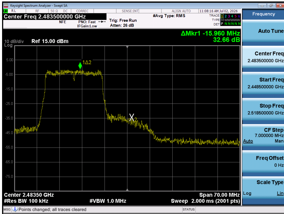
Plot 7-39. Band Edge Plot (802.11n (2.4GHz) – Ch. 12)
