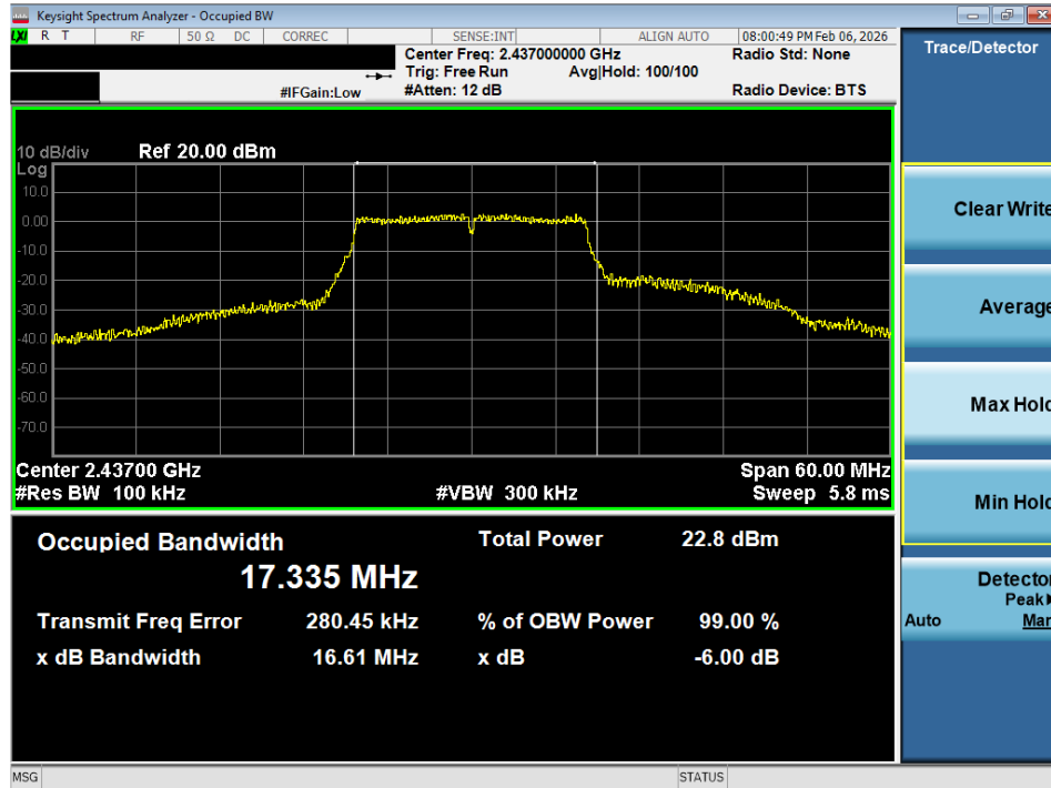
Plot 7-5 6dB BW (20MHz BW 802.11g - Ch.6)
