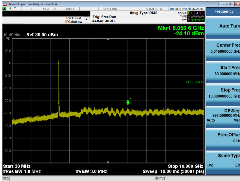
Plot 7-57. Conducted Spurious Plot (802.11n – Ch. 11)
