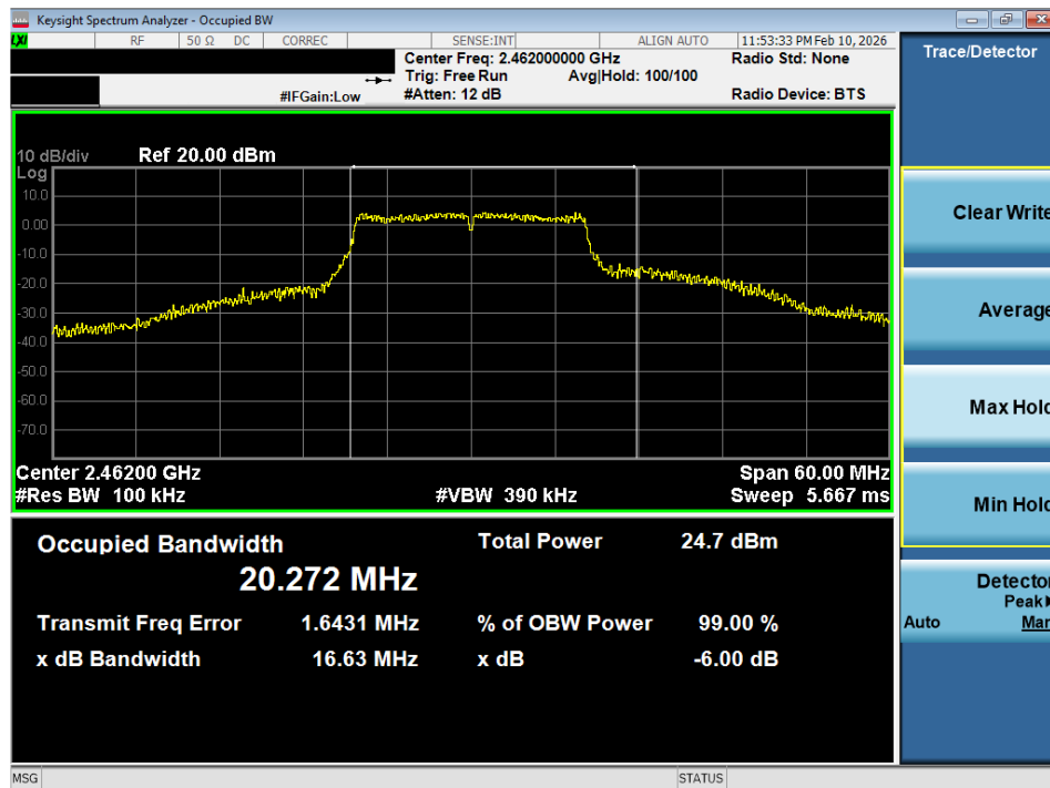
Plot 7-14 99% OBW Plot (20MHz BW 802.11g - Ch.11)
