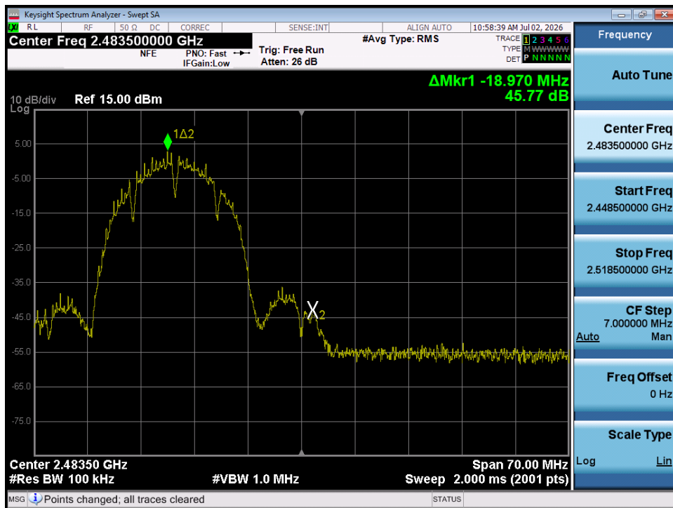
Plot 7-30. Band Edge Plot (802.11b – Ch. 12)
