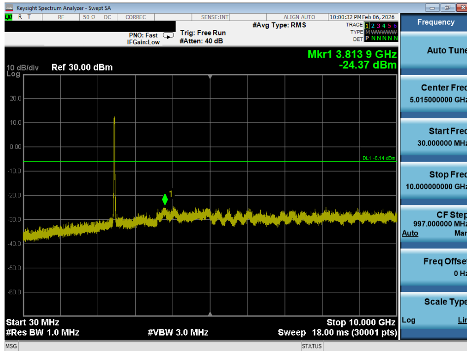
Plot 7-51. Conducted Spurious Plot (802.11g – Ch. 11)
