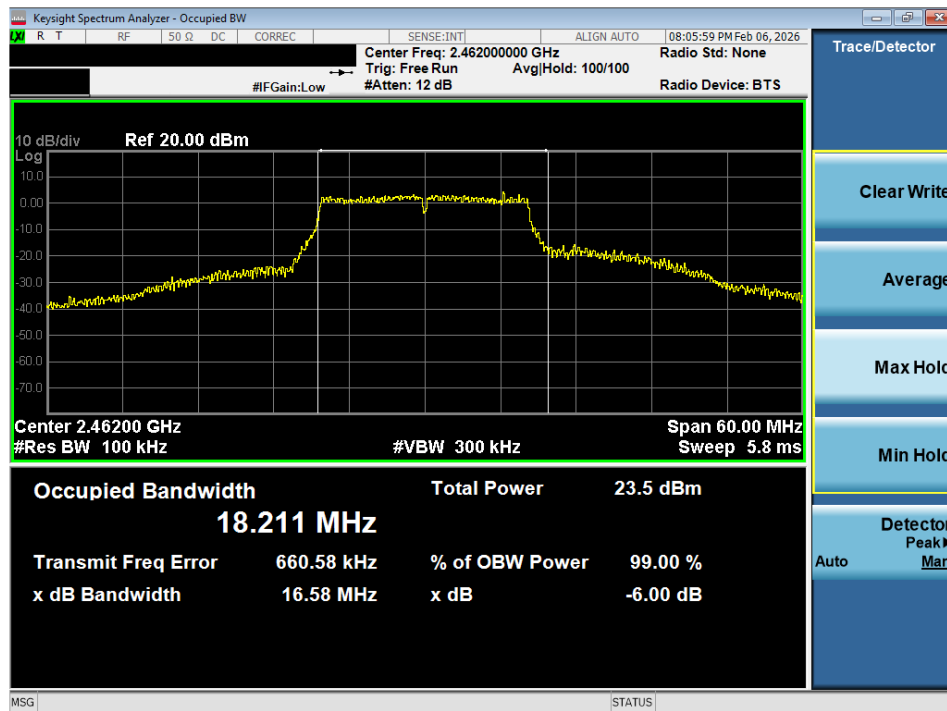
Plot 7-6 6dB BW (20MHz BW 802.11g - Ch.11)
