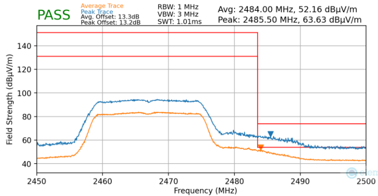
Plot 7-68. Radiated Restricted Upper Band Edge Measurement (Average & Peak)
