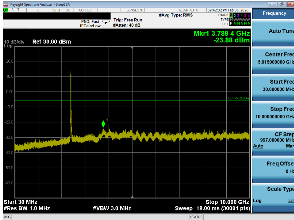
Plot 7-47. Conducted Spurious Plot (802.11g – Ch. 1)
