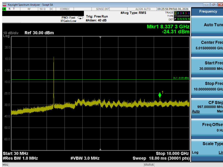
Plot 7-41. Conducted Spurious Plot (802.11b – Ch. 1)
