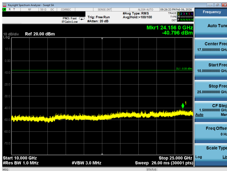
Plot 7-42. Conducted Spurious Plot (802.11b – Ch. 1)
