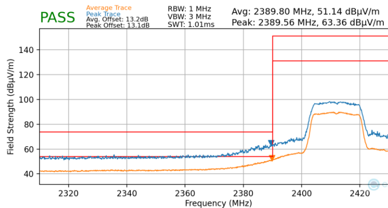
Plot 7-64. Radiated Restricted Lower Band Edge Measurement (Average & Peak)
