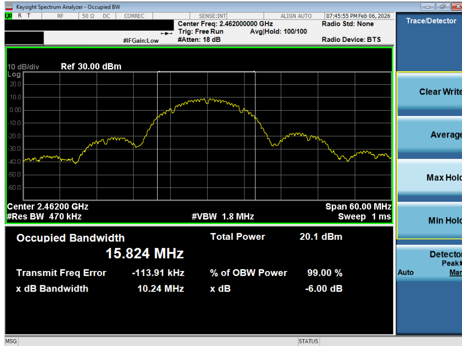
Plot 7-11 99% OBW Plot (20MHz BW 802.11b - Ch.11)
