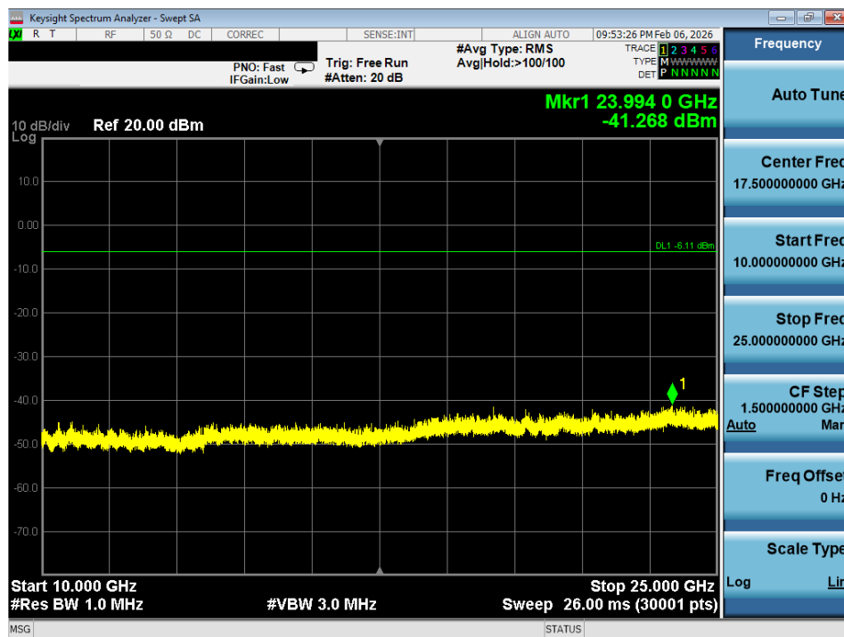
Plot 7-50. Conducted Spurious Plot (802.11g – Ch. 6)
