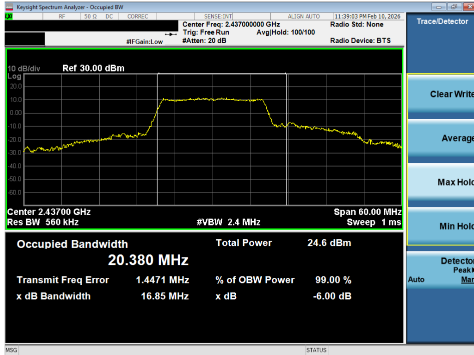
Plot 7-13 99% OBW Plot (20MHz BW 802.11g - Ch.6)
