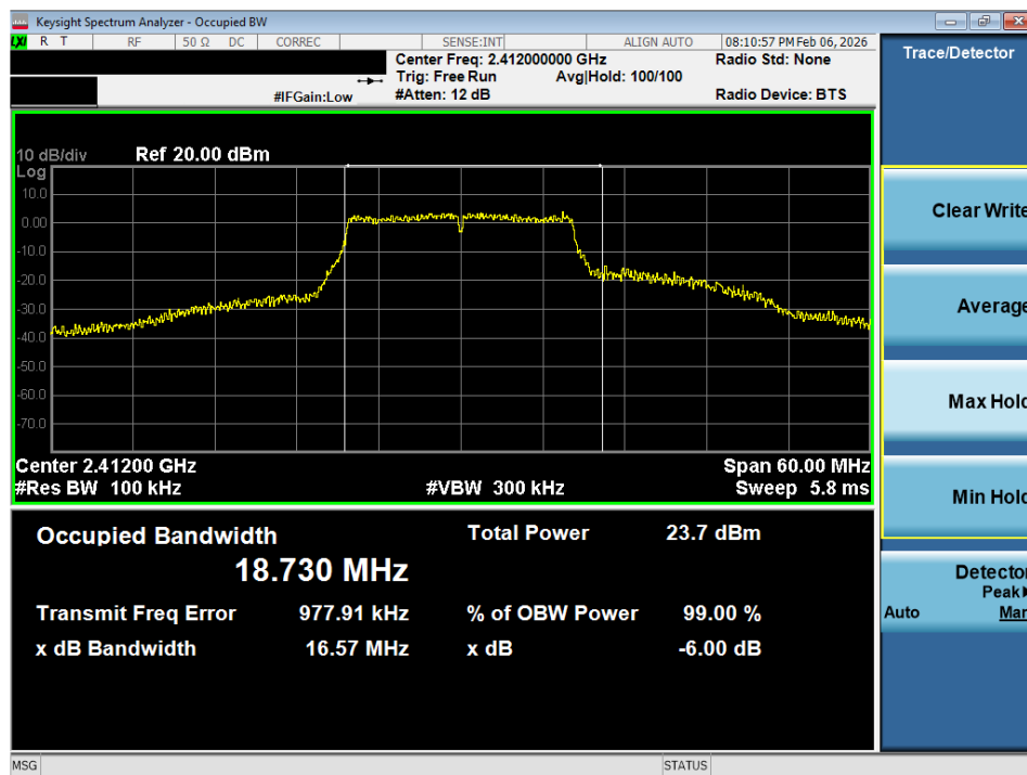
Plot 7-4 6dB BW (20MHz BW 802.11g - Ch.1)
