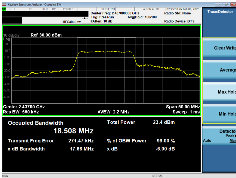
Plot 7-16 99% OBW Plot (20MHz BW 802.11n - Ch.6)
