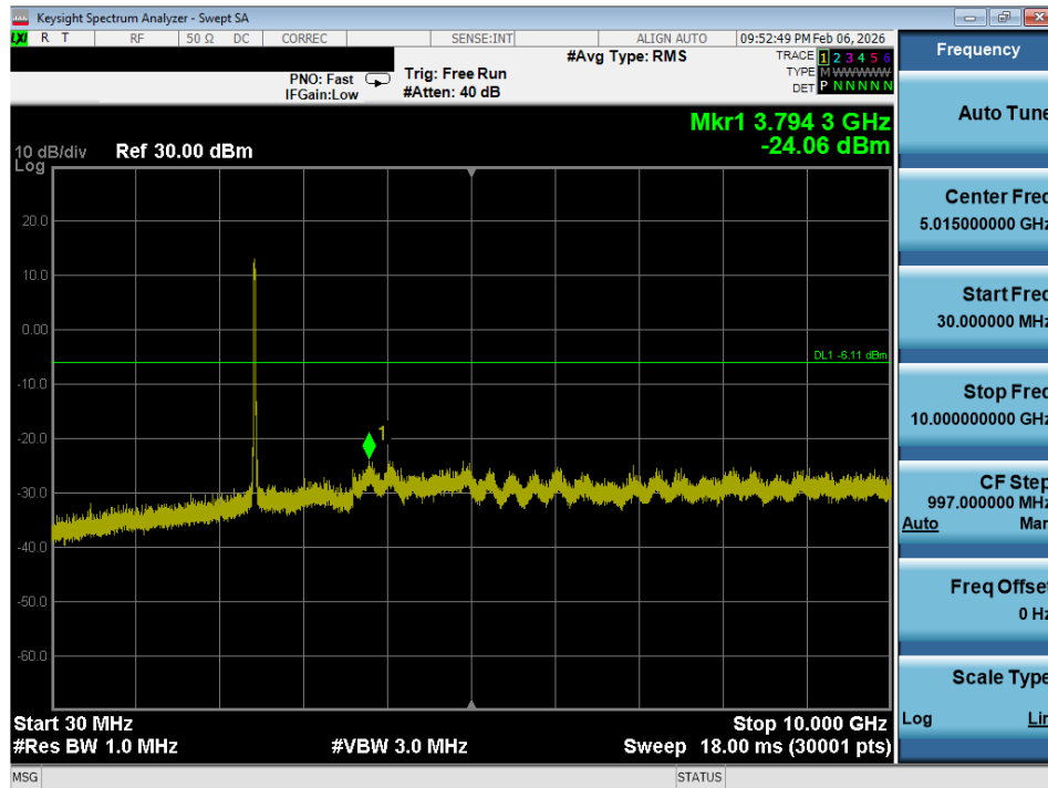
Plot 7-49. Conducted Spurious Plot (802.11g – Ch. 6)
