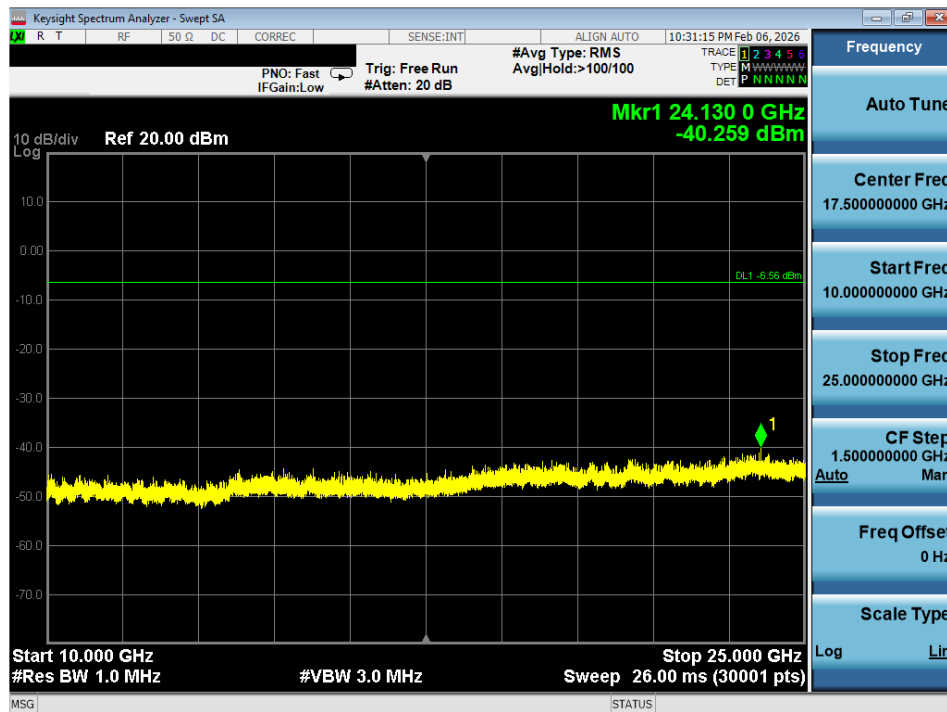
Plot 7-58. Conducted Spurious Plot (802.11n – Ch. 11)
