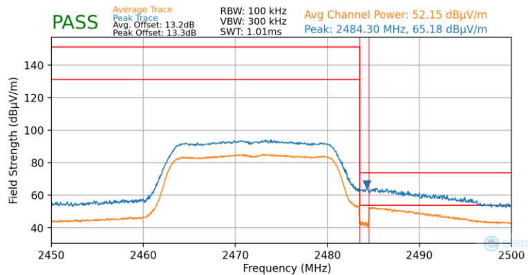
Plot 7-69. Radiated Restricted Upper Band Edge Measurement (Average & Peak)
