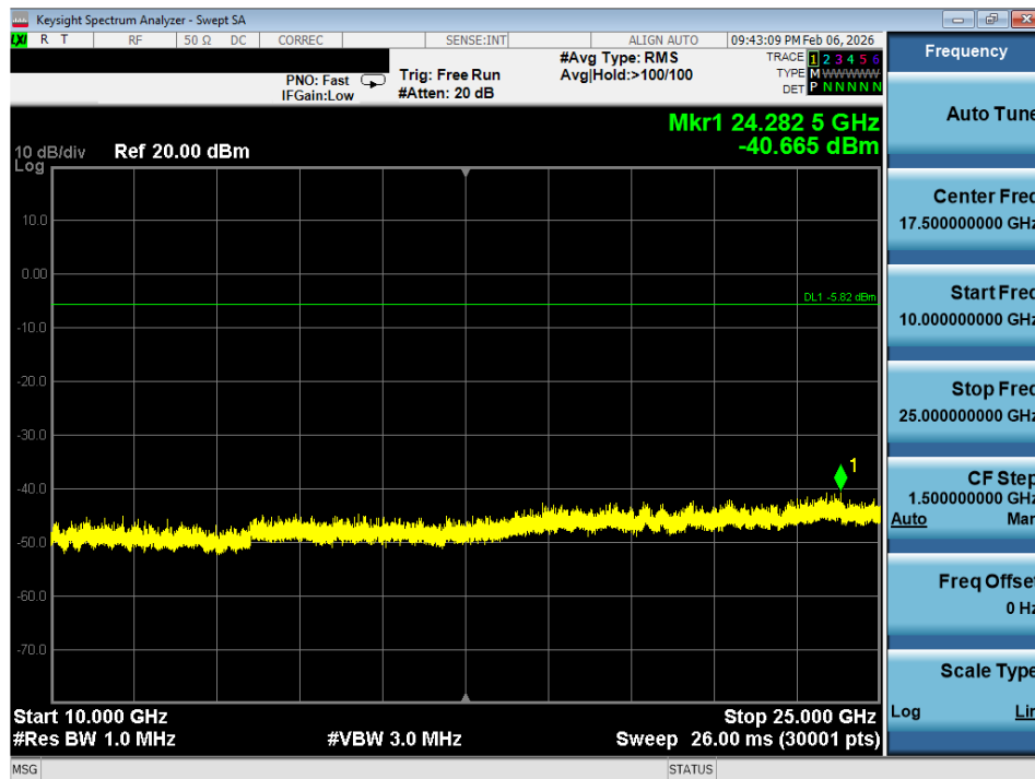
Plot 7-48. Conducted Spurious Plot (802.11g – Ch. 1)
