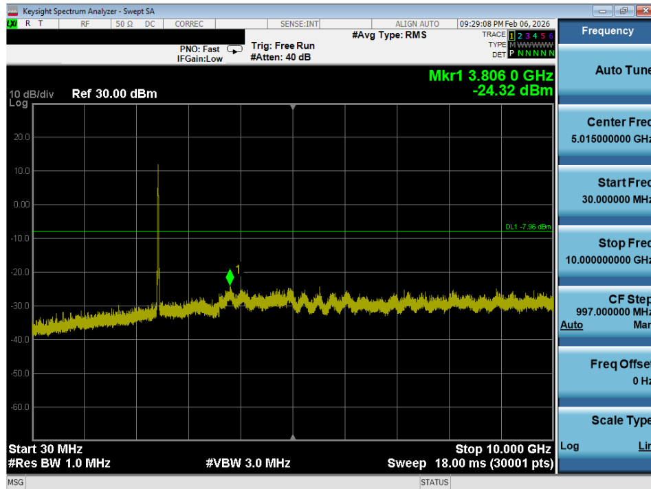
Plot 7-43. Conducted Spurious Plot (802.11b – Ch. 6)
