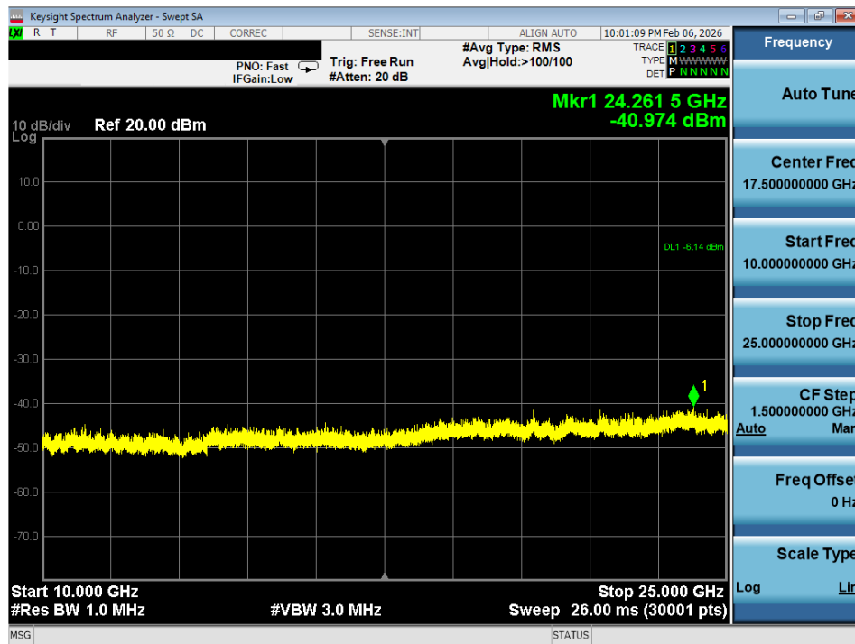
Plot 7-52. Conducted Spurious Plot (802.11g – Ch. 11)
