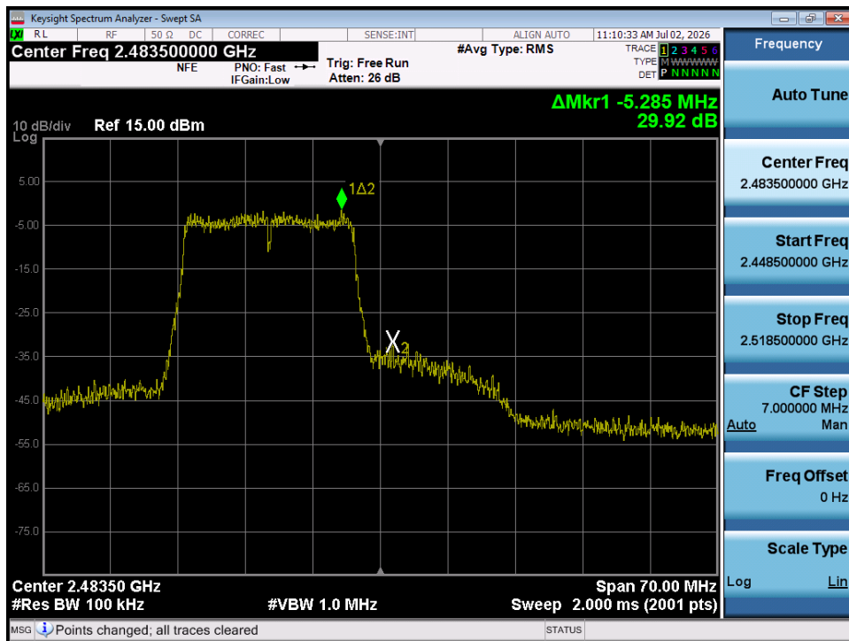
Plot 7-40. Band Edge Plot (802.11n (2.4GHz) – Ch. 13)
