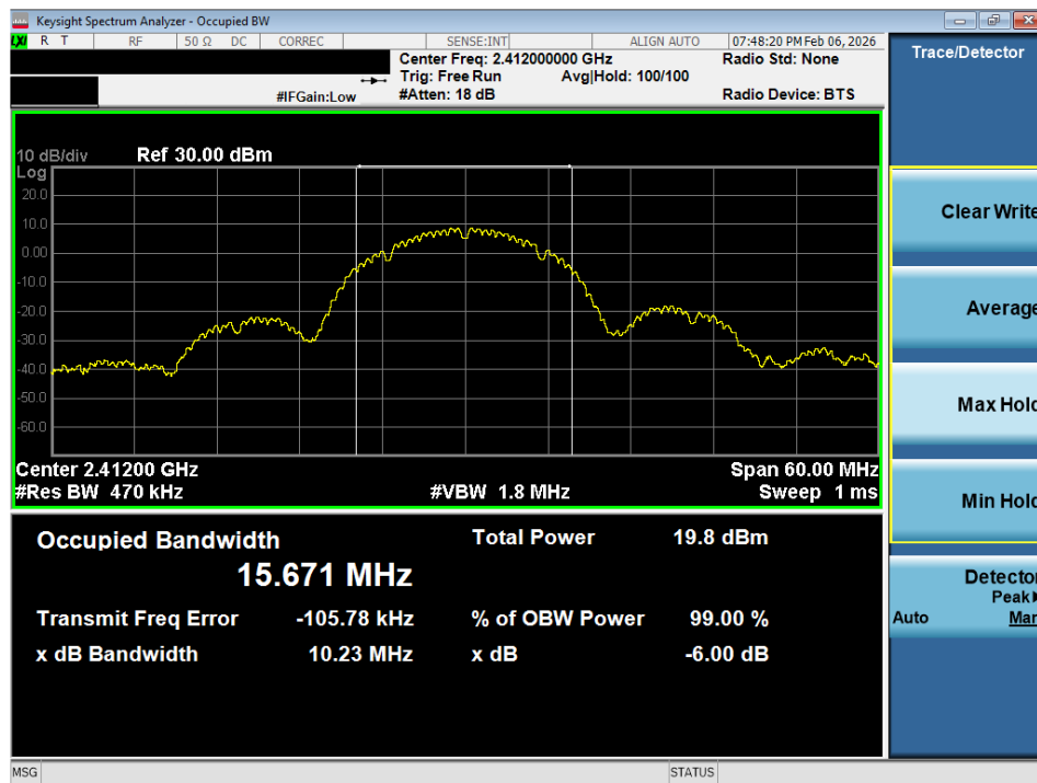
Plot 7-10 99% OBW Plot (20MHz BW 802.11b - Ch.1)
