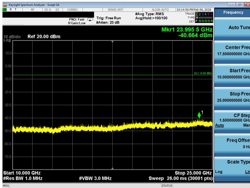
Plot 7-54. Conducted Spurious Plot (802.11n – Ch. 1)
