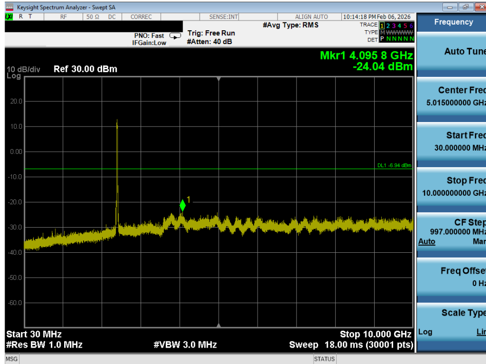
Plot 7-53. Conducted Spurious Plot (802.11n – Ch. 1)
