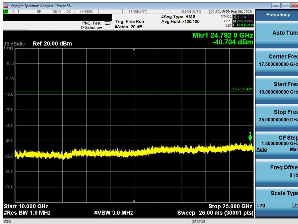
Plot 7-46. Conducted Spurious Plot (802.11b – Ch. 11)
