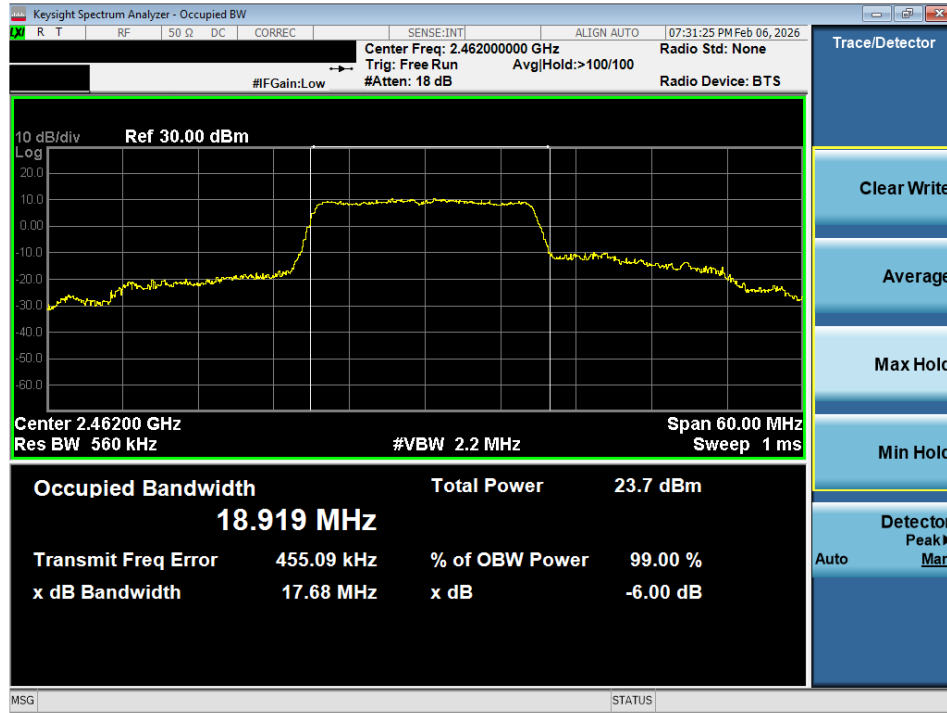
Plot 7-17 99% OBW Plot (20MHz BW 802.11n - Ch.11)
