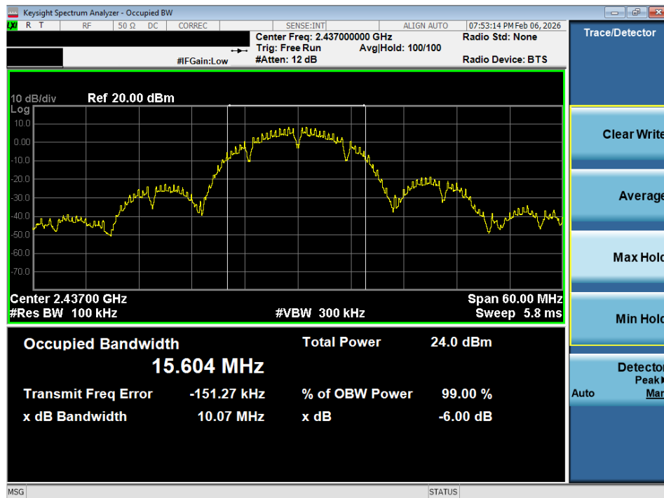
Plot 7-2 6dB BW (20MHz BW 802.11b - Ch.6)
