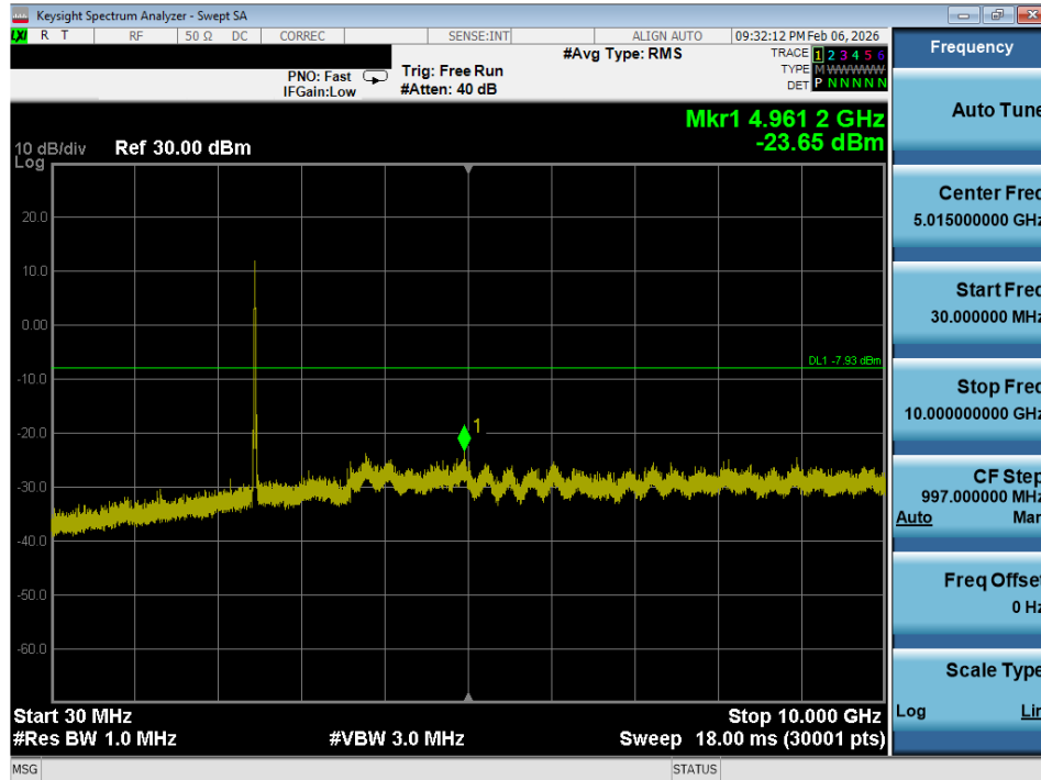
Plot 7-45. Conducted Spurious Plot (802.11b – Ch. 11)
