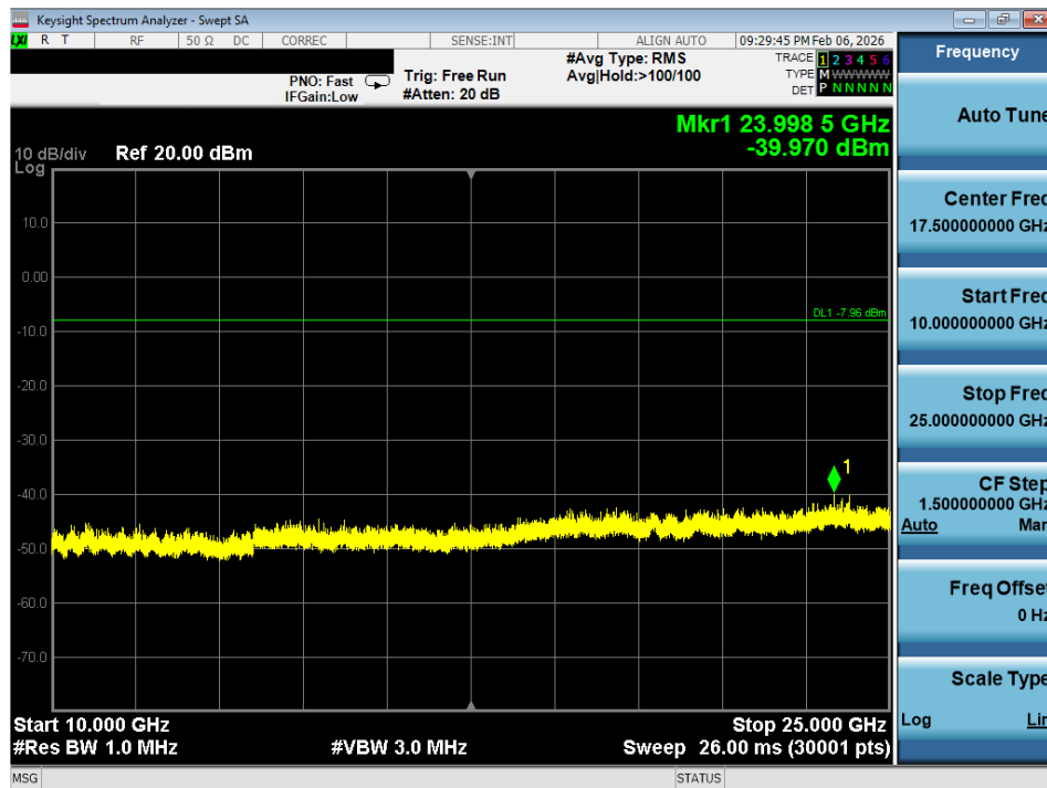
Plot 7-44. Conducted Spurious Plot (802.11b – Ch. 6)
