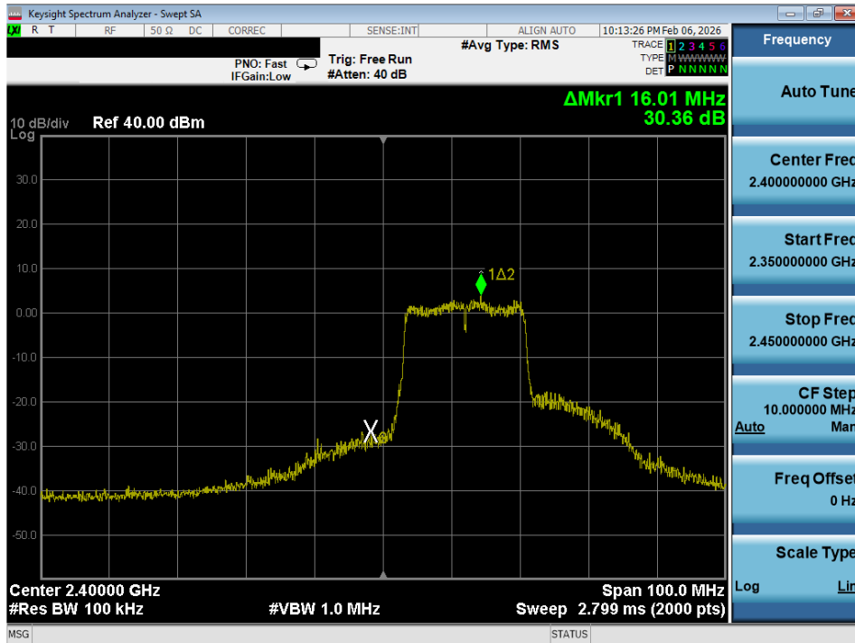
Plot 7-36. Band Edge Plot (802.11n (2.4GHz) – Ch. 1)
