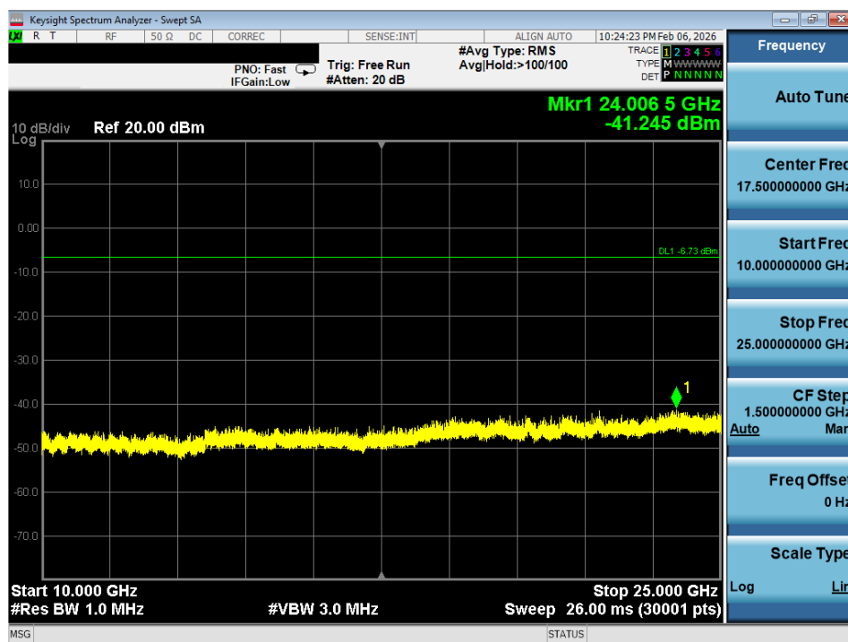
Plot 7-56. Conducted Spurious Plot (802.11n – Ch. 6)
