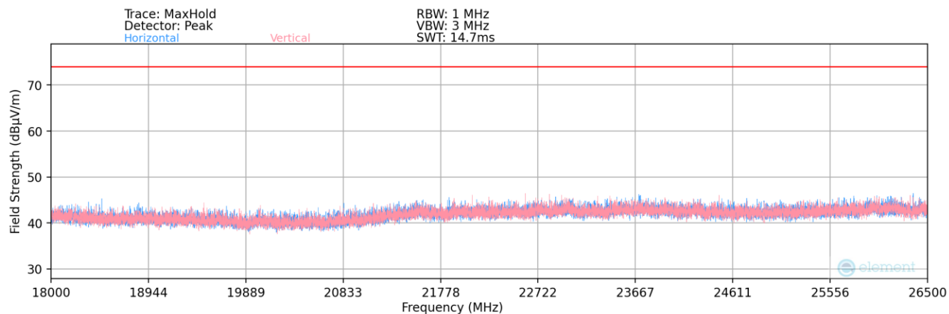
Plot 7-63. Radiated Spurious Plot above 18GHz
