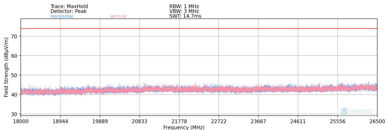
Plot 7-45. Radiated Spurious Plot above 18GHz – Ant 1
