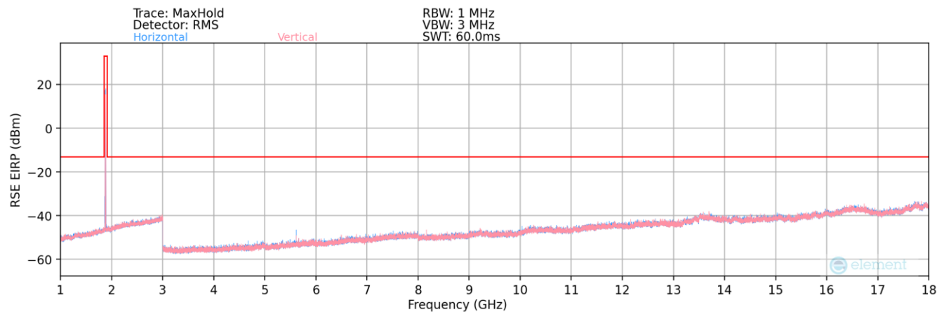
Plot 7-2. Radiated Spurious Plot (LTE CAT-M1 Band 2)
