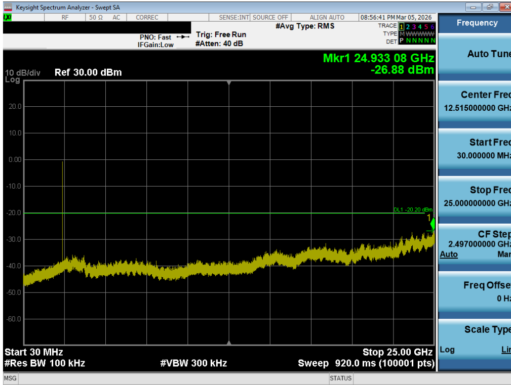
Plot 7-31. Conducted Spurious Plot (Bluetooth (LE), 1Mbps – Ch. 37)
