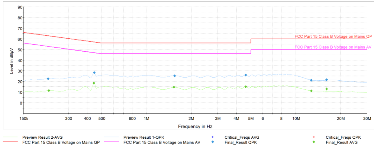
Plot 7-49. AC Line Conducted Plot with Bluetooth LE (N, 1Mbps– Ch.17, with AC/DC Adapter)
