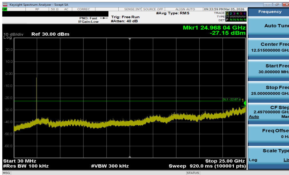
Plot 7-36. Conducted Spurious Plot (Bluetooth (LE), 2Mbps – Ch. 36)
