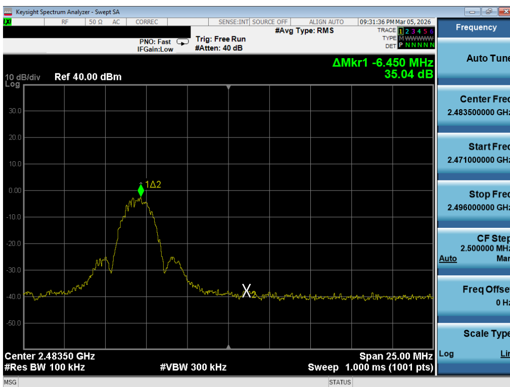
Plot 7-30. Band Edge Plot (Bluetooth (LE), 2Mbps – Ch. 36)
