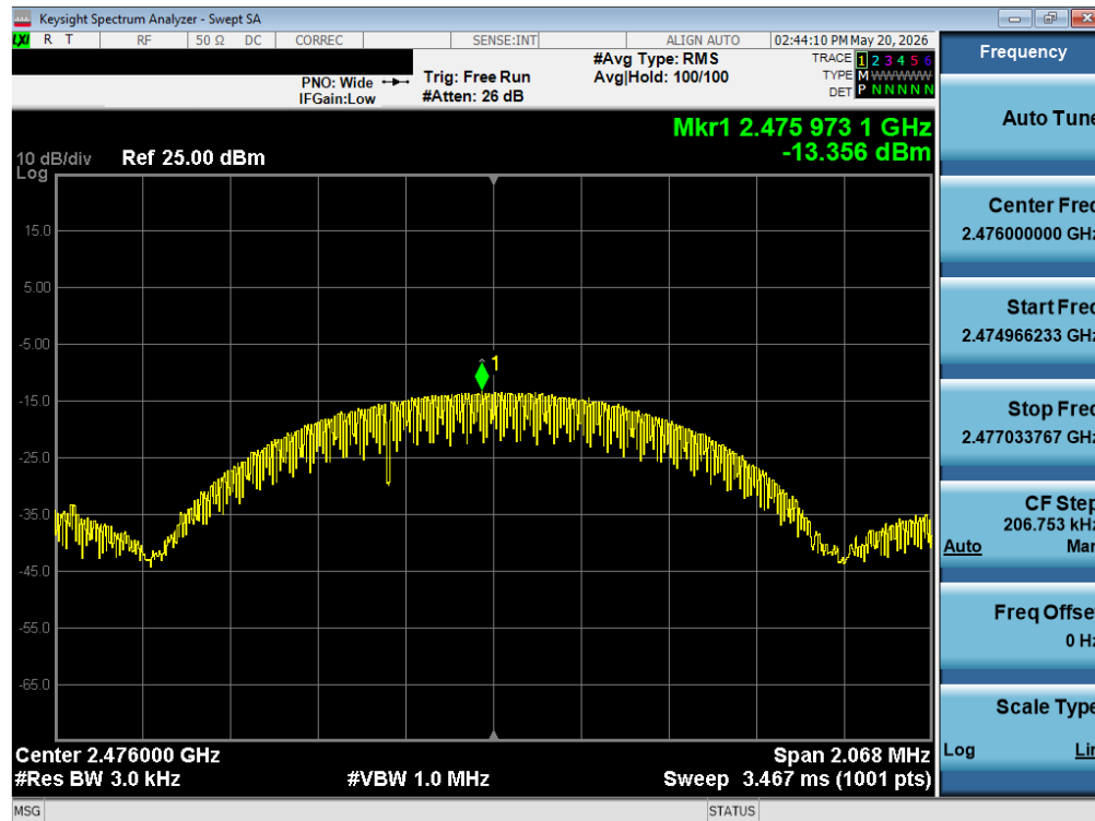
Plot 7-16. Power Spectral Density Plot (Bluetooth (LE), 1Mbps – Ch. 35)
