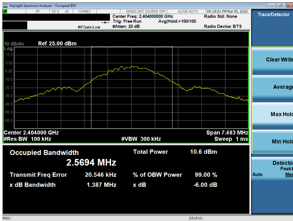
Plot 7-10. 6dB BW Plot (Bluetooth (LE), 2Mbps – Ch. 0)
