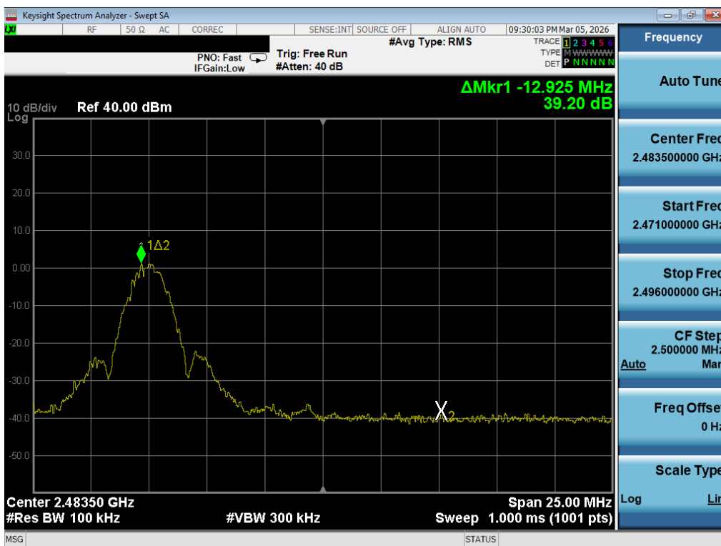
Plot 7-29. Band Edge Plot (Bluetooth (LE), 2Mbps – Ch. 35)
