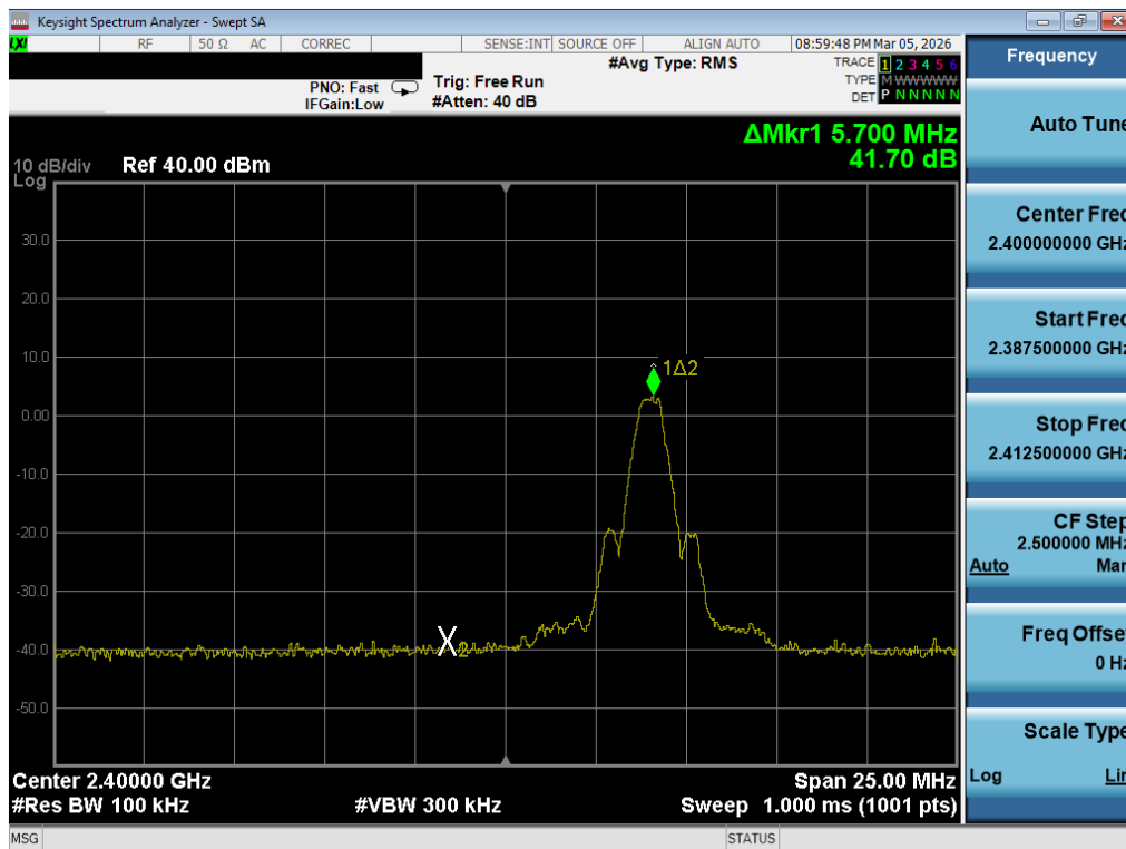
Plot 7-24. Band Edge Plot (Bluetooth (LE), 1Mbps – Ch.0)
