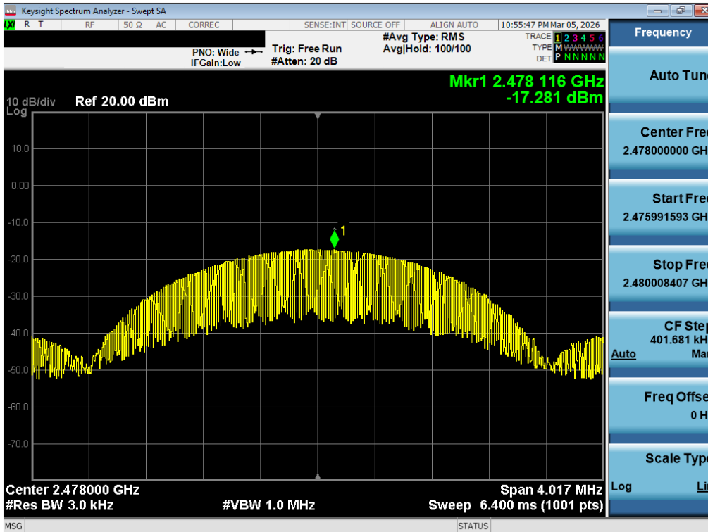
Plot 7-22. Power Spectral Density Plot (Bluetooth (LE), 2Mbps – Ch. 36)
