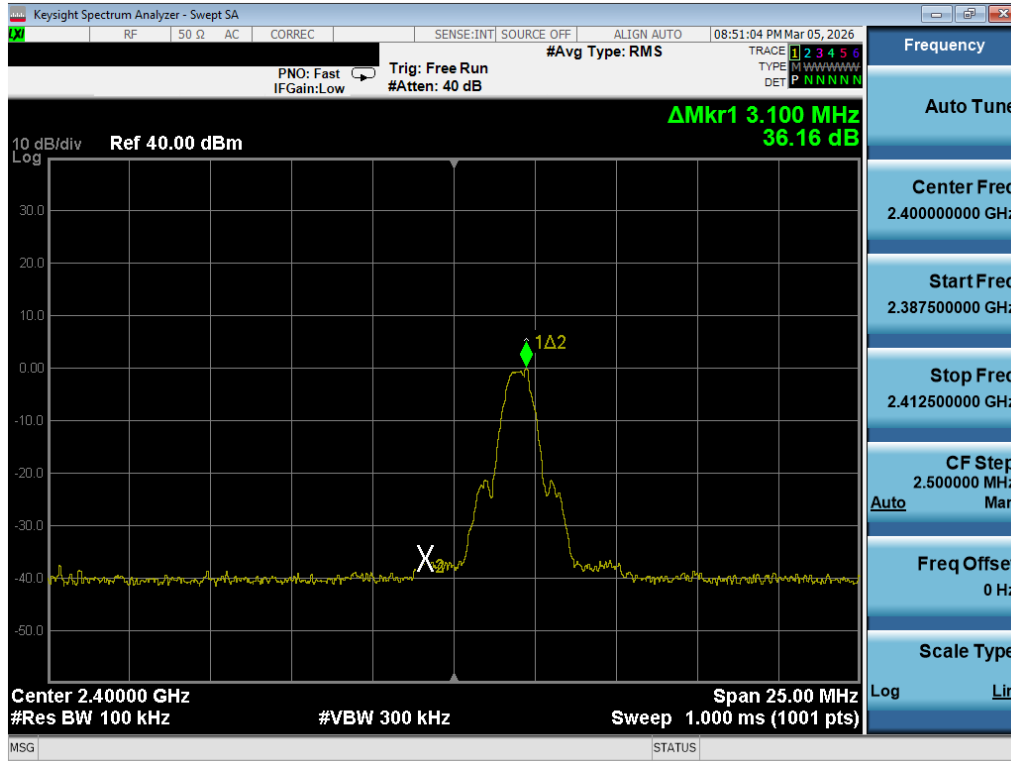
Plot 7-23. Band Edge Plot (Bluetooth (LE), 1Mbps – Ch.37)
