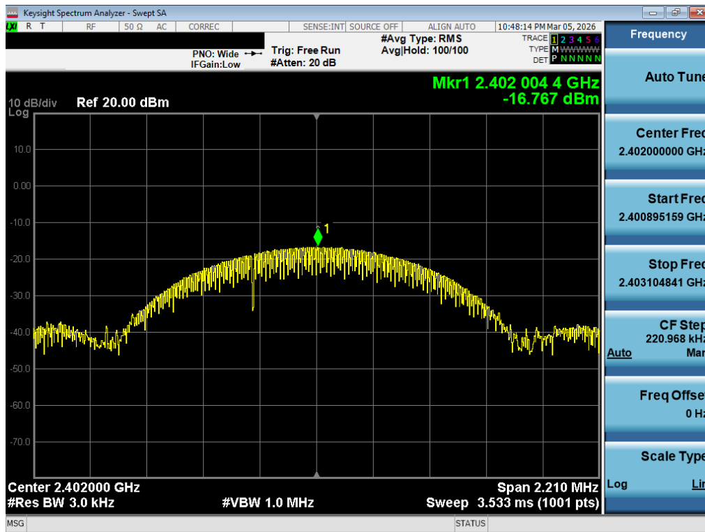
Plot 7-13. Power Spectral Density Plot (Bluetooth (LE), 1Mbps – Ch. 37)
