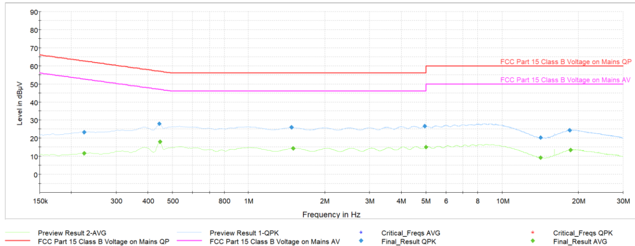
Plot 7-48. AC Line Conducted Plot with Bluetooth LE (L1, 1Mbps- Ch.17 with AC/DC Adapter)
