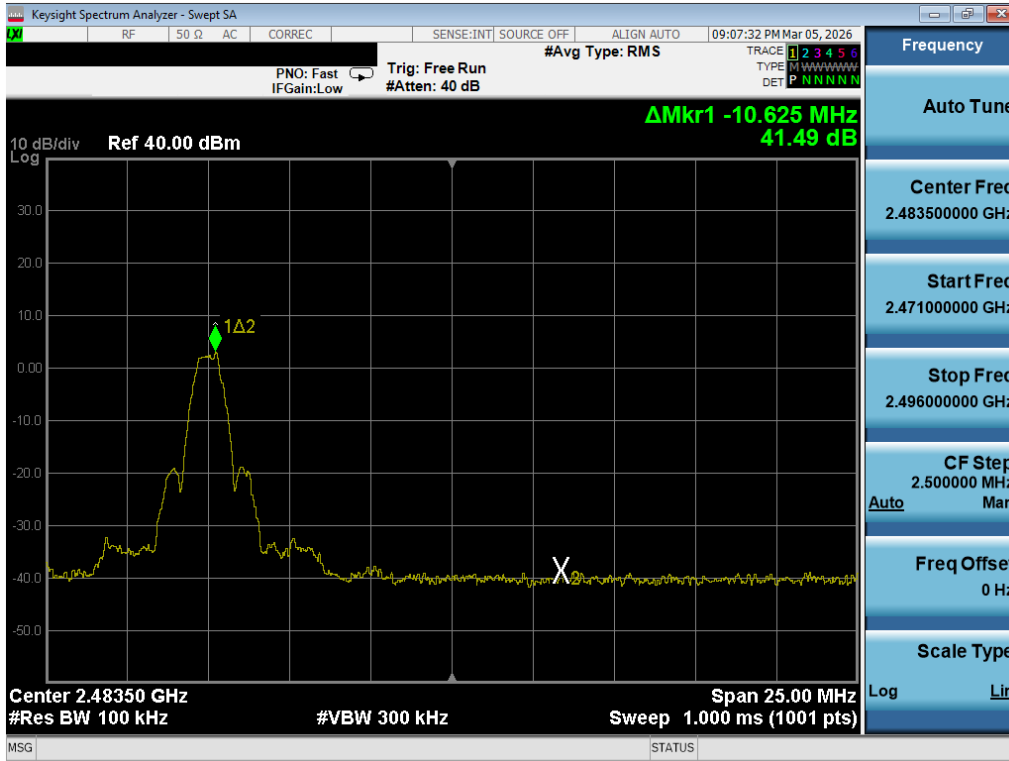
Plot 7-25. Band Edge Plot (Bluetooth (LE), 1Mbps – Ch.35)
