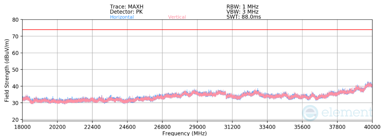
Plot 7-39. Radiated Spurious Emissions Above 18GHz (1Mbps – Ch. 17)
