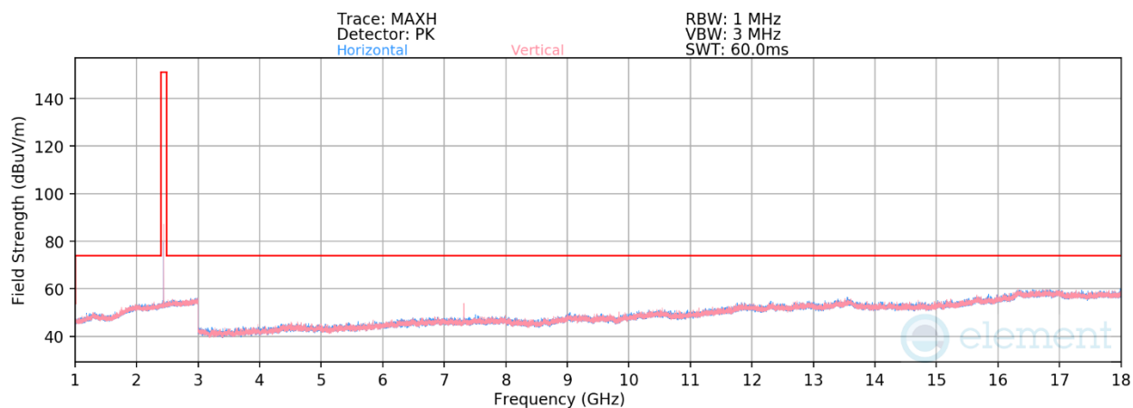
Plot 7-38. Radiated Spurious Emissions 1-18GHz (1Mbps – Ch. 17)
