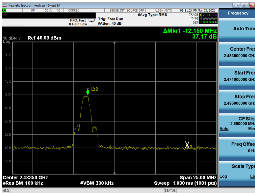
Plot 7-27. Band Edge Plot (Bluetooth (LE), 1Mbps – Ch. 39)
