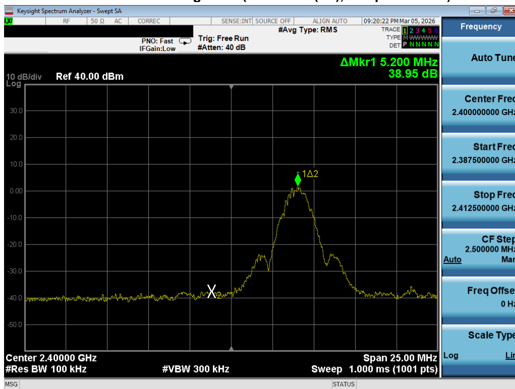
Plot 7-28. Band Edge Plot (Bluetooth (LE), 2Mbps – Ch. 0)
