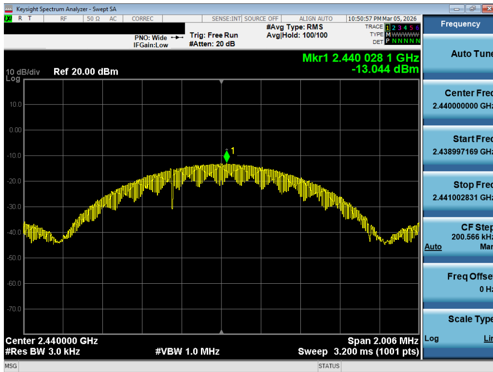
Plot 7-15. Power Spectral Density Plot (Bluetooth (LE), 1Mbps – Ch. 17)
