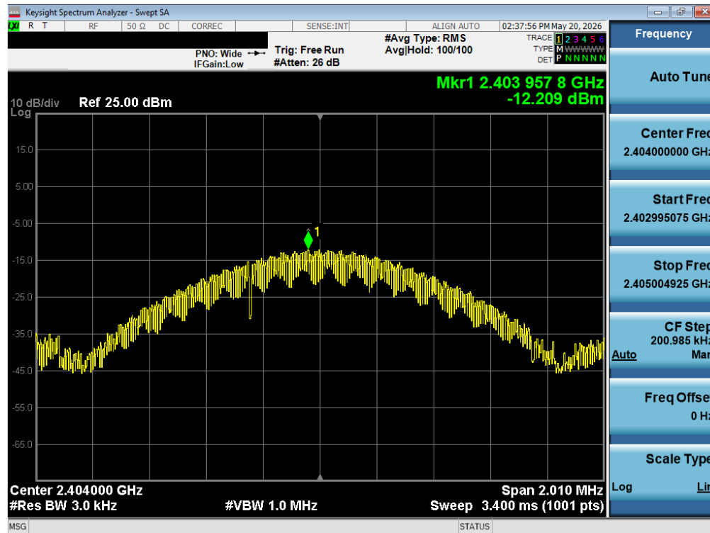
Plot 7-14. Power Spectral Density Plot (Bluetooth (LE), 1Mbps – Ch. 0)
