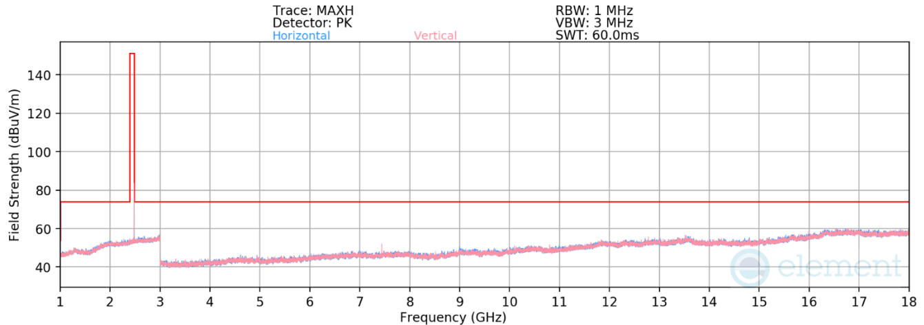
Plot 7-40. Radiated Spurious Emissions 1-18GHz (1Mbps – Ch. 39)
