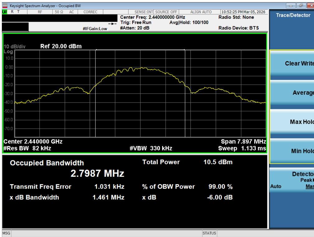
Plot 7-5. 99% OBW Plot (Bluetooth (LE), 2Mbps – Ch. 17)
