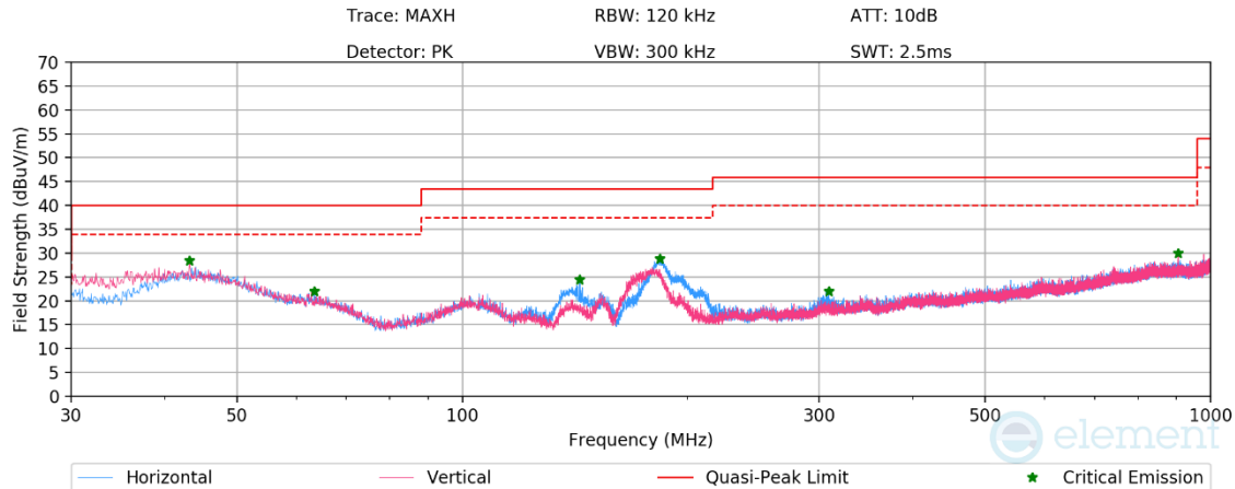
Plot 7-47. Radiated Spurious Emissions Below 1GHz (1Mbps – Ch.17, Pol. H & V, with AC/DC Adapter)
