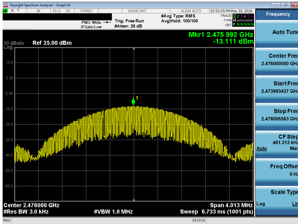
Plot 7-21. Power Spectral Density Plot (Bluetooth (LE), 2Mbps – Ch. 35)
