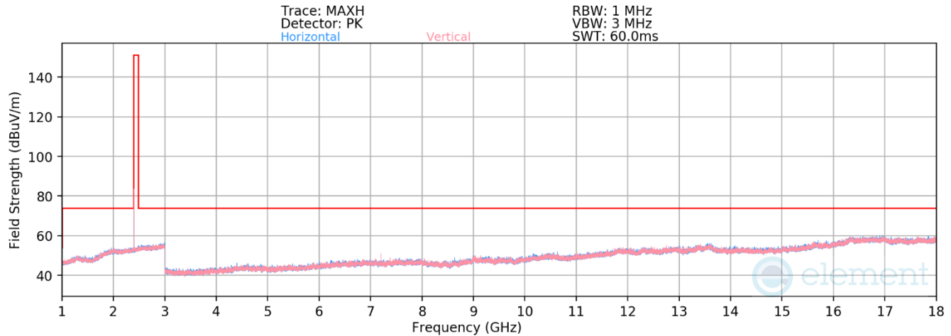
Plot 7-37. Radiated Spurious Emissions 1-18GHz (1Mbps – Ch. 37)
