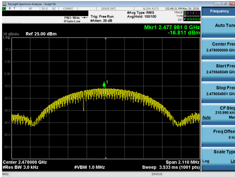
Plot 7-17. Power Spectral Density Plot (Bluetooth (LE), 1Mbps – Ch. 36)
