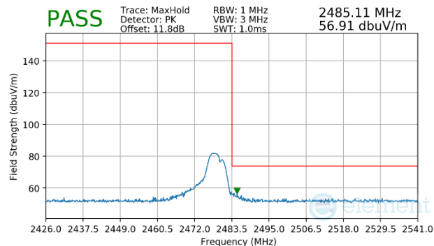
Plot 7-46. Radiated Restricted Upper Band Edge Measurement (Peak)
