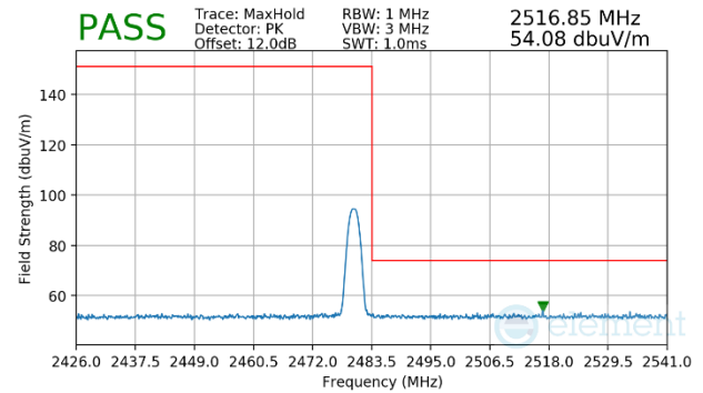
Plot 7-40. Radiated Restricted Upper Band Edge Measurement (Peak)
