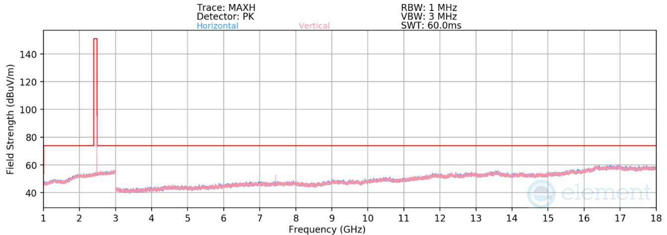
Plot 7-34. Radiated Spurious Emissions above 1GHz (BT GFSK – Ch. 78)
