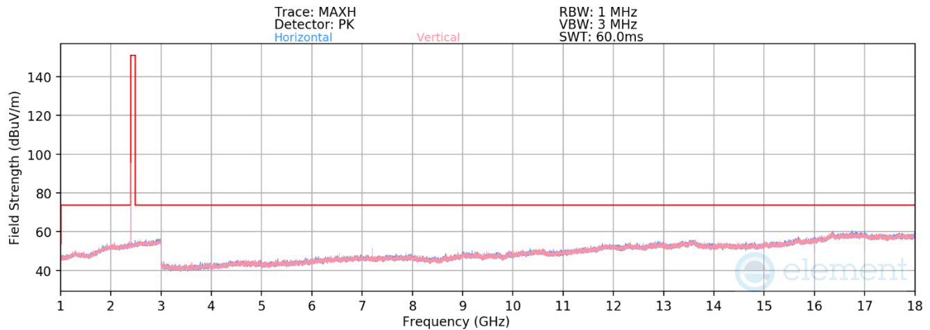
Plot 7-31. Radiated Spurious Emissions above 1GHz (BT GFSK – Ch. 0)
