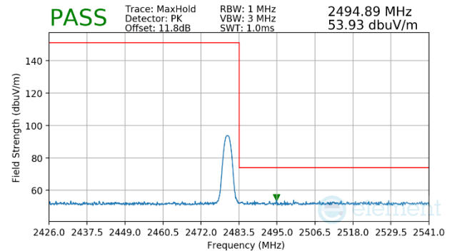
Plot 7-42. Radiated Restricted Upper Band Edge Measurement (Peak)
