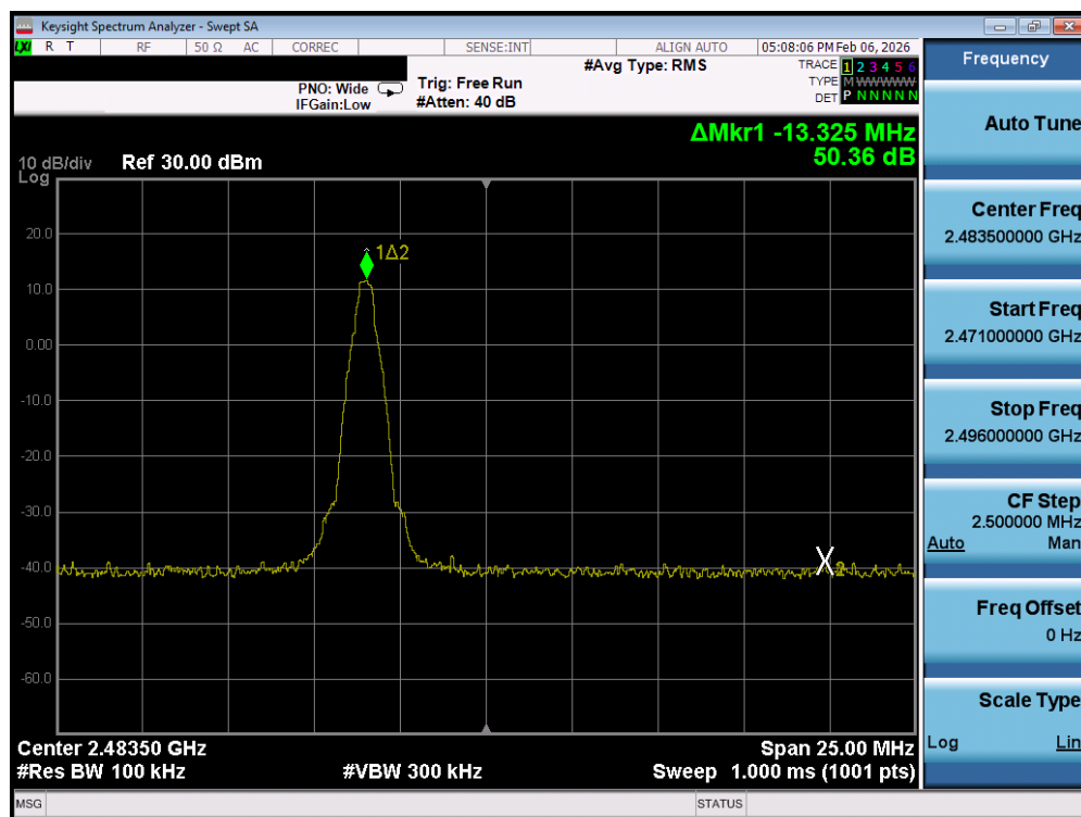
Plot 7-5. Band Edge Plot (Bluetooth with Hopping Disabled, GFSK – Ch. 78)
