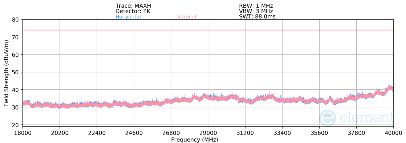
Plot 7-33. Radiated Spurious Emissions above 18GHz (BT GFSK – Ch. 39)
