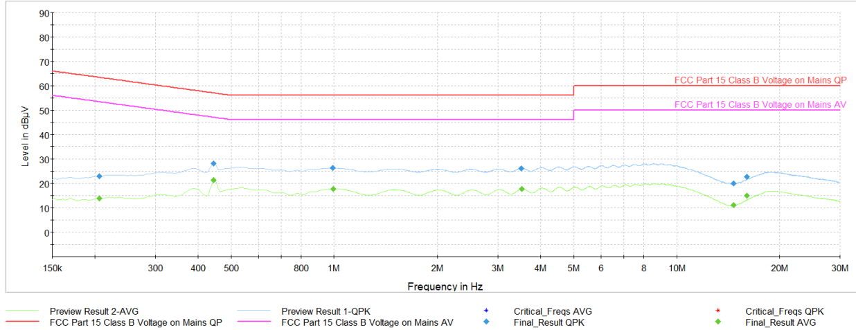
Plot 7-44. AC Line-Conducted Test Plot (L1, GFSK – Ch.39, with AC/DC Adapter)
