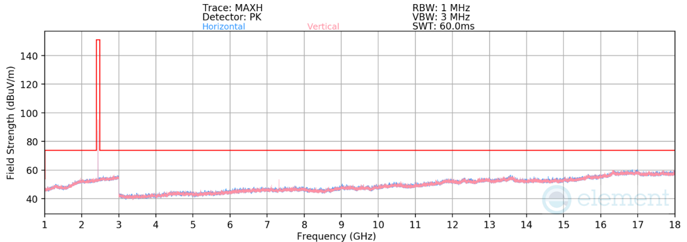
Plot 7-32. Radiated Spurious Emissions above 1GHz (BT GFSK – Ch. 39)
