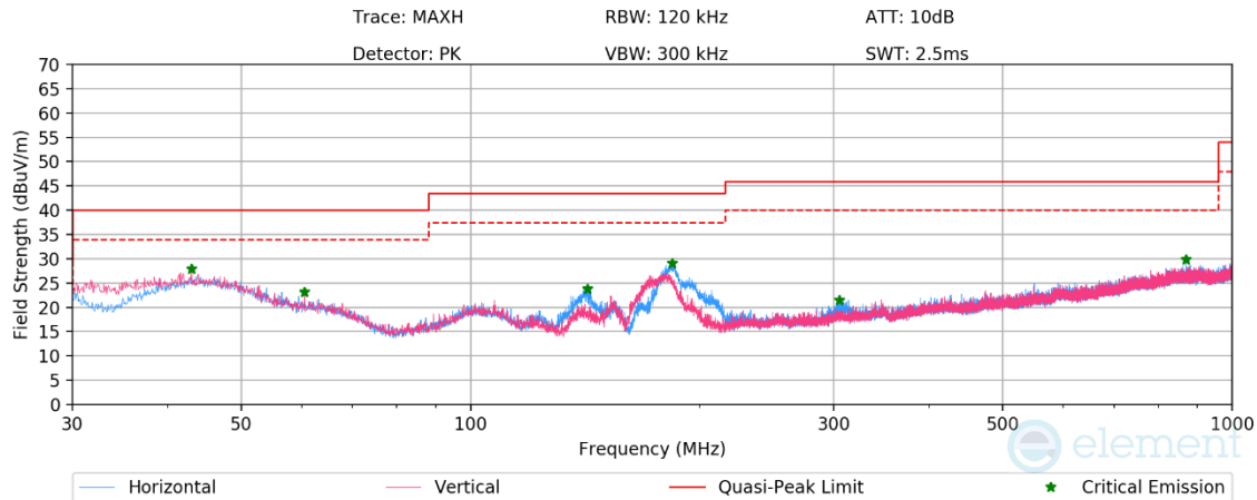
Plot 7-43. Radiated Spurious Emissions Below 1GHz (GFSK – Ch.39, with AC/DC Adapter)
