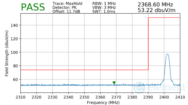
Plot 7-36. Radiated Restricted Lower Band Edge Measurement (Peak)
