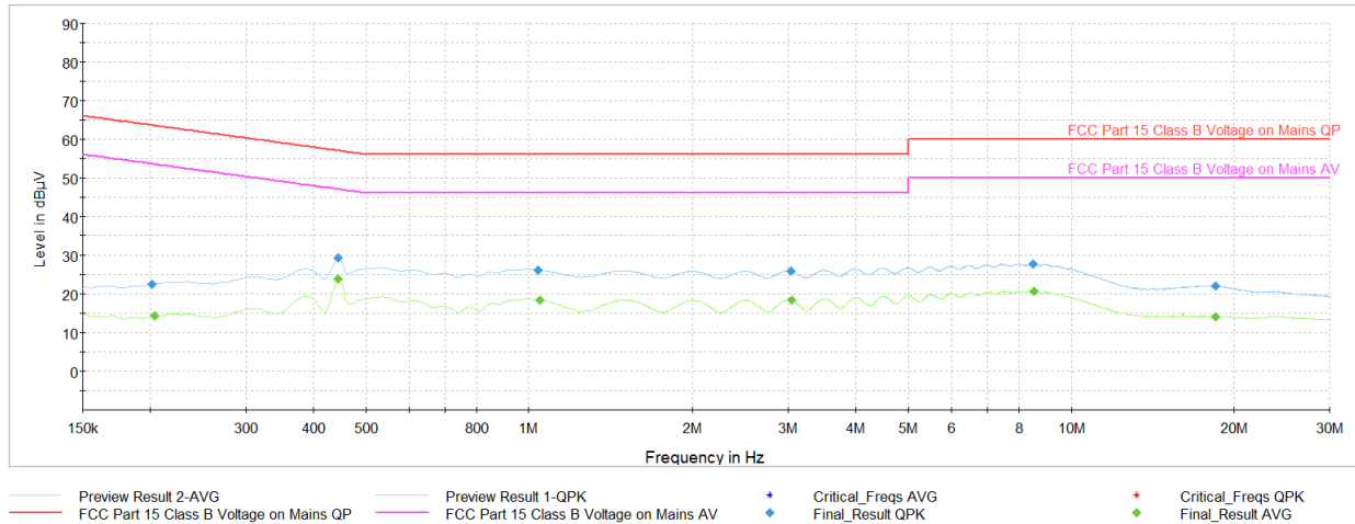
Plot 7-45. AC Line-Conducted Test Plot (N, GFSK – Ch.39, with AC/DC Adapter)
