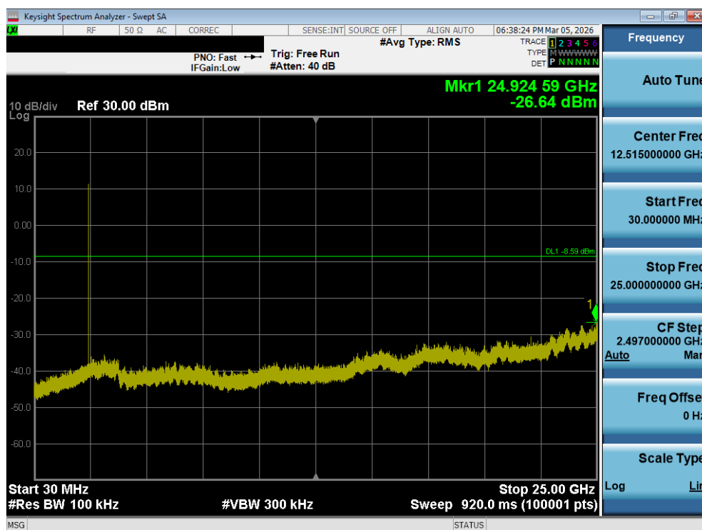
Plot 7-29. Conducted Spurious Plot (Bluetooth, GFSK - Ch. 39)
