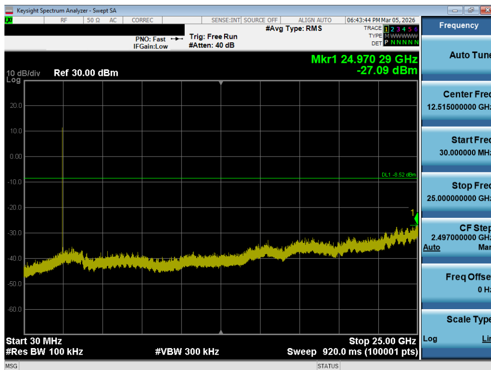
Plot 7-30. Conducted Spurious Plot (Bluetooth, GFSK – Ch. 78)
