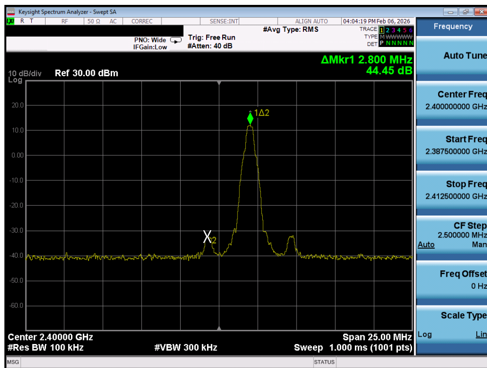
Plot 7-4. Band Edge Plot (Bluetooth with Hopping Disabled, GFSK – Ch. 0)
