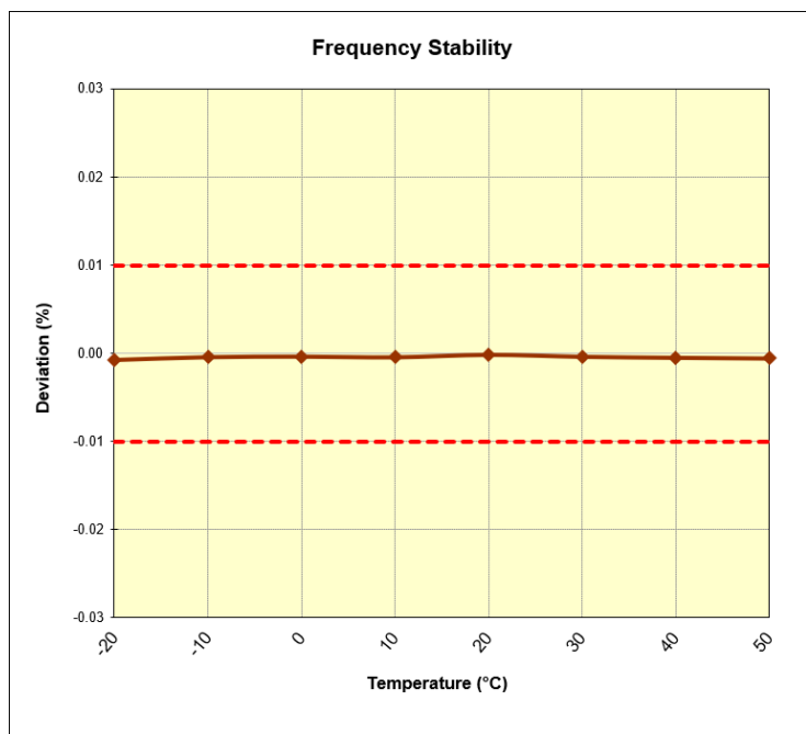
Figure 7-3. Frequency Stability Plot
