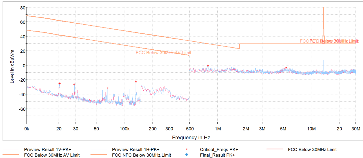
Plot 7-3. Radiated Spurious Emissions 9kHz – 30MHz (with AC/DC Adapter)
