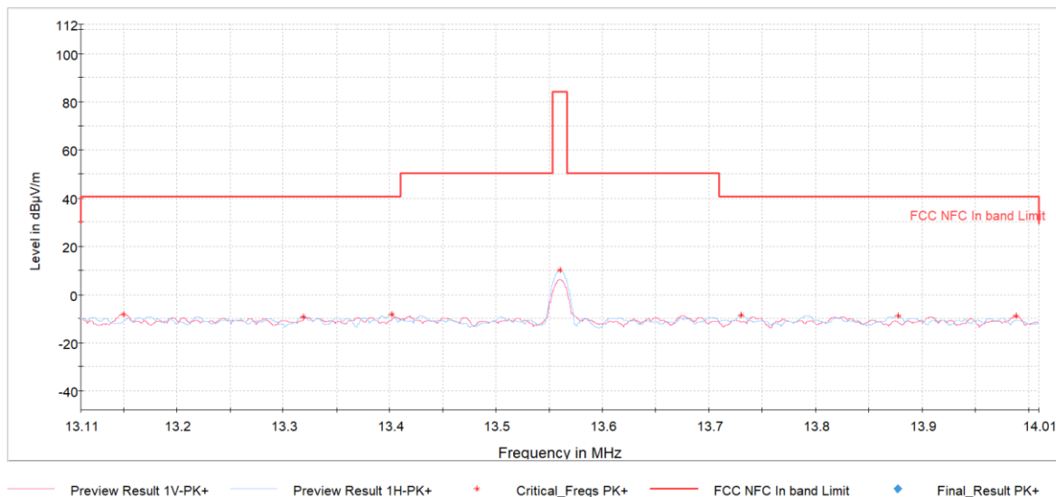
Plot 7-2. In Band Radiated Spurious Emissions (AC/DC Adapter)
