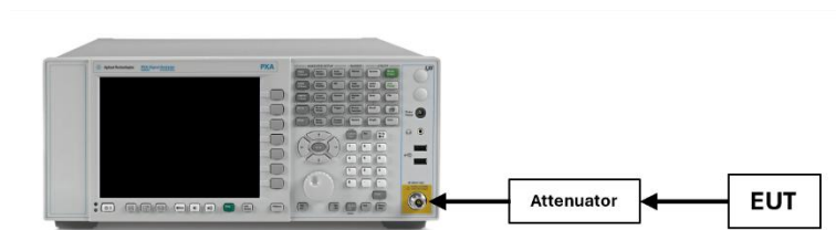
Figure 7-2. Test Instrument & Measurement Setup
