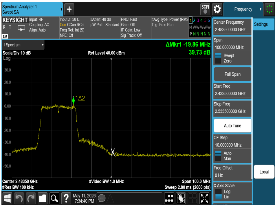
Plot 7-38. Band Edge Plot (802.11n (2.4GHz) – Ch. 10)
