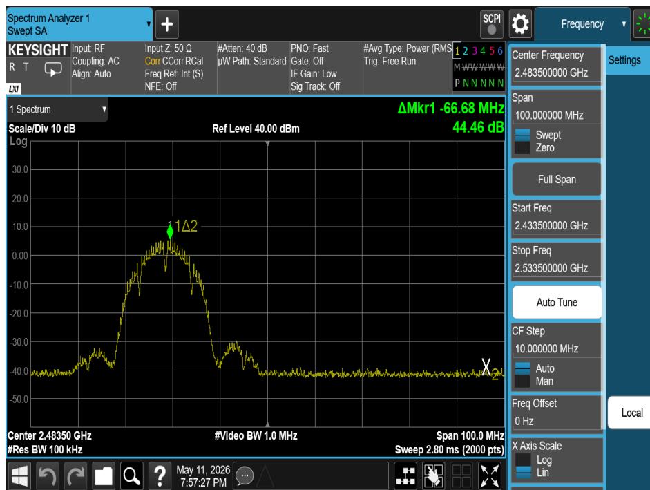
Plot 7-15. Band Edge Plot (802.11b – Ch. 11)
