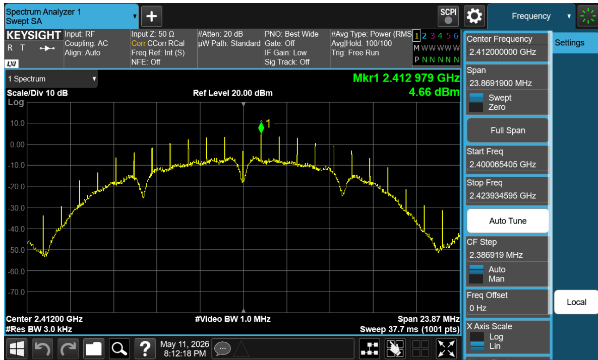
Plot 7-7 PSD (20MHz BW 802.11b - Ch.1)
