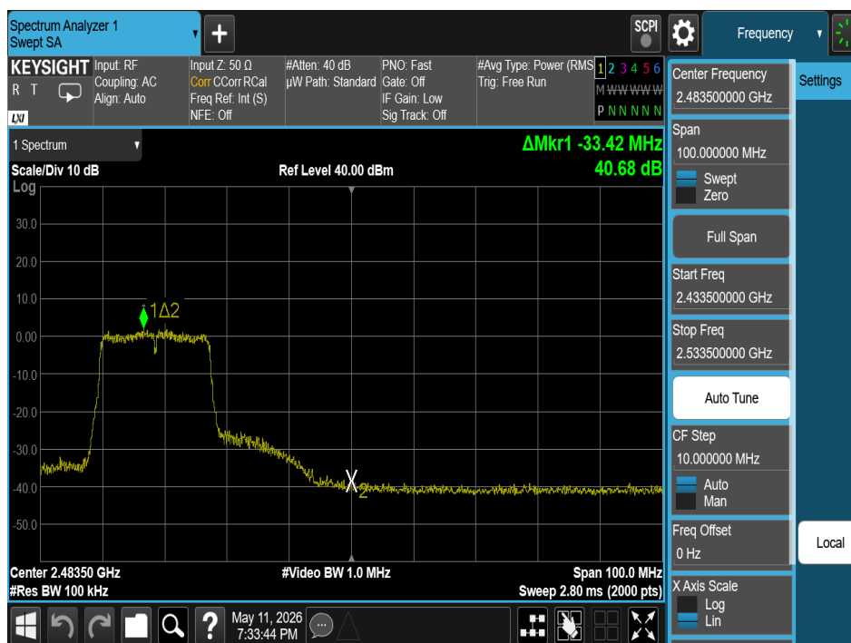
Plot 7-37. Band Edge Plot (802.11n (2.4GHz) – Ch. 9)
