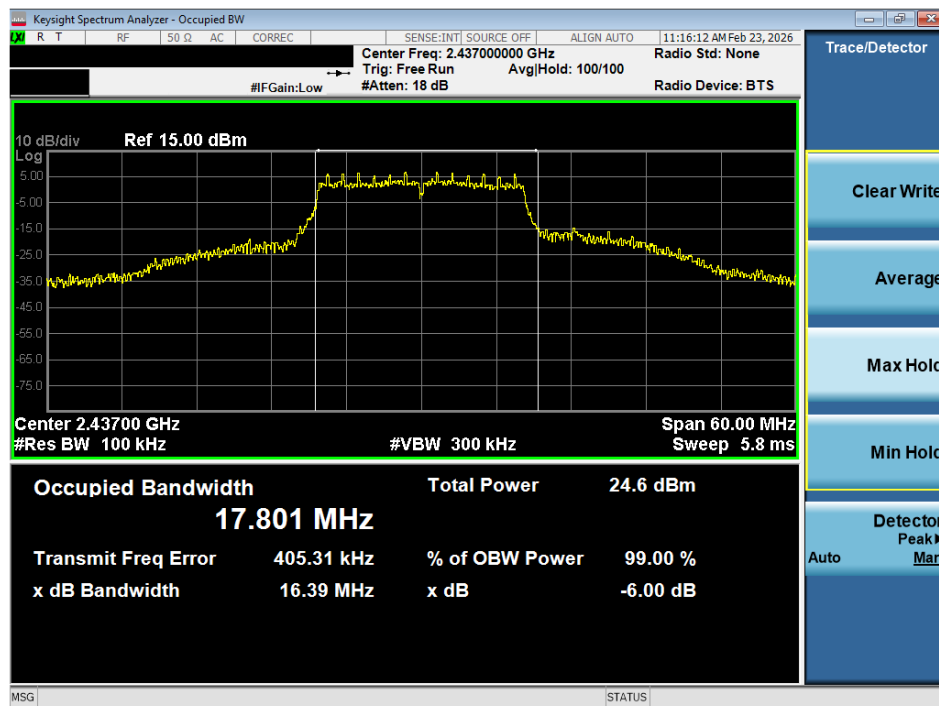
Plot 7-5 6dB BW Antenna 1 (20MHz BW 802.11g - Ch.6)
