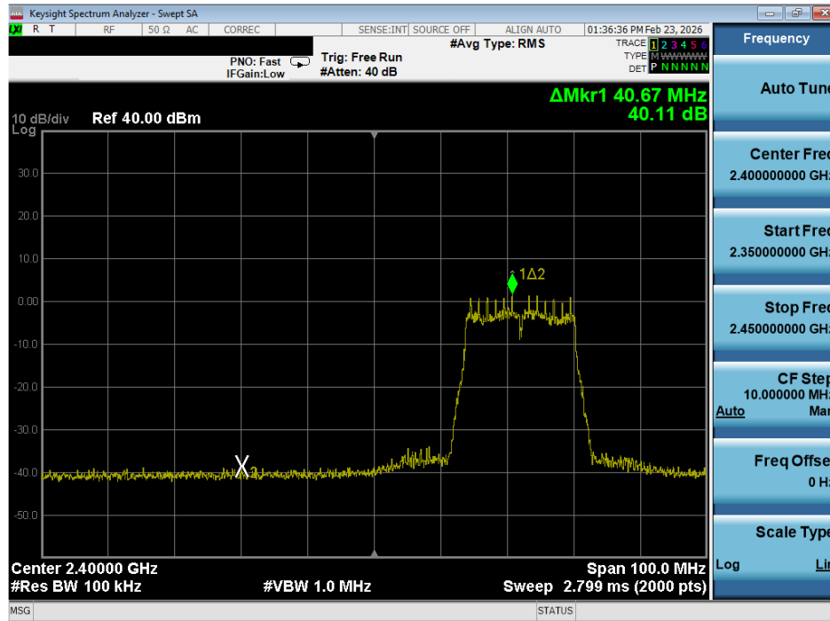
Plot 7-20. Band Edge Plot (802.11g – Ch. 3)
