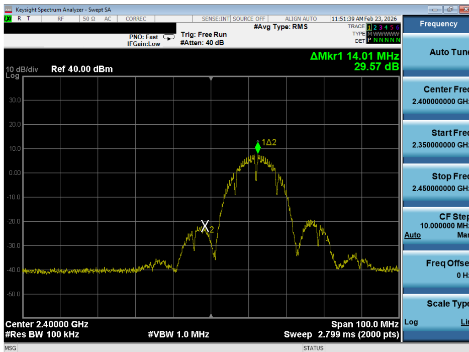
Plot 7-10. Band Edge Plot (802.11b – Ch. 1)
