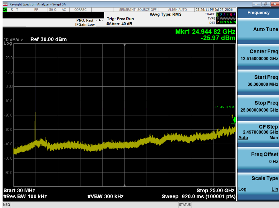
Plot 7-46. Conducted Spurious Plot (802.11g – Ch. 6)
