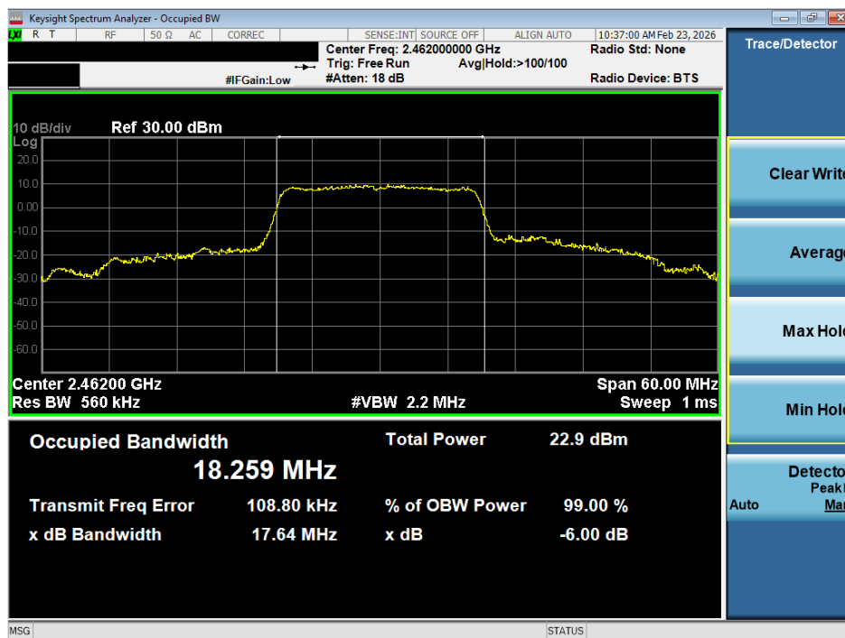
Plot 7-3 99% OBW (20MHz BW 802.11n - Ch.11)
