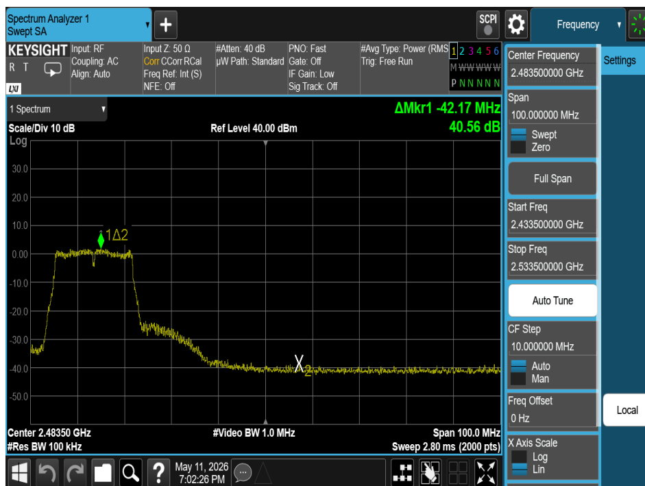
Plot 7-24. Band Edge Plot (802.11g – Ch. 8)
