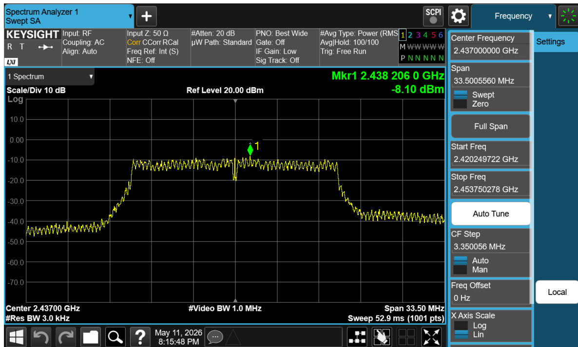
Plot 7-8 PSD (20MHz BW 802.11g - Ch.6)
