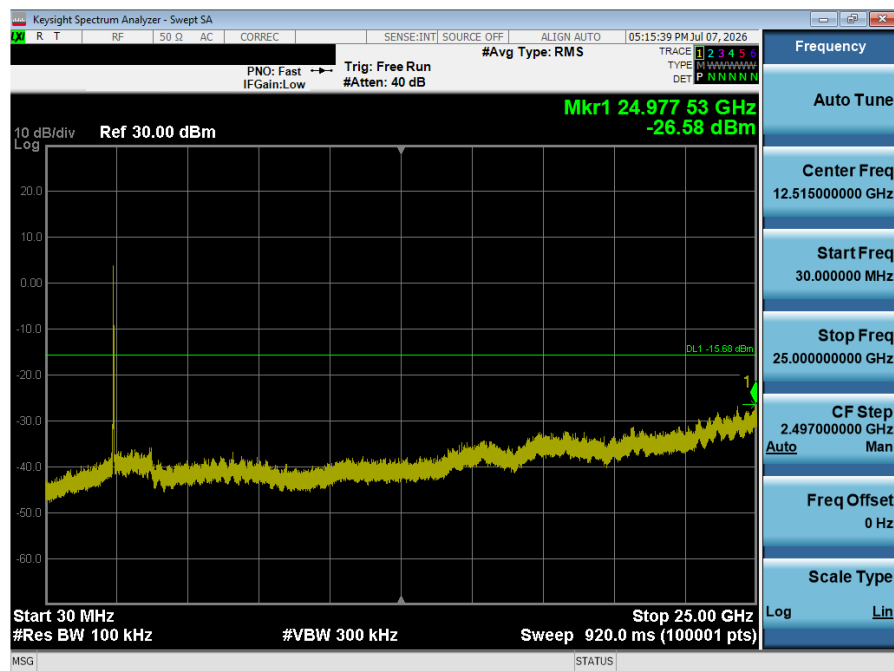
Plot 7-45. Conducted Spurious Plot (802.11g – Ch. 1)
