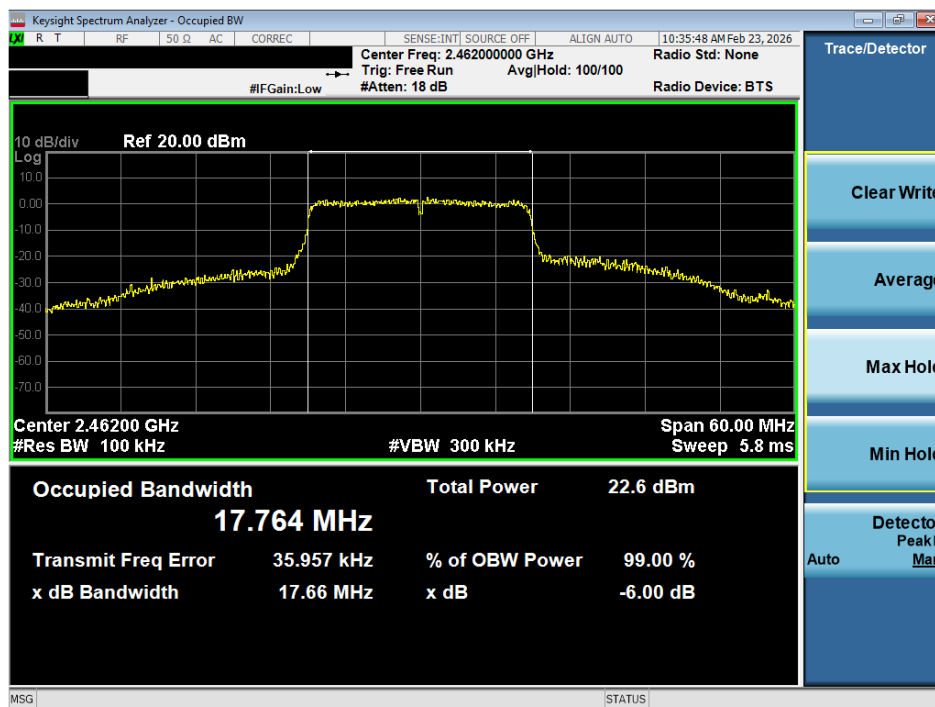
Plot 7-6 6dB BW Antenna 1 (20MHz BW 802.11n - Ch.11)
