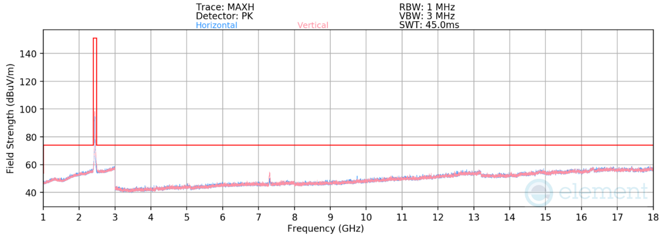
Plot 7-56. Radiated Spurious Emissions above 1GHz (802.11g – Ch. 6)
