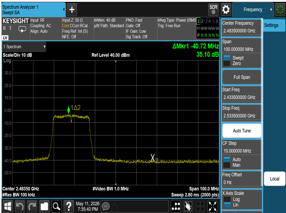
Plot 7-39. Band Edge Plot (802.11n (2.4GHz) – Ch. 11)
