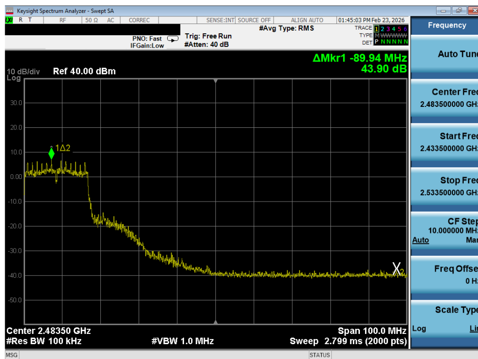
Plot 7-23. Band Edge Plot (802.11g – Ch. 7)
