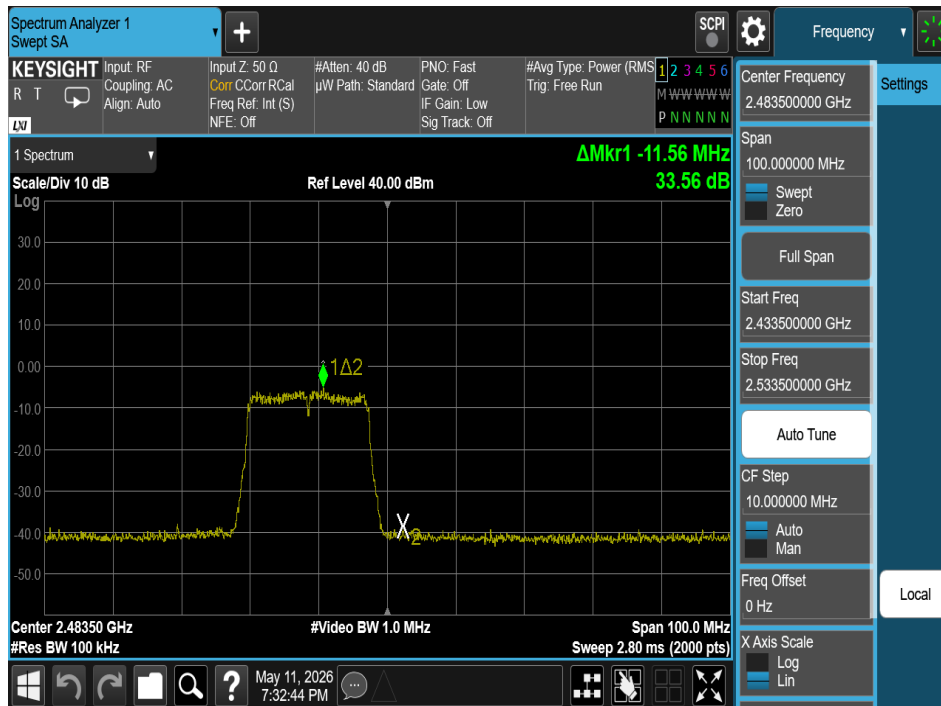
Plot 7-41. Band Edge Plot (802.11n (2.4GHz) – Ch. 13)
