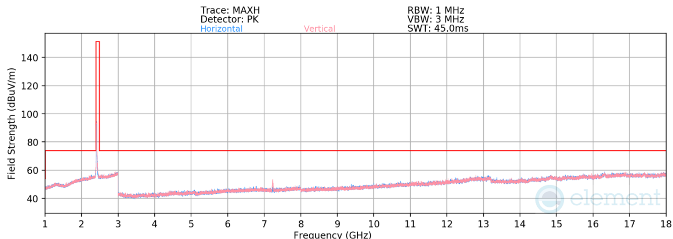
Plot 7-59. Radiated Spurious Emissions above 1GHz (802.11n – Ch. 1)
