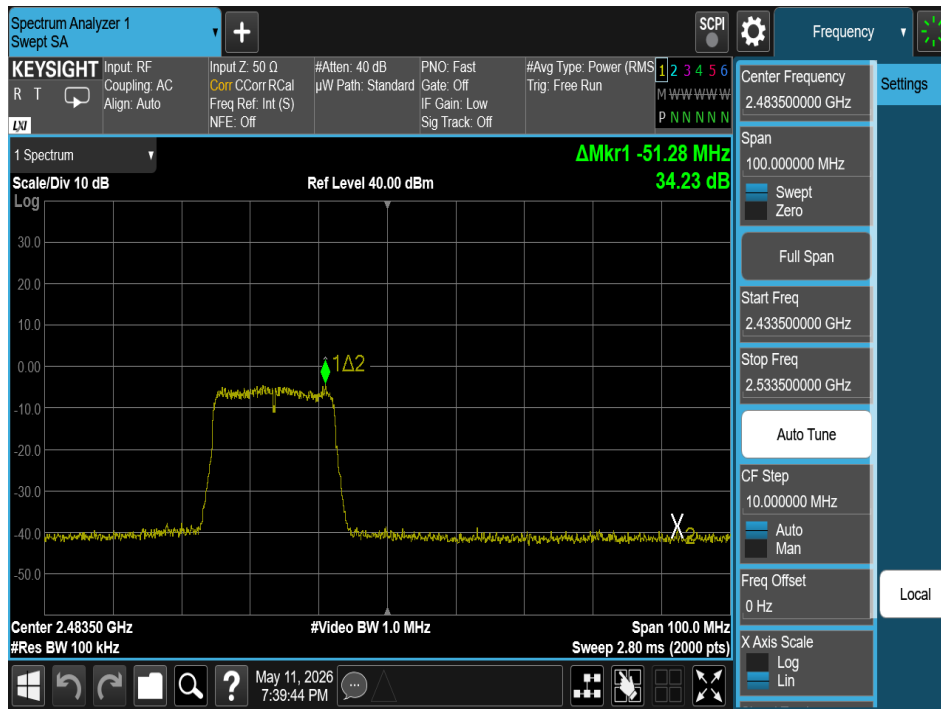
Plot 7-40. Band Edge Plot (802.11n (2.4GHz) – Ch. 12)
