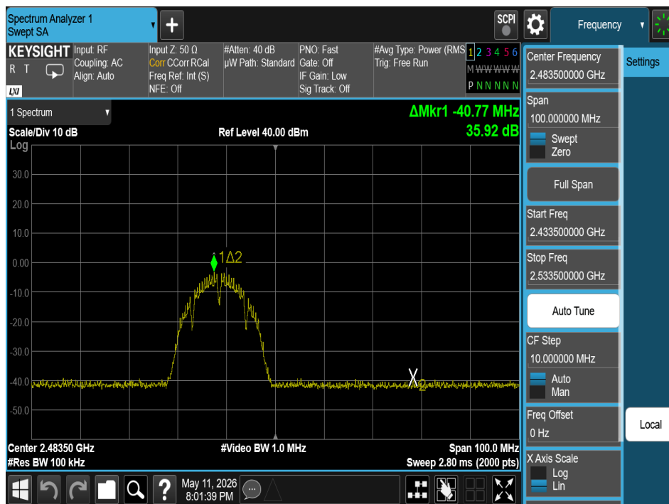
Plot 7-17. Band Edge Plot (802.11b – Ch. 13)
