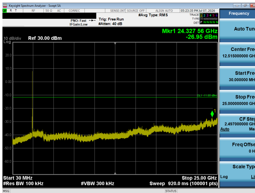
Plot 7-43. Conducted Spurious Plot (802.11b – Ch. 6)
