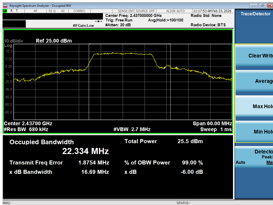
Plot 7-2 99% OBW (20MHz BW 802.11g - Ch.6)
