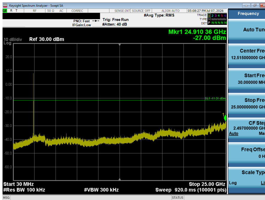
Plot 7-42. Conducted Spurious Plot (802.11b – Ch. 1)
