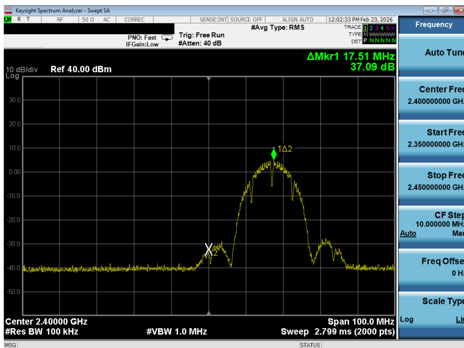
Plot 7-11. Band Edge Plot (802.11b – Ch. 2)
