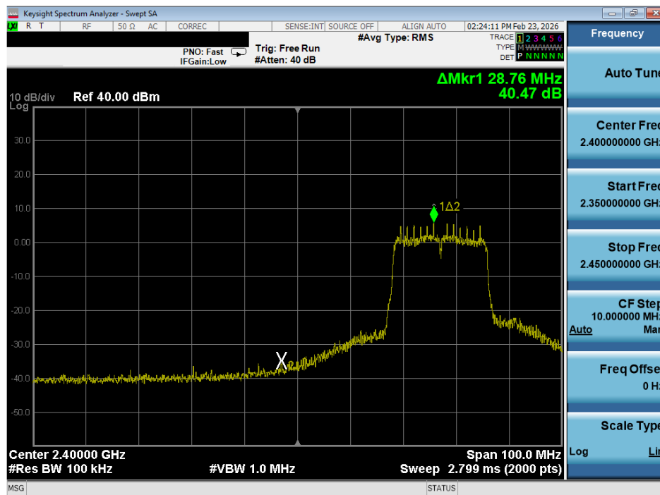
Plot 7-33. Band Edge Plot (802.11n (2.4GHz) – Ch. 4)
