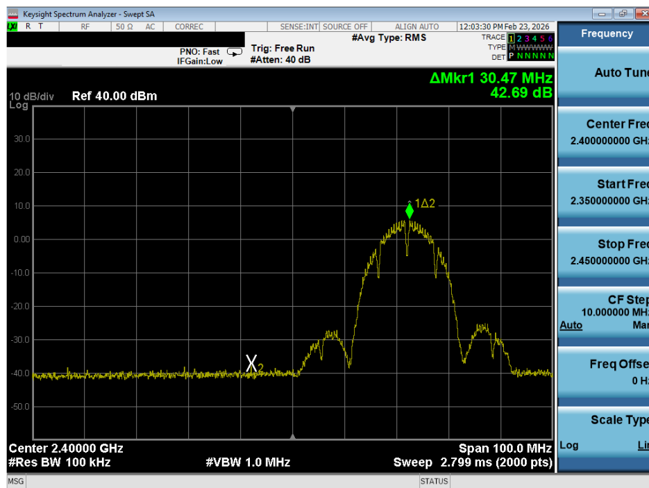
Plot 7-12. Band Edge Plot (802.11b – Ch. 3)
