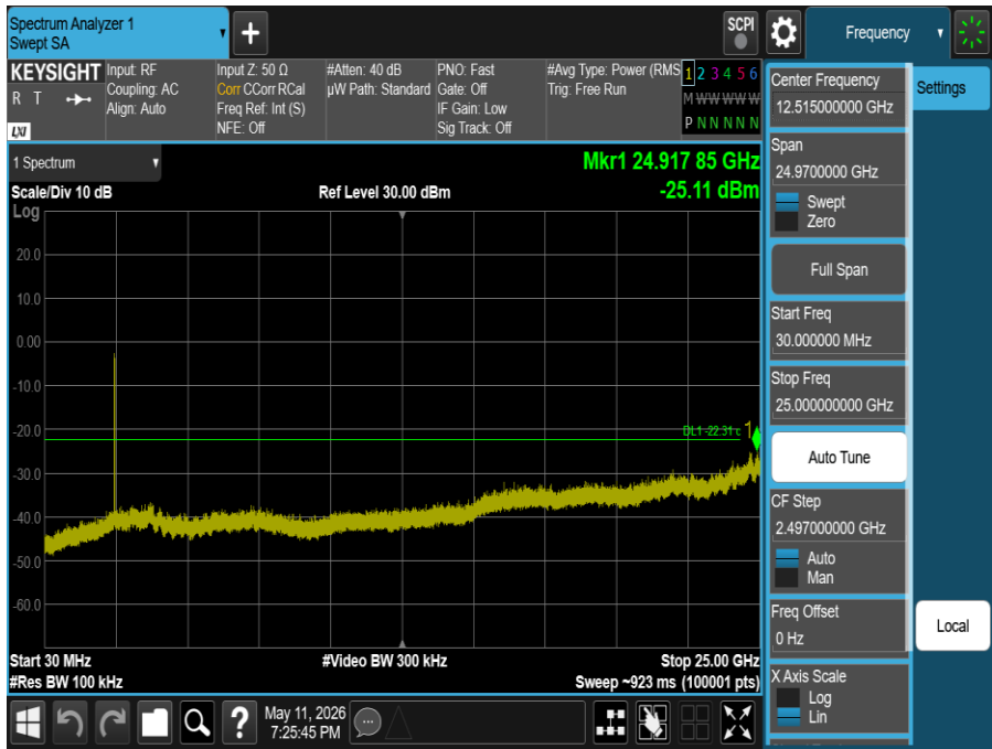
Plot 7-47. Conducted Spurious Plot (802.11g – Ch. 11)
