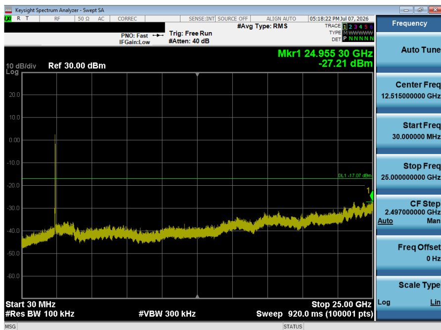
Plot 7-48. Conducted Spurious Plot (802.11n – Ch. 1)
