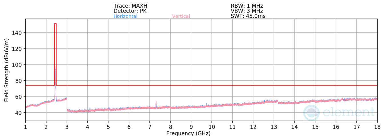
Plot 7-57. Radiated Spurious Emissions above 1GHz (802.11g – Ch. 11)
