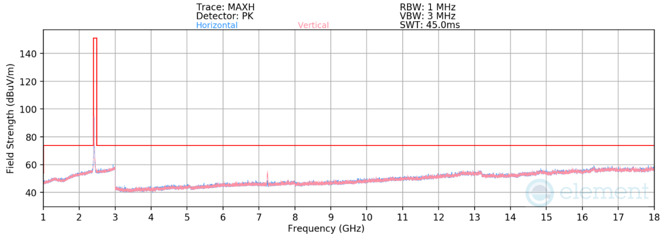
Plot 7-55. Radiated Spurious Emissions above 1GHz (802.11g – Ch. 1)
