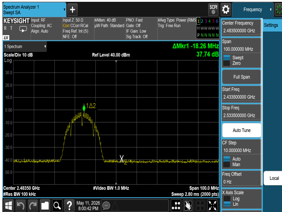
Plot 7-16. Band Edge Plot (802.11b – Ch. 12)
