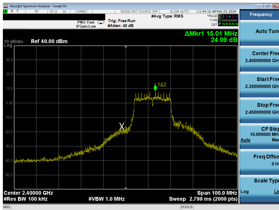
Plot 7-18. Band Edge Plot (802.11g – Ch. 1)
