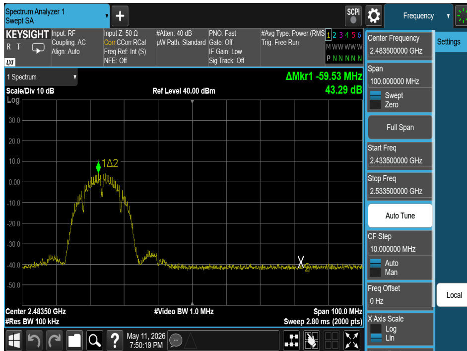
Plot 7-14. Band Edge Plot (802.11b – Ch. 10)
