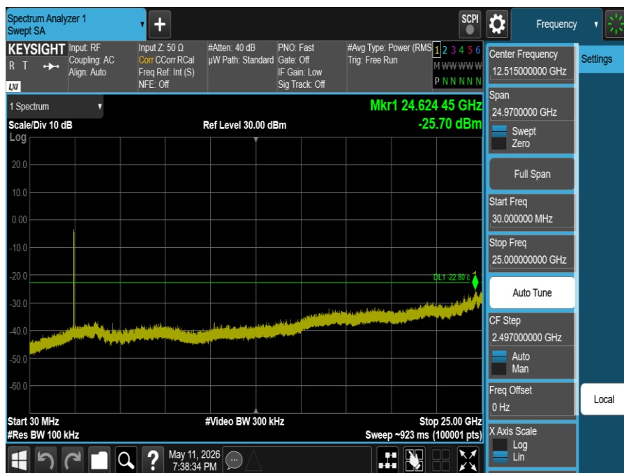
Plot 7-50. Conducted Spurious Plot (802.11n – Ch. 11)
