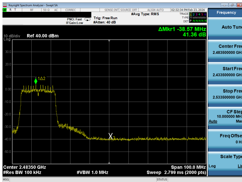
Plot 7-36. Band Edge Plot (802.11n (2.4GHz) – Ch. 8)
