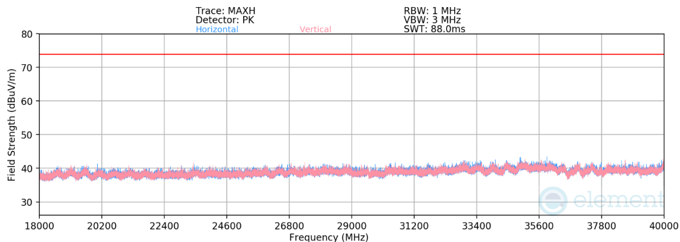
Plot 7-58. Radiated Spurious Emissions above 18GHz (802.11g – Ch.11)
