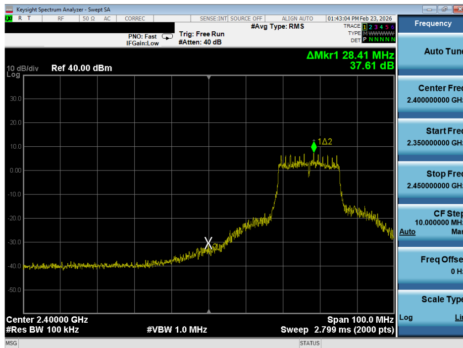
Plot 7-21. Band Edge Plot (802.11g – Ch. 4)
