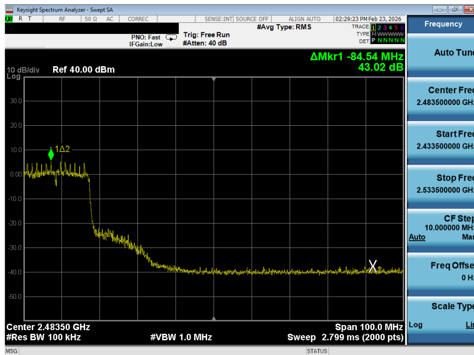
Plot 7-35. Band Edge Plot (802.11n (2.4GHz) – Ch. 7)
