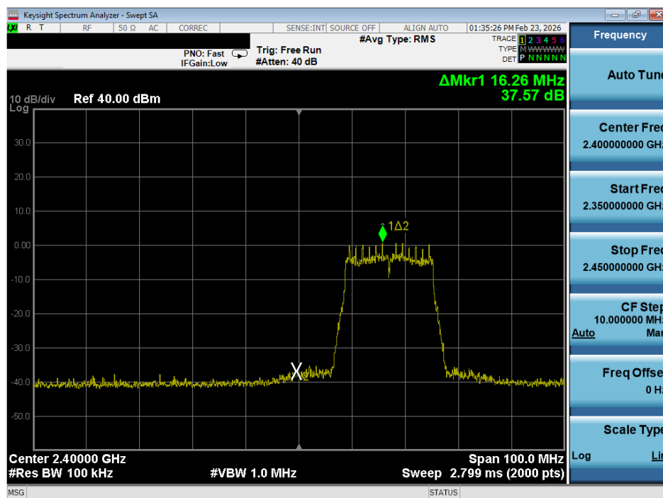
Plot 7-19. Band Edge Plot (802.11g – Ch. 2)
