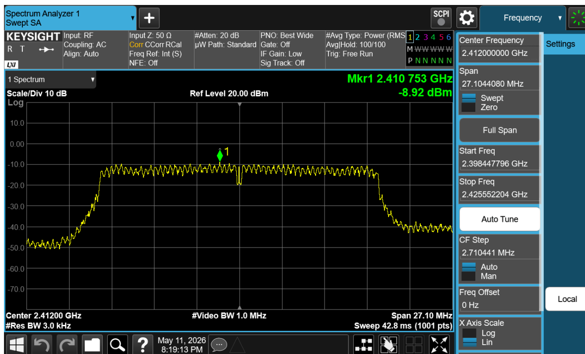
Plot 7-9 PSD (20MHz BW 802.11n - Ch.1)
