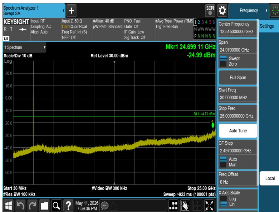
Plot 7-44. Conducted Spurious Plot (802.11b – Ch. 11)
