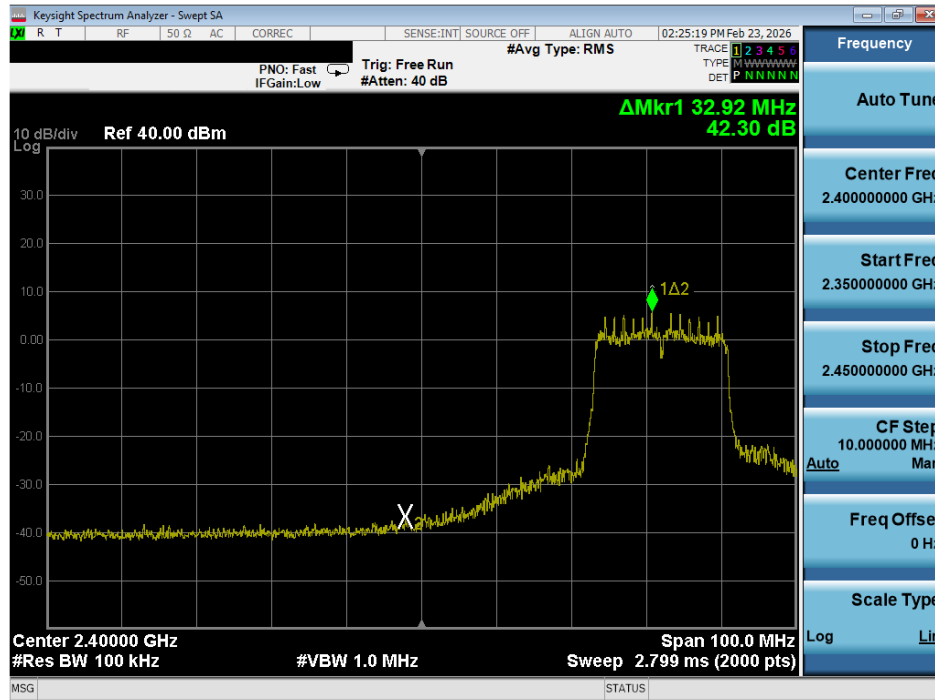
Plot 7-34. Band Edge Plot (802.11n (2.4GHz) – Ch. 5)
