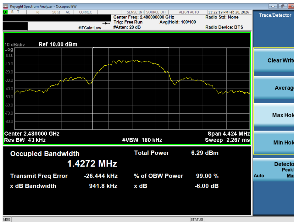
Plot 7-3. 99% OBW Plot (ANT+ – Ch. 79)
