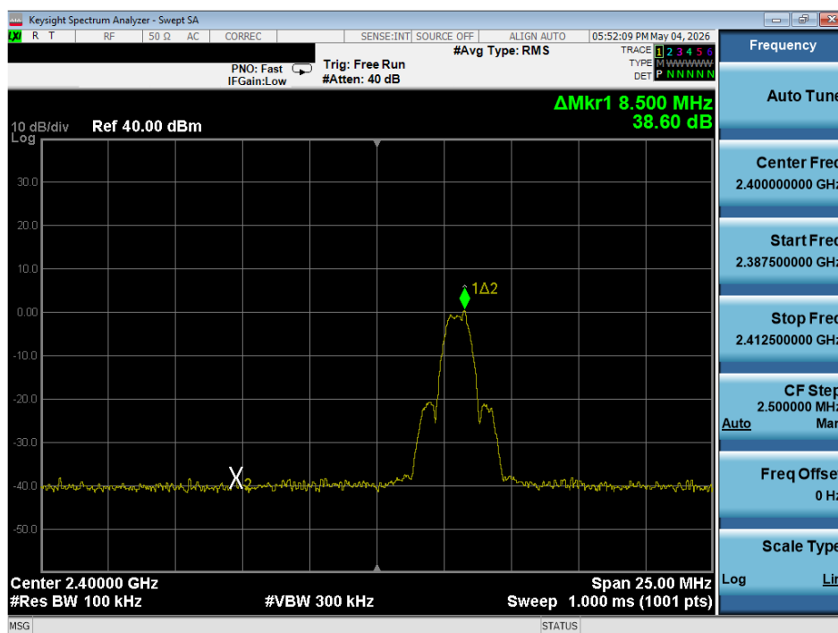
Plot 7-16. Band Edge Plot (ANT+ – Ch. 2)
