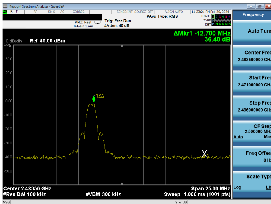
Plot 7-20. Band Edge Plot (ANT+ – Ch. 79)
