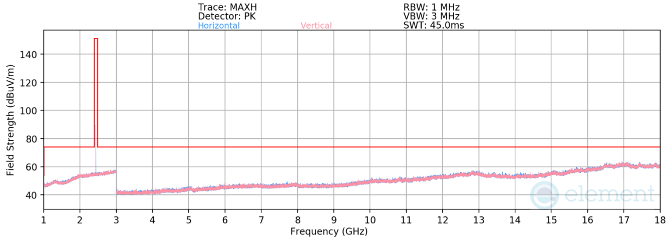
Plot 7-25. Radiated Spurious Emissions 1-18GHz (ANT+ – Ch. 39)
