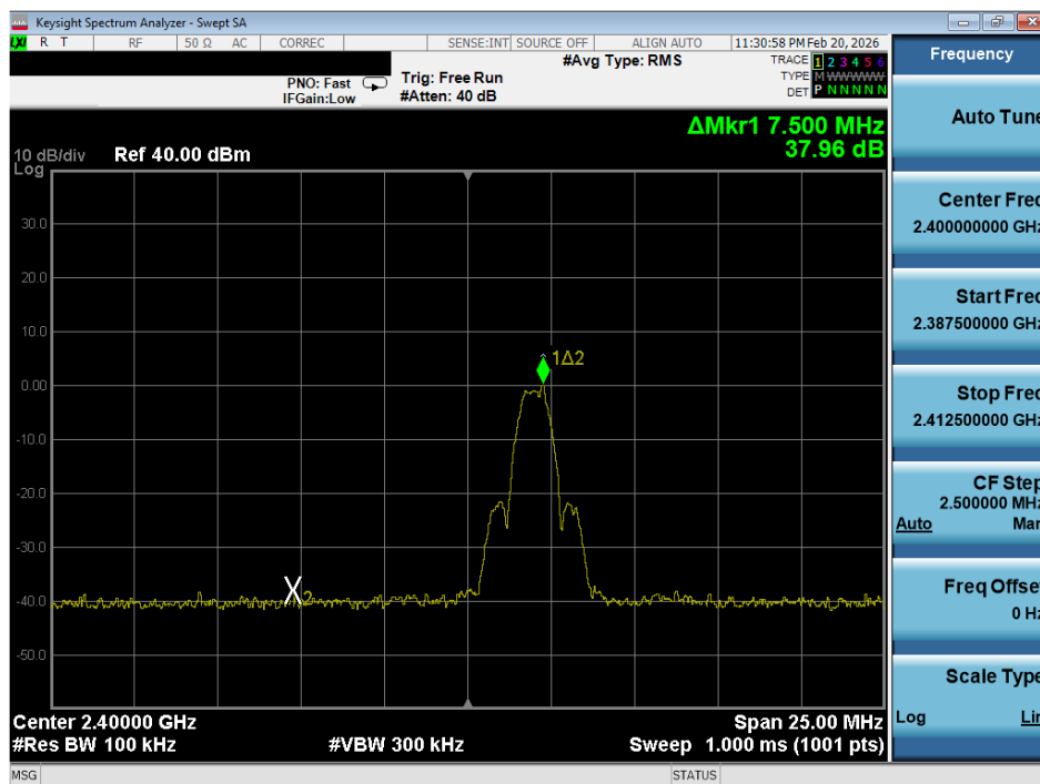
Plot 7-15. Band Edge Plot (ANT+ – Ch. 1)
