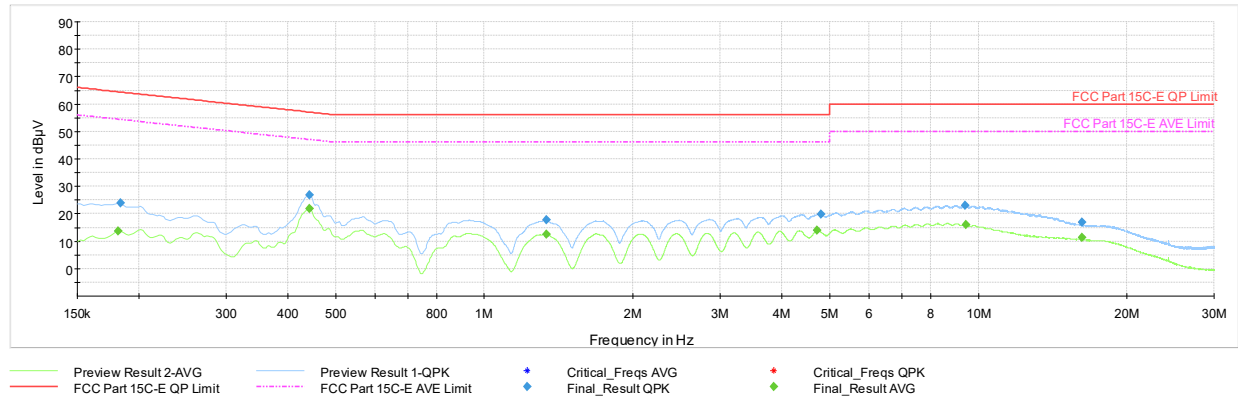
Plot 7-34. AC Line Conducted Plot with Bluetooth ANT+ (N, ANT+ - Ch.39 with AC/DC Adapter)
