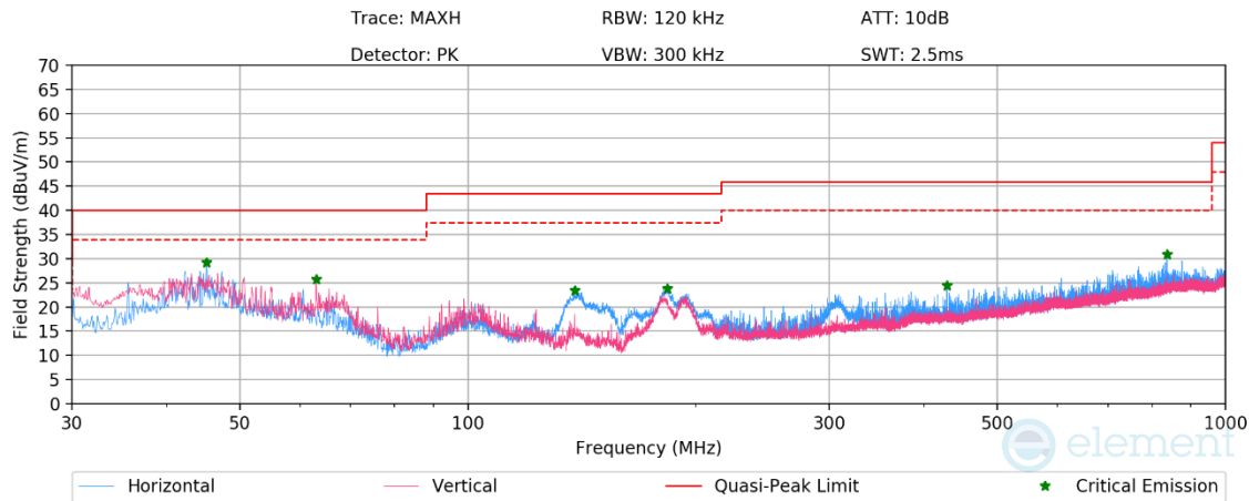
Plot 7-32. Radiated Spurious Emissions Below 1GHz (ANT+ – Ch.39 with AC/DC Adapter)
