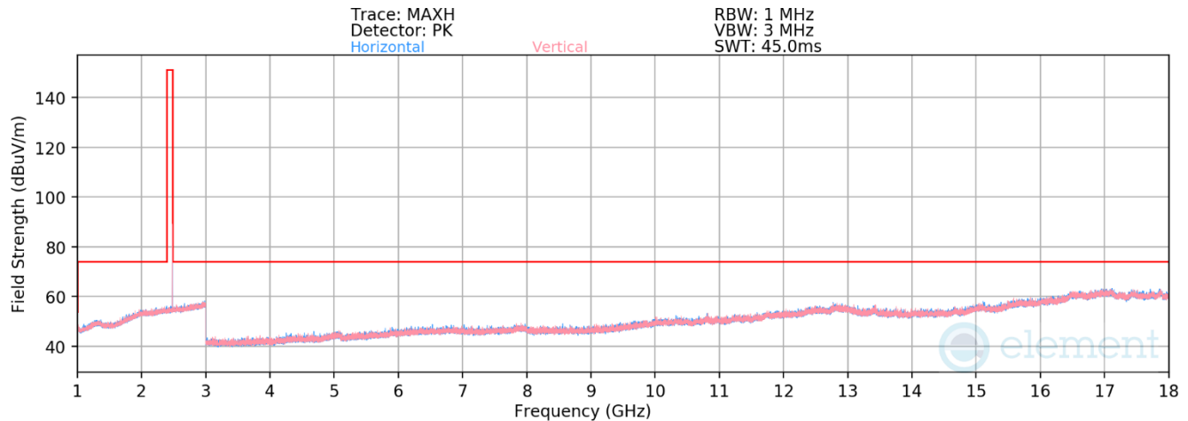
Plot 7-27. Radiated Spurious Emissions 1-18GHz (ANT+ – Ch. 79)
