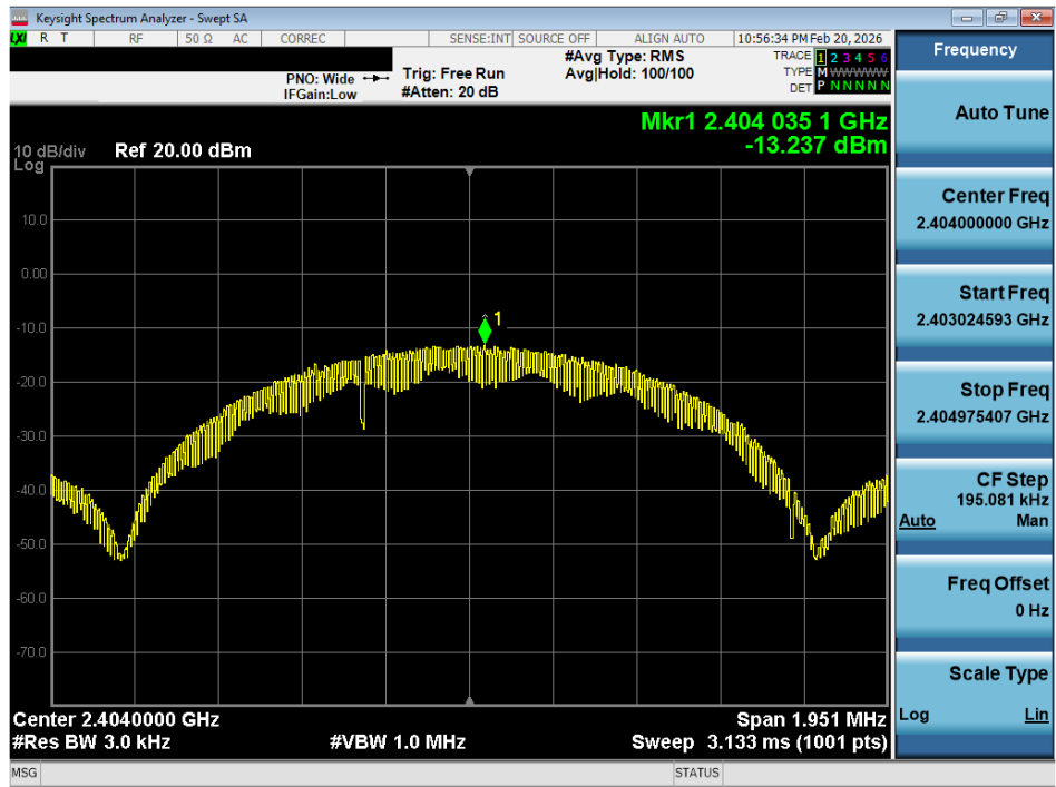
Plot 7-10. Power Spectral Density Plot (ANT+ – Ch. 3)
