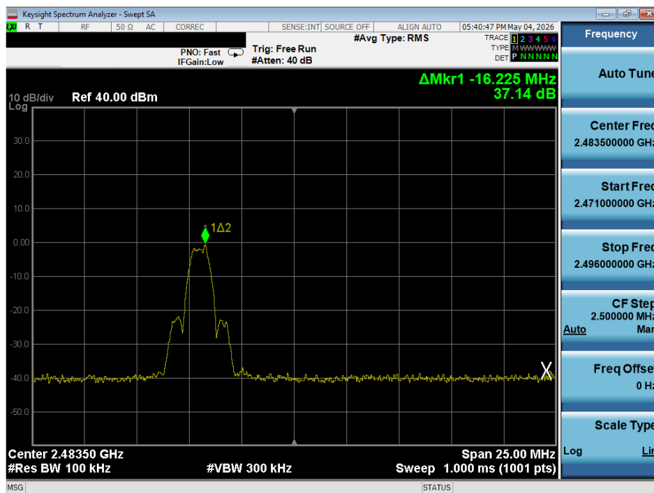
Plot 7-19. Band Edge Plot (ANT+ – Ch. 78)
