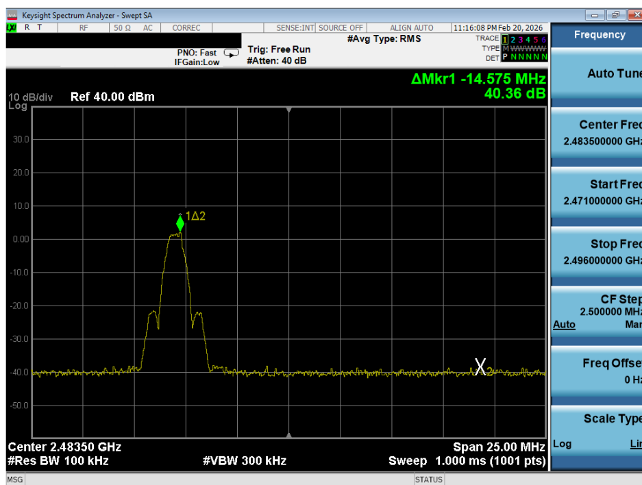
Plot 7-18. Band Edge Plot (ANT+ – Ch. 77)
