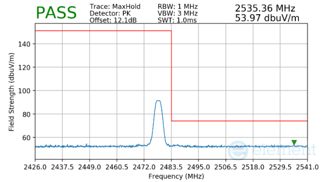
Plot 7-29. Radiated Restricted Upper Band Edge Measurement (Peak)
