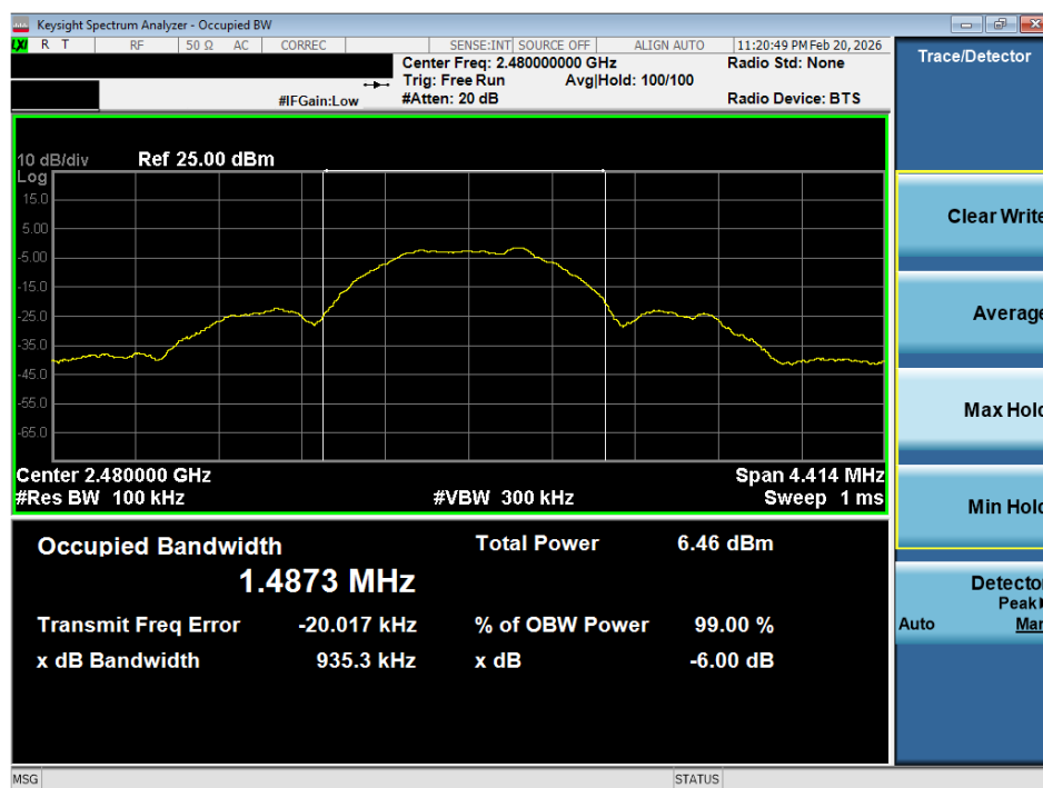
Plot 7-7. 6dB BW Plot (ANT+ – Ch. 79)
