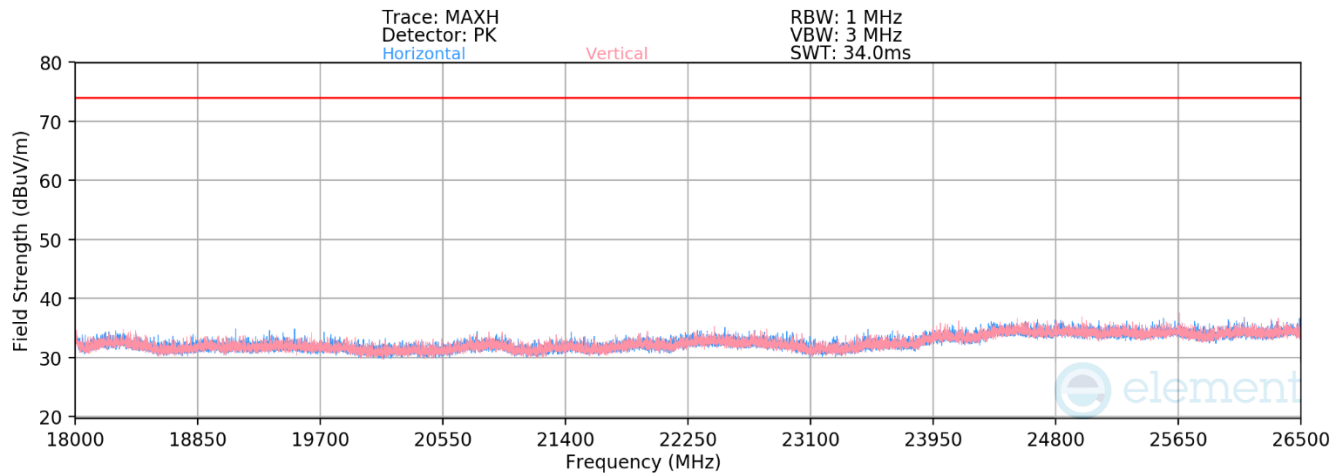
Plot 7-26. Radiated Spurious Emissions Above 18GHz (ANT+ – Ch. 39)
