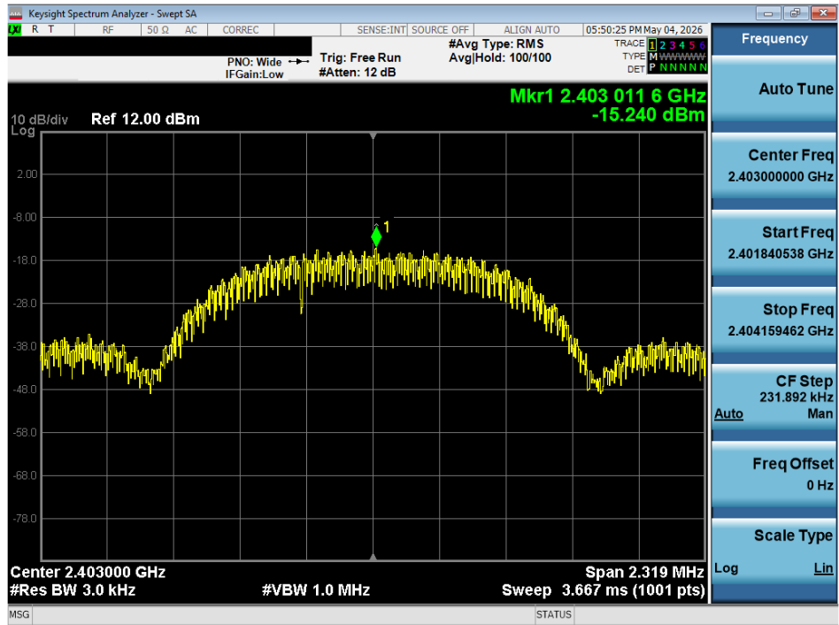
Plot 7-9. Power Spectral Density Plot (ANT+ – Ch. 2)
