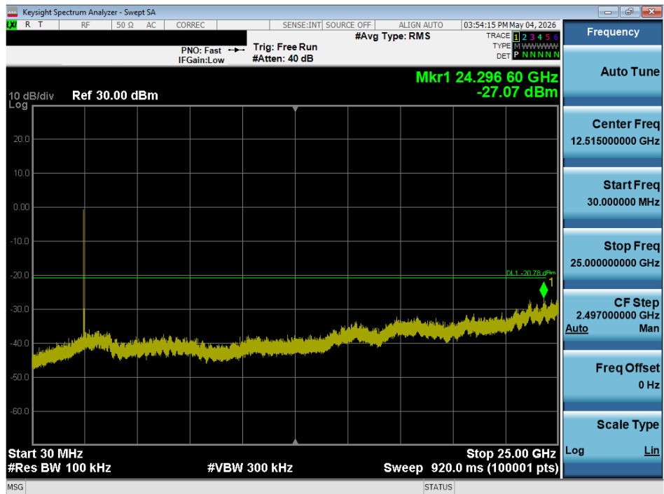
Plot 7-23. Conducted Spurious Plot (ANT+ – Ch. 79)
