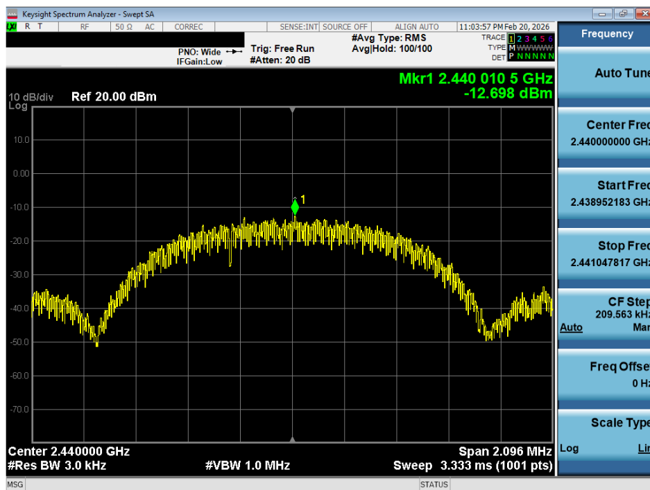
Plot 7-11. Power Spectral Density Plot (ANT+ – Ch. 39)
