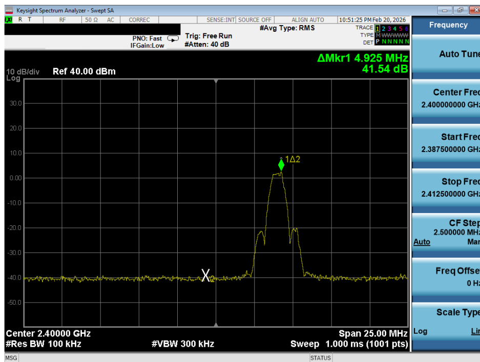
Plot 7-17. Band Edge Plot (ANT+ – Ch. 3)
