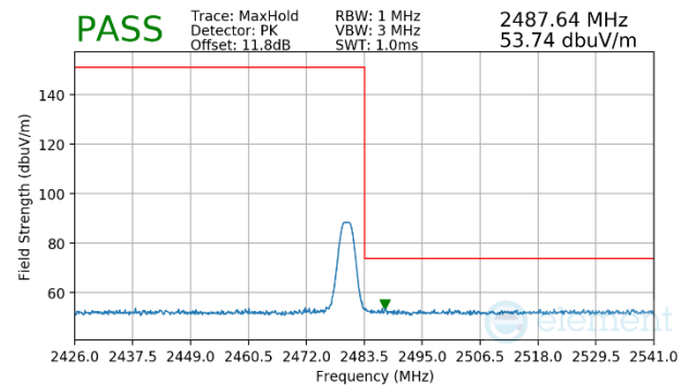
Plot 7-31. Radiated Restricted Upper Band Edge Measurement (Peak)
