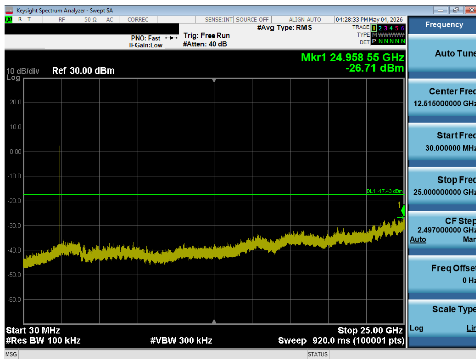
Plot 7-22. Conducted Spurious Plot (Bluetooth (ANT+ – Ch. 39)
