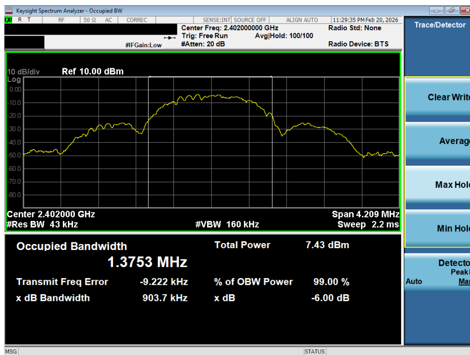
Plot 7-1. 99% OBW Plot (ANT+ – Ch. 1)
