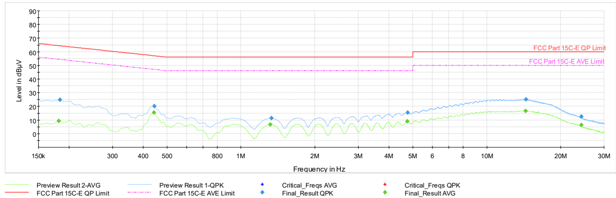
Plot 7-33. AC Line Conducted Plot with Bluetooth ANT+ (L1, ANT+ - Ch.39 with AC/DC Adapter)
