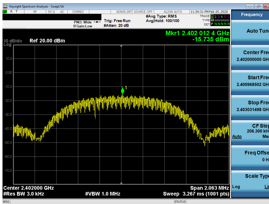
Plot 7-8. Power Spectral Density Plot (ANT+ – Ch. 1)
