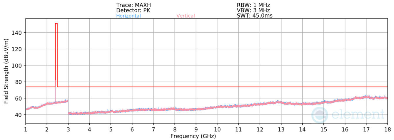
Plot 7-24. Radiated Spurious Emissions 1-18GHz (ANT+ – Ch. 1)
