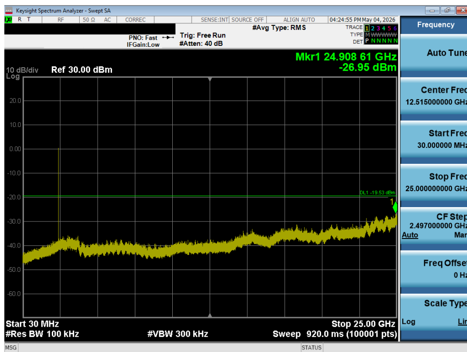
Plot 7-21. Conducted Spurious Plot (ANT+ – Ch. 1)
